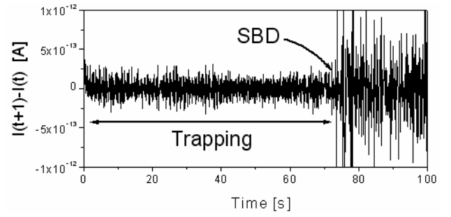
Fig. 6. Fluctuating behavior of the leakage current before and after the SBD event calculated from the upper curve shown in Fig. 5.
