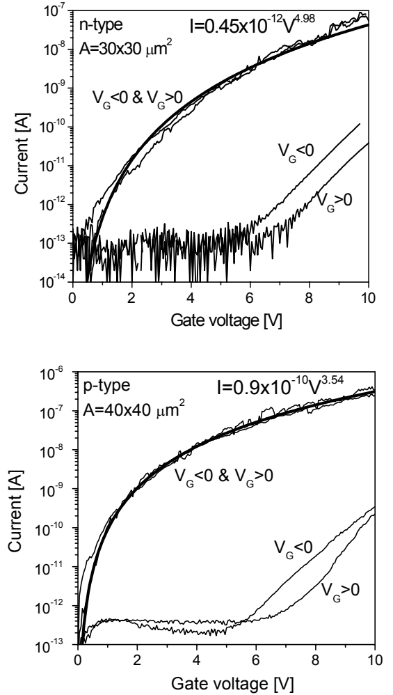
Fig. 4. Experimental (thin lines) and model (thick line) SBD I-V characteristics
