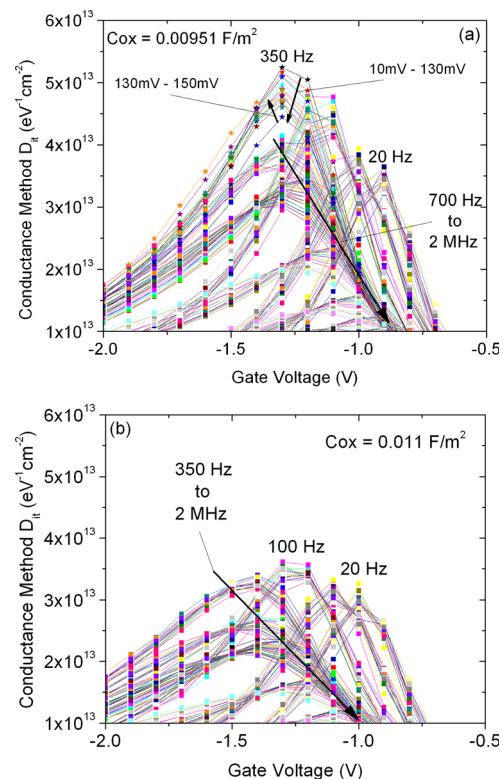
FIG. 2. (Color online) Sample S1 D_{it} extractions using the CM [Eq. (2)] for a C_{ox} of (a) 0.00951 F/m² and (b) 0.011 F/m² for 15 different AC voltage amplitudes (10–150 mV) for each of the 25 AC frequencies between 20 Hz and 2 MHz (see Table II). This illustrates the CM analysis technique carried out for all samples S1–S6 .
