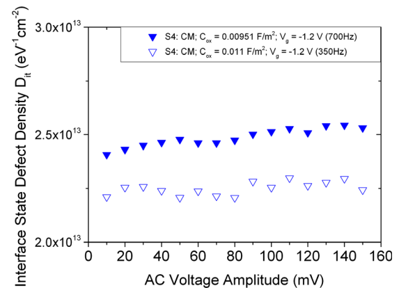
FIG. 8. (Color online) Sample S4 extracted D_{it} for the most appropriate gate voltage and AC frequency for each of the 15 different AC voltage amplitudes (10–150 mV). Results are summarized in Table III. CM extractions carried out for C_{ox} = 0.00951 \text{ F/m}^2 , V_g = -1.2 \text{ V} ( E - E_v \sim 0.41 \text{ eV} ), and at an AC frequency of 700 Hz; and CM extractions carried out for C_{ox} = 0.011 \text{ F/m}^2 , V_g = -1.2 \text{ V} ( E - E_v \sim 0.38 \text{ eV} ), and at an AC frequency of 350 Hz.
