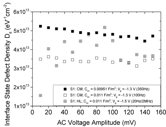
FIG. 5. Sample S1 extracted D_{it} for the most appropriate gate voltage and AC frequency for each of the 15 different AC voltage amplitudes (10–150 mV). Results are summarized in Table III. CM extractions carried out for C_{ox} = 0.00951 \text{ F/m}^2 , V_g = -1.3 \text{ V} ( E - E_v \sim 0.36 \text{ eV} ), and at an AC frequency of 350 Hz; CM extractions carried out for C_{ox} = 0.011 \text{ F/m}^2 , V_g = -1.3 \text{ V} ( E - E_v \sim 0.37 \text{ eV} ), and at an AC frequency of 100 Hz; and HL extractions carried out for C_{ox} = 0.011 \text{ F/m}^2 , V_g = -1.5 \text{ V} ( E - E_v \sim 0.36 \text{ eV} ), and AC frequencies of 20 Hz (LF) and 2 MHz (HF).
