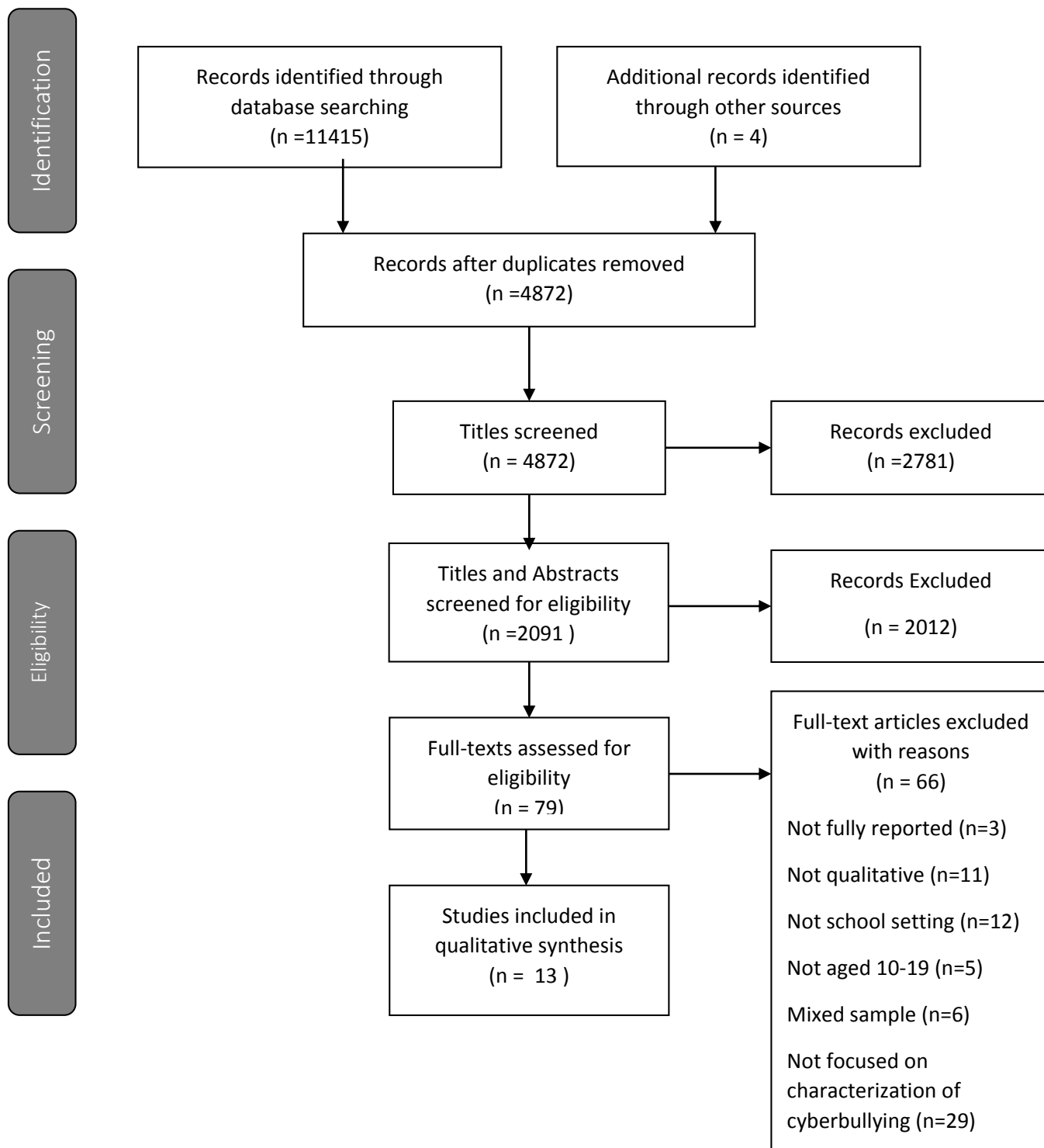
Figure 1 PRISMA Flow Diagram of Search Strategy
