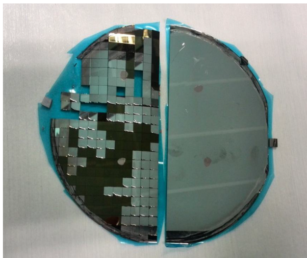
Figure 3.8: Planarised Silicon wafer with spun on BCB polymer coating.
