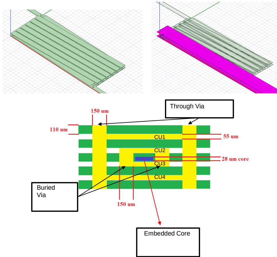
Figure 4.33: (Top Left) FEM of primary inductor structure with embedded released 32 layer CZT core for EU GaNonCMOS coupled inductor. (Top-Right) Primary and secondary windings for coupled inductor structure. (Bottom) Illustration of nested coupled inductor with embedded released thin film magnetic core in prepreg layers of PCB stack.
