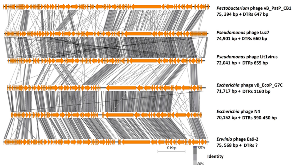
Figure 4. Comparison of the genomes of Pectobacterium phage CB1 with those phages representing the genera of N4virus , G7cvirus , Ea92virus , Lit1virus , and Luz7virus employing TBLASTX and visualized with Easyfig. Genome maps comprise of arrows indicating the locations of genes on the different phage genomes, and lines between genome maps indicate the level of homology.
