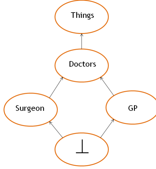
Figure 4.1: Concept hierarchy
