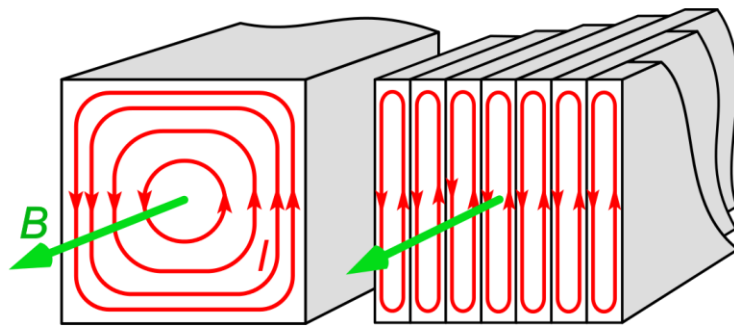
Figure 5 - Skin effect of single thickness core (left) and laminated core (right)
