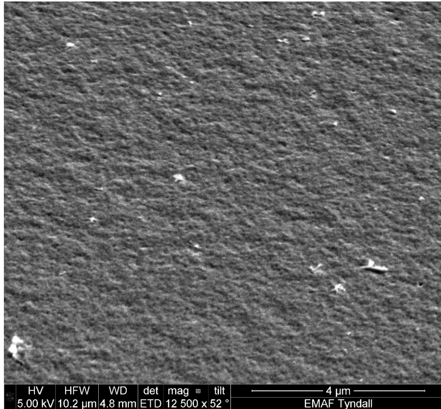
Figure 92 - AD CoNiFe Surface (58° Angle)
