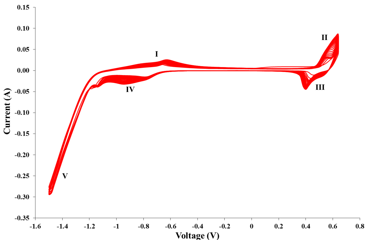
Figure 51 - Voltammogram of the \text{Ni}_{45}\text{Fe}_{55} electrode
