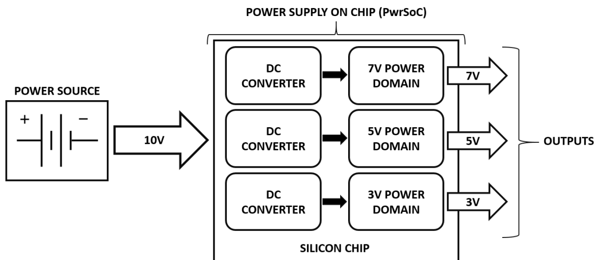
Figure 9 - Example of PwrSoC circuit setup
