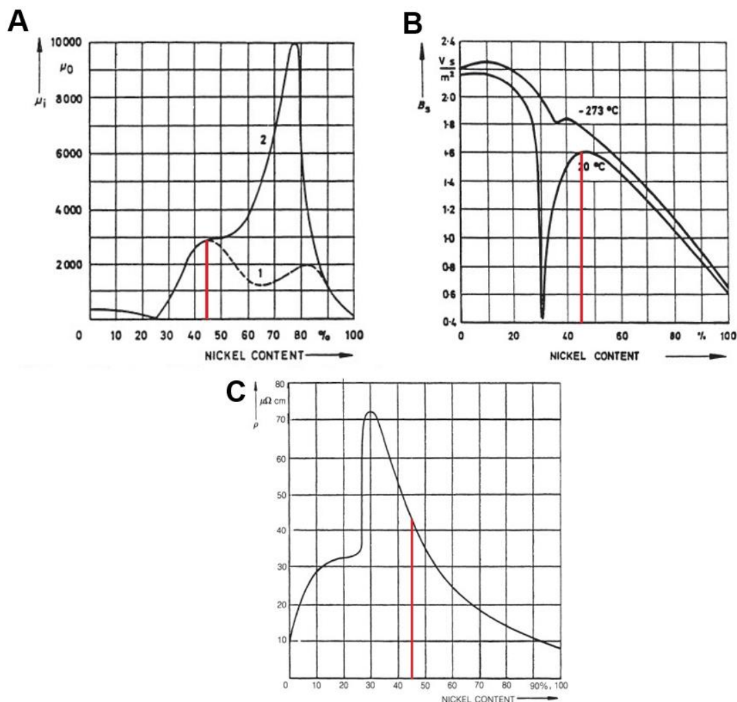
Figure 34: A - Permeability B - Saturation magnetic induction C - Electrical resistance of Ni alloys
