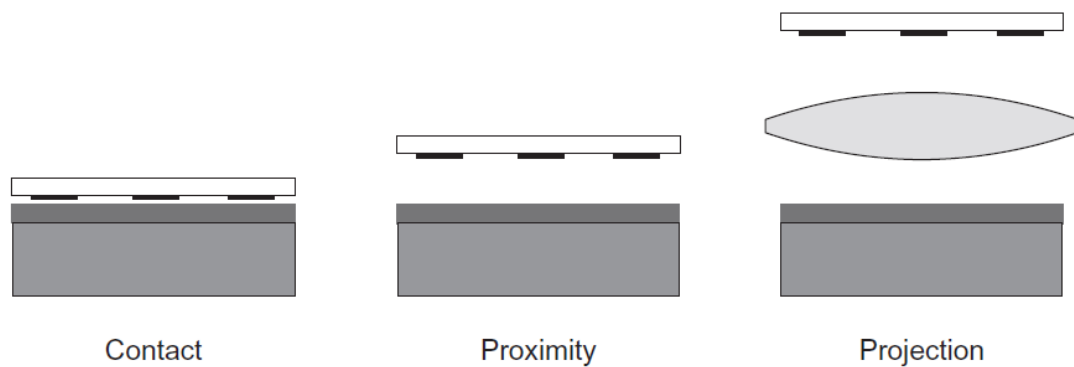
Figure 21 - Modes of contact for photolithography
