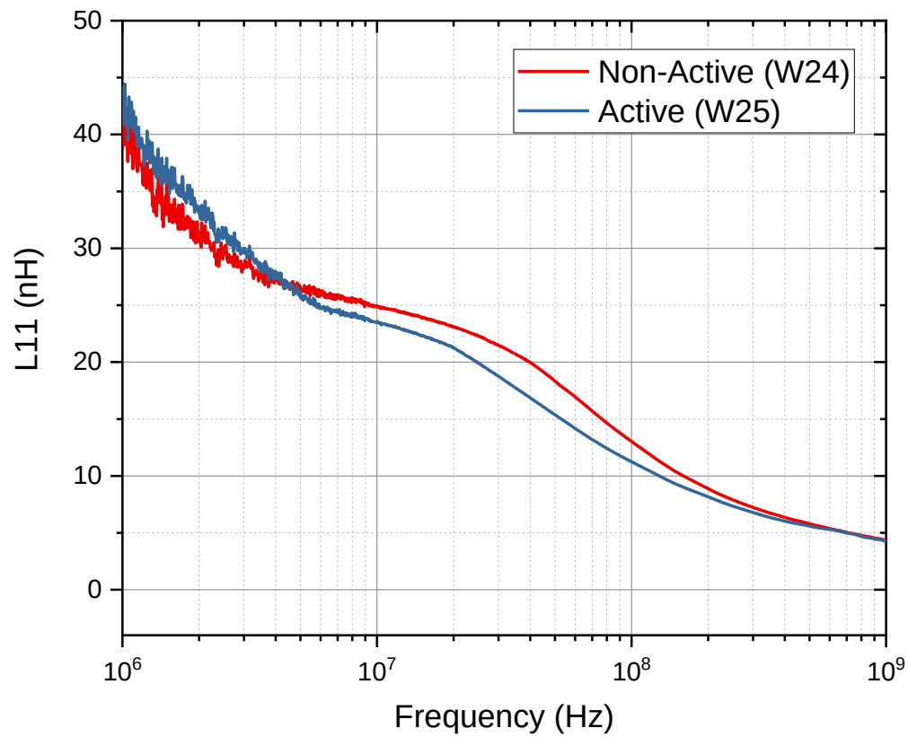
Figure 117 - Figure 116 - Inductance of CoNiFe MC2 Inductor Devices
