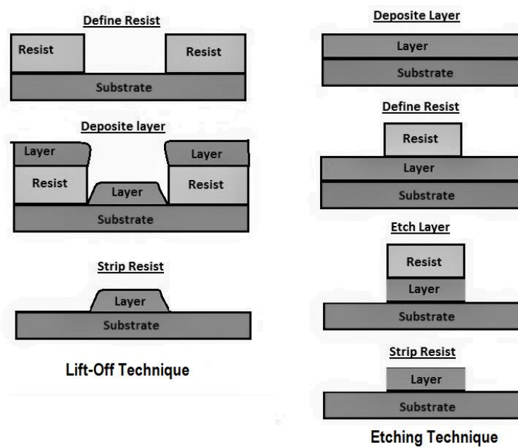
Figure 12 – Lift-off & Etch Photoresist techniques
