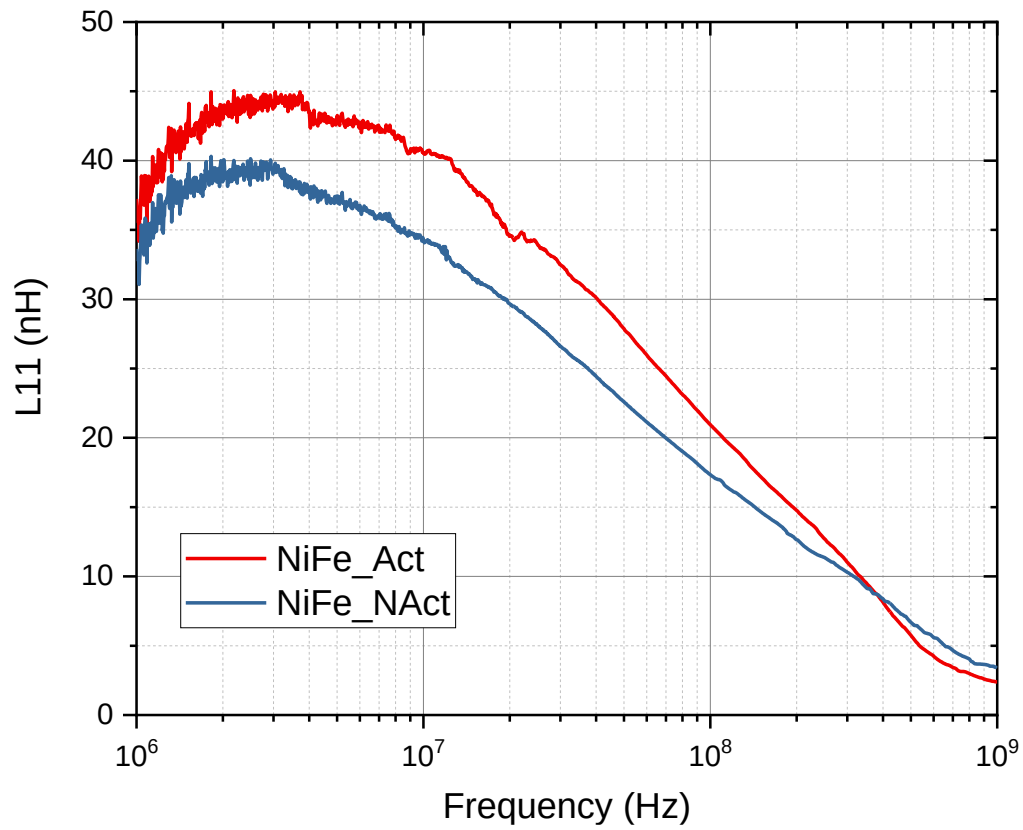
Figure 88 - Inductance of NiFe MC2 Inductor Devices
