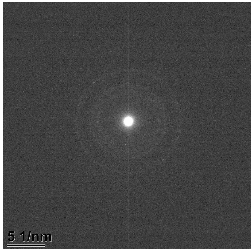
Figure 66 – SAED 1 of Oxi-NiFe
