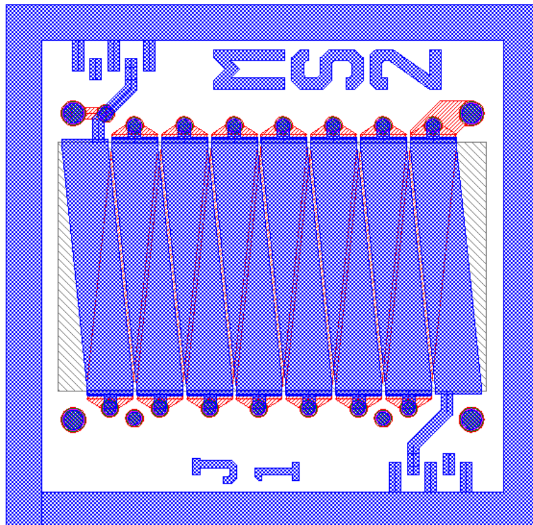
Figure 46 - MS2 Inductor Design
