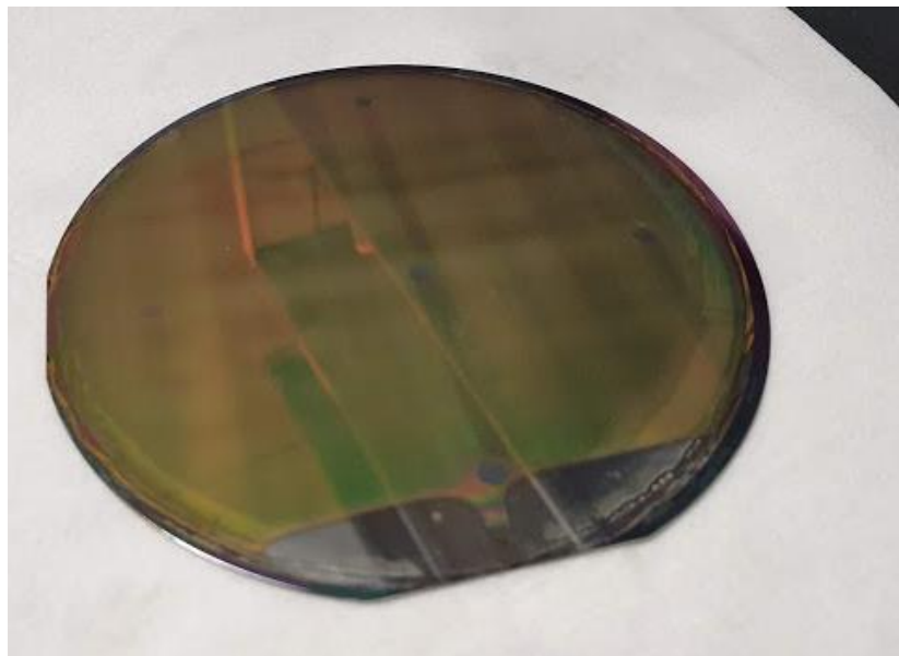
Figure 74 - NiFe wafer after oxidation, showing the iridescent colouring of Oxi-NiFe. Note the bottom of the wafer is AD NiFe - This area was not submerged in the bath and was used as the electrical connection point
