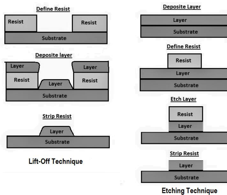
Figure 12 – Lift-off & Etch Photoresist techniques
