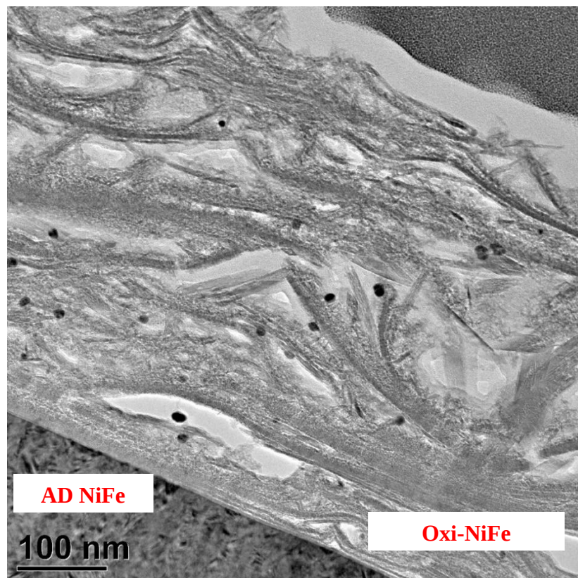
Figure 63 – 100nm scaling showing a 1 \mu m thick layer of Oxi-NiFe on top of AD NiFe
