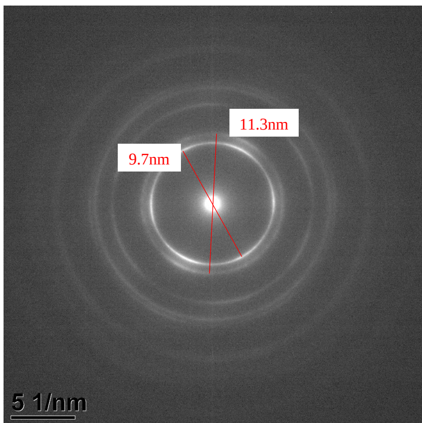
Figure 99 - SAED of AD CoNiFe
