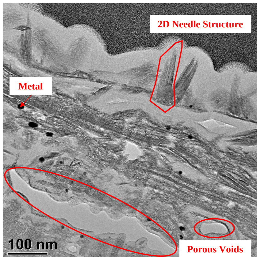
Figure 64 – 100nm scaling, showing the surface of Oxi-NiFe & the needle-like grains
