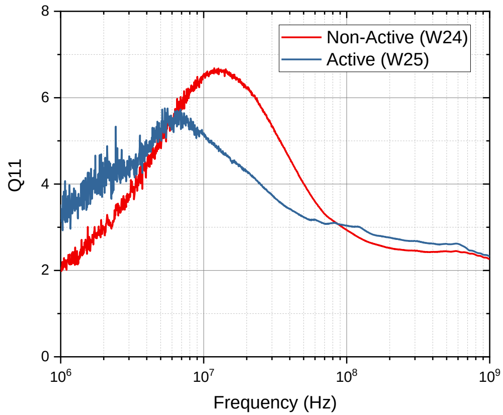
Figure 119 - Q-Factor of CoNiFe MC2 Inductor Devices
