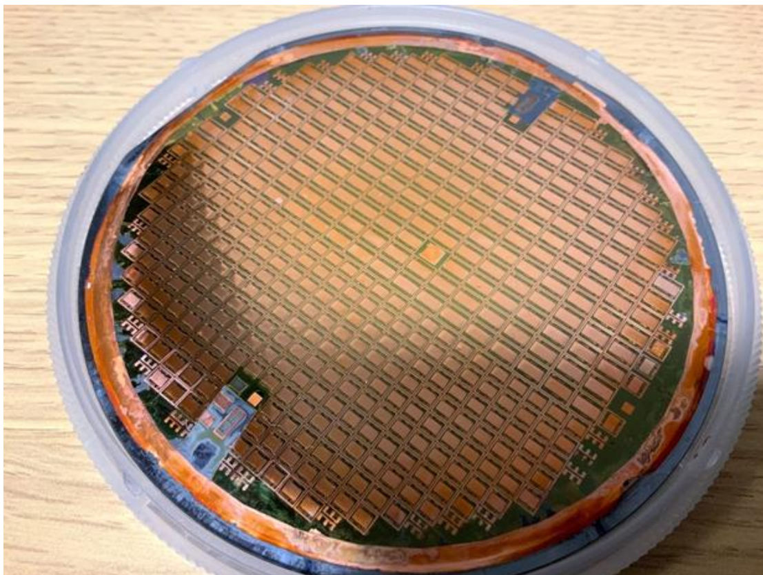
Figure 77 – Fully Constructed Oxi-CoNiFe Device Wafer
