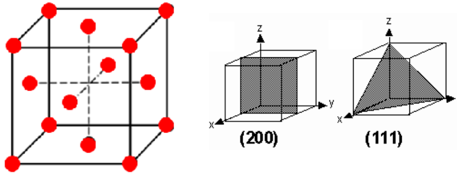
Figure 62 - Face centred cubic lattice, with (200) & (111) crystal planes
