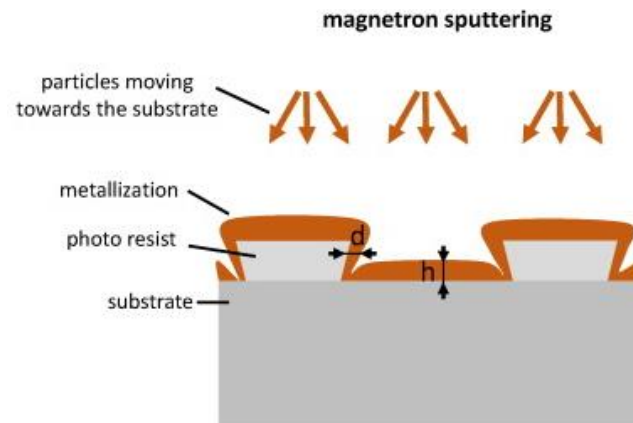
Figure 26 - Sputter deposition for lift-off technique
