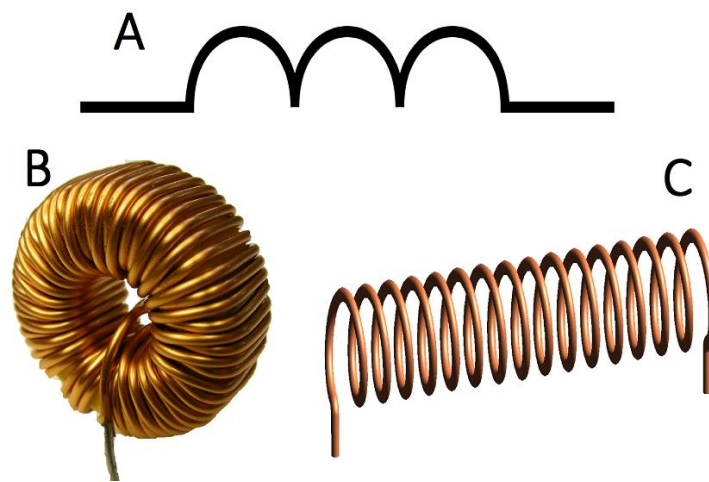
Figure 1 - (a) Inductor circuit element symbol (4) (b) Toroidal ferrite inductor (5) (c) Solenoid air inductor (6)
