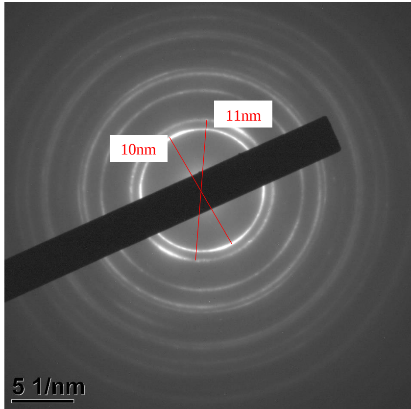
Figure 61 – SAED of AD NiFe with selected area aperture
