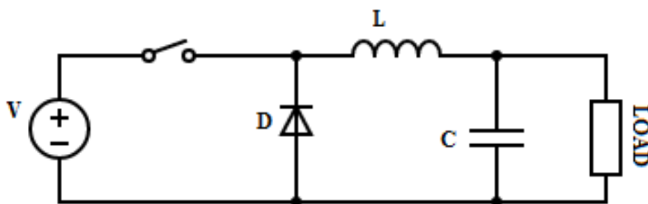
Figure 6 - Circuit diagram for a simple buck converter
