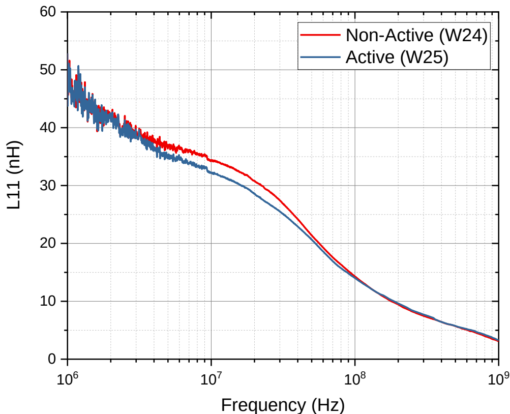
Figure 108 - Inductance of CoNiFe MS1 Inductor Devices
