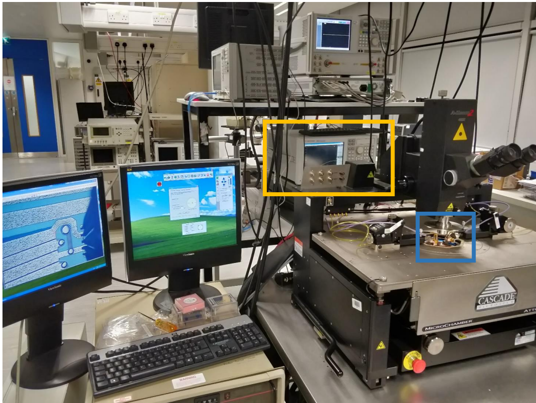
Figure 43 - Probe Station for testing of devices on a device wafer. Orange Box indicates the Network Analyser and the Blue Box indicates the RF Probes and device wafer holder.
