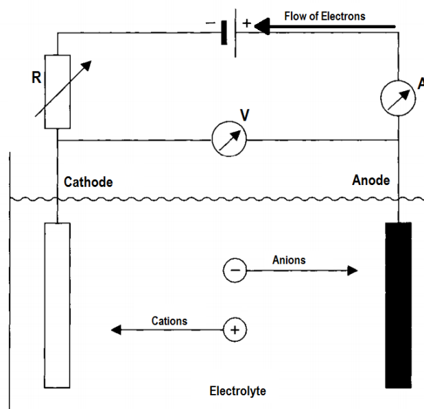
Figure 30 - Diagram of a basic electroplating setup
