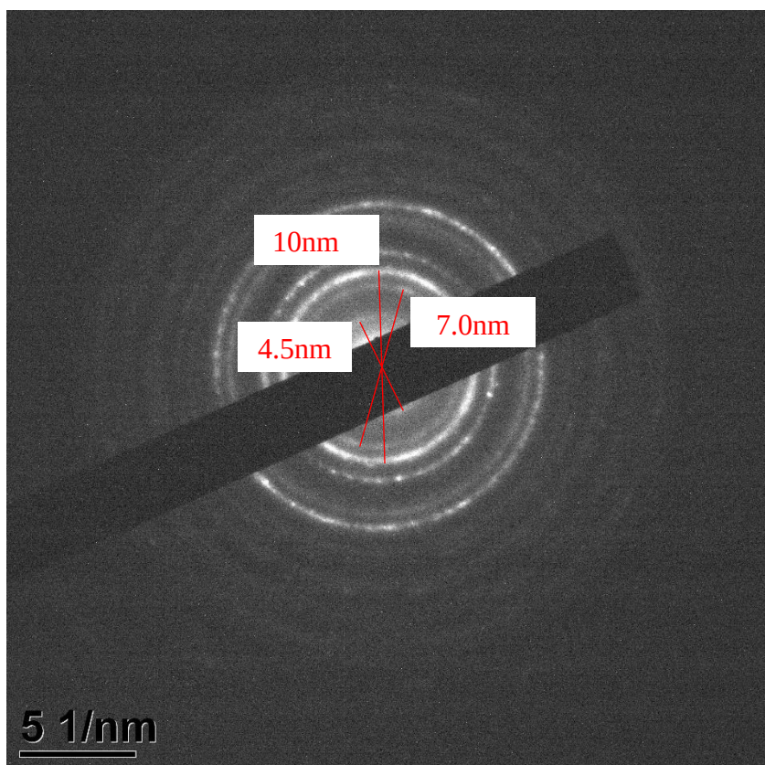
Figure 105 - SAED of CoNiFe with selected area aperture
