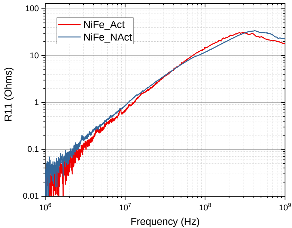
Figure 80 - AC Resistance of NiFe MS1 Inductor Devices
