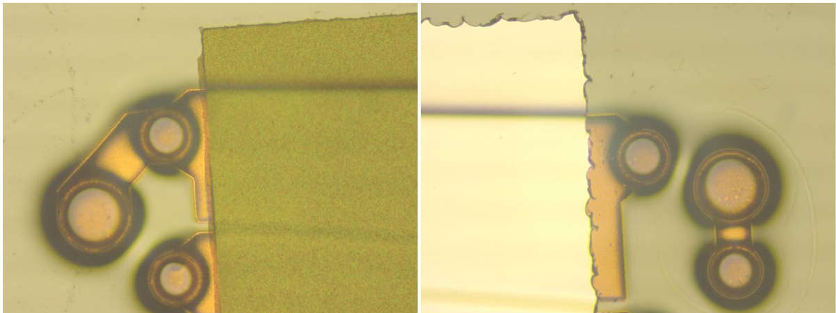
Figure 70 - Light microscope image of the vias and cores of the oxidised devices (left) and as-deposited devices (right)
