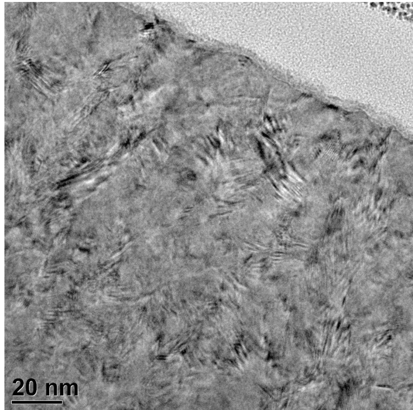
Figure 97 - 20nm scaling of the top surface of AD CoNiFe
