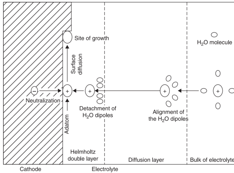
Figure 29 - Movement of ions through the bulk electrolyte, diffusion layer and double layer
