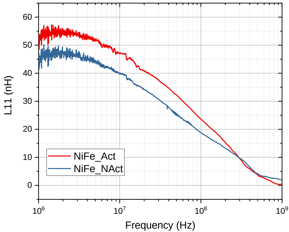
Figure 82 - Inductance of NiFe MS2 Inductor Devices
