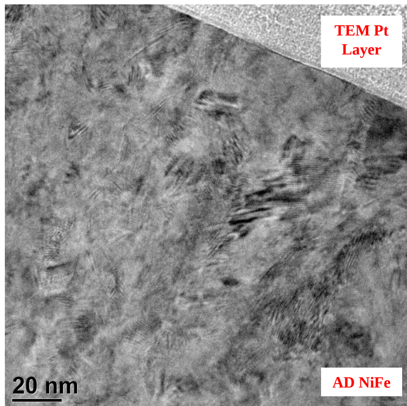
Figure 58 – Top Section of AD NiFe layer, with Sputtered Pt Layer for TEM Analysis
