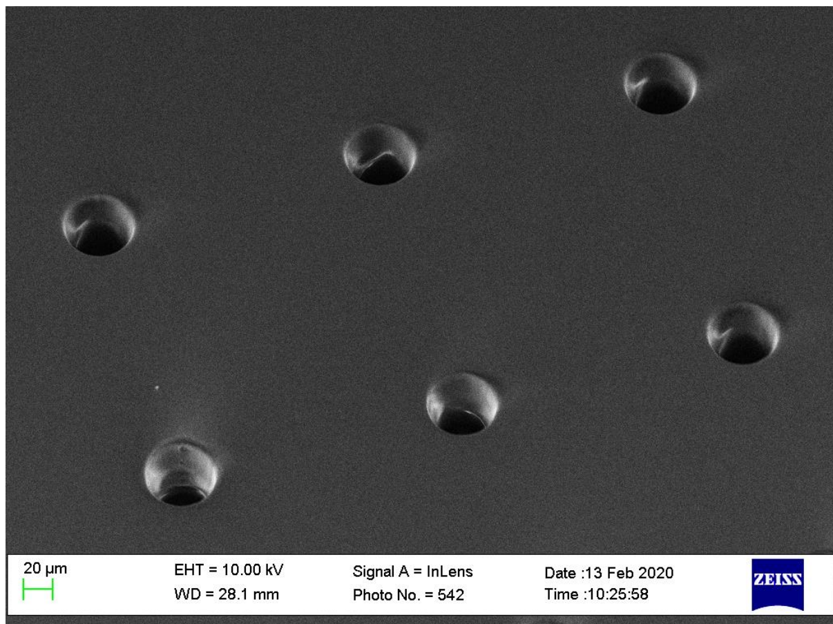
Figure 11 - Patterned and developed photoresist layer containing via holes
