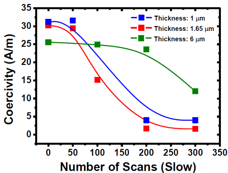
Figure 49 – Coercivity measured at different stages of post-processing (slow cycles) for different film thickness
