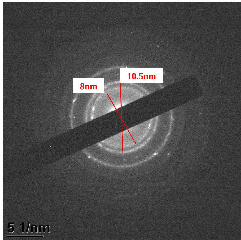
Figure 67 – SAED 2 of Oxi-NiFe with a selected area aperture
