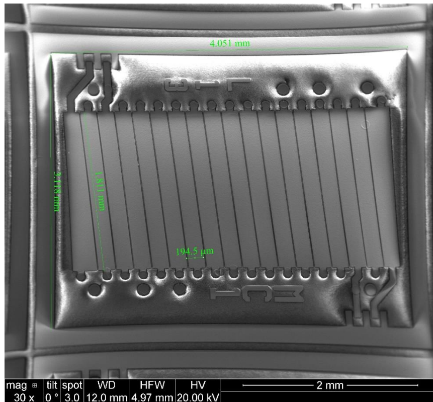
Figure 71 – MC1 coupled inductor with measurements
