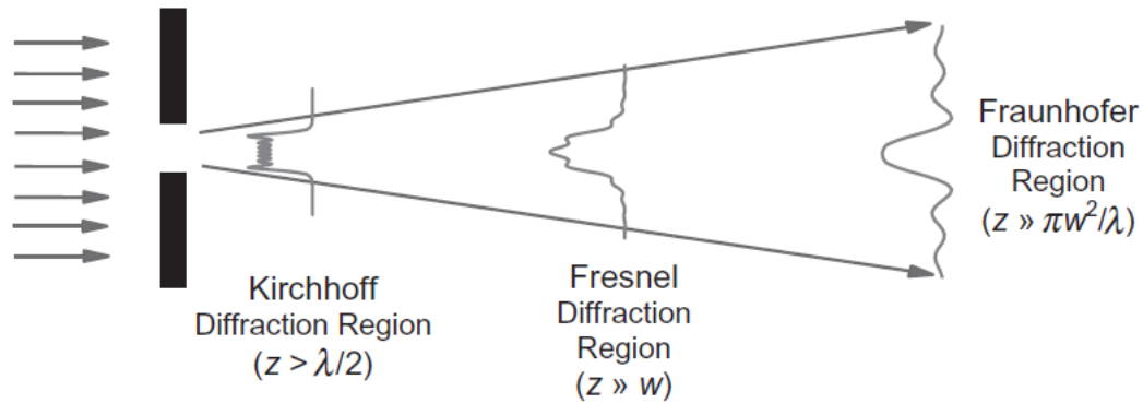
Figure 22 - Forms of diffraction seen in photolithography
