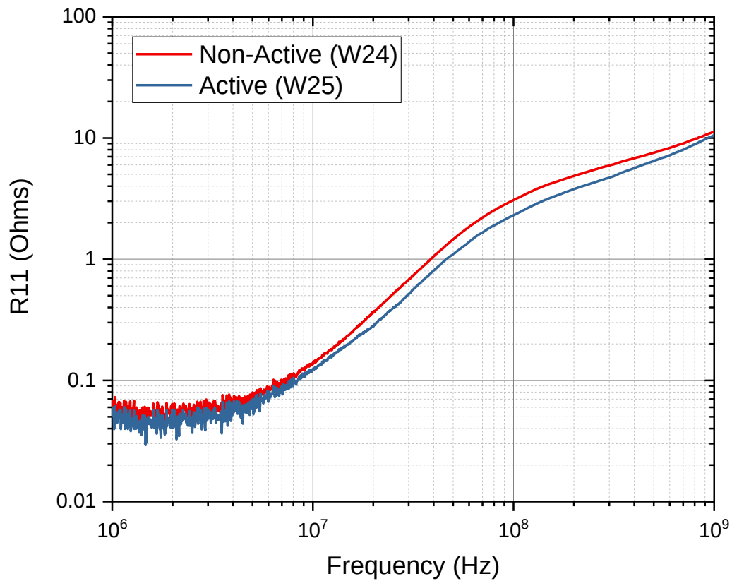
Figure 112 - AC Resistance of CoNiFe MS2 Inductor Devices
