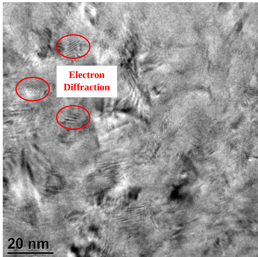
Figure 59 – Large portion of nanocrystalline AD NiFe grains
