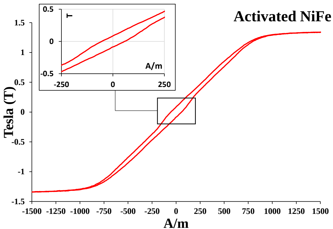
Figure 69 - Hysteresis Loop of 1.5cm x 1.5cm sample of Oxi-NiFe
