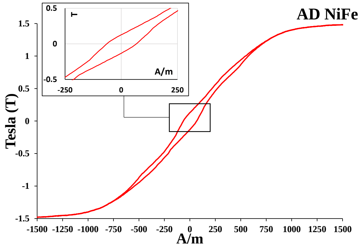
Figure 68 - Hysteresis Loop of 1.5cm x 1.5cm AD NiFe
