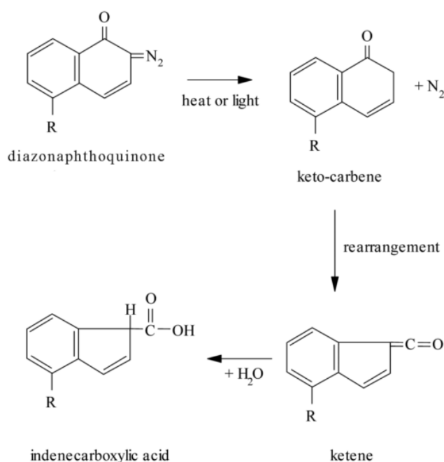
Figure 17 - Diazonaphthoquinone's reaction mechanism to form an indene carboxylic acid
