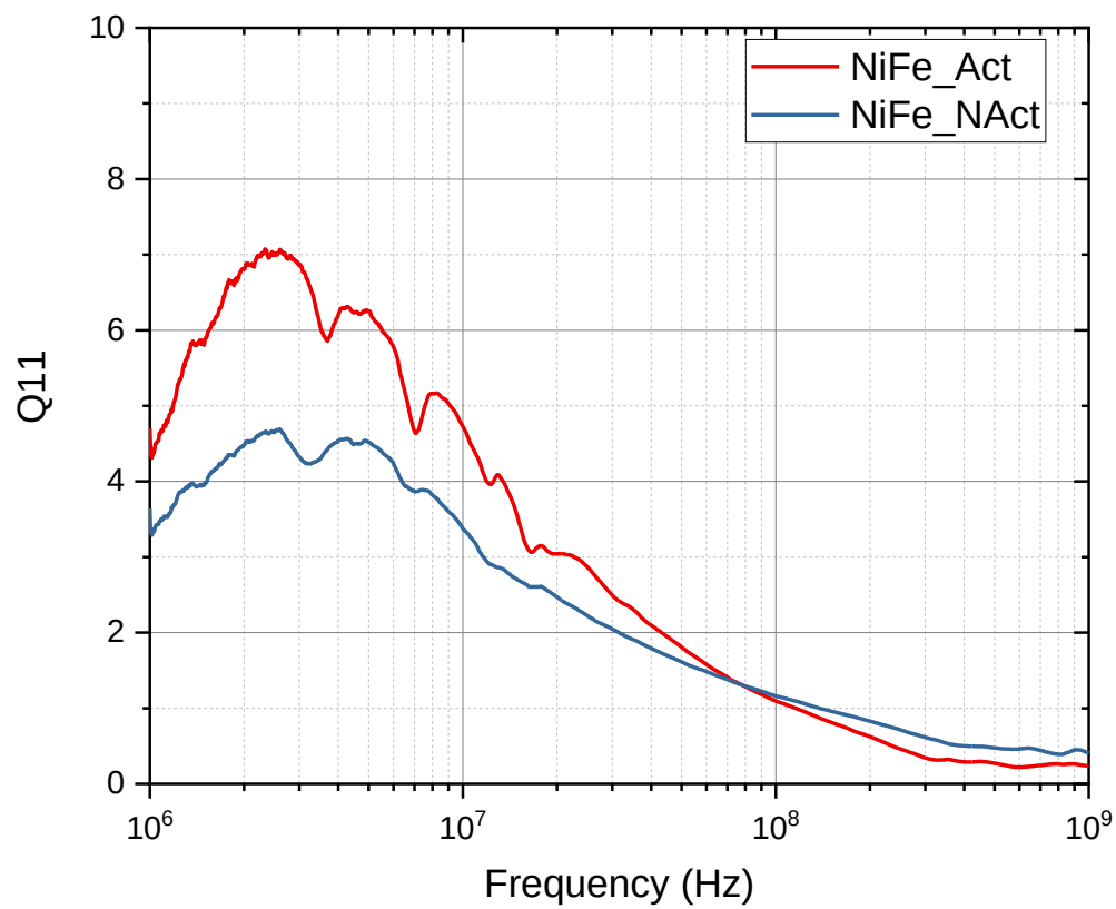
Figure 87 - Q-Factor of NiFe MC1 Inductor Device
