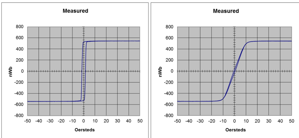
Figure 4 - Hysteresis loop of the easy axis (left) and hard axis (right) of anisotropic \text{Ni}_{45}\text{Fe}_{55}
