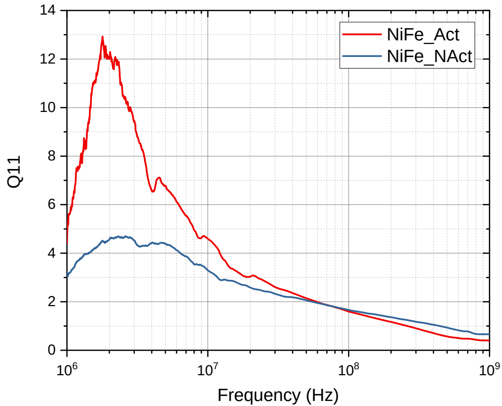
Figure 90 - Q-Factor of NiFe MC2 Inductor Devices
