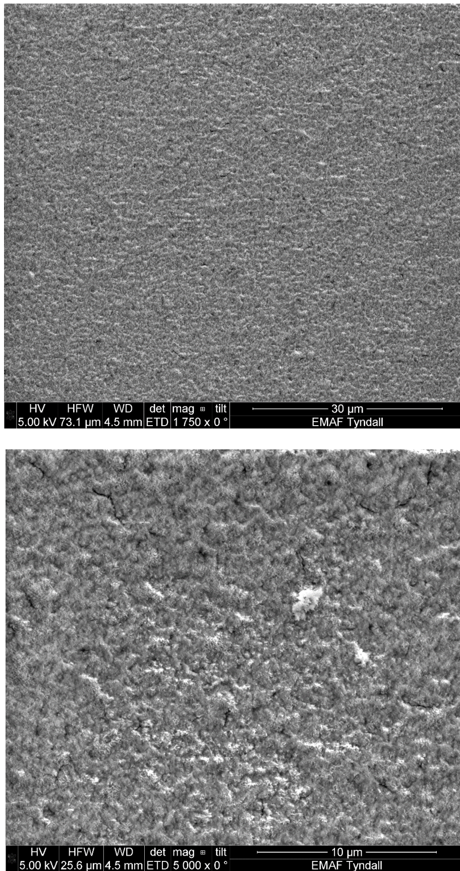
Figure 55 – Oxi-NiFe Surface – 1750x Mag (Top) & 5000x Mag (Bottom)
