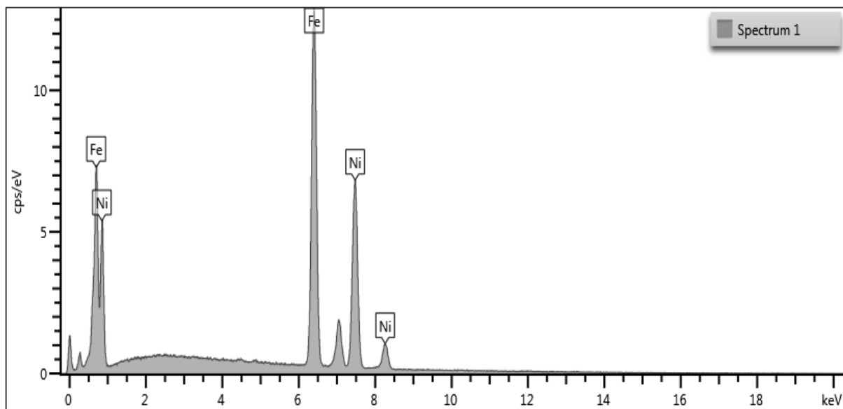
Figure 56 - EDX Spectrum of AD NiFe
