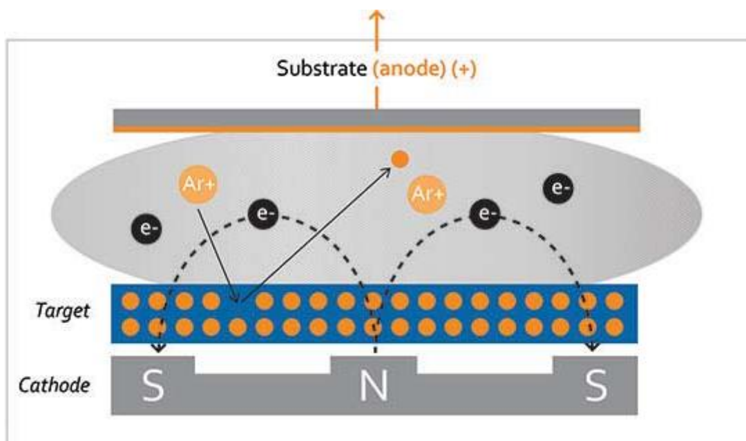
Figure 25 - Diagram of a Magnetron Sputter Deposition System
