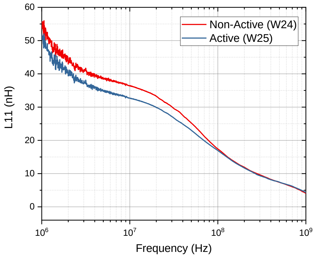
Figure 114 - Inductance of CoNiFe MC1 Inductor Devices
