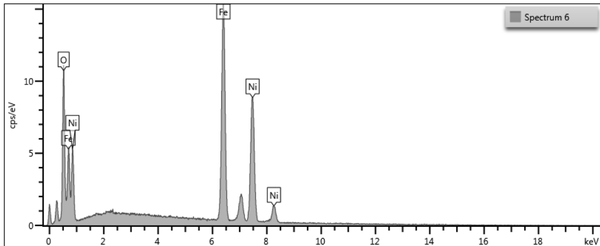
Figure 57 - EDX Spectrum of Oxi-NiFe
