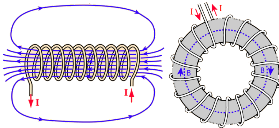
Figure 2 - (a) Solenoid's magnetic field lines (b) Toroidal's magnetic field lines
