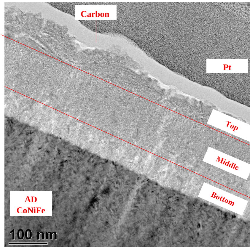
Figure 101 - 0.5µm Oxi-CoNiFe & its interphases between AD CoNiFe & TEM Pt / C Layers
