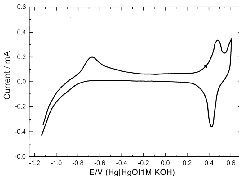
Figure 39 - Voltammogram of nickel in 1M KOH between -1.15V and +0.6V
