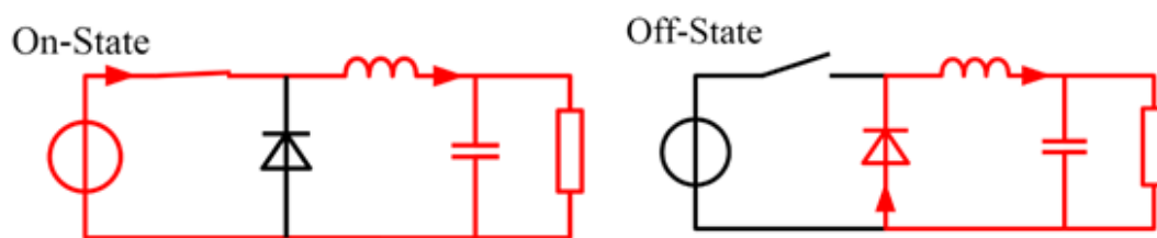
Figure 7 - ON (a) & OFF (b) State of a buck converter
