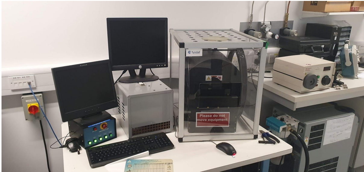
Figure 42 – Tyndall's MESA HF200P BH Looper system
