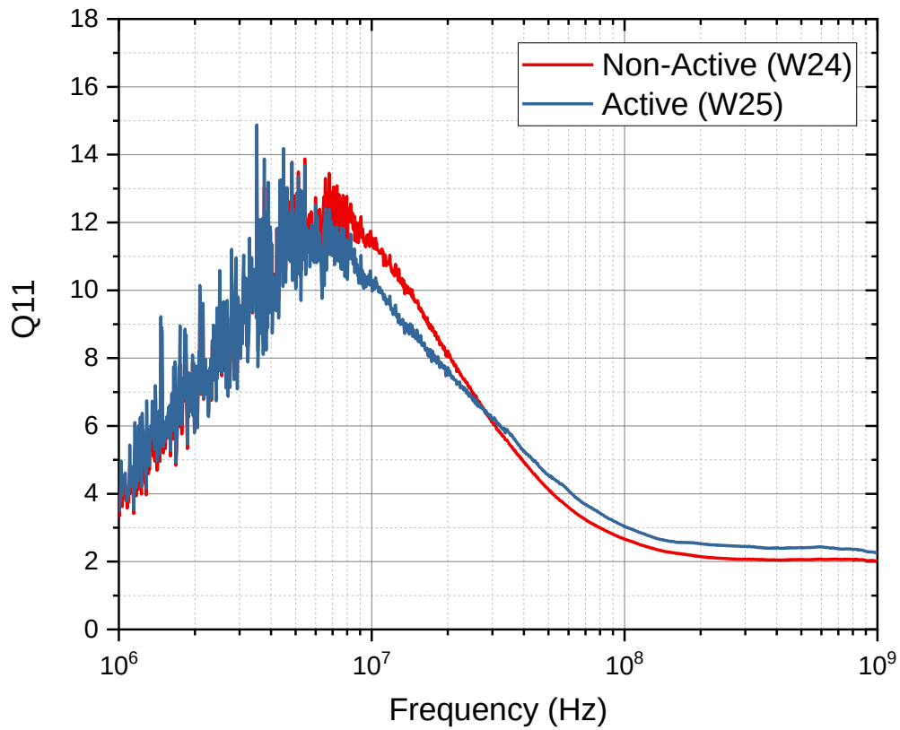
Figure 113 - Q-Factor of CoNiFe MS2 Inductor Devices
