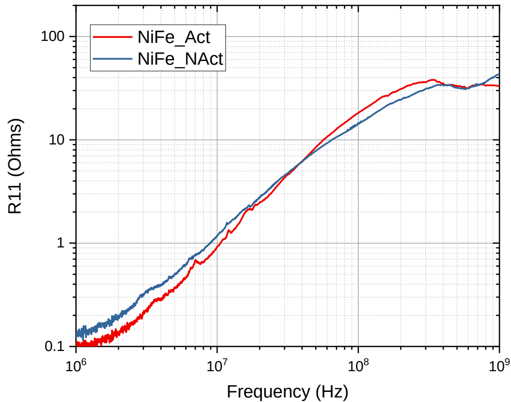
Figure 86 - AC Resistance of NiFe MC1 Inductor Devices
