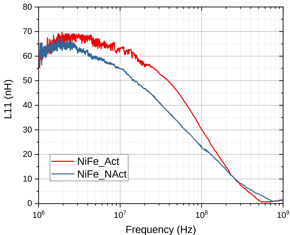
Figure 79 - Inductance of NiFe MS1 Inductor Devices
