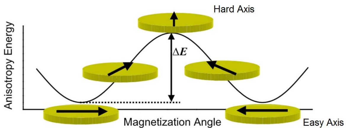
Figure 33 – Anisotropy energy relative to the magnetization angle
