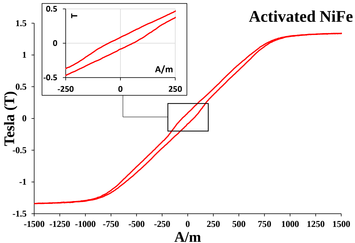
Figure 69 - Hysteresis Loop of 1.5cm x 1.5cm sample of Oxi-NiFe
