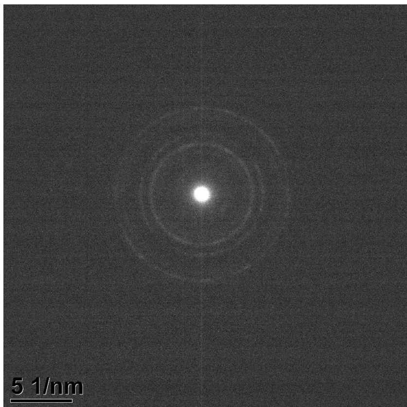
Figure 104 - SAED of Oxi-CoNiFe
