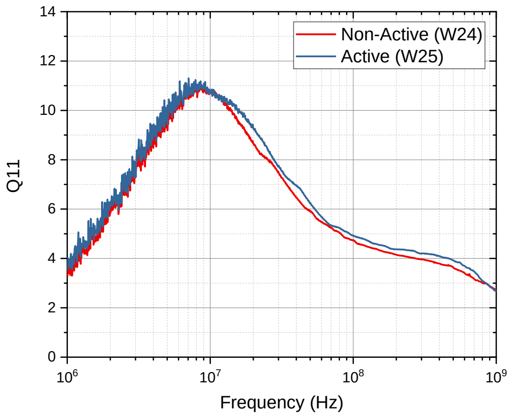
Figure 110 - Q-Factor of CoNiFe MS1 Inductor Devices
