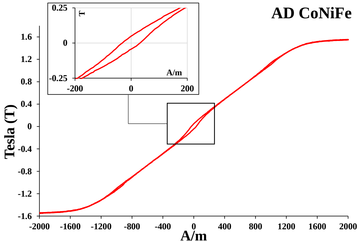
Figure 106 - Hysteresis Loop of 1.5cm x 1.5cm sample of AD CoNiFe
