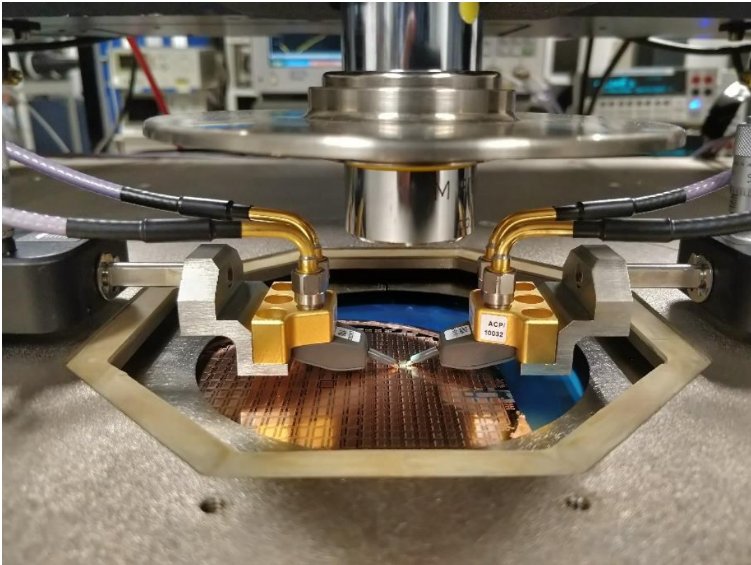
Figure 44 - Testing of a device at the wafer level. The device was contacted by the Formfactor ACP 100 Rf Probes in order to create a circuit.
