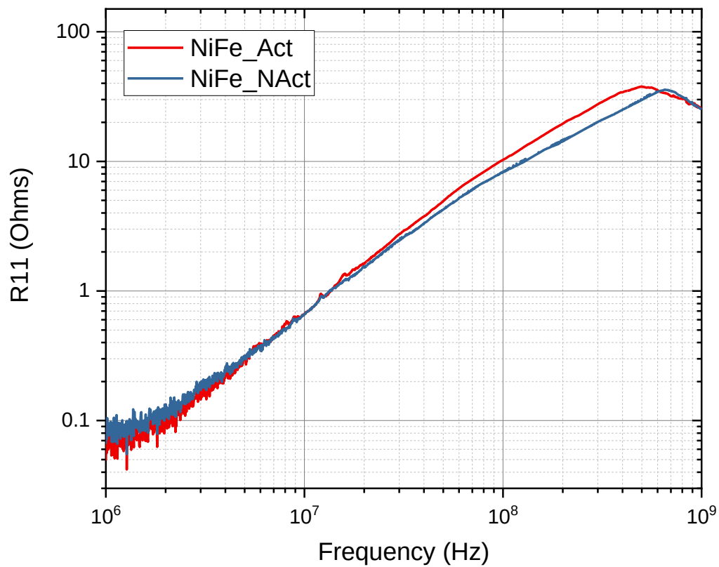
Figure 83 - AC Resistance of NiFe MS2 Inductor Devices
