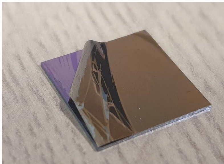
Figure 24 - Delamination of NiFe from the silicon substrate
