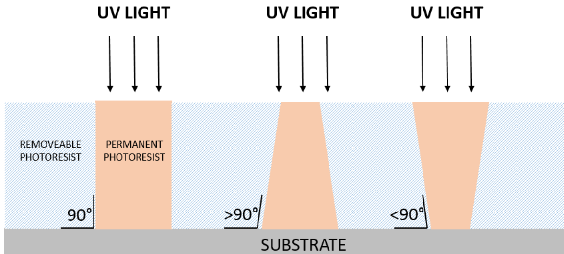
Figure 13 - Left: Sidewall of 90° Centre: Sidewall of >90° Right: Sidewall of <90°
