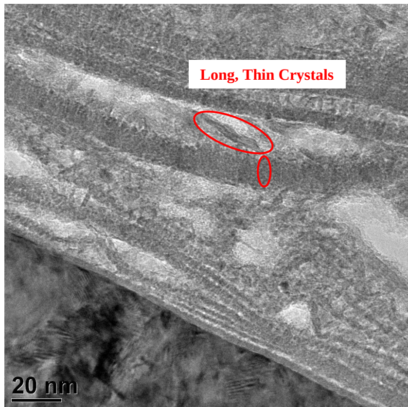
Figure 65 – 20nm scaling, showing the interphase between the two NiFe materials
