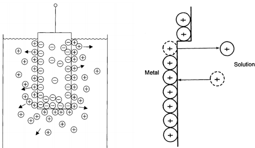
Figure 27 - Metal - Ion interphase
