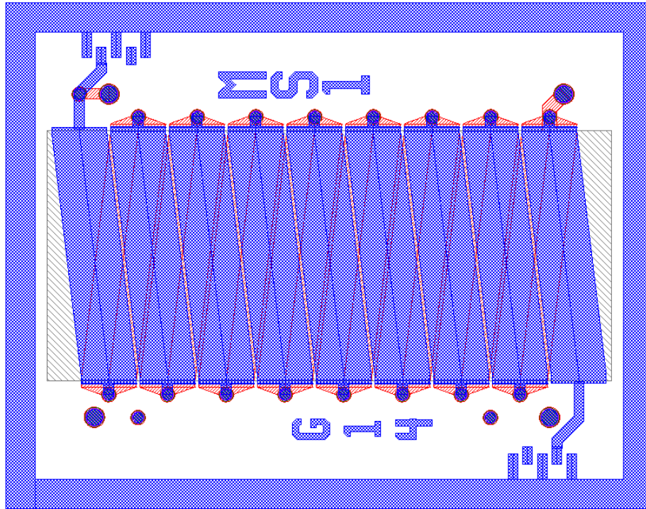
Figure 45 - MS1 Inductor Design
