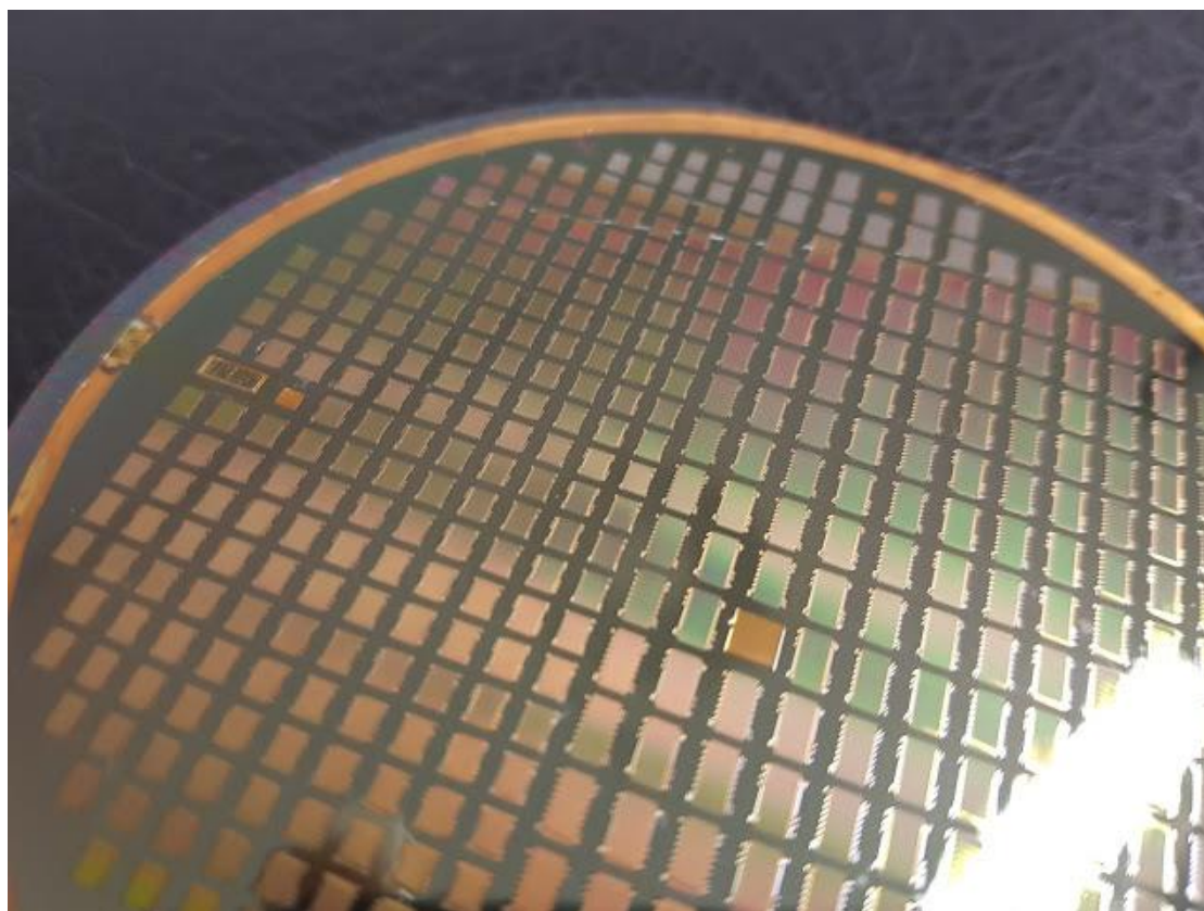
Figure 76 - Oxi-NiFe Wafer after Core Etching. Cores show the iridescent colouration.
