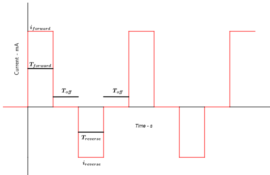
Figure 32 - Pulse reverse waveform
