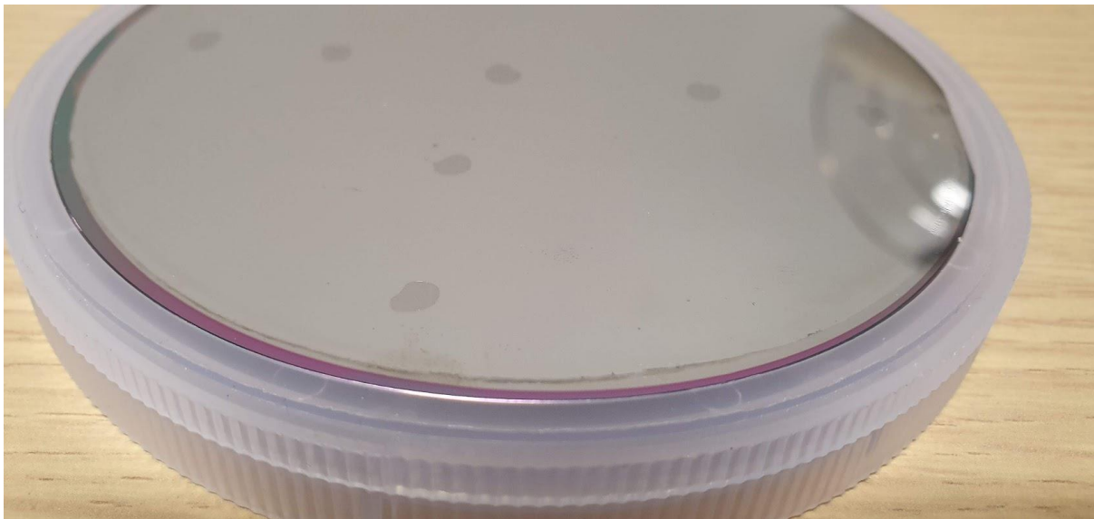
Figure 40 - Varnish Marks on the wafer after electroplating
