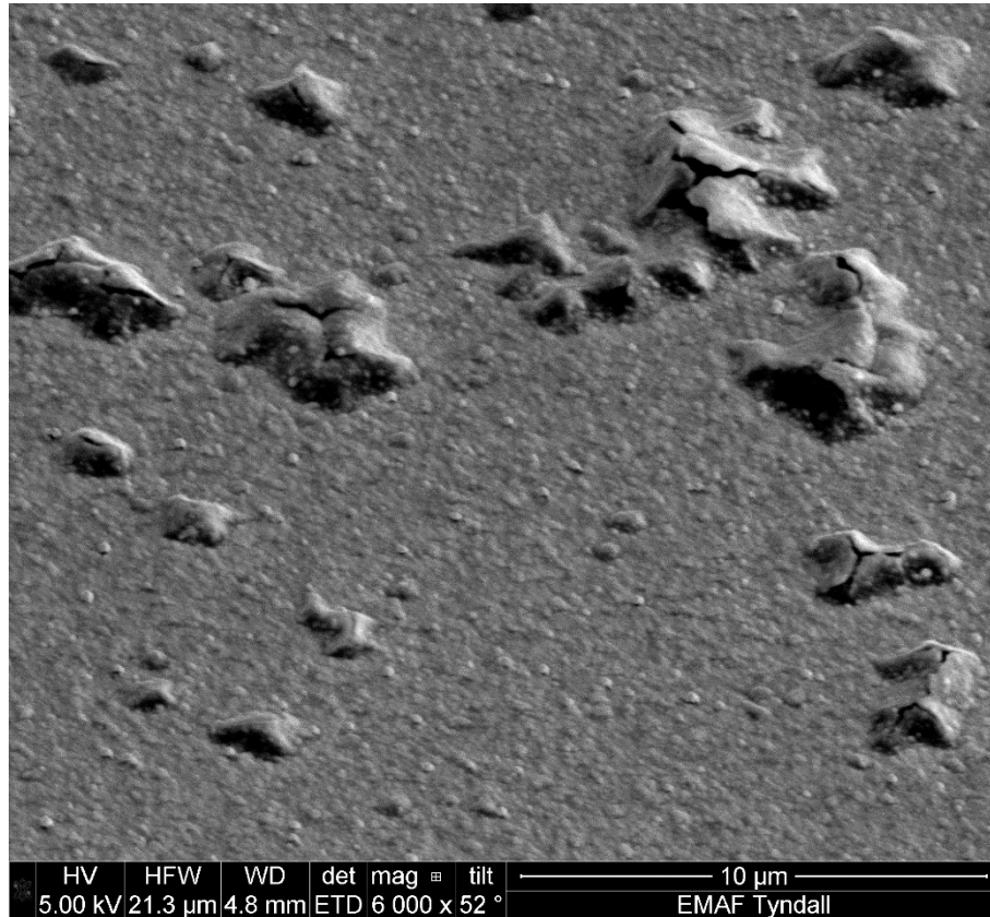
Figure 94 - Oxi-CoNiFe Surface (52° Angle)
