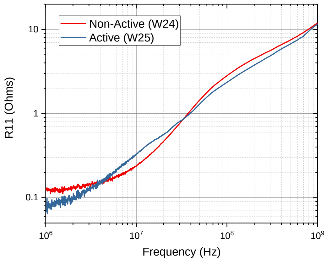
Figure 118 - AC Resistance of CoNiFe MC2 Inductor Devices
