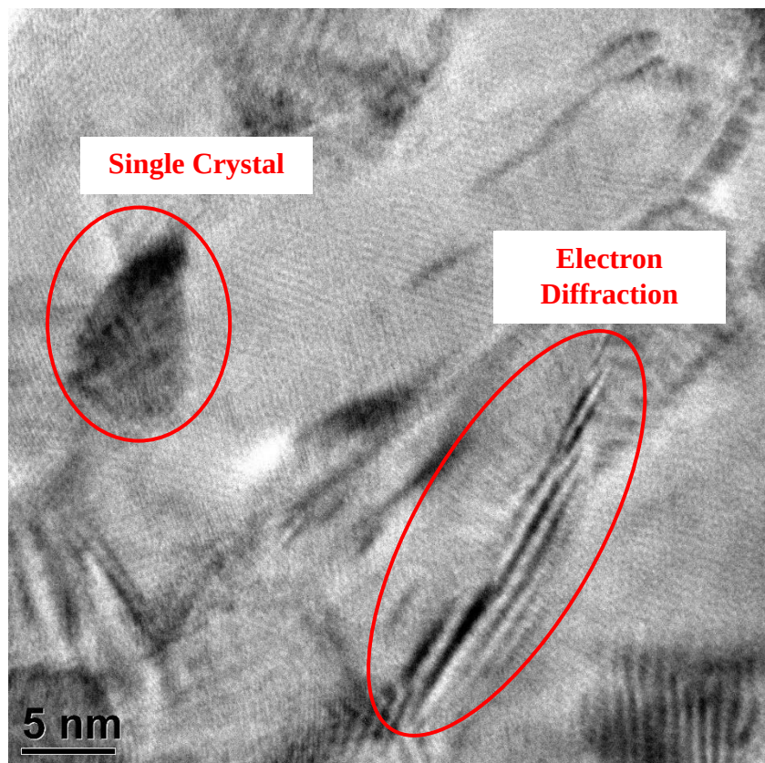
Figure 98 - Individual Grain of AD CoNiFe
