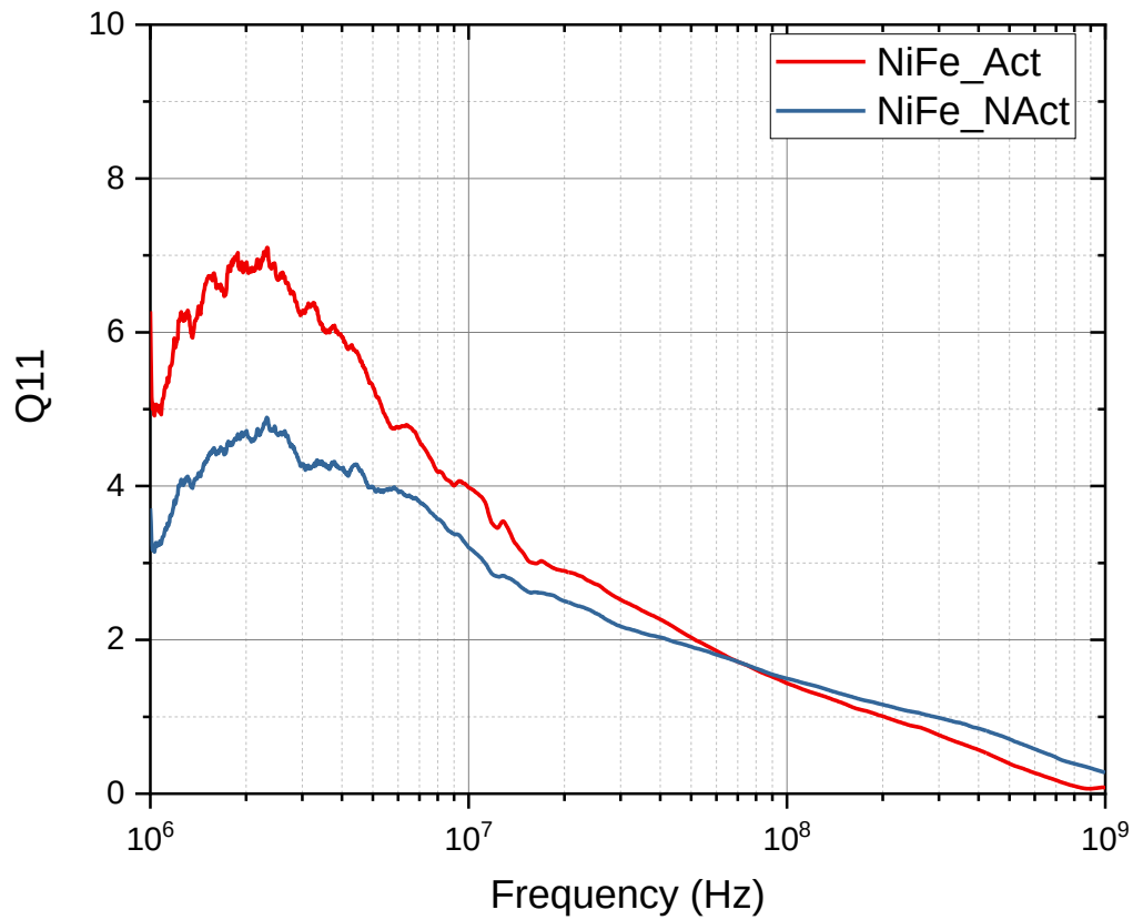
Figure 84 - Q-Factor of NiFe MS2 Inductor Devices
