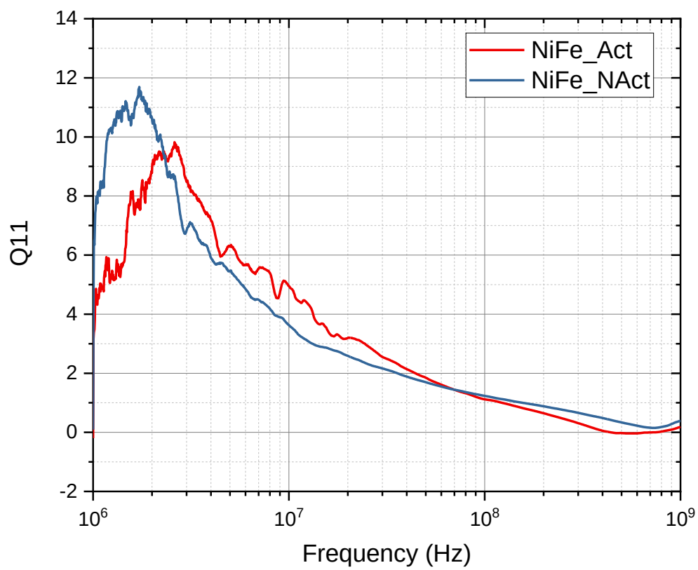
Figure 81 - Q-Factor of NiFe MS1 Inductor Devices
