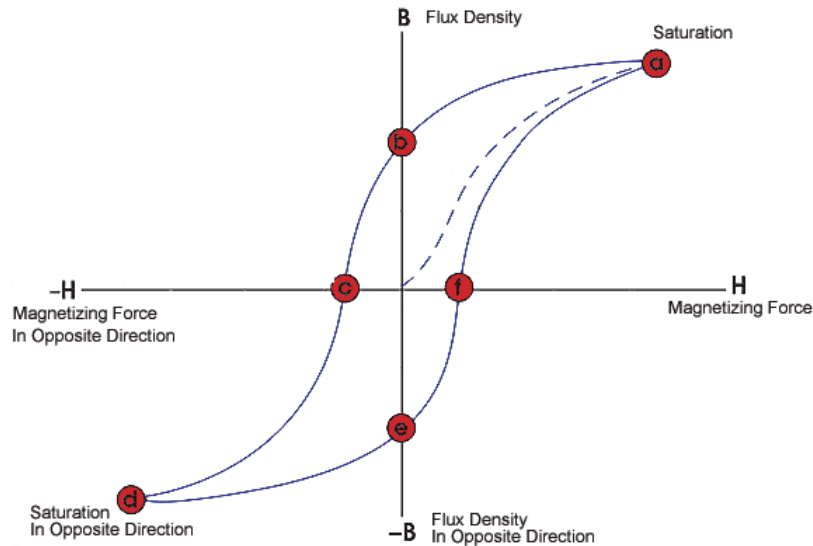
Figure 3 - Hysteresis Loop of a typical ferromagnetic material
