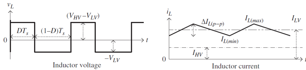
Figure 8 - Graph of inductor's voltage (a) and current (b)
