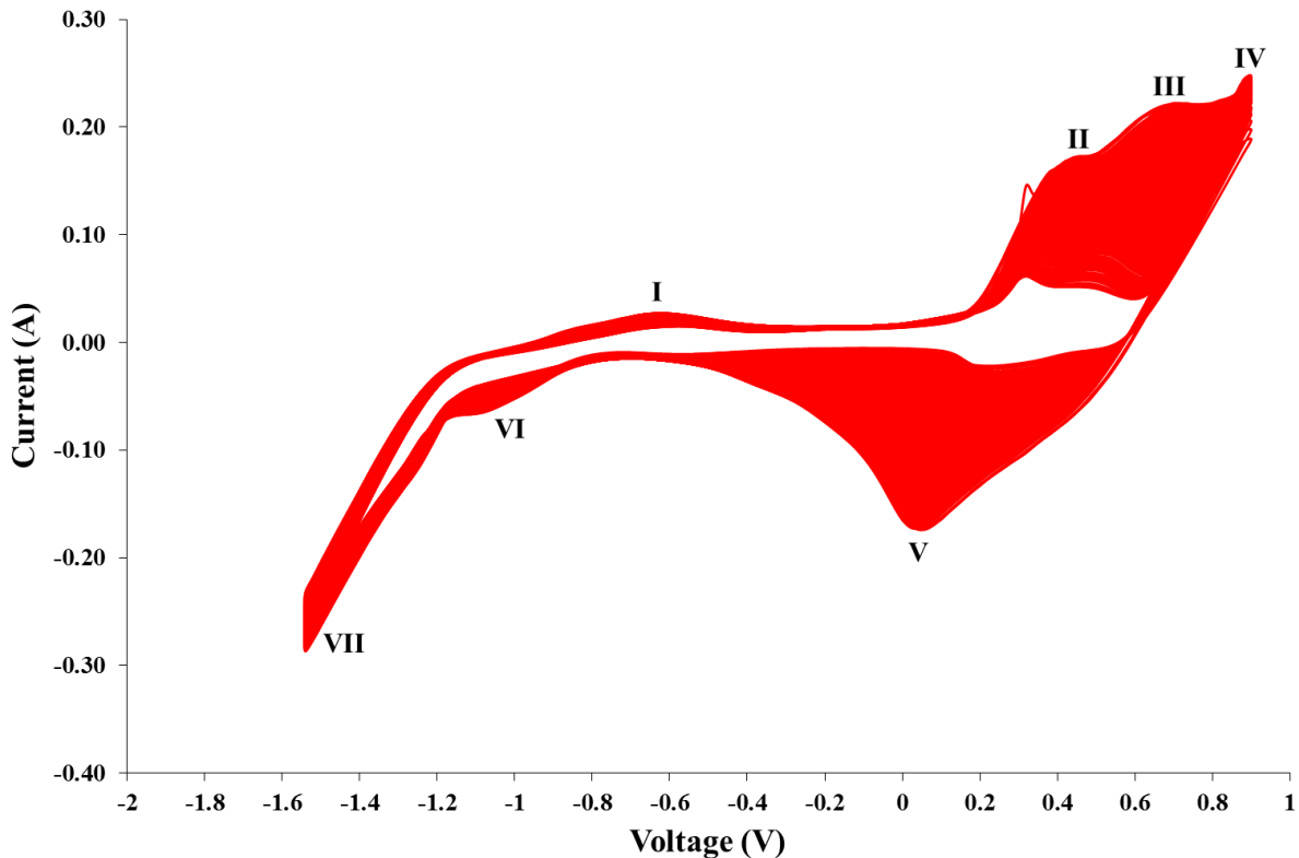
Figure 53 – Voltammogram of CoNiFe Electrode
