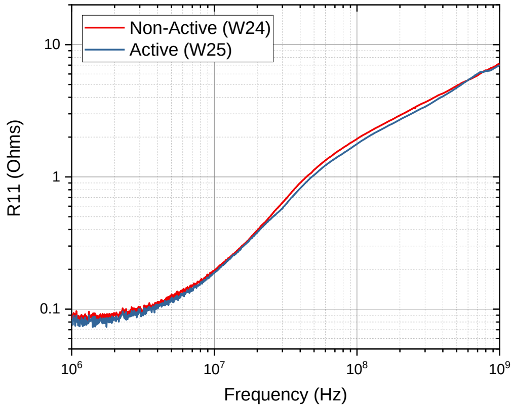
Figure 109 - AC Resistance of CoNiFe MS1 Inductor Devices
