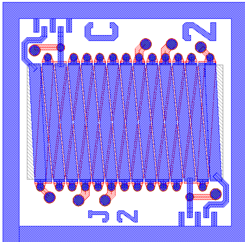
Figure 48 - MC2 Inductor Design
