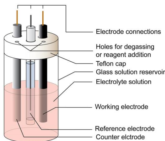
Figure 35 - Electrochemical cell set-up
