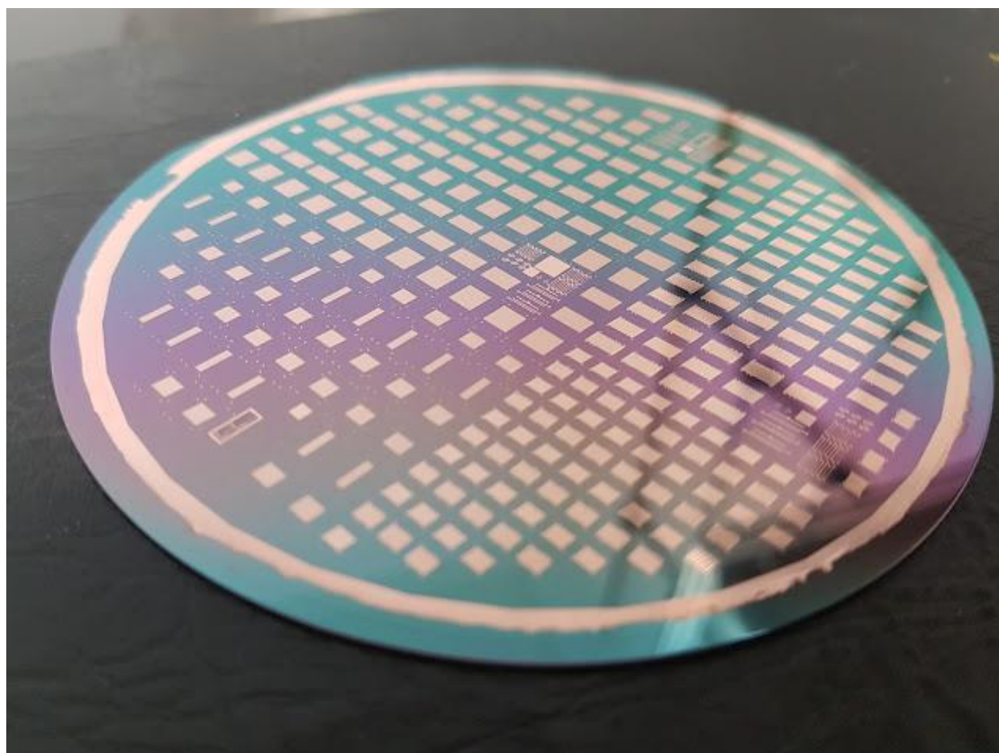
Figure 75 - Device Wafers with bottom windings and vias built
