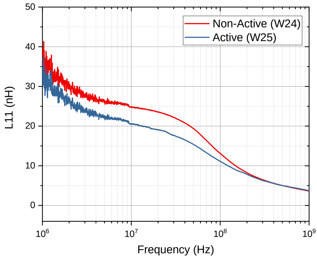
Figure 111 - Inductance of CoNiFe MS2 Inductor Devices
