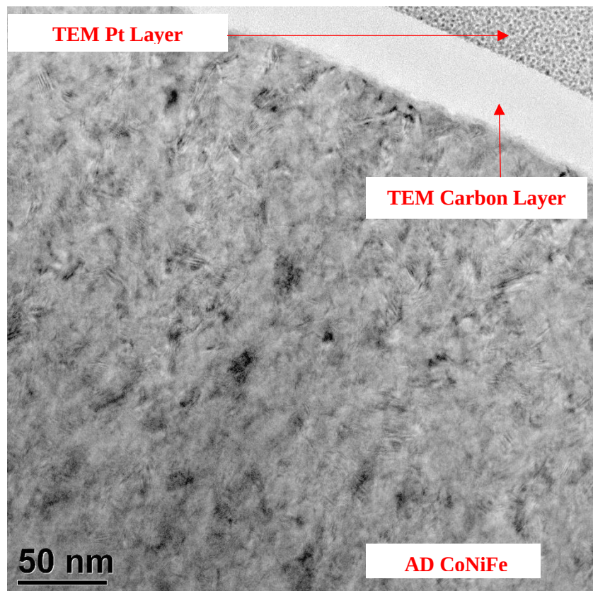
Figure 96 - Top surface of the AD CoNiFe & Pt / Carbon Layer
