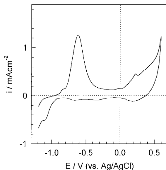
Figure 37 - Voltammogram of cobalt in 0.2M KOH between -1.2V and +0.6V
