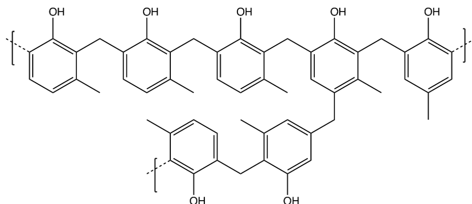
Figure 16 - Example of a novalac derivative polymer chain
