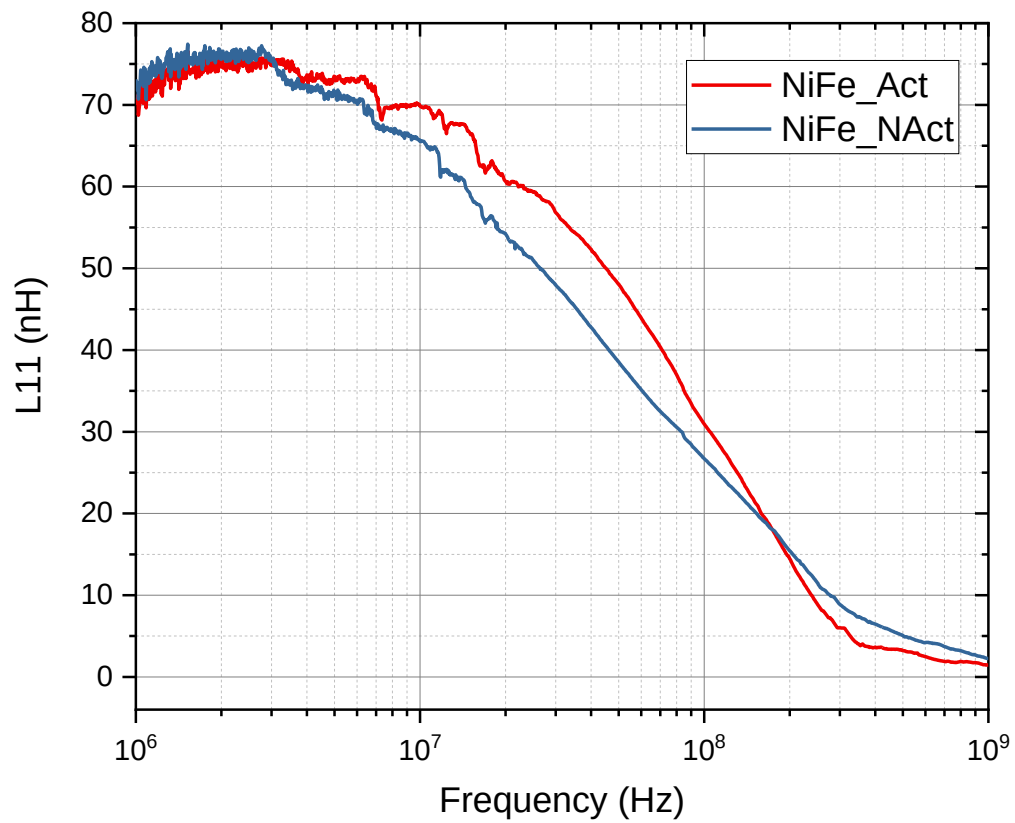
Figure 85 - Inductance of MC1 Inductor Devices
