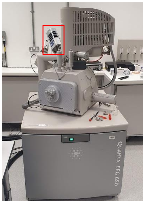
Figure 41 - Quanta FEG 650 SEM with Oxford X-Max EDX System (Red Box)
