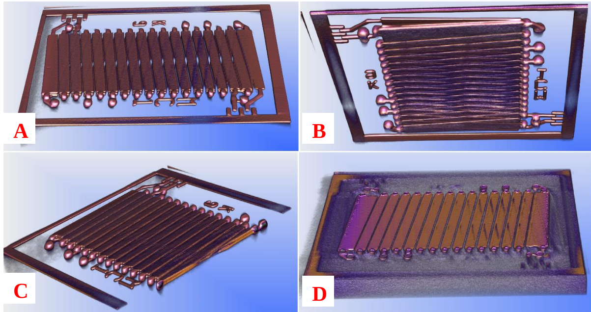
Figure 73 - 3D X-Ray Images of MC1 Inductor
