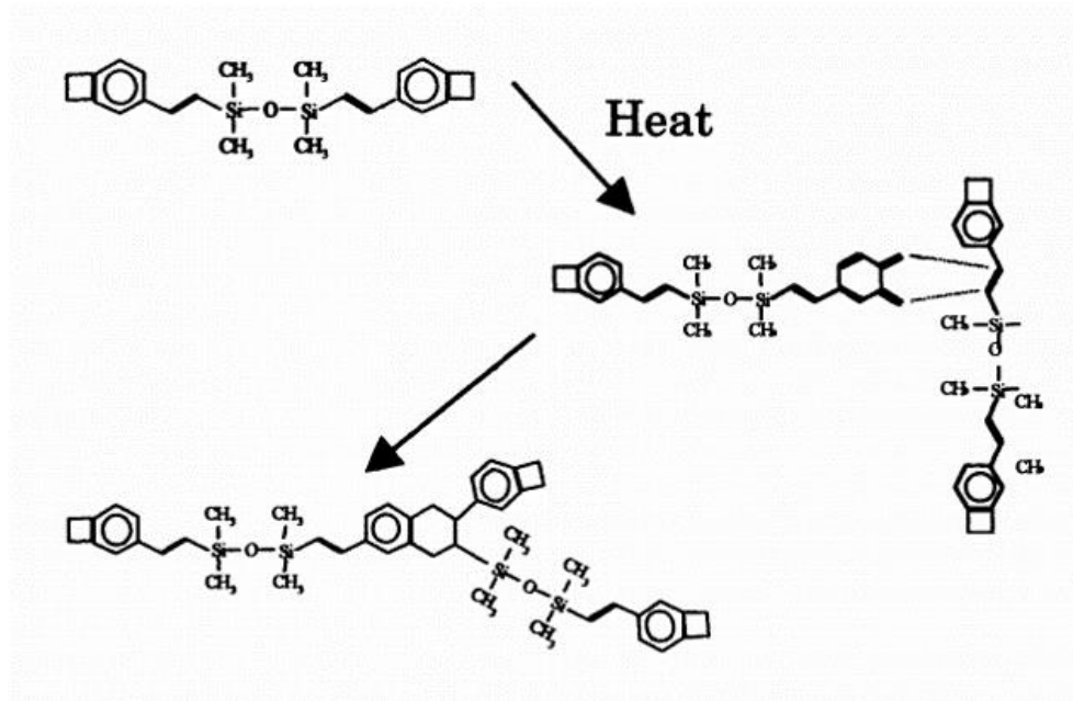
Figure 19 - DVS BCB polymerisation
