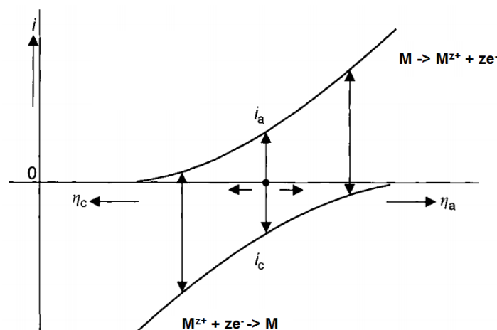
Figure 28 - Polarisation plot showing the rates of both the anodic dissolution and cathodic metal deposition as a function of potential
