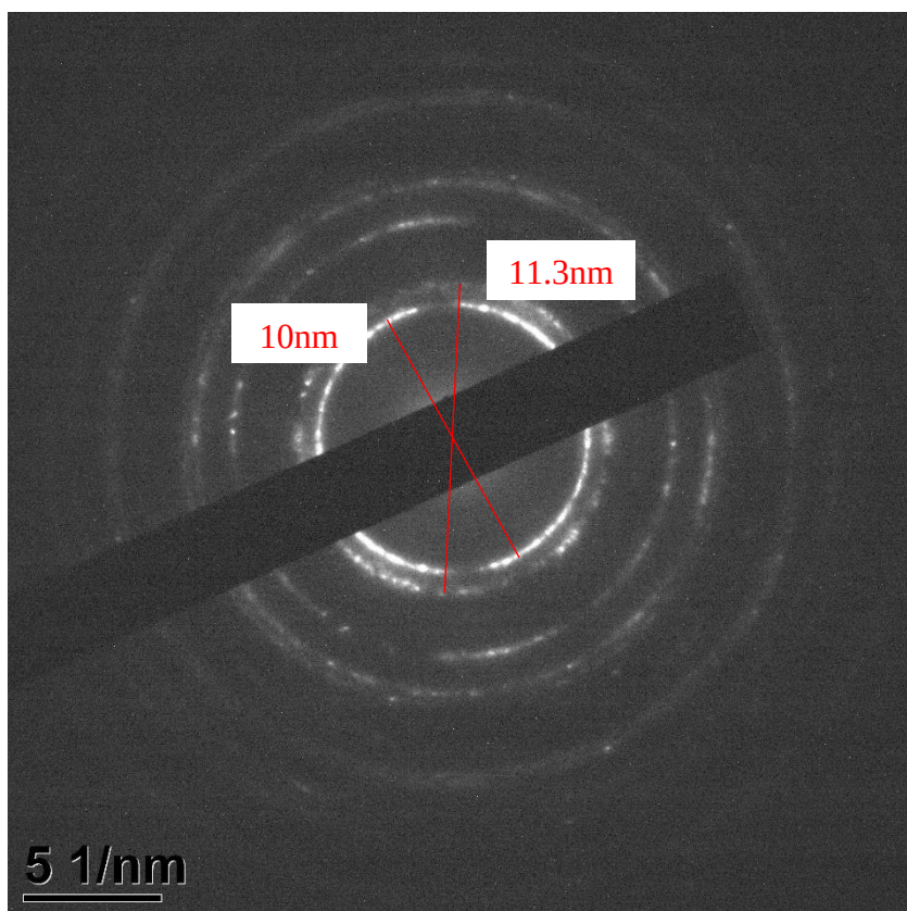
Figure 100 - SAED of AD CoNiFe with Selected area aperture
