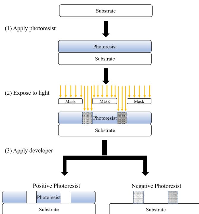
Figure 15 – Photolithography of positive and negative photoresists and their resulting pattern
