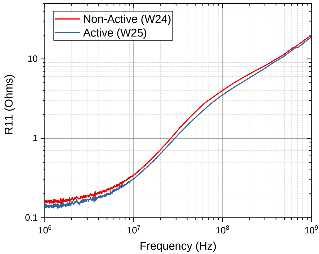
Figure 115 - AC Resistance of CoNiFe MC1 Inductor Devices
