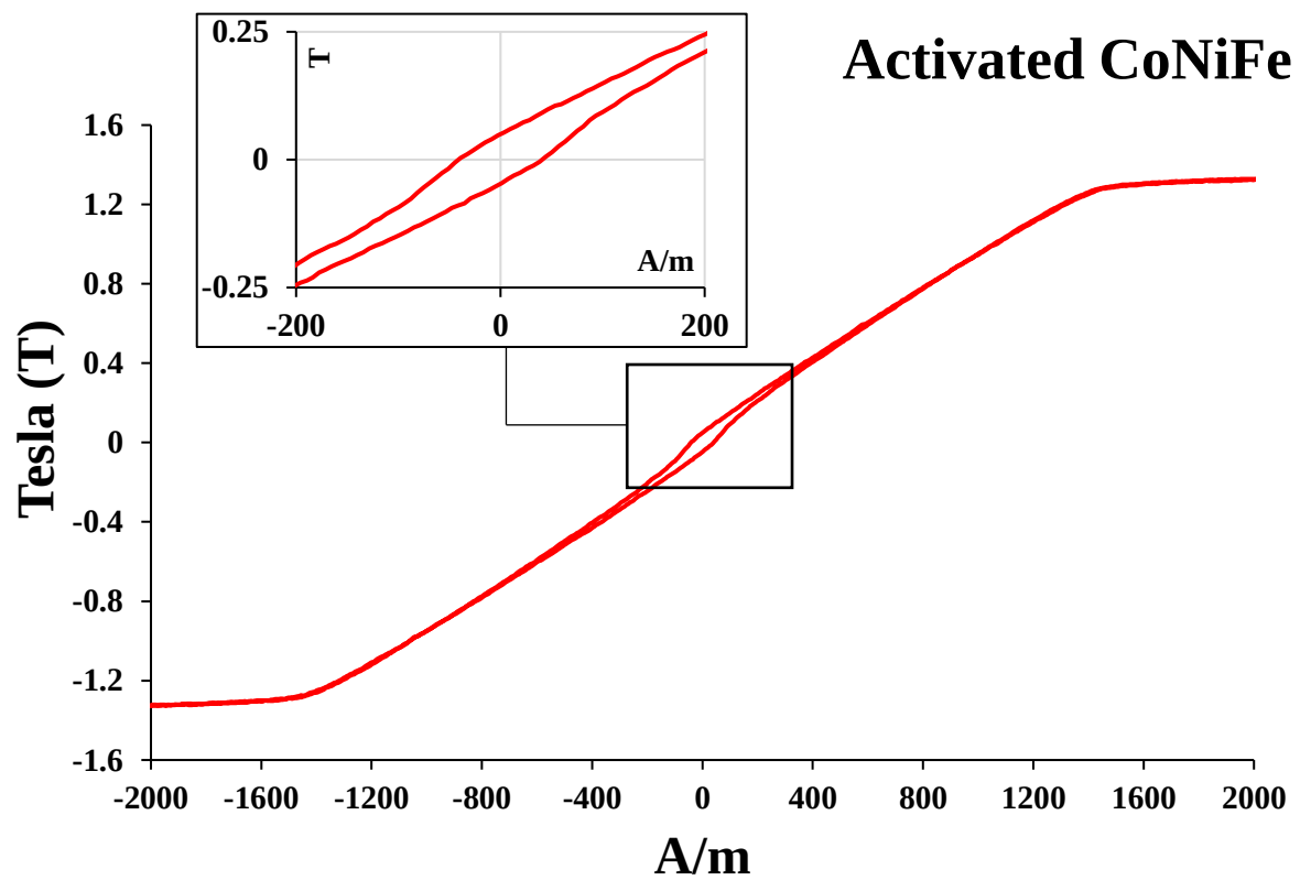
Figure 107 - Hysteresis Loop of 1.5cm x 1.5cm sample of Oxi-CoNiFe
