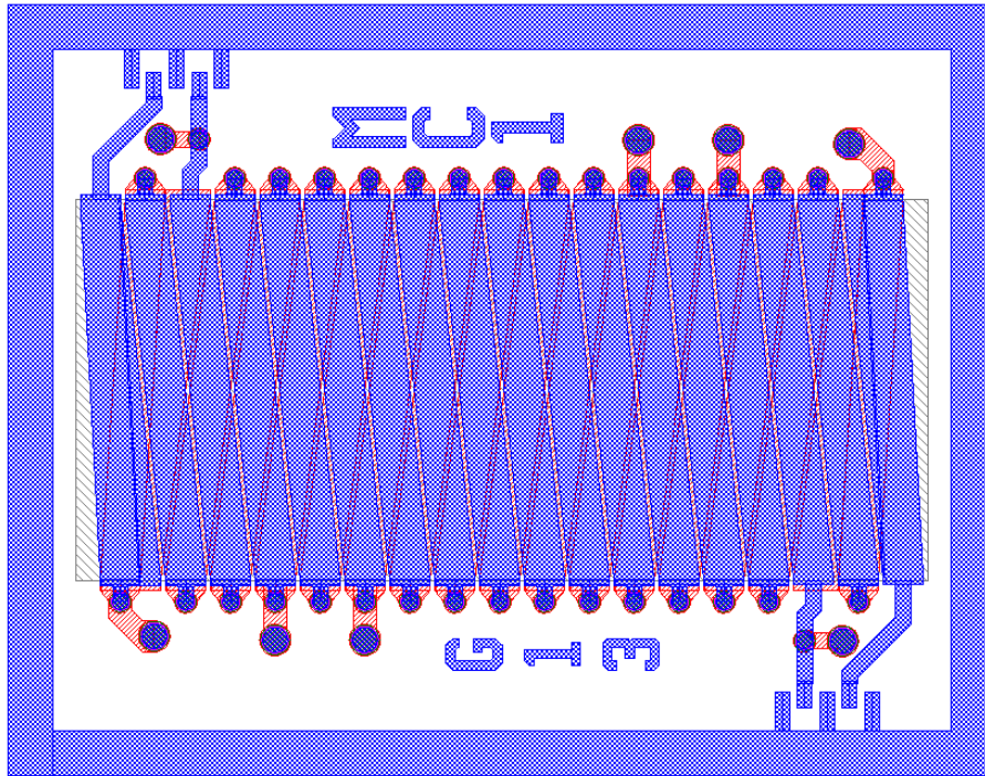
Figure 47 - MC1 Inductor Design
