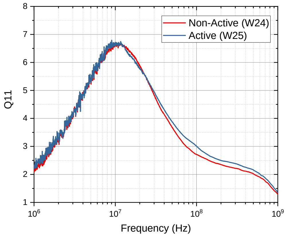
Figure 116 - Q-Factor of CoNiFe MC1 Inductor Devices
