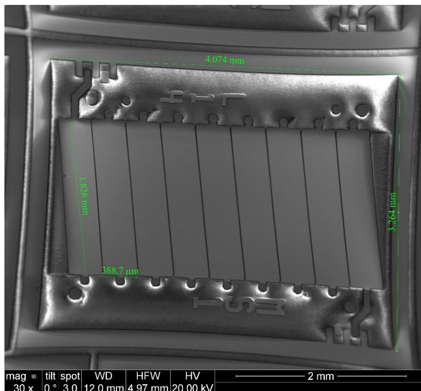
Figure 72 – MS1 single inductor with measurements
