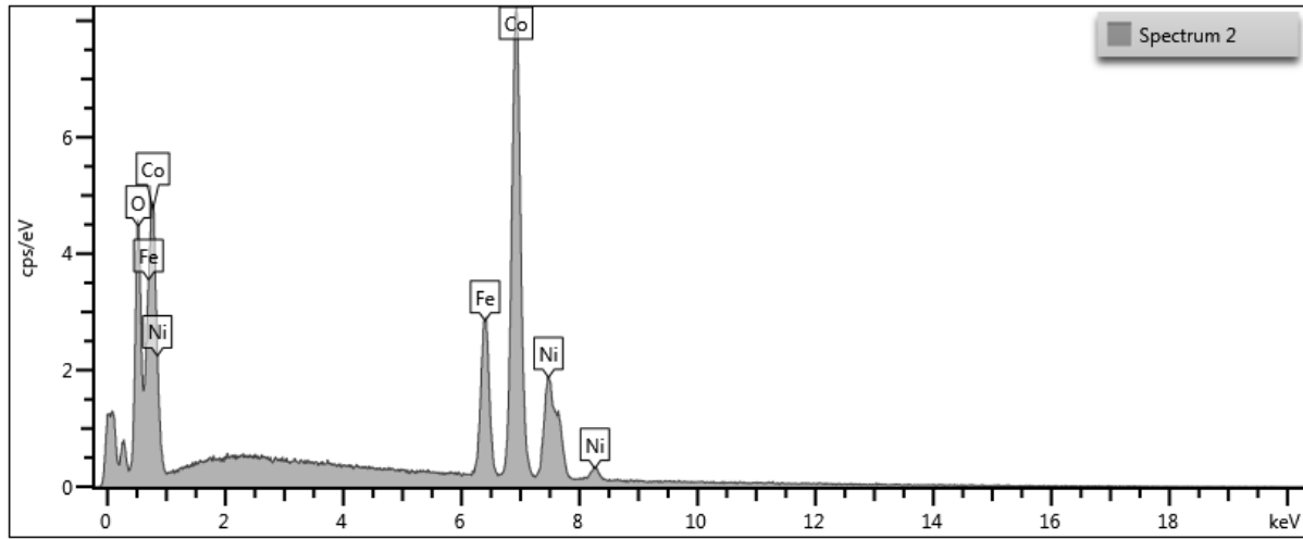
Figure 95 - EDX Spectrum of Oxi-CoNiFe
