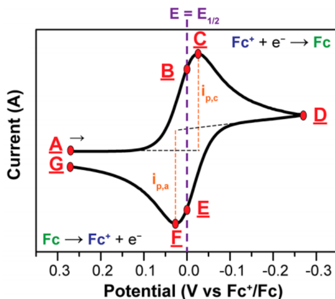
Figure 36 - Voltammogram of Ferrocene ( X^+ + e^- \rightleftharpoons X )
