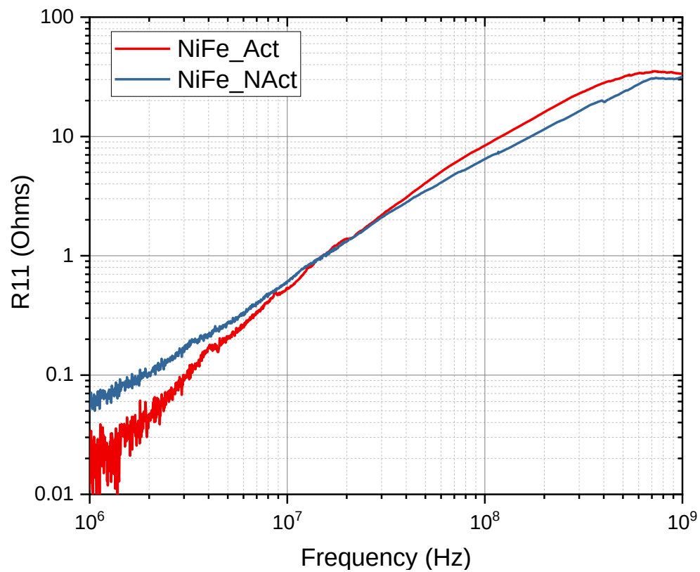
Figure 89 – AC Resistance of NiFe MC2 Inductor Devices
