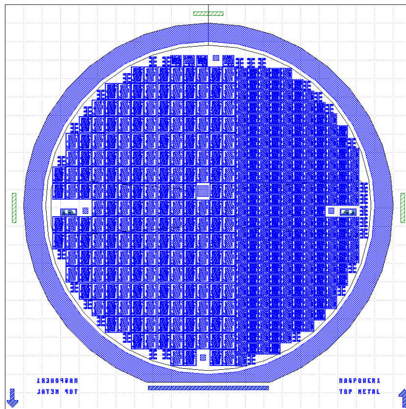
Figure 20 – The top metal winding photomask design used in this project
