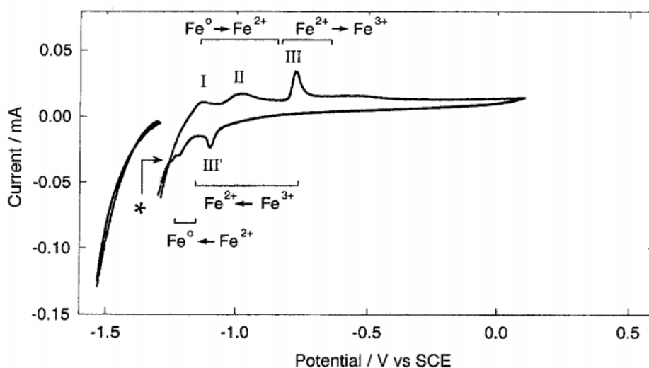
Figure 38 - Voltammogram of iron in 1M KOH between -1.275V and >0V
