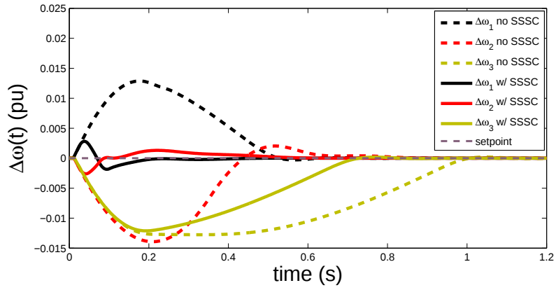
(a) Plot of the frequencies both with the SSSC and without the SSSC between areas 1 and 2.
