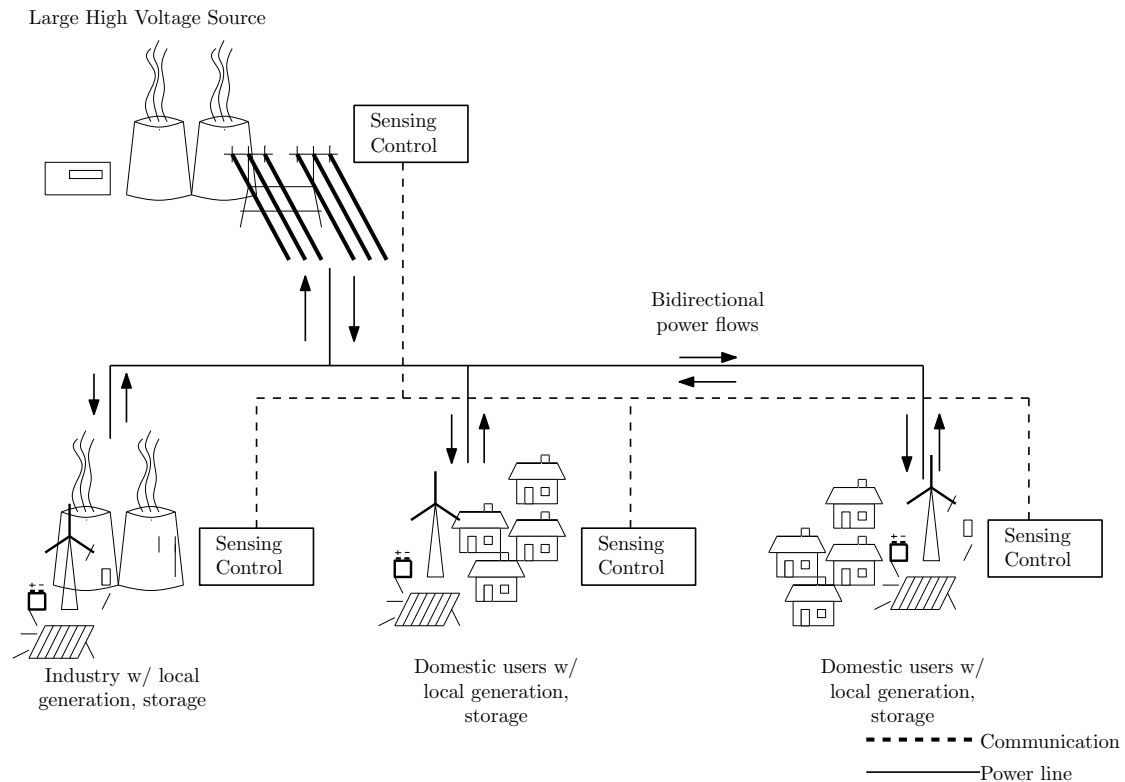
Figure 2.3: Future of power distribution.
