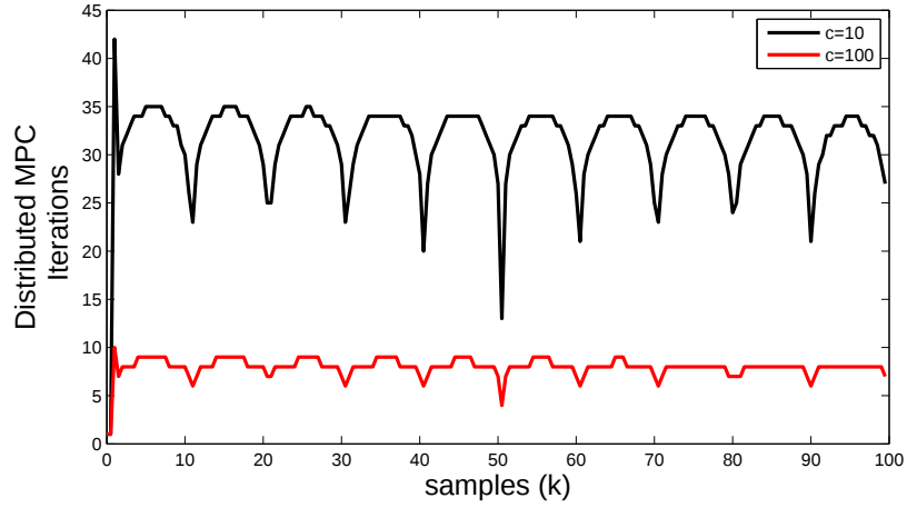
Figure 4.5: Distributed MPC iterations at each sample with large values of c when K_{S_{12}} = 258 , \epsilon = 10^{-3} .
