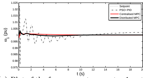
(a) Plot of the frequency at generator 1 vs time.
