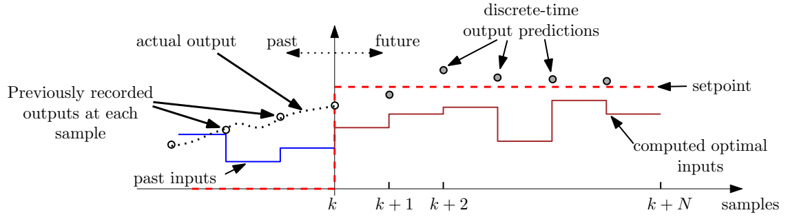
Figure 3.1: Model Predictive Control, showing past inputs and outputs, and predicted optimal inputs and outputs.
