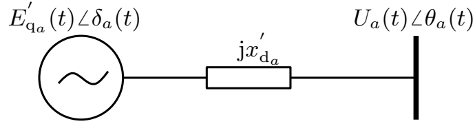
Figure 5.2: Generator a connected to a bus.
