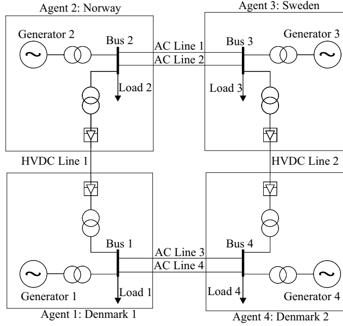
Figure 5.1: The multiple HVDC link system with areas controlled by agents (Eriksson, 2008).
