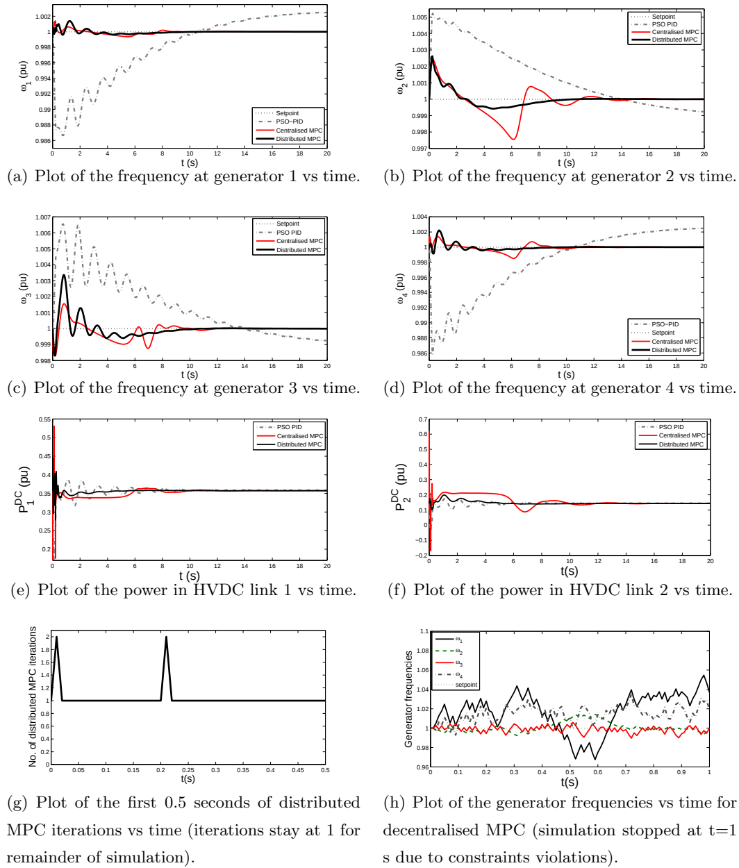
Figure 5.6: Plots of pu frequency and HVDC powers vs. time for a 100ms fault followed by a 100ms line break applied to line 1.
