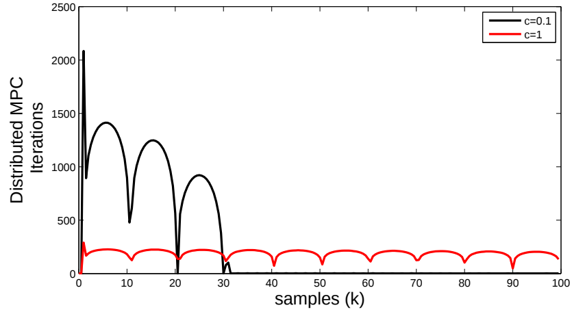
Figure 4.4: Distributed MPC iterations at each sample with small values of c when K_{S_{12}} = 258 , \epsilon = 10^{-3} .
