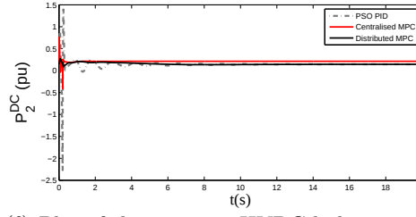
(f) Plot of the power in HVDC link 2 vs time.
