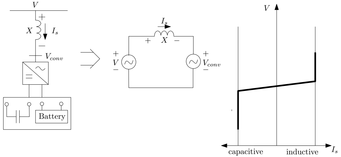
Figure 2.7: Static Compensator setup and its voltage/current characteristic (Mohan, 2006).
