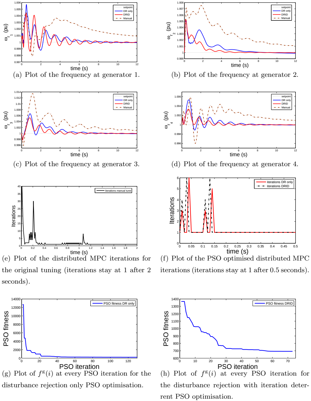
Figure 6.4: Plots of pu frequency and iterations over time for the 200ms line fault applied to lines 1 and 3 simultaneously.
