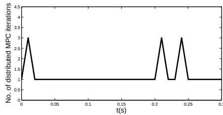
(g) Plot of the first 0.3 seconds of distributed MPC iterations vs time (iterations stay at 1 for remainder of simulation).
