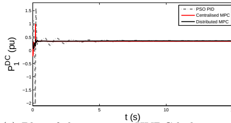
(e) Plot of the power in HVDC link 1 vs time.
