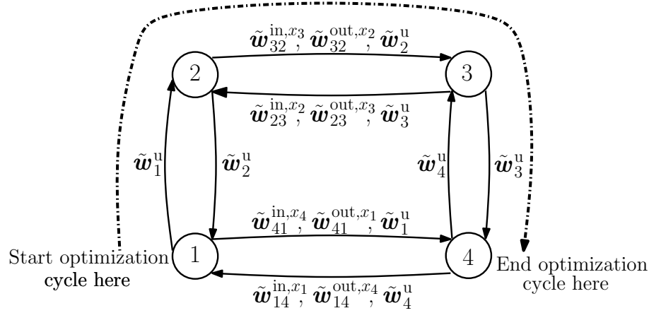
Figure 5.5: Order of serial distributed MPC optimizations and variables communicated between agents
