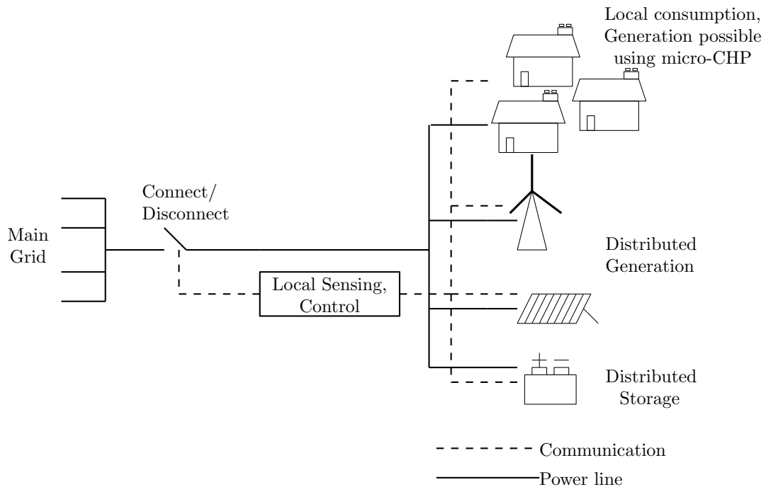
Figure 2.2: Microgrid which can disconnect from the main grid during instances of grid instability.
