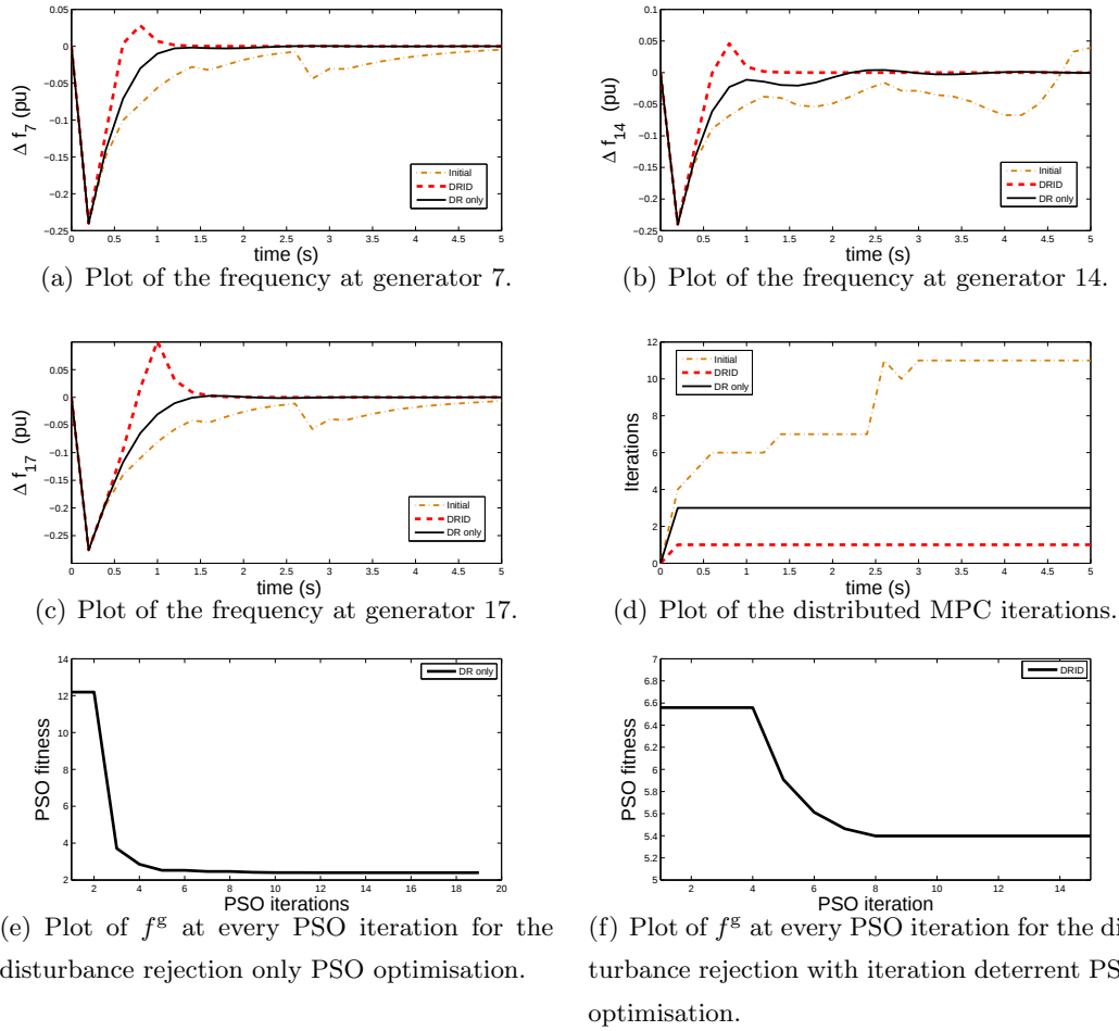
Figure 6.3: Plots of pu frequency and distributed MPC iterations over time, and PSO iterations for the disturbance rejection scenario applied to the 20 area discrete-time LFC network.
