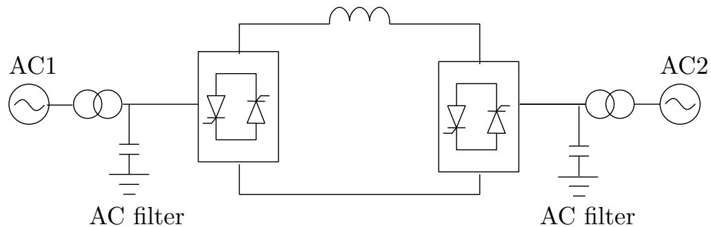
Figure 2.10: HVDC LCC system (Mohan, 2006).
