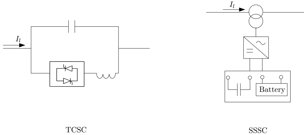
Figure 2.8: Thyristor Controlled Series Compensator (Mohan, 2006) and Static Synchronous Series Compensator setup (Zhang et al., 2006).
