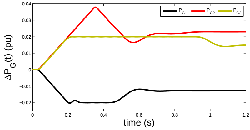
(b) Plot of the power generated by each generator for the simulation with no SSSC.
