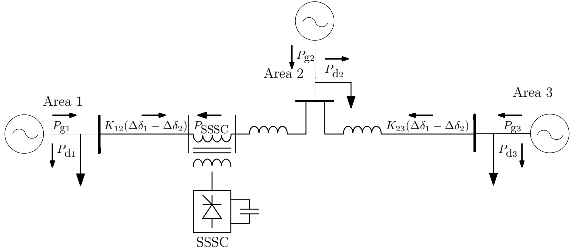
Figure 3.3: The 3 area LFC system with a Static Synchronous Series Compensator between areas 1 and 2.
