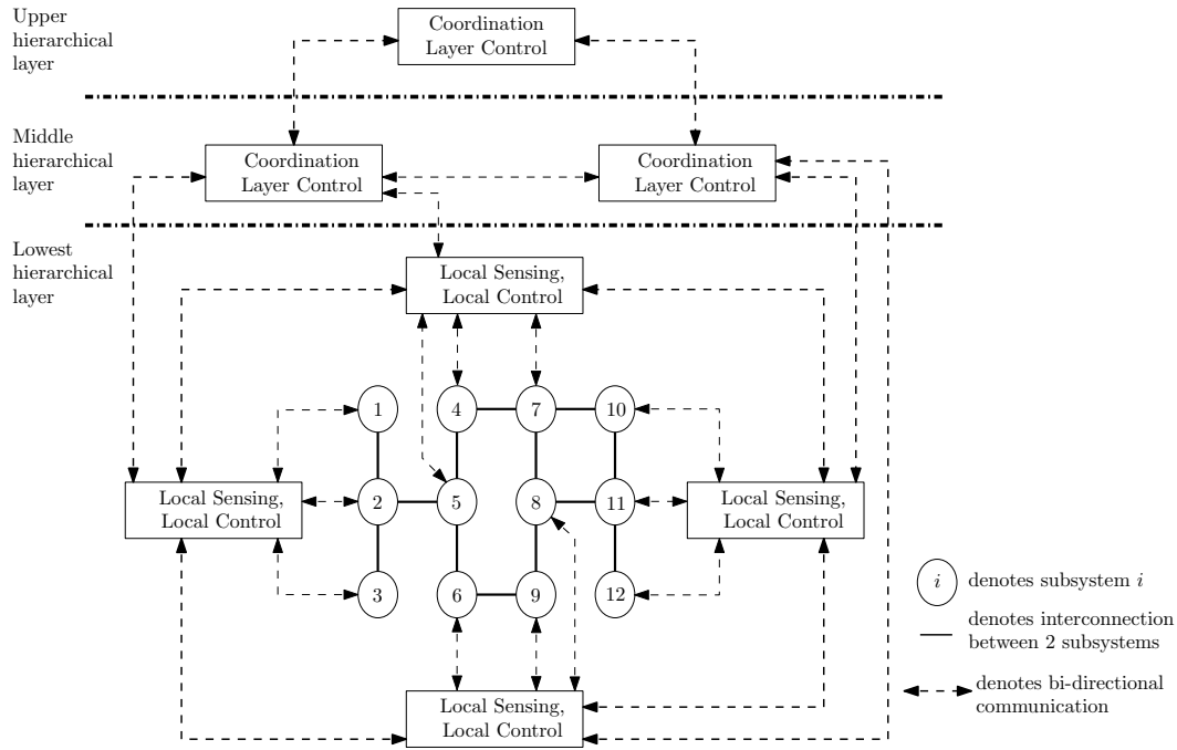
Figure 2.13: Distributed control architecture with coordination layers for hierarchical control.
