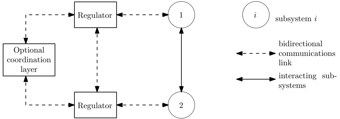
Figure 1.2: Distributed control of 2 interacting subsystems.
