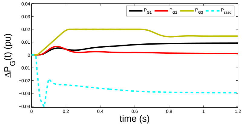
(c) Plot of the power generated by generator and the SSSC power when the SSSC is between areas 1 and 2 .
