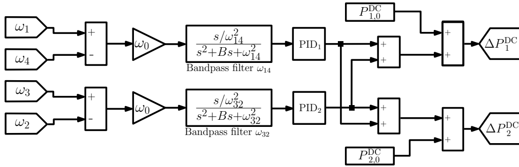
Figure 5.4: An extension of the control strategy used in (Eriksson, 2008) to control the multiple link HVDC system, which uses PID rather than P controllers
