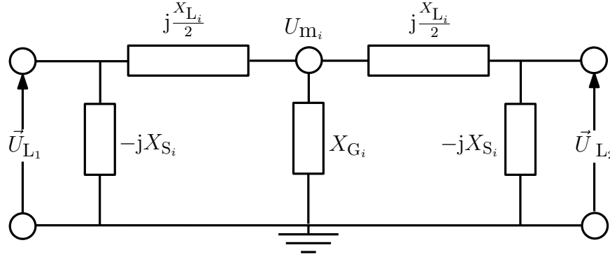
Figure 5.3: \pi -Model of lines.
