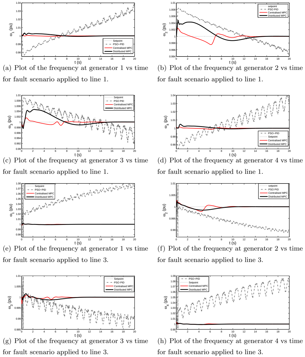
Figure 5.8: Plots of pu frequency and HVDC powers vs. time for a 100ms fault followed by a 200ms line break applied to lines 1 and 3 separately.
