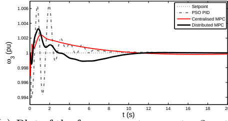
(c) Plot of the frequency at generator 3 vs time.
