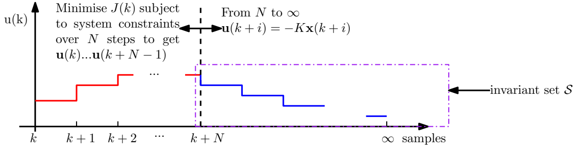
Figure 3.2: Stability constrained dual mode MPC.
