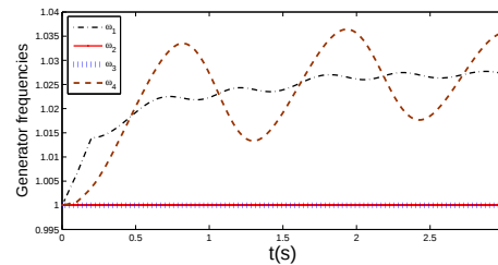
(h) Plot of the generator frequencies vs time for decentralised MPC (simulation stopped at t=3 s due to constraints violations).
