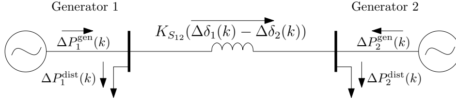
Figure 4.3: The 2 area discrete time LFC.
