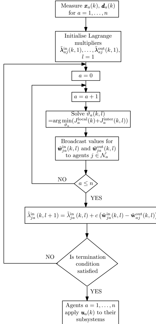
Figure 4.2: The distributed MPC algorithm, at the k^{\text{th}} sample step.
