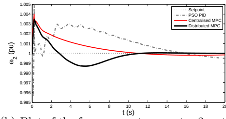
(b) Plot of the frequency at generator 2 vs time.
