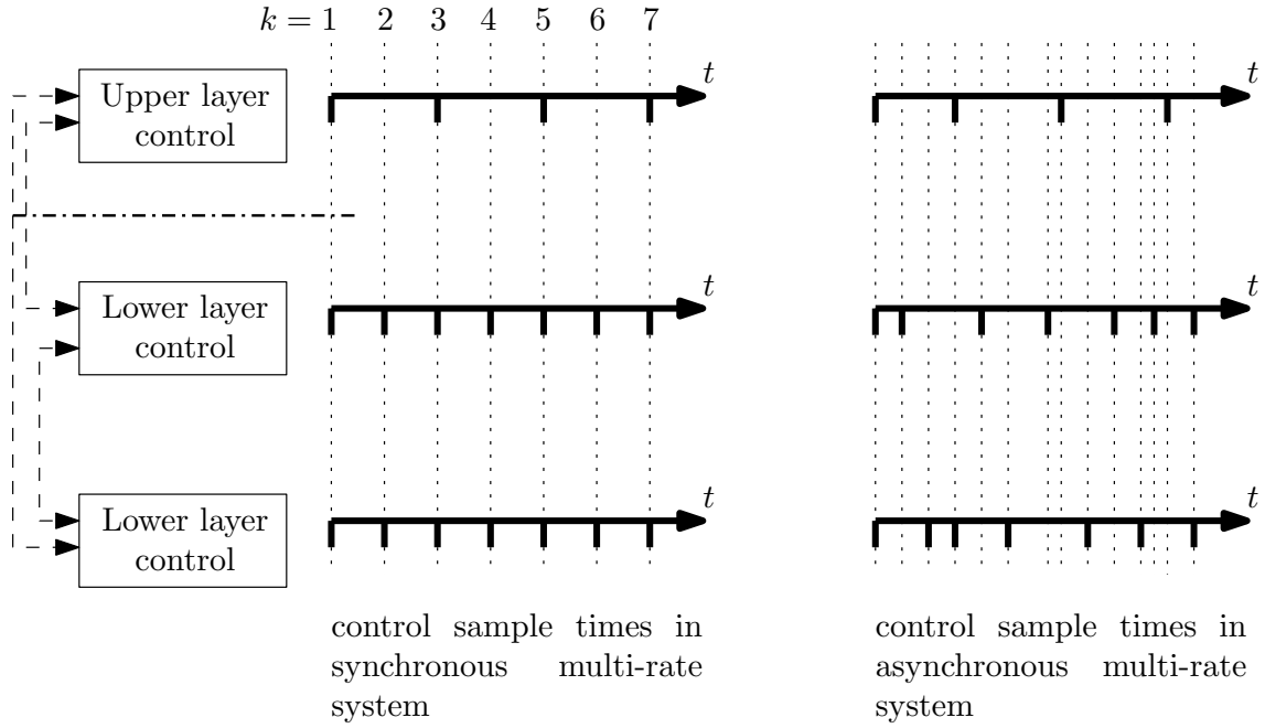
Figure 2.14: Hierarchical and distributed control architecture showing multi-rate synchronous and asynchronous updating.
