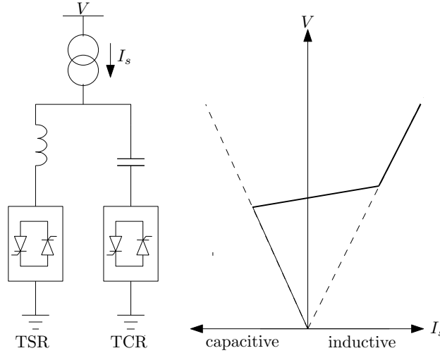
Figure 2.5: Static Var Compensator setup and its voltage/current characteristic.
