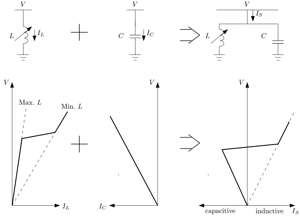
Figure 2.6: Illustration of voltage regulation using a shunt variable inductor and fixed capacitor connected in parallel (Kundur, 1994).
