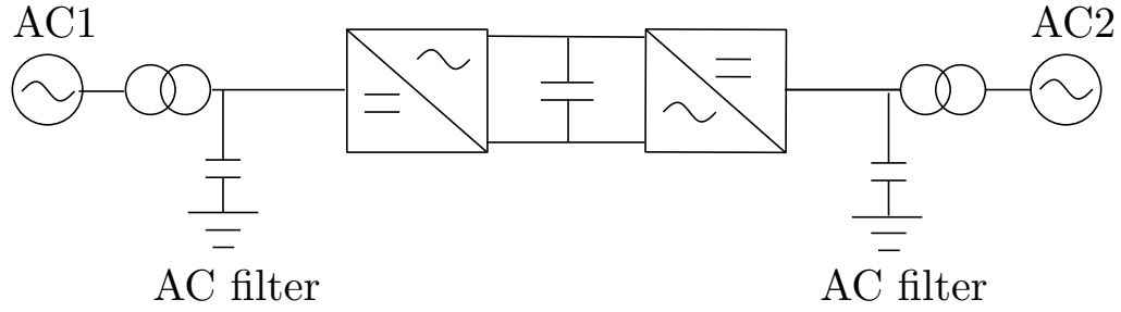
Figure 2.11: HVDC VSC system (Mohan, 2006).
