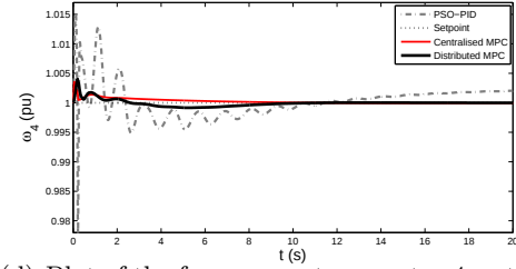
(d) Plot of the frequency at generator 4 vs time.
