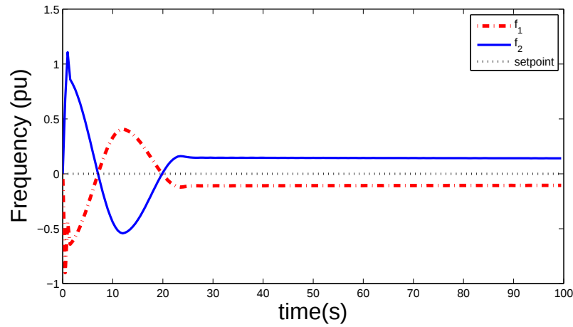
Figure 4.6: Response when K_{S_{12}} = 260 , c=1 , and \epsilon = 10^{-2} .
