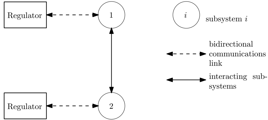
Figure 1.1: Decentralised control of 2 interacting subsystems.
