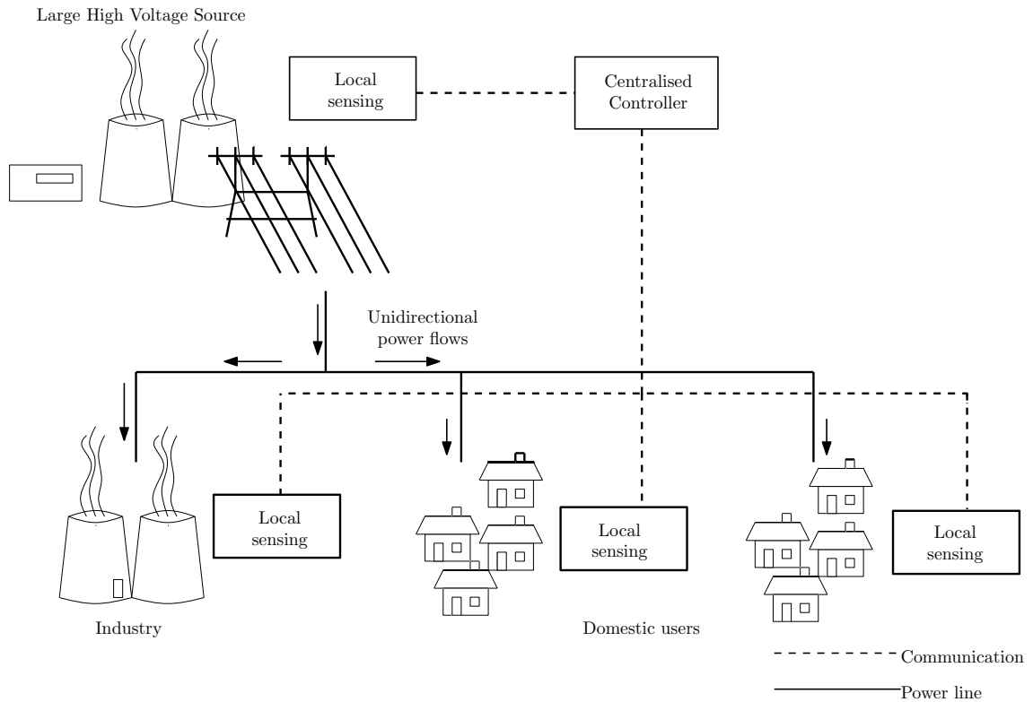
Figure 2.1: Traditional centralised monopolistic power distribution.
