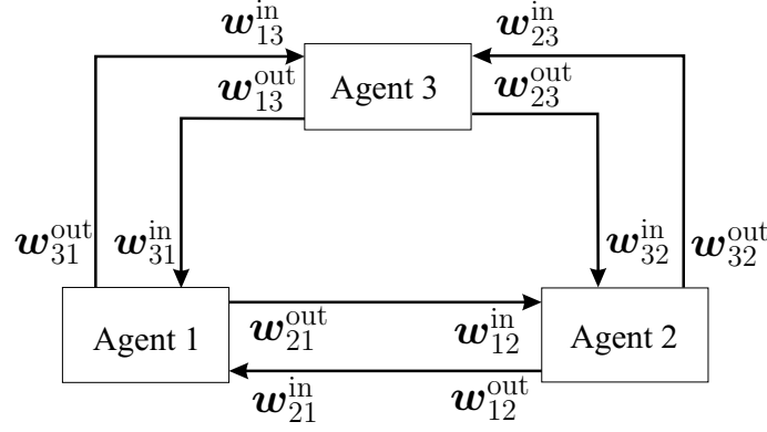
Figure 4.1: Interconnecting inputs and outputs for 3 connected subsystems.
