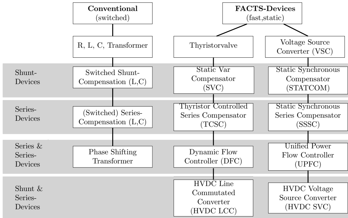
Figure 2.4: Overview of FACTS devices (Zhang et al., 2006).
