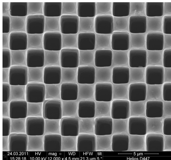
Fig. 1. Top view of a typical macroporous sample prepared for this work. The distance from center to center of the pores is 3\text{ }\mu\text{m} .
