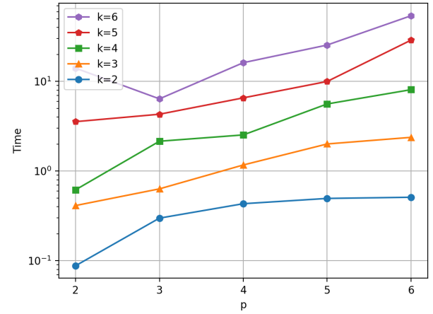
Figure 3: Average computation time in seconds to compute SMMR_{\mathcal{W}}^k(\mathcal{A}) with EPI SAT (y-axis) over 20 repetitions varying k and p with an input set of 100 undominated alternatives and \mathcal{W} = \mathcal{U} .
