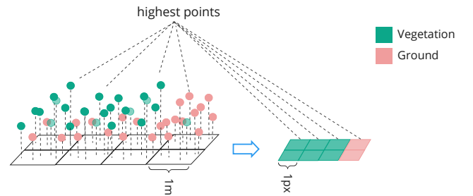
Fig. 3: Projection of a classified LiDAR 3D point cloud onto a 2D plane
