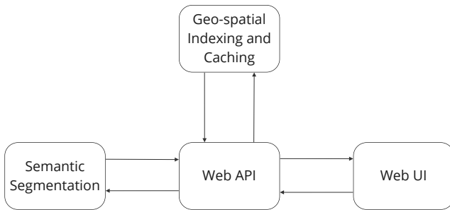
Fig. 8: Our GIS system architecture.
