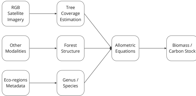
Fig. 7: Our GIS carbon stock estimation workflow.
