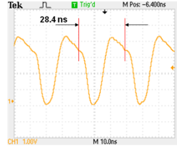
Fig. 6. Plot of V_{cathode} for saturated count-rate
