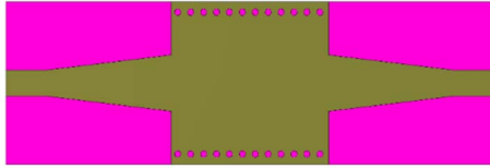
Fig.1. Configuration of conventional SIW.
