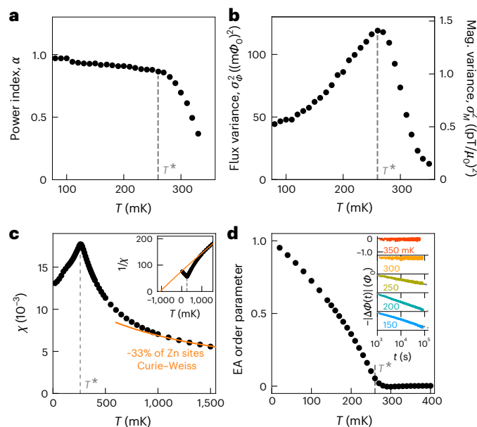
Fig. 3 | Spin noise spectroscopy analysis of witness spin dynamics in \text{ZnCu}_3(\text{OH})_6\text{Cl}_2 . a , Measured witness spin flux noise power index \alpha from S_\phi(\omega, T) \propto \omega^{-\alpha(T)} as a function of temperature (from Fig. 2c), obtained by fitting the PSD S_\phi(\omega, T) = A(T)\omega^{-\alpha(T)} in the frequency range of 0.6 \text{ rad Hz} \leq \omega \leq 600 \text{ rad Hz} . A clear transition to \alpha \approx 1 is detected at T^* \approx 260 \text{ mK} (dashed line). b , Measured witness spin flux noise variance \sigma_\phi^2 as a function of temperature (from Fig. 2c), obtained by integrating S_\phi(\omega, T) in the range of 0.6 \text{ rad Hz} \leq \omega \leq 600 \text{ rad Hz} . Right axis: the equivalent magnetization noise variance \sigma_M^2(T) . These data indicate a transition in noise power at T^* \approx 260 \text{ mK} (dashed line). c , Measured witness spin susceptibility \chi(T) (SI units; the inset shows 1/\chi ) in micro-Tesla magnetic fields revealing a Curie–Weiss-like \chi(T) at higher temperatures (orange line), yielding an estimated witness spin density of 33% of Zn sites. However, this diverging \chi(T) is interrupted by a sharp transition to a rapidly diminishing \chi(T) below T^* \approx 260 \text{ mK} (dashed line). d , Measured EA spin glass order parameter for witness spins from c , indicating a transition to a witness spin glass below T^* \approx 260 \text{ mK} (dashed line). Inset: time evolution of the average flux against a 2\text{-}\mu\text{T} applied field after the temperature is suddenly dropped from a thermalized condition at 400 \text{ mK} . The sample flux \Phi(t) shows a -\ln(t) relaxation (dashed line) on periods of a day only below T \approx 250 \text{ mK} , providing direct evidence of the appearance of a witness spin glass. The error bars are invisible as they are smaller than the symbol points in all panels.
