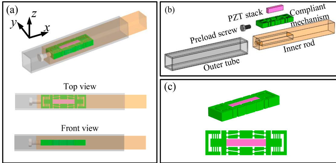
Fig. 2. The CAD model of the lockable joint. (a) Assembled views. (b) Explosion views. (c) The inner CM with PZT actuation.
