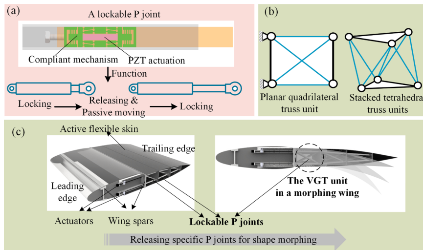
Fig. 1. Functions of the proposed design and one of its applications. (a) A PZT actuated lockable P joints design. (b) Its application in the variable geometry truss units. (c) One of the applications in morphing airfoil wings [29].
