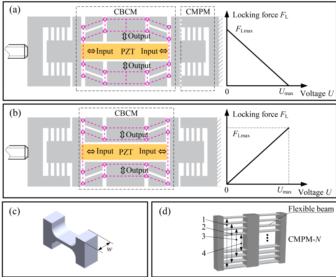
Fig. 3. The designs of two types of locking. (a) Normally locking design. (b) Normally releasing design. (c) A corner-filletted flexure hinge used in the CBCM. (d) A CMPM with N = 4 .
