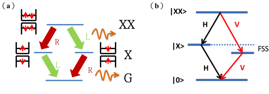
Fig. 6.1: Schematics of XX-X-G decay cascade with (a) zero FSS and (b) with finite FSS.
