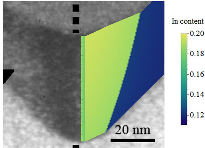
Fig. 3.3: TEM image of a layer of \text{In}_{0.12}\text{Ga}_{0.88}\text{As} with nominal thickness of 40 nm and simulation results of indium concentration distribution with color scale bar at the right-hand side.
