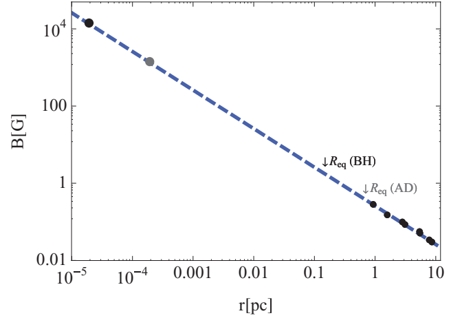
Figure 10. Extended plot of B versus r for 2007+777 to include the extrapolated magnetic field strength ( B \simeq 0.26 r^{-1} ) at the accretion disc ( 10 r_g ) and black holes ( r_g ) distances. The estimated equipartition radii from the model K07 are indicated by the arrows with R_{eq,AD} \sim 0.7 pc and R_{eq,BH} \sim 0.1 pc. Also plotted are points at 10 r_g (grey) and r_g (black) representing the theoretically expected magnetic field strengths for a magnetically powered jet.
