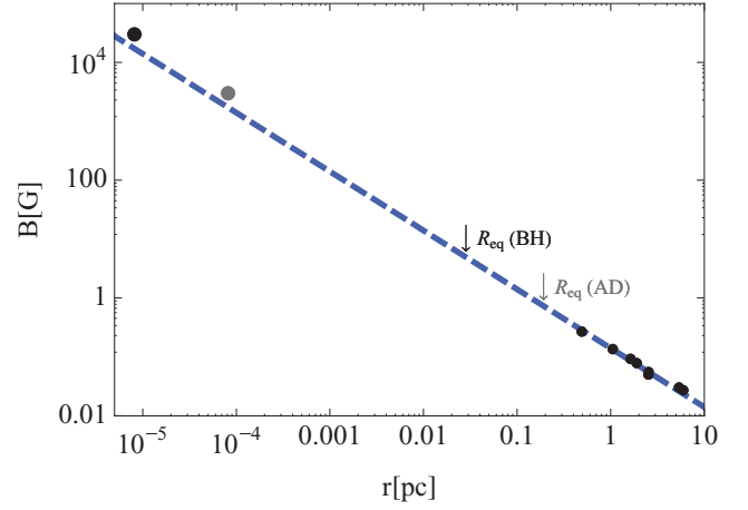
Figure 5. Extended plot of B versus r for 2200+420 to include the extrapolated magnetic field strength ( B \approx 0.14r^{-1} ) at the accretion disc ( 10r_g ) and black holes ( r_g ) distances. The estimated equipartition radii from K07 are indicated by the arrows with R_{\text{eq,AD}} \sim 0.2 pc and R_{\text{eq,BH}} \sim 0.03 pc. Also plotted are points at 10r_g (grey) and r_g (black) representing the theoretically expected magnetic field strengths for a magnetically powered jet.
