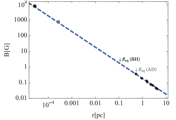
Figure 15. Extended plot of B versus r for 1418+546 to include the extrapolated magnetic field strength ( B \simeq 0.18r^{-1} ) at the accretion disc ( 10r_g ) and black holes ( r_g ) distances. The estimated equipartition radii from the model K07 are indicated by the arrows with R_{\text{eq,AD}} \sim 0.5 pc and R_{\text{eq,BH}} \sim 0.1 pc. Also plotted are points at 10r_g (grey) and r_g (black) representing the theoretically expected magnetic field strengths for a magnetically powered jet.
