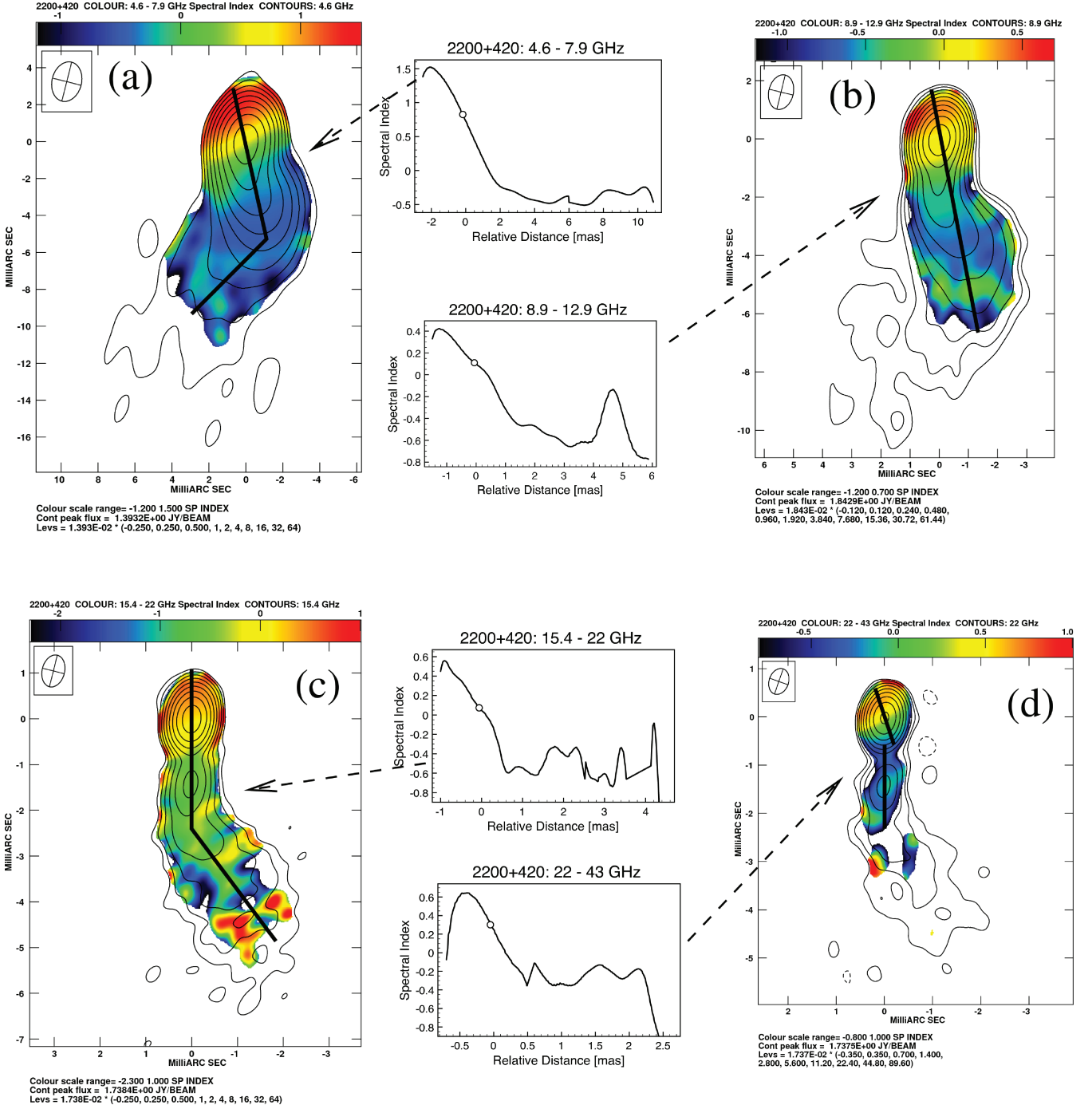
Figure 1. Spectral index maps for 2200+420 constructed from frequency pairs, with plots of slices along the jet region indicated by the solid line. (a) 4.6–7.9 GHz. Spectral index scale range: -1.2 to 1.5 . Clip levels of I maps: 3.5 mJy (4.6 GHz), 3.8 mJy (7.9 GHz). Beam FWHM and position angle: 2.17 \times 1.60 mas, -14^\circ (4.6 GHz). Contours: 4.6 GHz I , starting at 3.48 mJy and increasing by factors of 2. (b) 8.9–12.9 GHz. Spectral index scale range: -1.2 to 0.7 . Clip levels of I maps: 2.2 mJy (8.9 GHz), 6.8 mJy (12.9 GHz). Beam FWHM and position angle: 1.21 \times 0.84 mas, -14^\circ (8.9 GHz). Contours: 8.9 GHz I , starting at 2.21 mJy and increasing by factors of 2. (c) 15.4–22 GHz. Spectral index scale range: -2.3 to 1.0 . Clip levels of I maps: 5.2 mJy (15.4 GHz), 5.9 mJy (22 GHz). Beam FWHM and position angle: 0.71 \times 0.49 mas, -14^\circ (15.4 GHz). Contours: 15.4 GHz I , starting at 4.35 mJy and increasing by factors of 2. (d) 22–43 GHz. Spectral index scale range: -0.8 to 1.0 . Clip levels of I maps: 6.9 mJy (22 GHz), 13.3 mJy (43 GHz). Beam FWHM and position angle: 0.55 \times 0.40 mas, -19^\circ (22 GHz). Contours: 22 GHz I , starting at 6.08 mJy and increasing by factors of 2. The arrows connect the plots of the spectral index slices to their corresponding maps. The hollow circle on the slice plot indicates the core position at the lower frequency of the pair.
