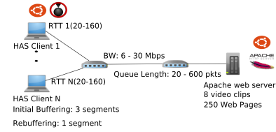
Fig. 1. Testbed Topology
