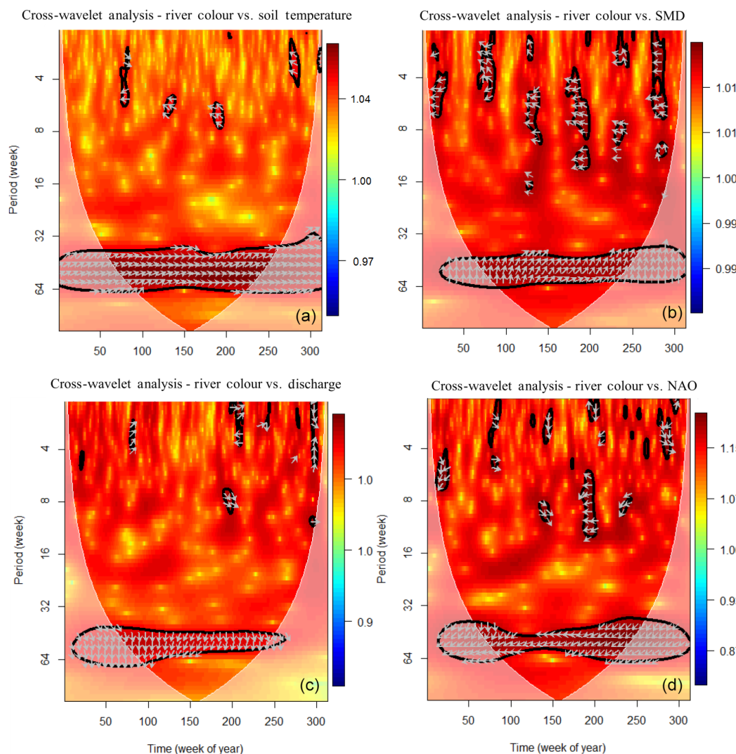
Figure 6. Cross-wavelet power spectrum of soil temperature at 1 m depth (a), soil moisture deficit (SMD) (b), river discharge in the Glenamong (c) and NAO (d) with river colour. Colour contours represent cross-wavelet power, and vectors indicate the relative phase relationship between the two time series (with in-phase pointing right, anti-phase pointing left, or a variable leading or following river colour by 90^\circ pointing straight down or up). The 5 % significance level is shown as a thick contour. Pink regions on either end indicate areas where the analysis is unreliable as there are no data before and after the study period.
