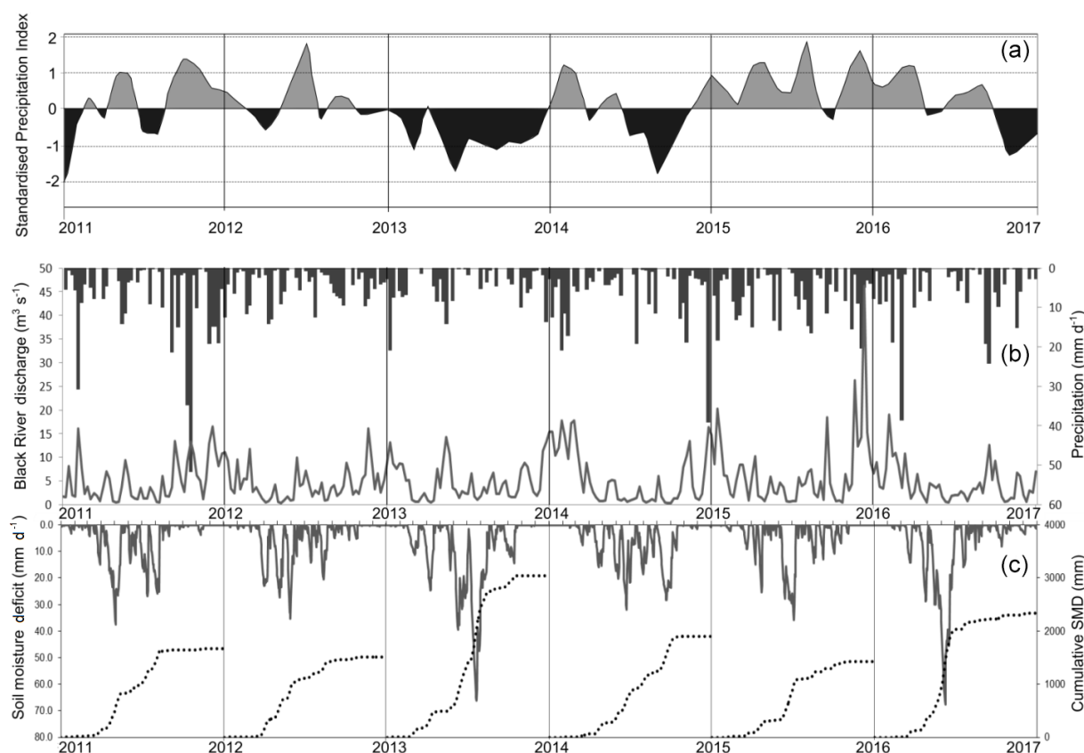
Figure 2. Panel (a) shows the 1-month Standardised Precipitation Index (SPI) calculated using precipitation data from the Newport climate station (reference period 1995 to 2010). Periods during which the index is > 1 represent moderately wet conditions, and periods during which the index < -1 indicate moderately dry conditions. (b) Black River discharge (grey line; \text{m}^3 \text{s}^{-1} ) and mean precipitation (black bars; \text{mm day}^{-1} ). (c) Cumulative soil moisture deficit (SMD) per year (mm; dotted line) and actual soil moisture deficit ( \text{mm day}^{-1} ; grey line).
