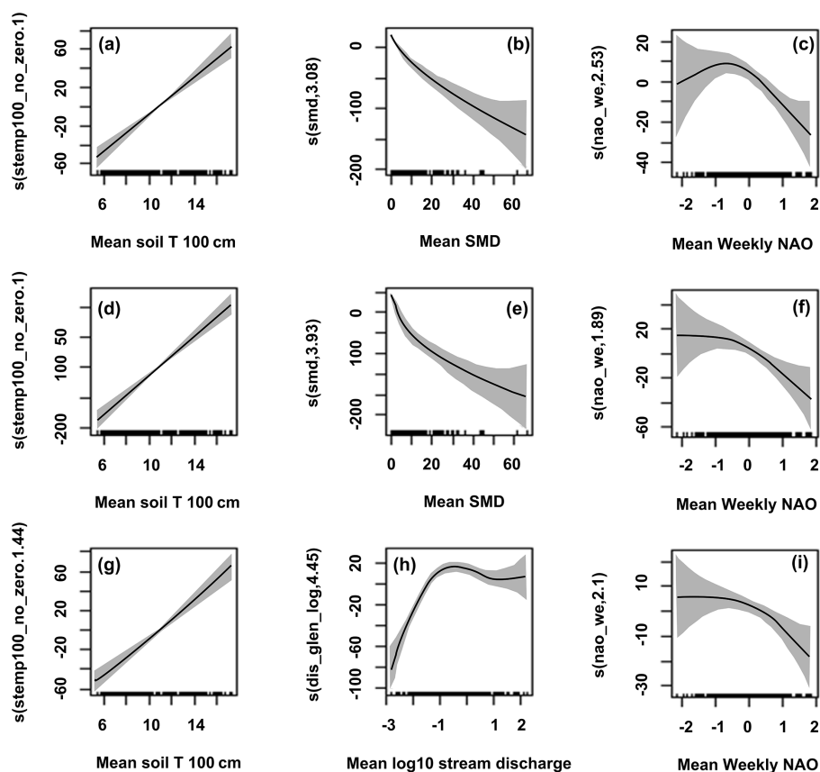
Figure 4. Selected smoothers for the contribution of explanatory variables for the optimal GAMM explaining water colour in each sub-catchment river: Black (a–c): (a) soil temperature, (b) soil moisture deficit (SMD) and (c) NAO; Srahrevagh (d–f): (d) soil temperature, (e) soil moisture deficit and (f) weekly NAO; Glenamong (g–i): (g) soil temperature, (h) log of discharge and (i) NAO. The solid line is the smoother, and the shaded area shows the 95 % confidence bands. The y axis units are the scaled smoother (s) for each explanatory variable with the variable name followed by the estimated degrees of freedom within the parentheses.
