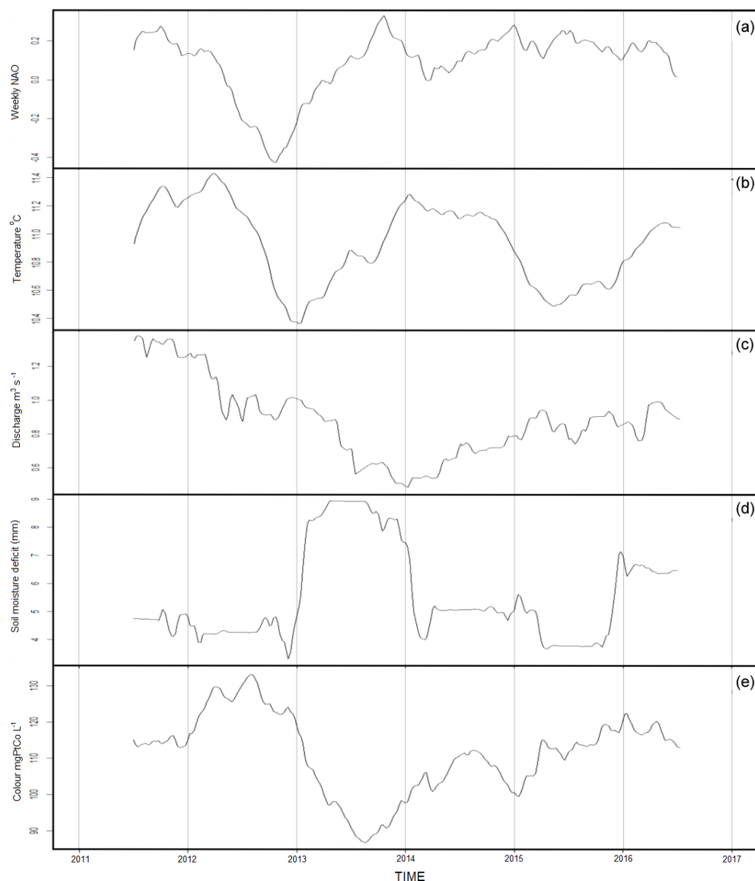
Figure 5. (a) Trend of weekly NAO during the study period, (b) trend of weekly soil temperature, (c) trend of weekly discharge in the Glenamong River, (d) trend of weekly soil moisture deficit (SMD) and (e) trend of mean weekly mean colour concentration in the three sub-catchment rivers.
