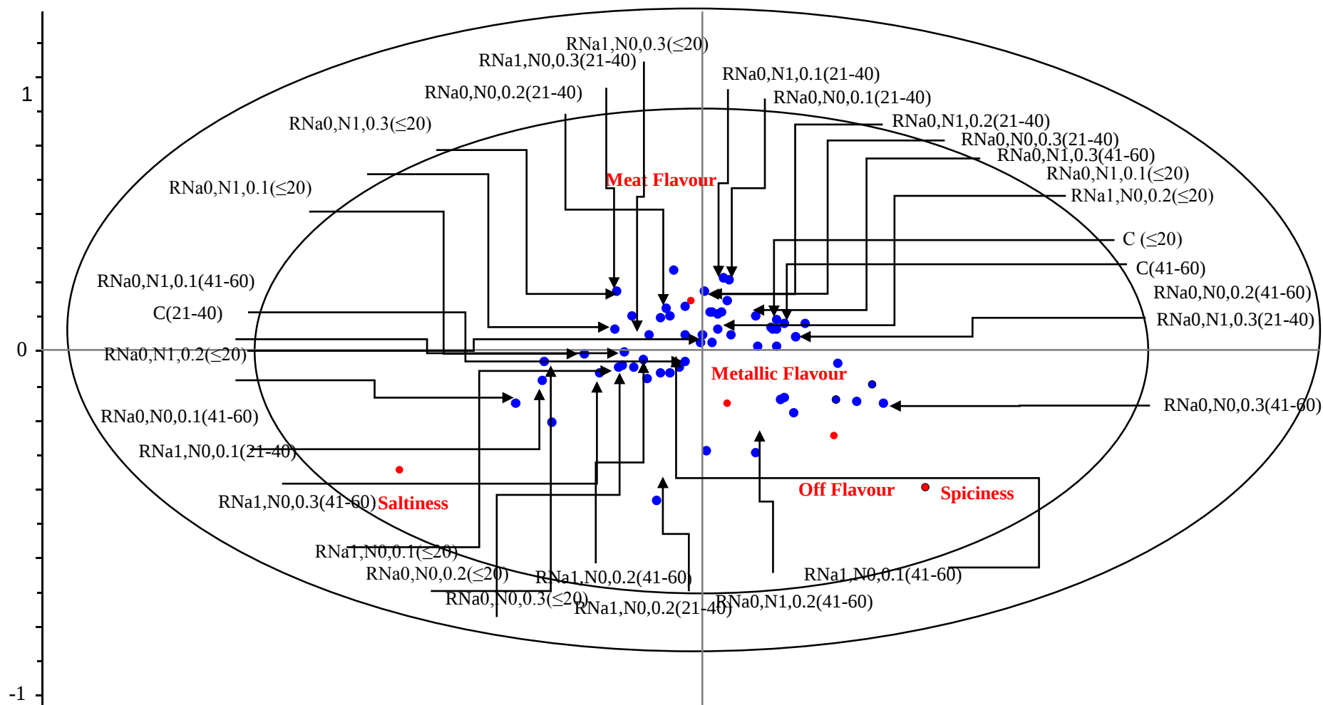
Figure 6.2: ANOVA – partial least squares regression (APLSR) correlation loading plot for each formulation, intensity descriptor and age category (≤20 yrs. old – 60 yrs. old) RNa = Reduced Sodium Salt, N = NaCl, M = MSG
