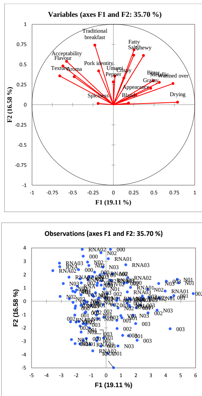
Figure 7.3. PCA illustrating attributes generated on training day 6
