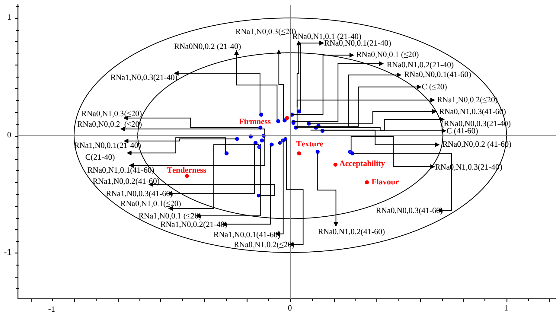
Figure 6.1: ANOVA – partial least squares regression (APLSR) correlation loading plot for each formulation, hedonic descriptor and age category (≤20 yrs. old – 60 yrs. old) RNA = Reduced Sodium Salt, N= NaCl
