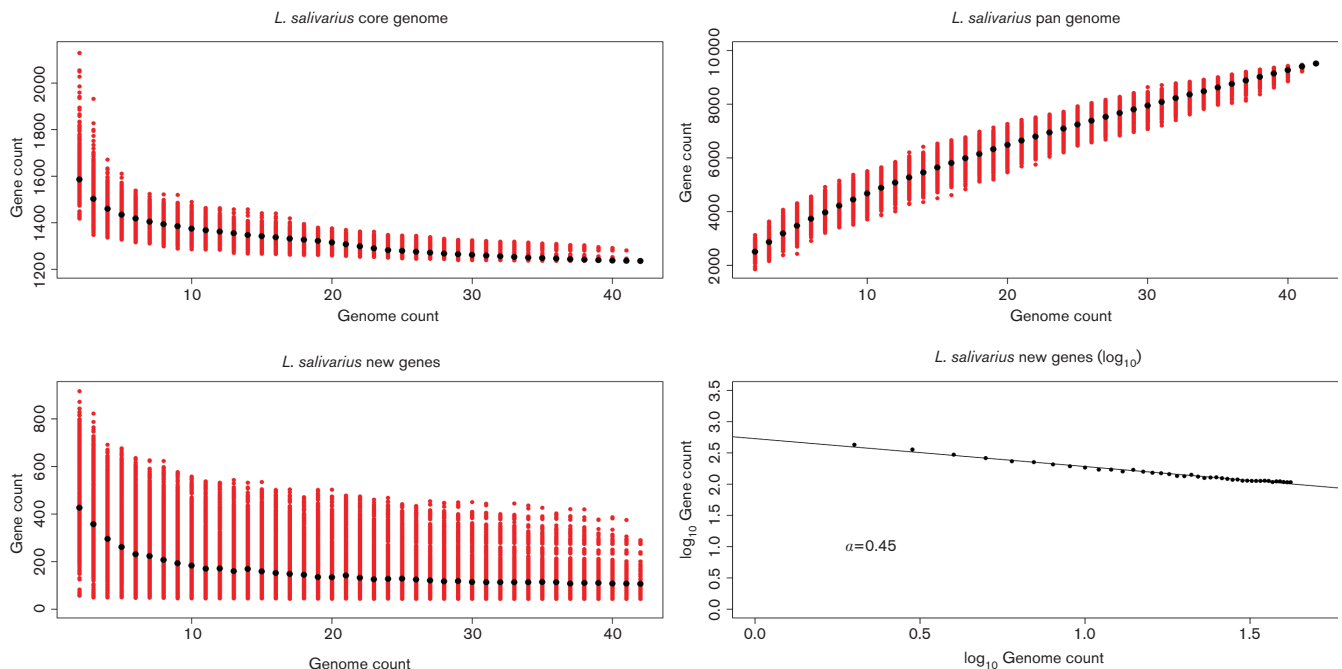
Fig. 1. A dataset of 42 genomes is not sufficient to define the L. salivarius pan-genome. The four panels show, with the sequential addition of 42 L. salivarius genomes (x-axis), the decrease in core genes (a; top-left), the increase in total genes (b; top-right), the decrease in new genes (c; bottom-left) and the log of the decrease in new genes (d; bottom-right). Genes are counted as orthologous gene families (percentage identity \geq 40 and percentage alignment length \geq 50 ) except for genes unique to each genome. The order of addition of genomes has been permuted 1000 times. Red dots show the variation in values while black dots show the median value. An alpha value of 0.44 shows that the pan genome of L. salivarius is open ( \alpha < 1 ).
