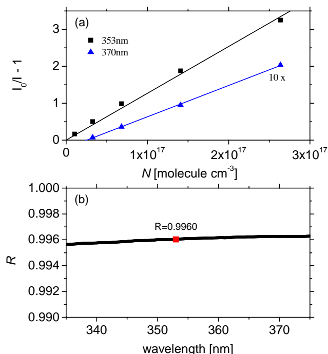
Fig. 2. (a) Fractional absorption of O_3 at 353 nm and 370 nm. The slope of the graph, \sigma_{O_3}d/(1-R) , was used to determine R based on the literature absorption cross-section at 353 nm. (b) Mirror reflectivity scaled to give the literature cross-section of O_3 absorption at 353 nm.
