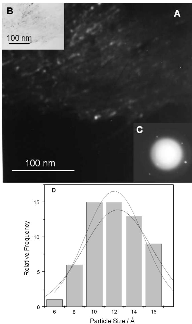
Fig. 3. Dark-field TEM image of the gold nanoparticles (Au-NPs) in acetone ( [\text{Au}]: 4 \times 10^{-3} \text{ mol dm}^{-3} ) (A). Bright-field TEM micrograph of randomly dispersed gold nanoparticles (B) and corresponding electron diffraction pattern (C). Histogram of Au-NPs size distribution. Gaussian fits are overlaid for comparison giving an average value of 1.2 nm for the nanoparticle diameter(D).
