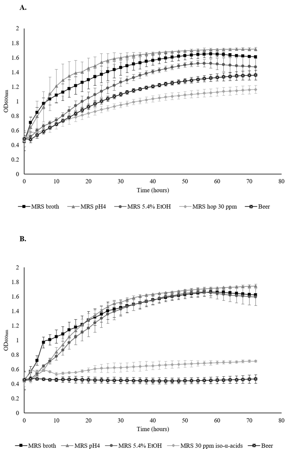
Figure 1. Growth of the WT beer-spoiling strain Lb. brevis UCCLBBS124 ( A ) and its plasmid-cured derivative MB569 ( B ) in beer, MRS broth, MRS broth at pH 4.0 and MRS broth supplemented with 5.4 % ethanol or 30 ppm iso - \alpha -acids.
