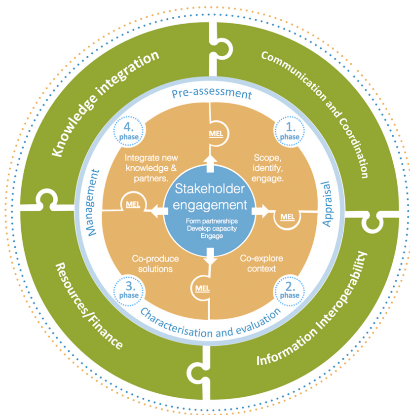
Fig. 6. Risk-Tandem framework
