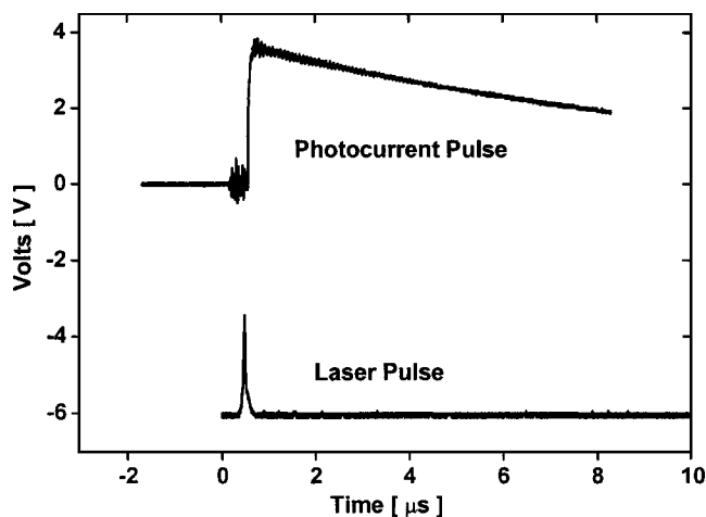
FIG. 2. Oscillogram of an induced photocurrent signal together with femtosecond UV pulse.
