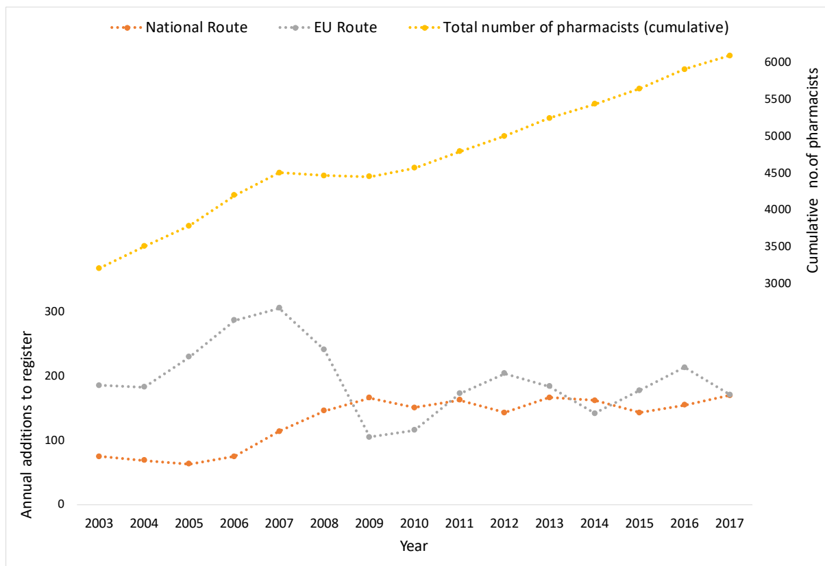
Figure 1. Graph showing total number of pharmacists added to the PSI register annually via national and EU routes and total number of pharmacists in Ireland (cumulative) between 2003 and 2017. Data taken from PSI Annual Reports 2004-2016 and PSI Statistics(9).
