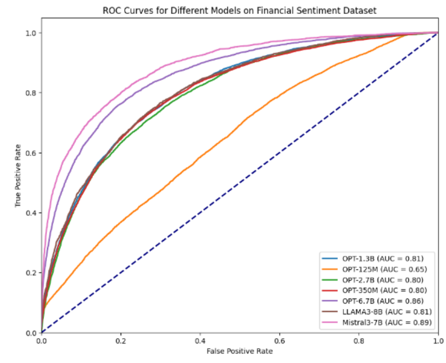
Figure 4. Receiver operating curve of different models on Financial Sentiment classification dataset.
