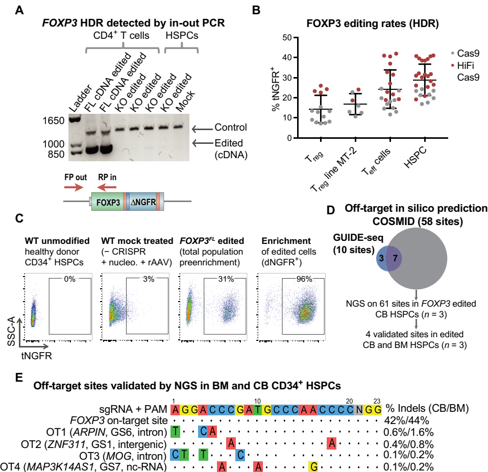
Fig. 2. CRISPR combined with a rAAV6 homology donor enables precise HDR-mediated FOXP3 cDNA transgene insertion into the endogenous locus. (A) Editing observed at the DNA level by an in-out PCR strategy that uses a primer inside the inserted divergent cDNA construct and a second primer outside of the 5' arm of homology. Control band represents unmodified region in the FOXP3 gene as a positive control for the presence of genomic DNA. PCR using in-out primers resulted in band only present in samples in which the cDNA was inserted (FL cDNA) and not in FOXP3 knockout (KO) or mock-treated samples. After the ladder, the first four lanes represent CD4 + T cells, and the last three lanes represent HSPCs. (B) Rates of HDR-mediated FOXP3 editing detected by flow cytometry for tNGFR marker gene expression in primary human CD4 + CD25 + T regs , MT-2 T reg cell line, primary CD4 + CD25 + T eff cells, and CD34 + HSPCs. Editing rates with standard Sp Cas9 (gray) and high-fidelity (HiFi) Cas9 (red) are shown for comparison. Dots represent cells from individual donors. (C) Representative flow cytometry plots showing tNGFR marker gene expression in edited cord blood-derived CD34 + HSPCs. Negative control: Mock-treated cells nucleofected with phosphate-buffered saline in place of CRISPR and transduced with rAAV6- FOXP3 donor. Edited cells enriched using tNGFR selection and purity are shown by flow cytometry. SSC-A, side scatter area. (D) Venn diagram showing overlap in predicted off-target sites identified by COSMID in silico prediction and GUIDE-seq DSB capture. All predicted sites were tested by NGS in edited CD34 + HSPCs derived from cord blood (CB) and validated by NGS in edited bone marrow (BM)-derived HSPCs. (E) The four off-target (OT) sites validated by NGS shown with highlighted mismatches in off-target site versus FOXP3 sgRNA target sequence, closest gene name, gene region, and average frequency of indel mutations detected by NGS (mean, n = 3).
