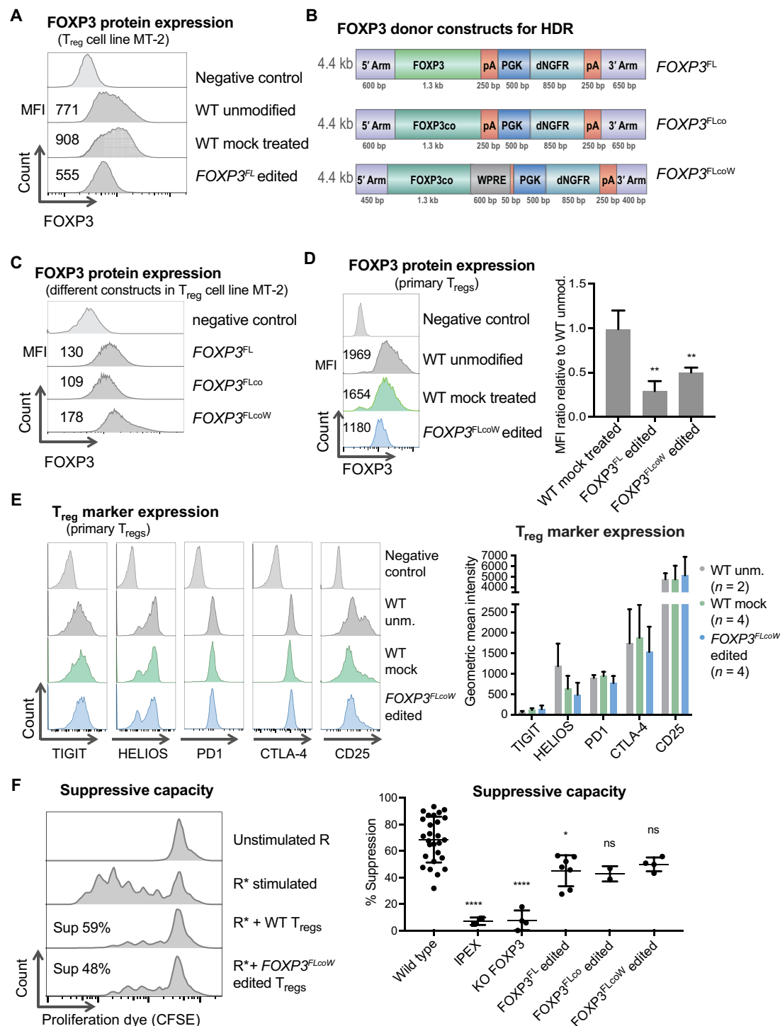
Fig. 3. FOXP3 edited T_{regs} express FOXP3 protein and display characteristic in vitro phenotype and function. (A) Quantification of FOXP3 protein expression in the MT-2 T_{reg} cell line by flow cytometry, showing median fluorescence intensity (MFI) values for one representative experiment out of three performed. (B) FOXP3 homology donor constructs designed to improve FOXP3 protein expression, including further codon optimization ( FOXP3^{FLco} ) and addition of a WPRE element ( FOXP3^{FLcoW} ). (C) Flow cytometry for FOXP3 in MT-2 cells comparing the different donor constructs. (D) FOXP3 expression in primary T_{regs} by flow cytometry and quantification represented as ratio of MFI in treated cells versus WT unmodified T_{regs} [mean \pm SD, one-way analysis of variance (ANOVA), Tukey's multiple comparisons]. Significance comparing FOXP3^{FL} ( n=2 , **P < 0.01 ) or FOXP3^{FLcoW} ( n=6 , **P < 0.01 ) to WT mock treated ( n=2 ). (E) Expression of signature T_{reg} marker proteins on primary T_{regs} by flow cytometry and corresponding quantification (mean \pm SD, n=2 to 4). (F) Suppression assay showing unstimulated responders (R), stimulated responders ( R^* ) alone or in coculture with T_{regs} , and calculated percent suppression. Responders stained with proliferation dye, carboxyfluorescein diacetate succinimidyl ester (CFSE). Average suppressive potential over several independent experiments is quantified (right). Significance comparing the WT T_{regs} with following T_{regs} : IPEX, FOXP3 KO, FOXP3^{FL} edited, FOXP3^{FLco} edited, and FOXP3^{FLcoW} edited (mean \pm SD, one-way ANOVA, Tukey's multiple comparisons test, *P < 0.05 ; ****P < 0.0001 ; ns, not significant).
