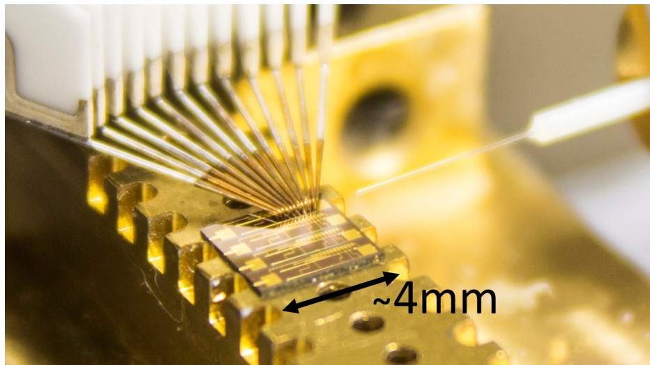
Figure 1.9: Photonic integrated circuit under test. This particular circuit integrates several lasers, splitters, and combiners, measuring approximately 4 mm in length. A multi-contact probe and lensed optical fibre for testing purposes are shown [70, 71].
