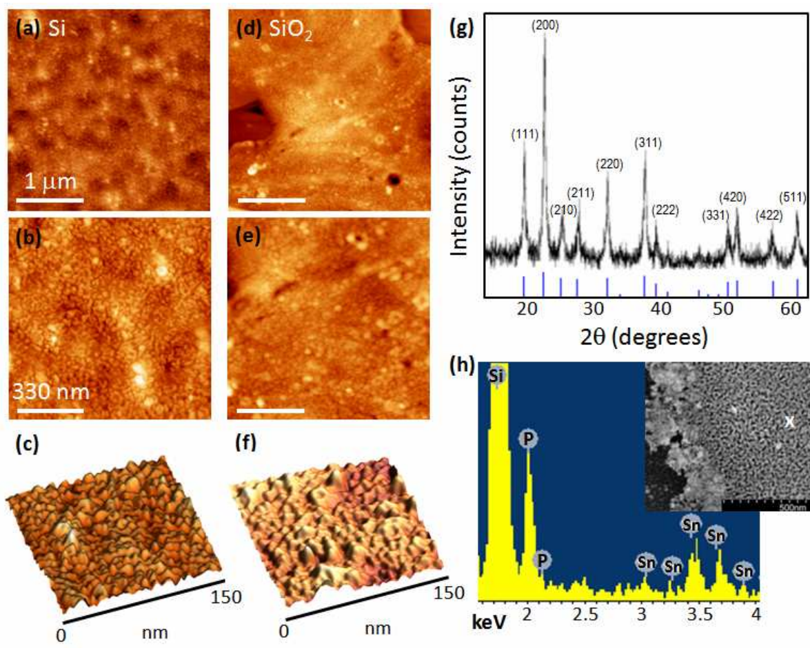
Figure 6. Morphological scans of the SnP 2 O 7 product on (a-c) Si and (d-f) SiO 2 at several magnifications. The labyrinthine arrangement of the dielectric SnP 2 O 7 materials is apparent, with greater surface uniformity routinely observed for deposition on Si, with a higher density of areal defects (vacancies in coverage) in depositions on SiO 2 . (g) XRD pattern of the pyrolytic SnP 2 O 7 product from (4) displaying only peaks corresponding to tin diphosphate, SnP 2 O 7 (JCPDS card No. 00-029 1352); no peaks for SnO 2 were observed. (h) EDX spectrum acquired from localized regions of the SnP 2 O 7 deposit as shown in the inset: at% Si K α (85.32); P K α (9.84); Sn L α (4.84).
