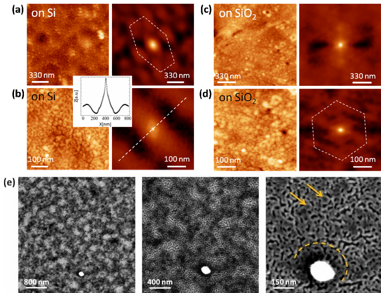
Figure 8 (a) 1.5 \times 1.5 \mu\text{m}^2 and (b) 0.5 \times 0.5 \mu\text{m}^2 AFM images of the \text{SnP}_2\text{O}_7 deposit on Si with corresponding correlation length maps. ( Inset ) 2D profile corresponding to the dashed line in the correlation map of AFM image (b). (c) 1.5 \times 1.5 \mu\text{m}^2 and (d) 0.5 \times 0.5 \mu\text{m}^2 AFM images of the \text{SnP}_2\text{O}_7 deposit on \text{SiO}_2 with corresponding correlation length maps. (e) SEM images at successively higher magnifications of a single area of deposit on Si. The white feature serves as comparison position marker and also a nucleation point for cyclic \text{SnP}_2\text{O}_7 . The dashed arc delineates cyclic structures.
