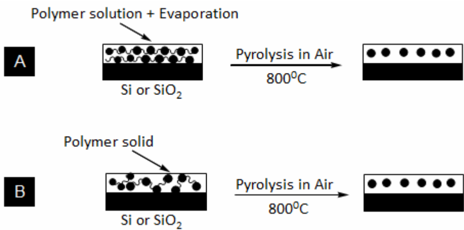
Scheme 3 Schematics of the two approaches, Method A and Method B (see main text for description) employed to created metallic nanostructured surfaces on Si or SiO 2 .
