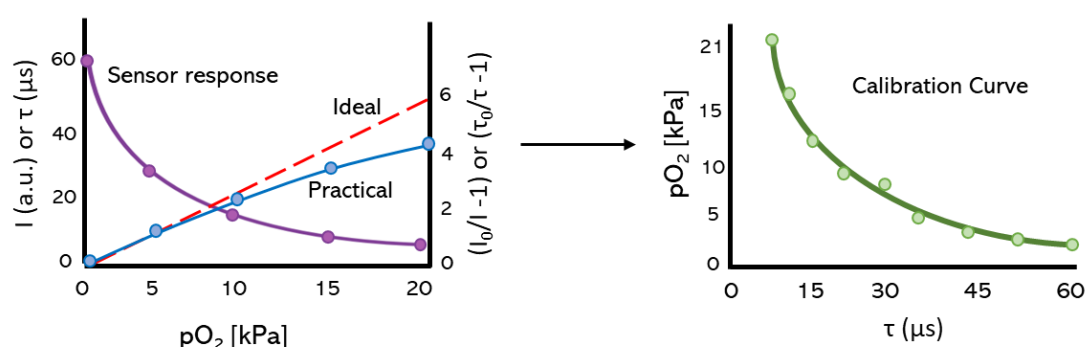
Figure 1.2: Plot of the luminescence intensity or decay time quenched by oxygen and the corresponding ideal and practical Stern–Volmer plots. Image modified from(21). Example of calibration curve obtained by measuring the lifetime of a phosphor at different known [O_2] between 0 and 21 kPa.
