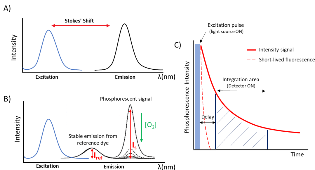
Figure 1.3: Intensity-based detection modes. A) Steady-state intensity measurements at one wavelength. B) Ratiometric intensity measurement: emission spectra measured at different [O_2] concentrations using an oxygen sensitive indicator dye and an O_2 insensitive reference dye (fluorescent or phosphorescent). C) TRF intensity measurements.
