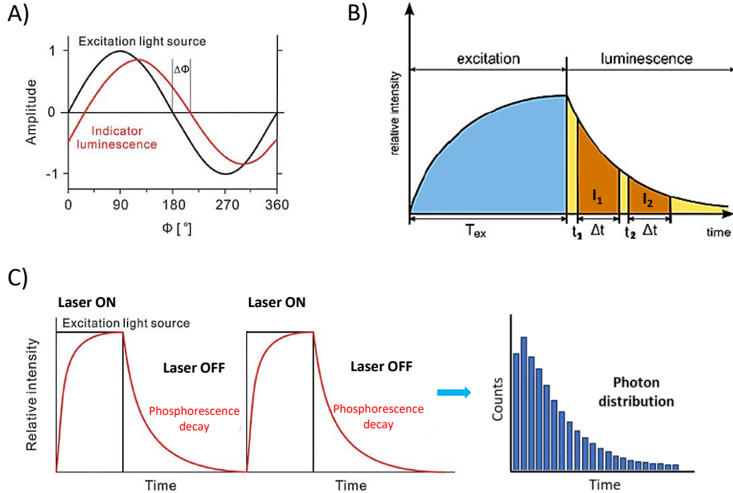
Figure 1.4: Examples of lifetime based measurements using A) frequency domain fluorometry, B) rapid lifetime determination (RLD) (84), or C) time-correlated single photon counting (TCSPC) (21).
