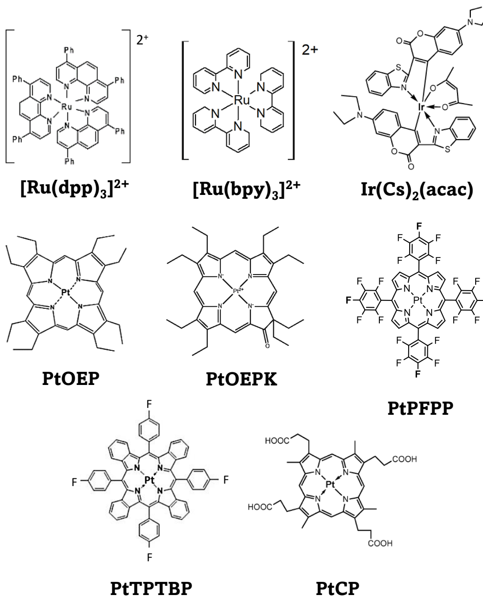
Figure 1.5: Examples of the most common O 2 -sensitive dyes. Structures obtained from (5, 10, 48, 113). [Ru(dpp) 3 ] 2+ - Ru(II)-tris(diphenylphenantroline) chloride; [Ru(bpy) 3 ] 2+ - ris(bipyridine)ruthenium(II) chloride; Ir(Cs) 2 (acac) - Ir(III)-(benzothiazol-2-yl)-7-(diethylamino)-coumarin acetylacetonate; PtOEP - Pt(II)-octaethylporphyrin; PtOEPK - Pt(II)-octaethylporphine ketone; PtPFPP - Pt(II)-tetrakis(pentafluorophenyl)porphine; PtTPTBP - Pt(II)-tetraphenyltetrabenzoporphyrin; PtCP - Pt(II)-coproporphyrin.
