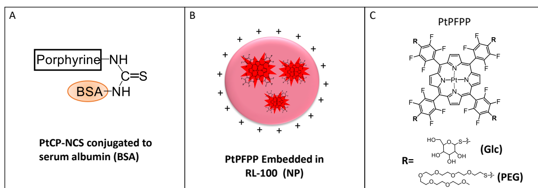
Figure 5.2: Schematic representation of the O 2 probes used in the study: A) The MitoXpress probe comprising a macromolecular conjugate of Bovine Serum Albumin (BSA) with PtCP-NCS phosphor. B) NanoO 2 probe comprising core-shell nanoparticles of a cationic hydrogel, RL-100 with embedded PtPFPP molecules. C) Small molecule probes: tetra-PEGylated, PtmPEG 4 , and tetra-glucosylated, Pt1Glc 4 , derivatives of PtPFPP phosphor.
