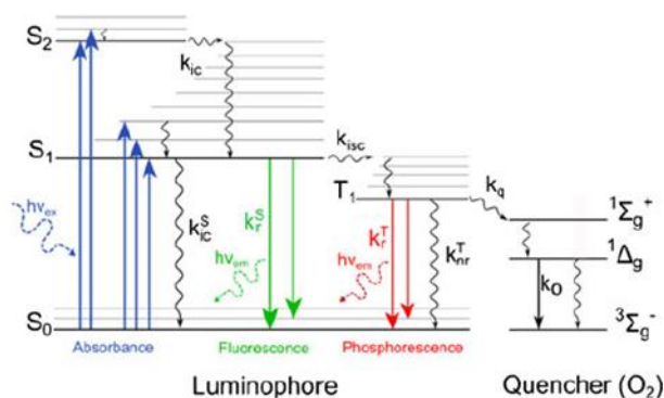
Figure 1.1: Perrin-Jablonski diagram, adopted from (64).
