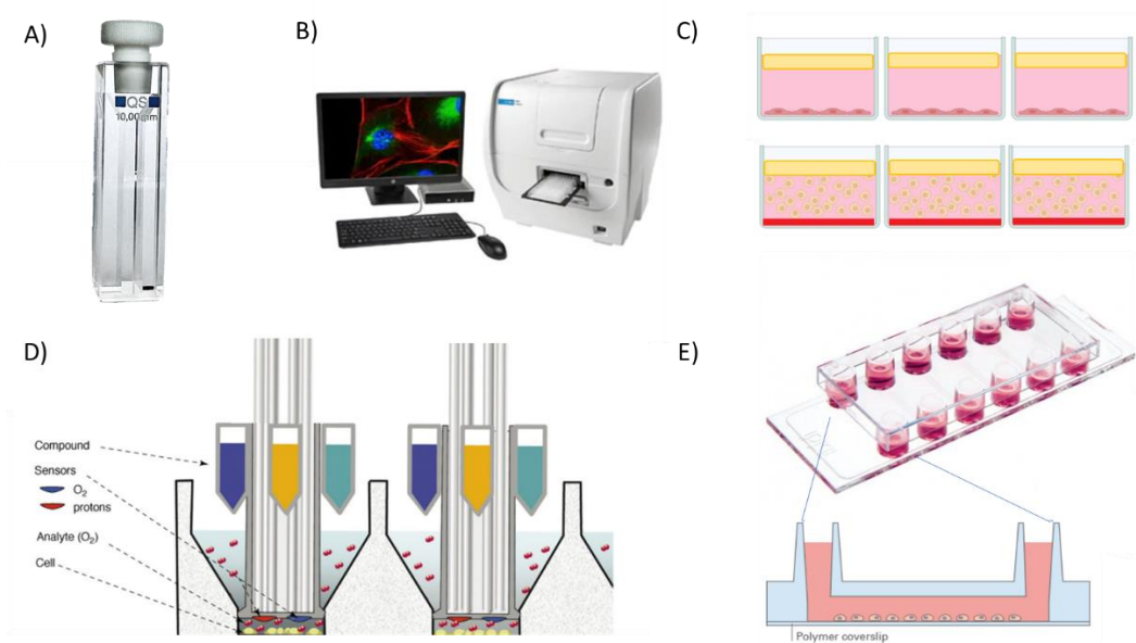
Figure 1.7: Common OCR measurements setups. A) Hermetically sealed quartz cuvette with Teflon stopper. B) BioTek (Agilent) Cytation 5 Cell Imaging Multimode Reader equipped with atmospheric control. C) Microwells sealed with oil, with either adherent cells (or suspension) and soluble probe, or suspension cells and sensor coating. D) Seahorse XF Analyser for OCR and ECAR measurements on adherent cells (222). E) A six channel \mu -Slide for parallel flow assays (Ibidi.com).
