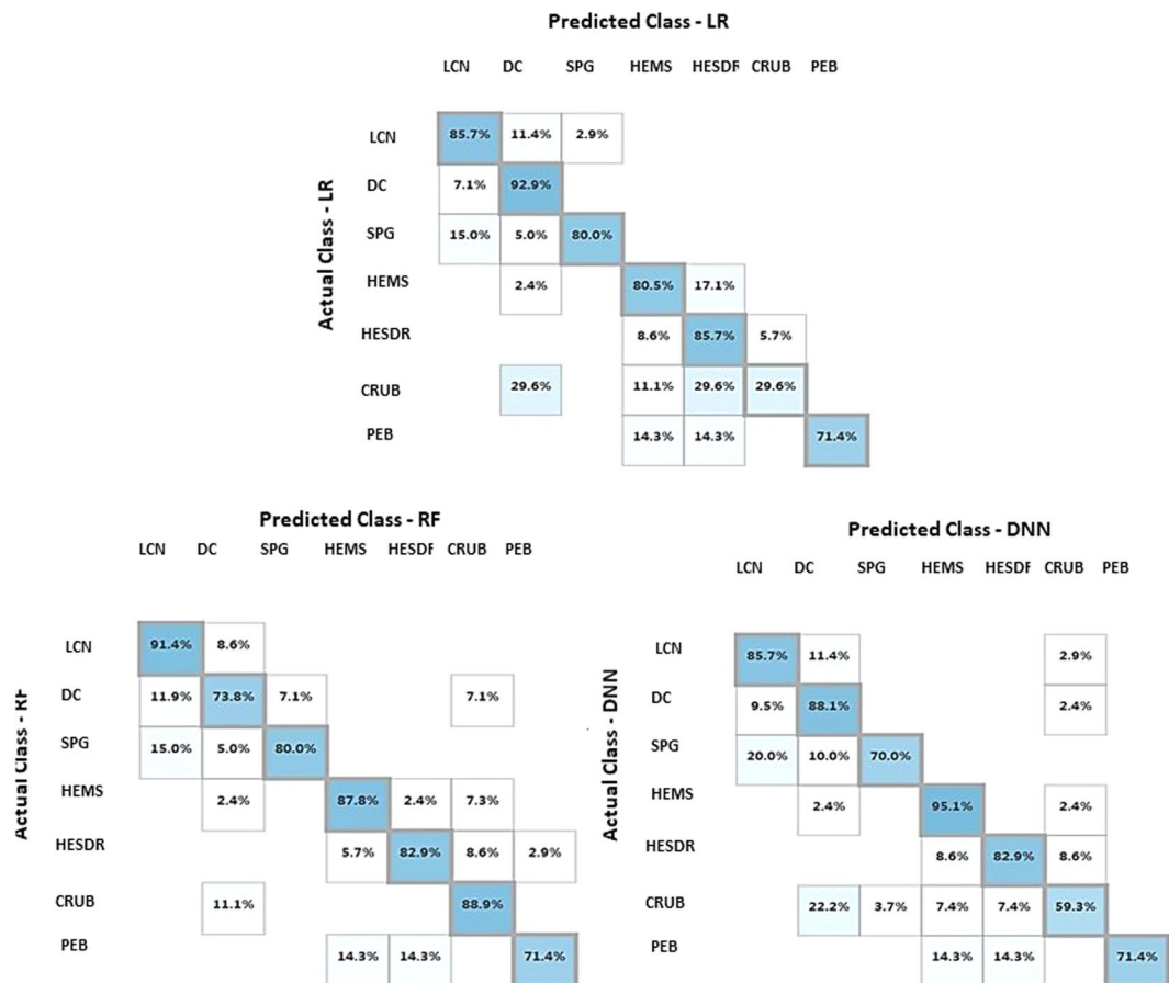
Figure 6. Accuracy matrix for classification methods LR, RF and DNN: Classes: LCN) Live Coral Framework; DC) Dead Coral Framework; SPG) Sponges; HEMS Hemipelagic Sediments; HESDR) Hemipelagic Sediments with Dropstones; CRUB) Coral Rubble; and PEB) Pebbles.
