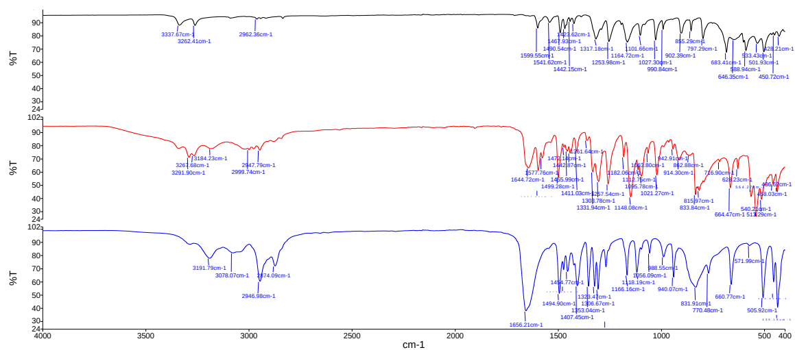
Figure S6: Stacked IR comparison of 4-OMeBSA-VLM cocrystal. (top – bottom, sulfonamide, cocrystal, valerolactam).
