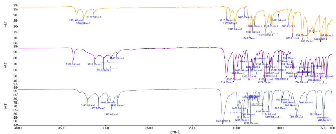
Figure S7: Stacked IR comparison of 4-NBSA-CPR cocrystal. (top – bottom, sulfonamide, cocrystal, caprolactam).
