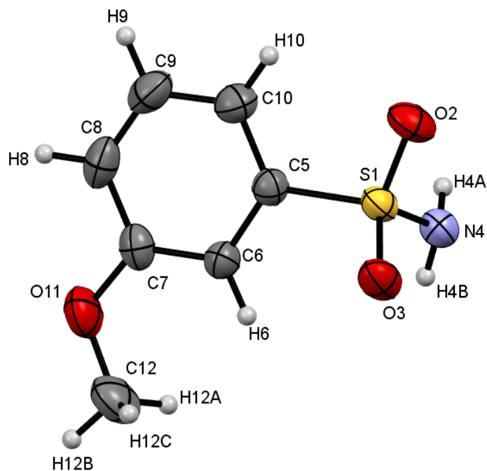
Figure S4: ORTEP diagram of 2 , with numbering scheme. Thermal ellipsoids are drawn at the 50% level.
