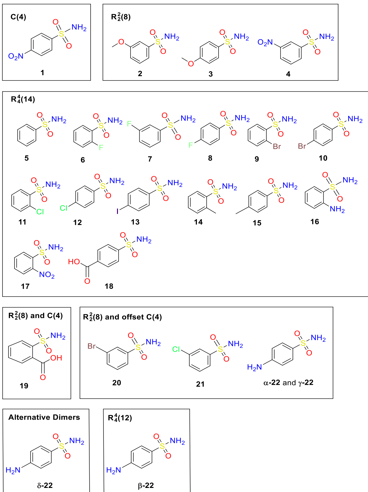
Figure 2.2 Sulfonamides (1–22) investigated in this study and arranged by the hydrogen-bonding motifs observed in their crystal structures, using Etter's graph set notation. 7-9
