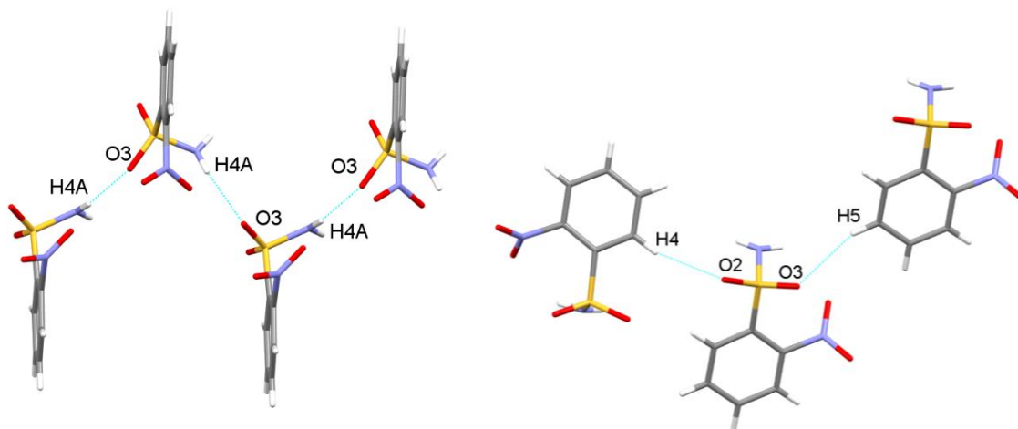
Figure S34: Hydrogen bonding in 17.
