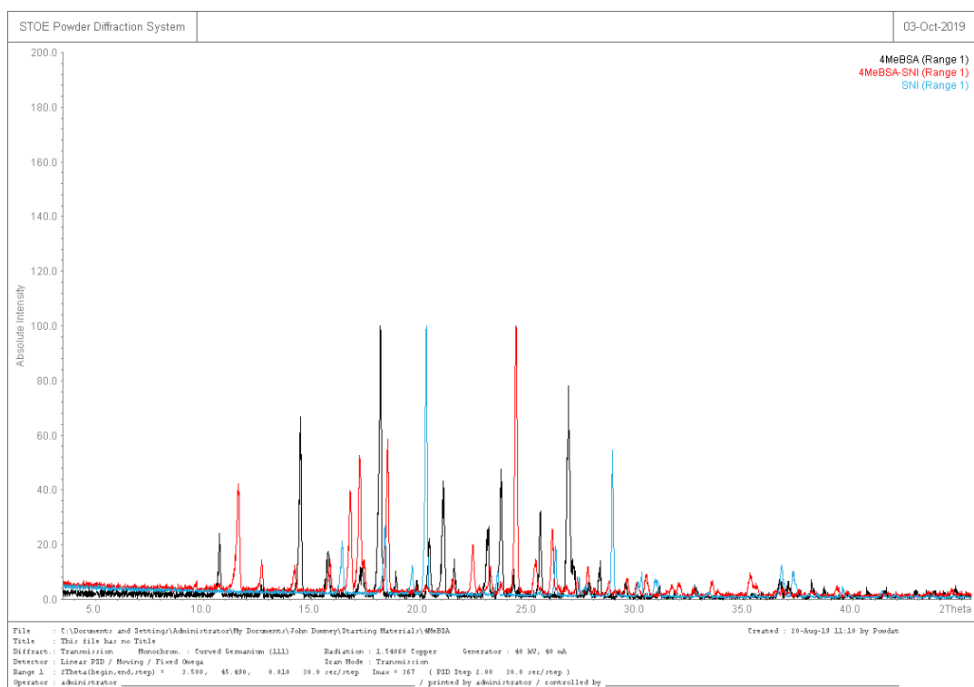
Figure S1: Overlay PXRD comparison of 4MeBSA-SNI (1:1) cocrystal.
