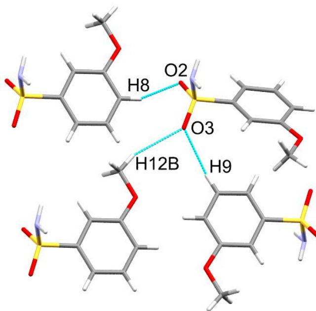
Figure S5: Weak C-H \cdots O=S hydrogen bonding in 2 .
