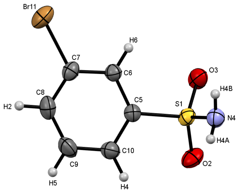
Figure S39: ORTEP diagram of 20 , with numbering scheme. Thermal ellipsoids are drawn at the 50% level.
