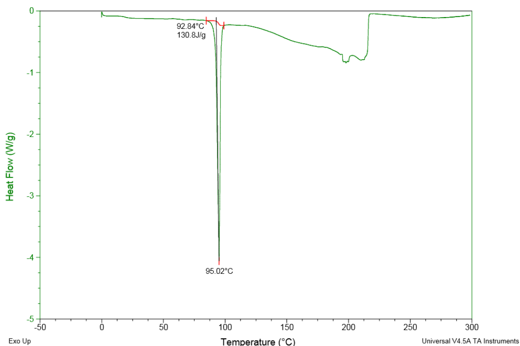
Figure S8: 4-MeBSA-SNI cocrystal.
