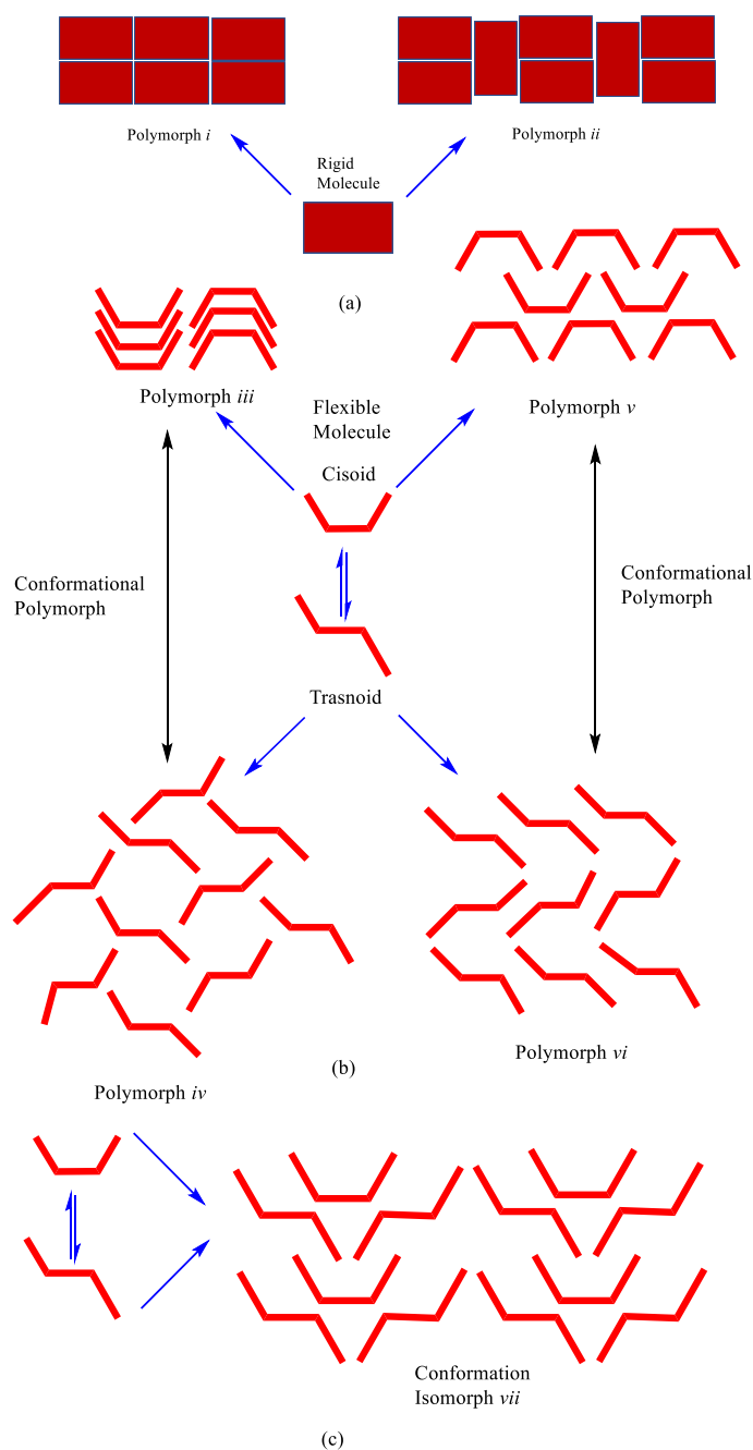
Figure 1.4: Schematic diagram of a) conformational polymorphism, b) synthon polymorphism and c) packing polymorphism, adapted from reference 16.
