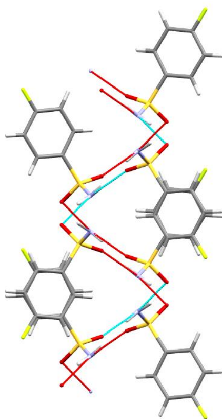
Figure S52: View of along the b -axis in 8 showing the zig-zag arrangement of the tetramers.
