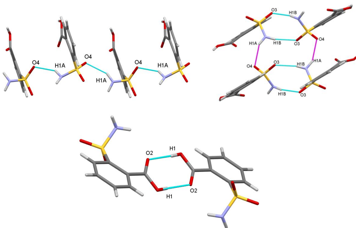
Figure S62: Hydrogen bonding in 19 . The blue and pink hydrogen bonding indicates the individual C(4) hydrogen bonding at the unitary level. The C(4) chains are related by the 2_1 -fold screw axis along the b-axis and a glide plane perpendicular to the b-axis. There is also a 2_1 -fold rotation axis along the b-axis. 15
