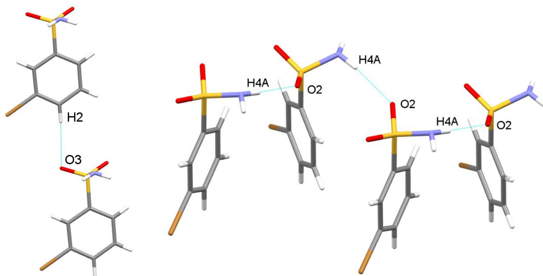
Figure S40: Hydrogen bonding in 20 .
