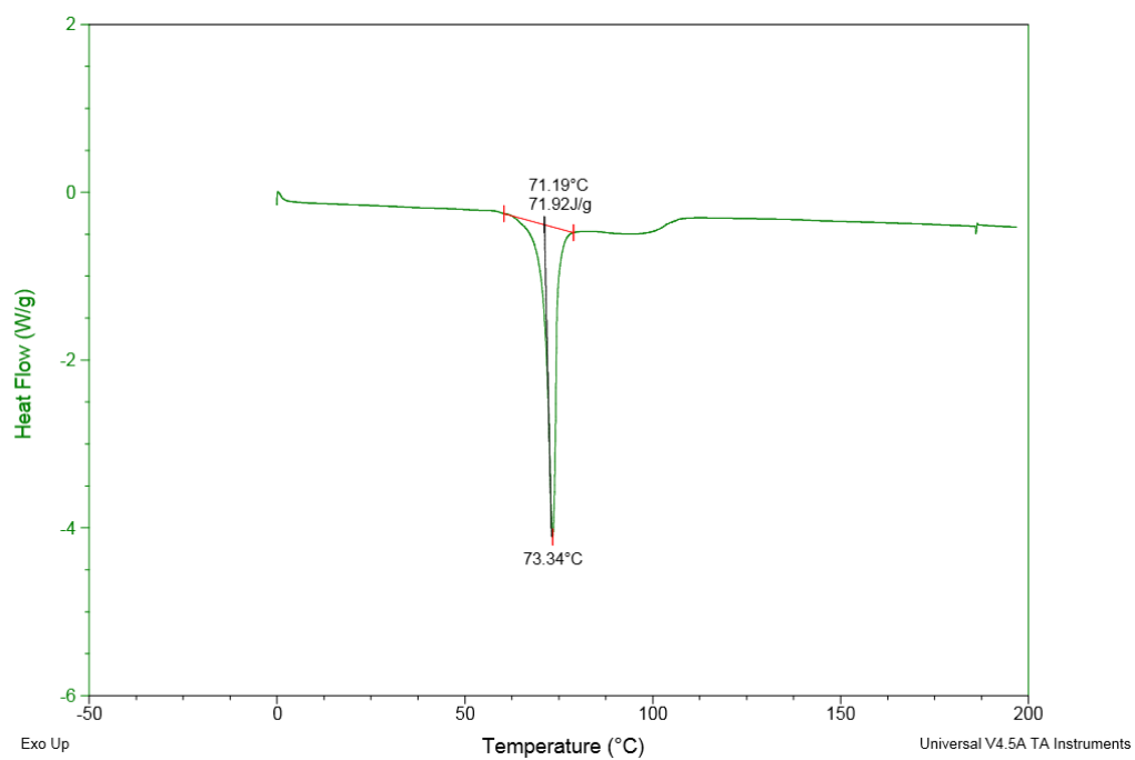
Figure S9: 4-OMeBSA–VLM cocrystal.
