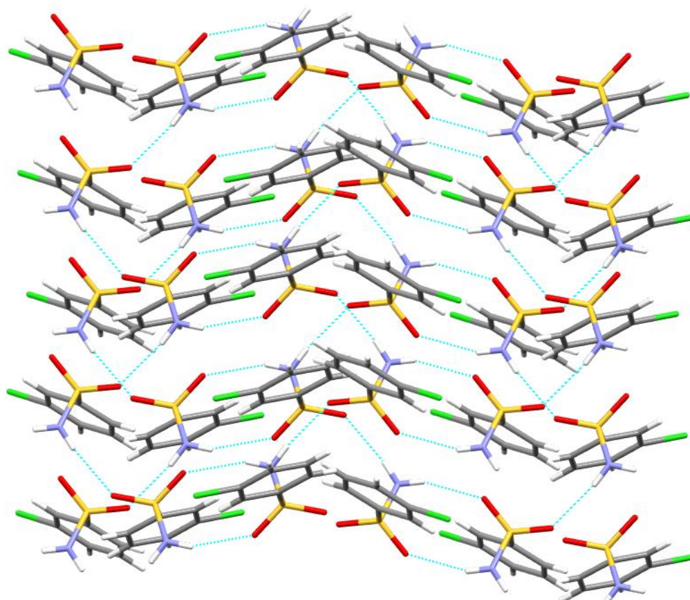
Figure S47: Packing diagram of 21 .
