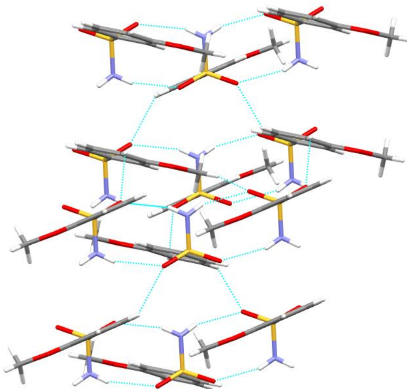
Figure S5: Weak C-H \cdots O=S hydrogen bonding in 2 .
