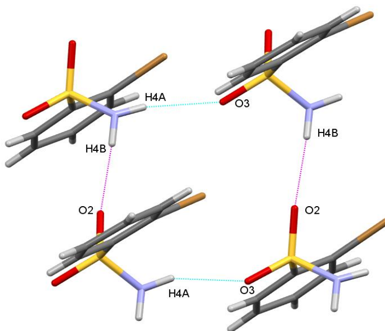
Figure 2.5: The R_4^4(14) motif observed for compound 9 .
