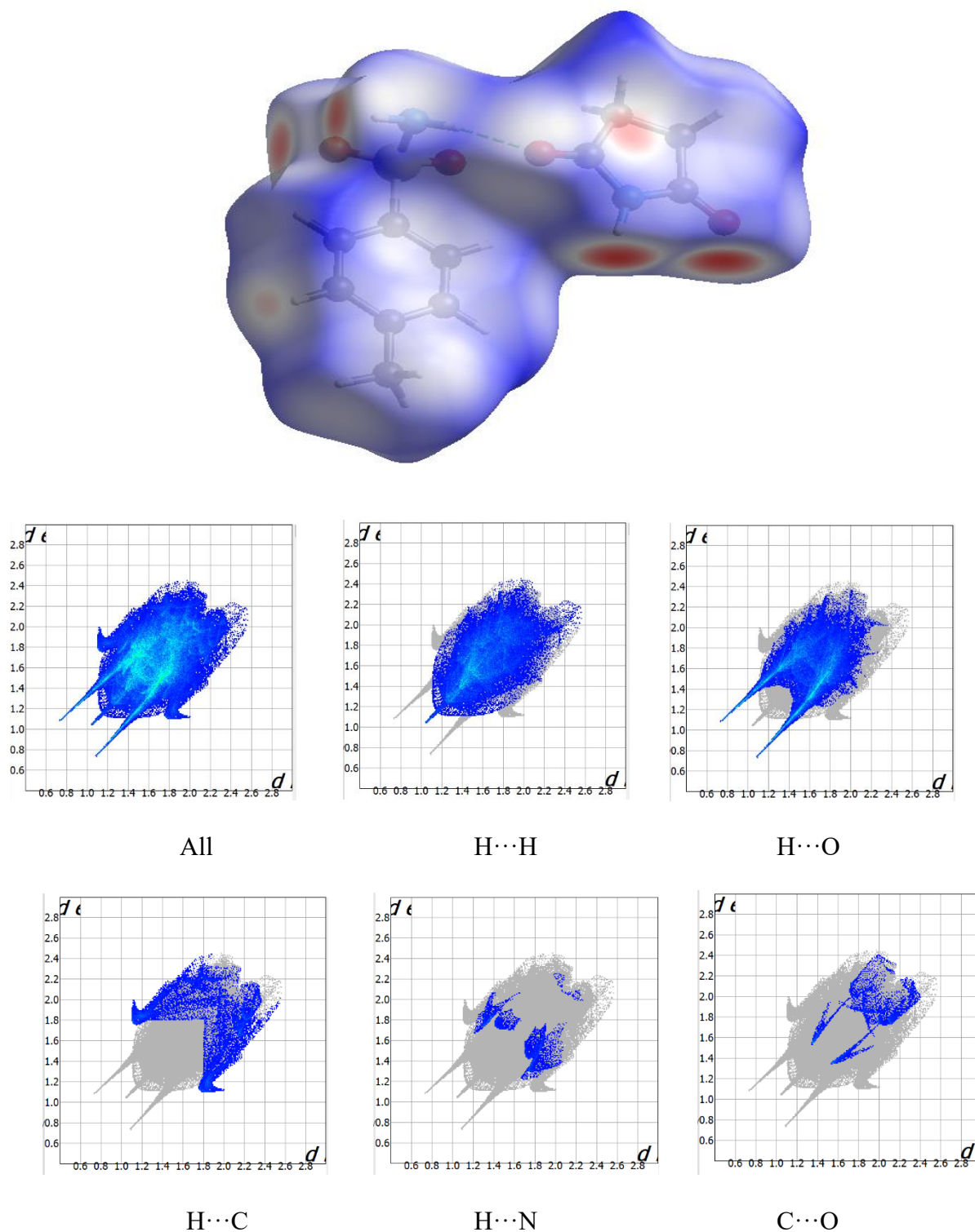
Figure 3.4: Hirshfeld surfaces of the 4-MeBSASNI cocrystals, top, and 2D fingerprint plots of the intermolecular contacts in the 4-Me-BSASNI cocrystals, bottom.
