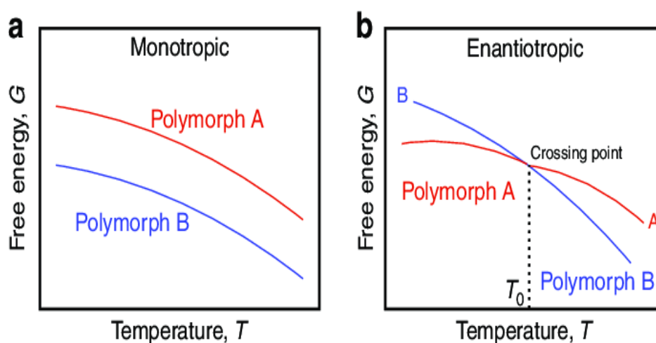
Figure 1.6: Outline of monotropic and enantiotropic systems. 20
