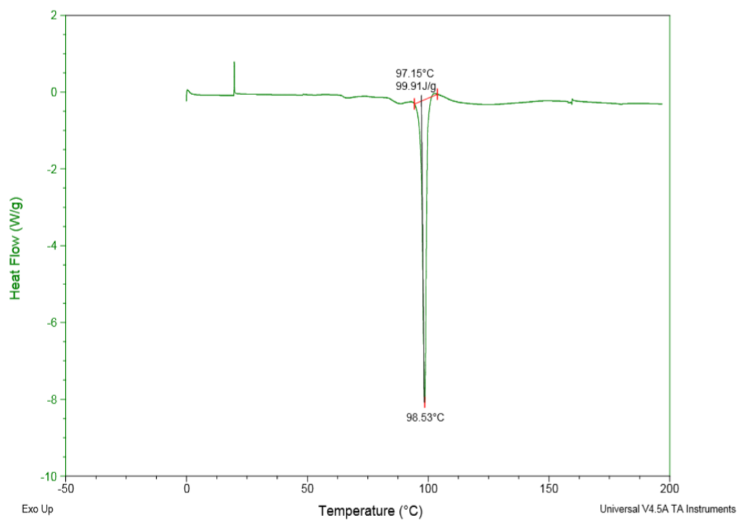
Figure S9: 4-OMeBSA–VLM cocrystal.
