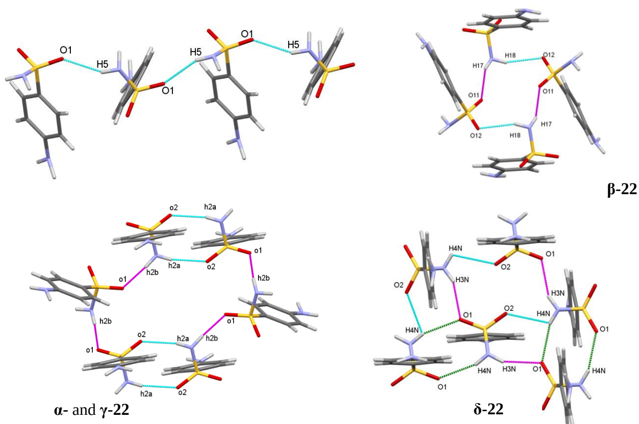
Figure S63: Hydrogen bonding in 22 . The blue and pink hydrogen bonding indicates the individual C(4) hydrogen bonding at the unitary level. The C(4) chains are related by the 2_1 -fold screw axis along the b-axis and a glide plane perpendicular to the b-axis. 11-14
