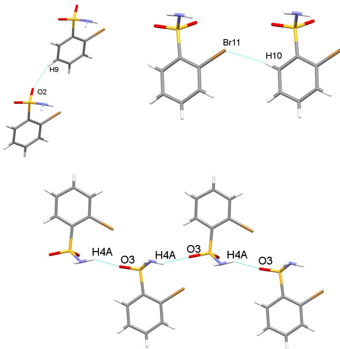
Figure S28: Hydrogen bonding in 9 .
