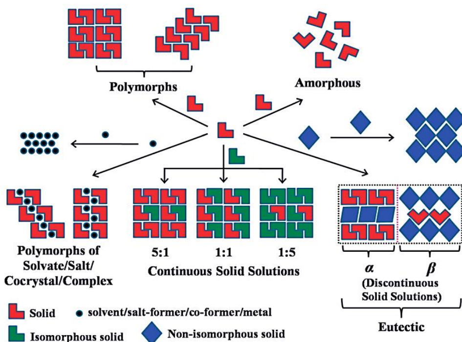
Figure 1.9: Diagram proposing eutectics can be classified under crystal engineering principles. 45
