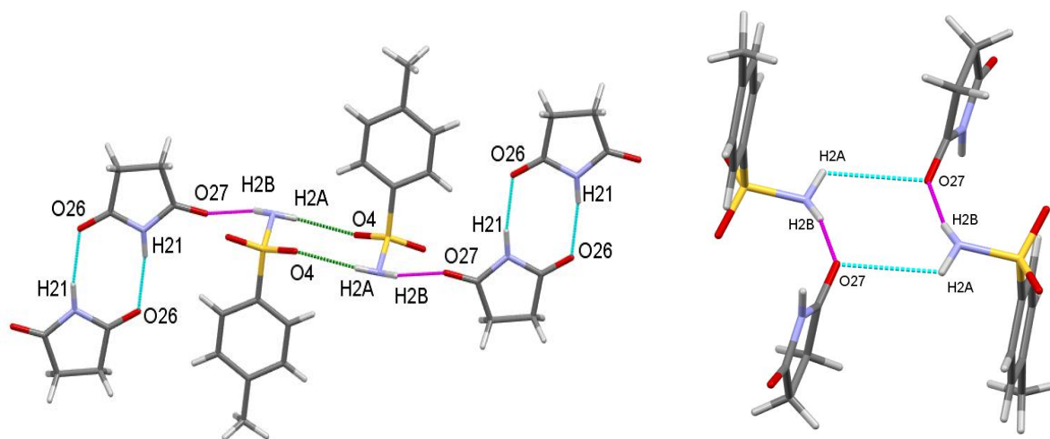
Figure 3.3: Syn N-H catemer and succinimide/sulfonamide dimers, (top) and tetramer ring (bottom).
