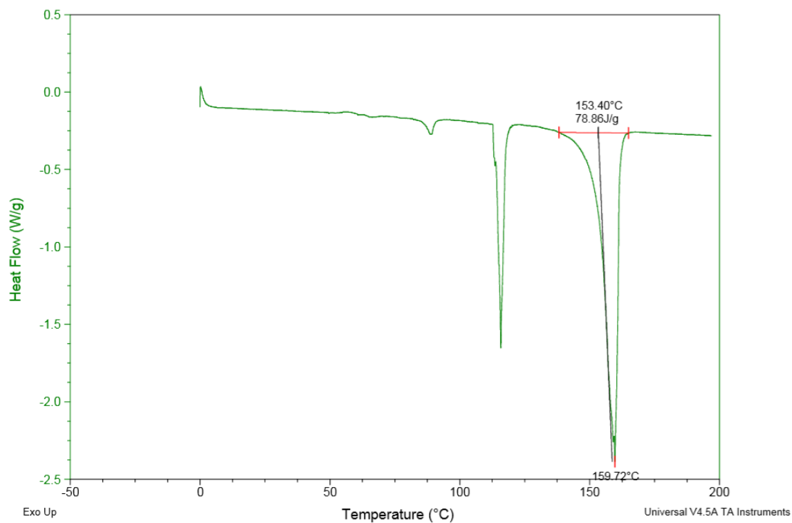
Figure S14: DSC data of 6 .
