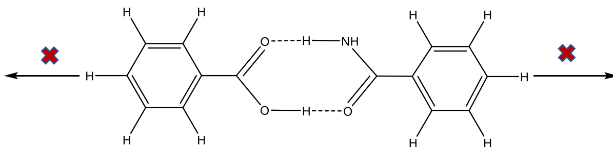
Figure 1.11: The absence of secondary-auxiliary interactions in benzoate-benzamide system means a eutectic product will form instead of a cocrystal, adapted from reference 45.
