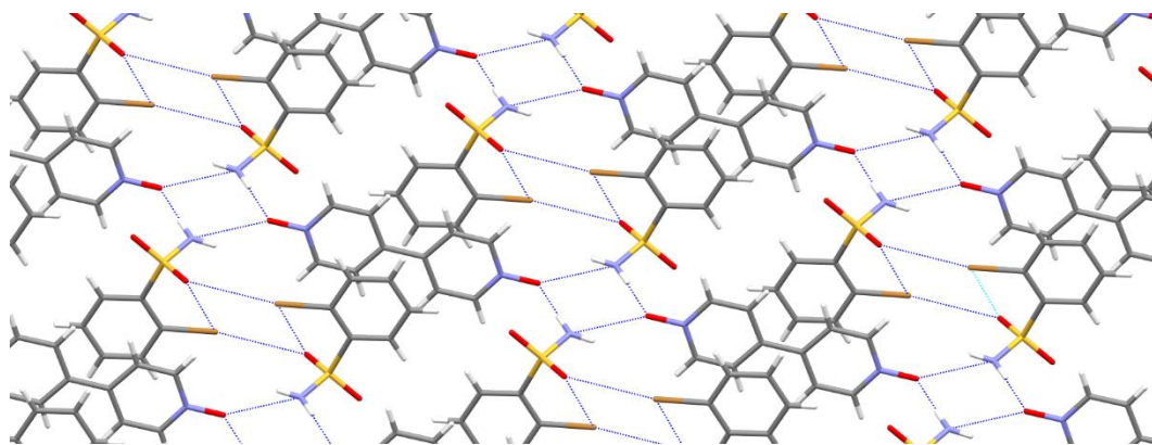
Figure 1.25: 2BrBSA-4,4-Bipyridine- N -oxide cocrystal as reported by Nangia . 60 2BrBSA and BPNO molecules form a two-dimensional array of tetrameric ring motif R_2^4(8) of N-H and O-N_{\text{oxide}} hydrogen bonds.
