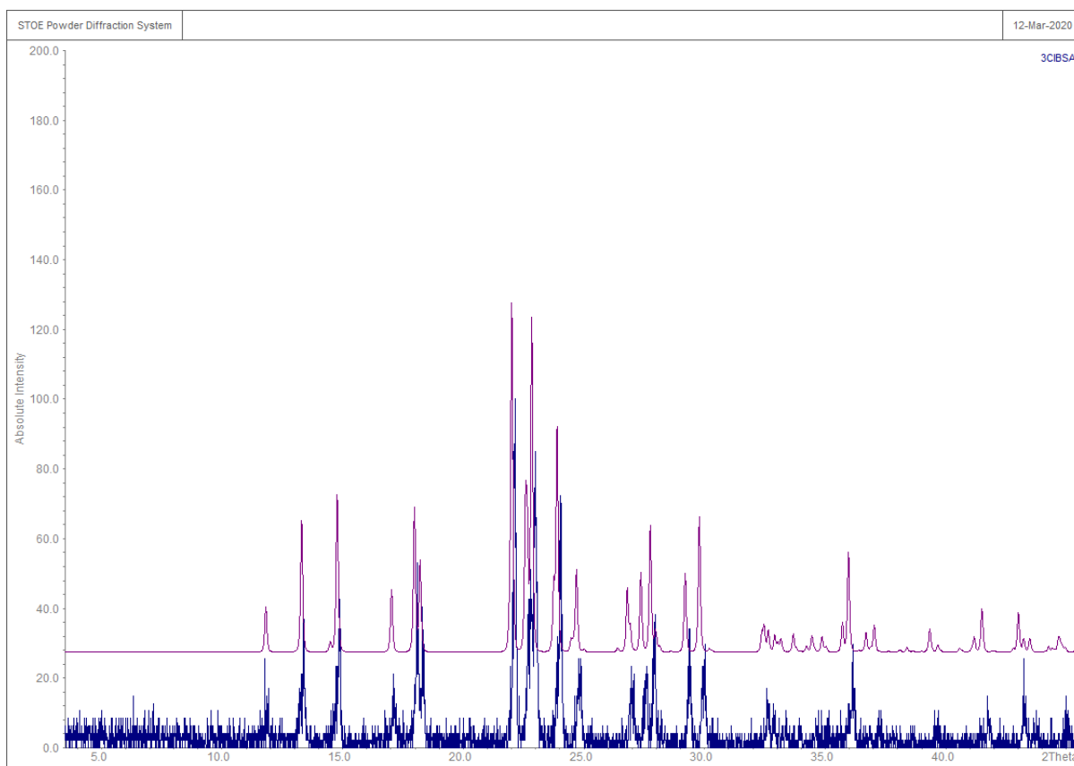
Figure S42: Experimental (blue) and theoretical (purple) PXRD data of 21 .
