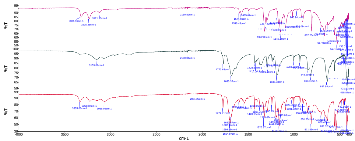
Figure S5: Stacked IR comparison of 4-MeBSA-SNI (1:1) cocrystal. (top – bottom, sulfonamide, succinimide, cocrystal).
