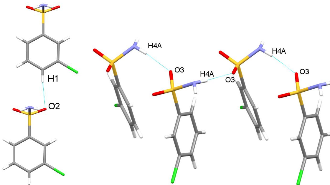
Figure S46: Hydrogen bonding in 21 .
