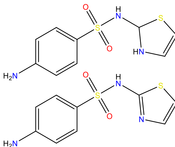
Figure 1.7: Two tautomers of sulfathiazole: top is the imino tautomer and bottom is the amino tautomer, adapted from reference 23.
