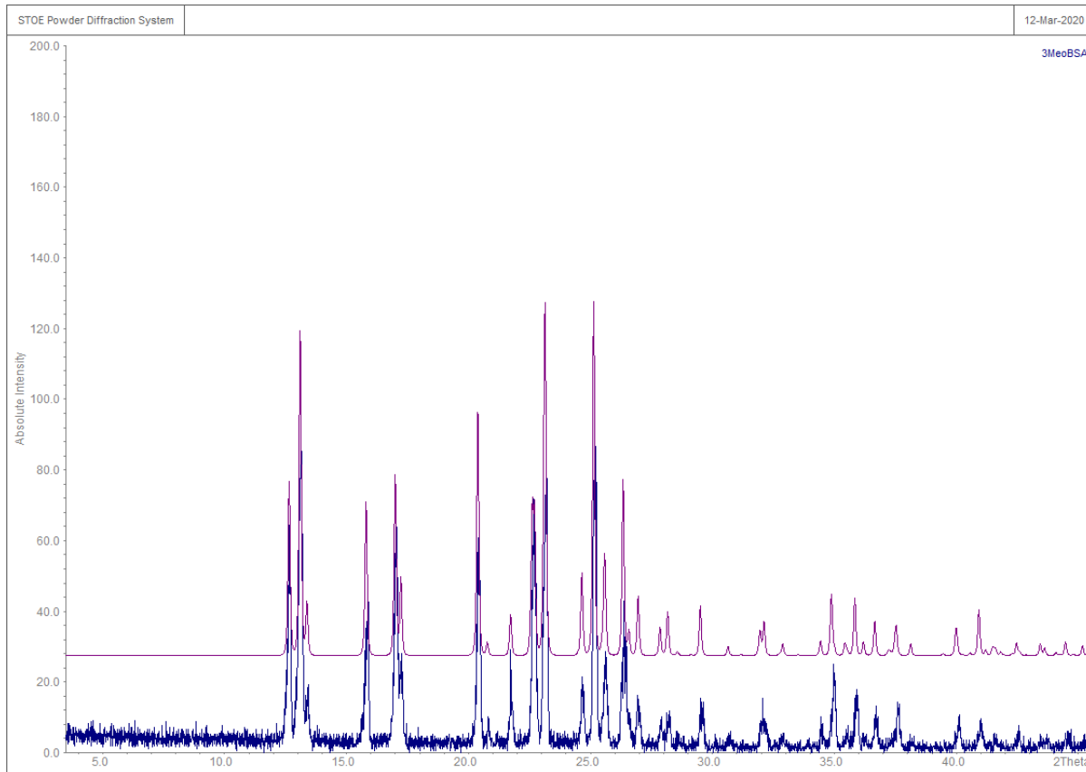
Figure S1: Experimental (blue) and theoretical (purple) PXRD data of 2 .
