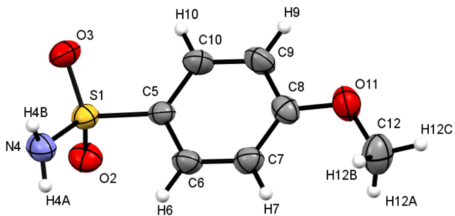
Figure S9: ORTEP diagram of 3 , with numbering scheme. Thermal ellipsoids are drawn at the 50% level.
