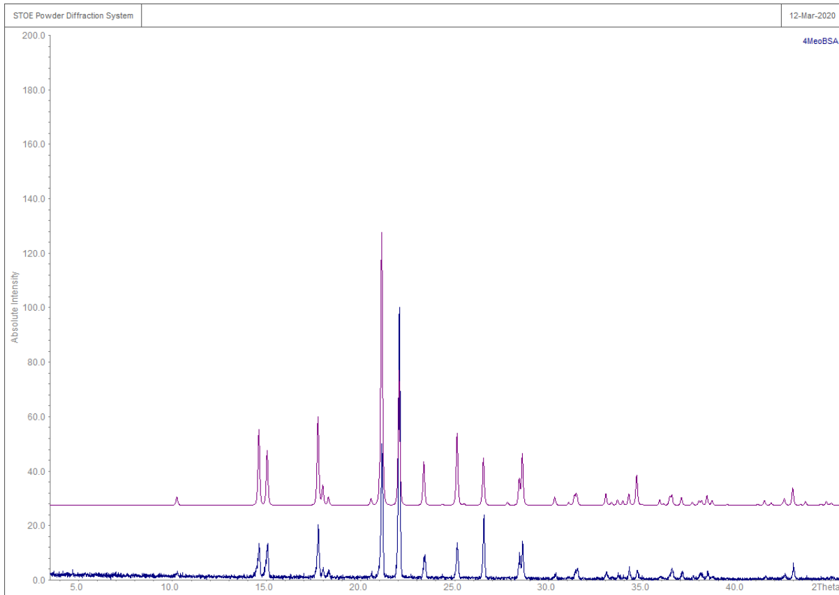
Figure S7: Experimental (blue) and theoretical (purple) PXRD data of 3 .
