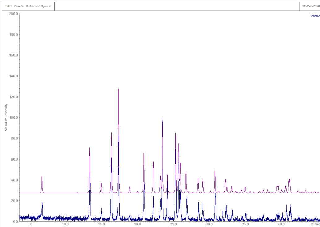
Figure S30: Experimental (blue) and theoretical (purple) PXRD data of 17 .
