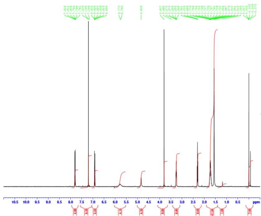
Figure S13: 1 H NMR of 4-OMeBSA-VLM cocrystal.
