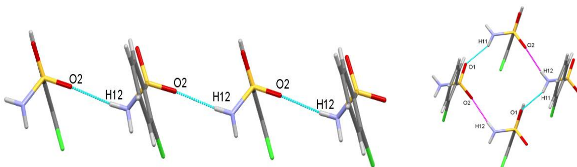
Figure S54: Hydrogen bonding in 11 . The blue and pink hydrogen bonding indicates the individual C(4) hydrogen bonding at the unitary level. The C(4) chains are related by the c glide plane and the C centering. 5
