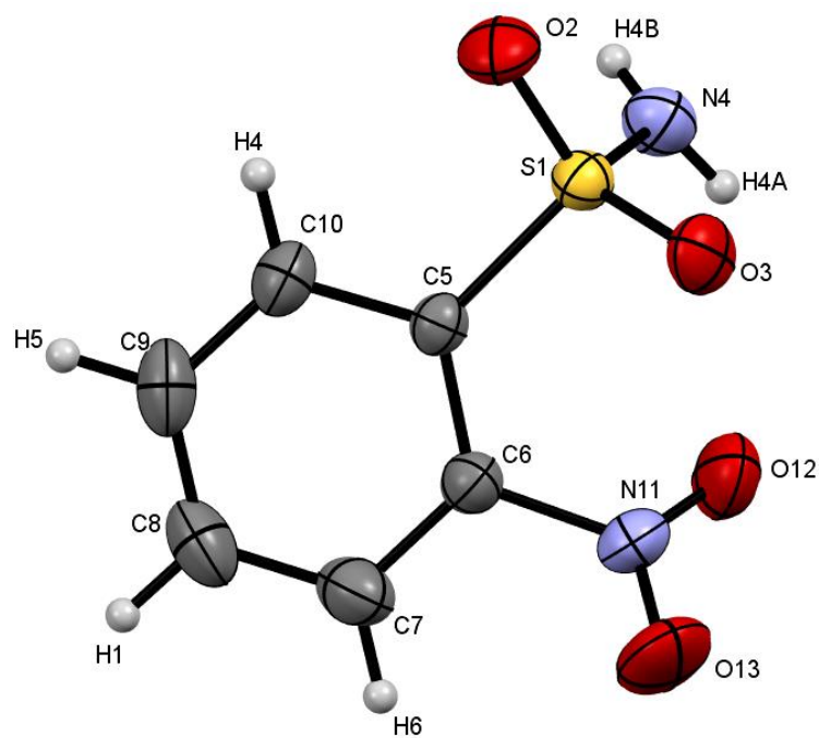
Figure S33: ORTEP diagram of 17 , with numbering scheme. Thermal ellipsoids are drawn at the 50% level.
