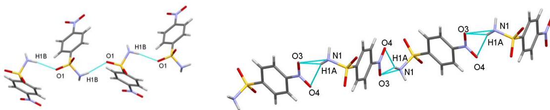
Figure S48: Hydrogen bonding in 1 . The blue hydrogen bonding indicates the C(4) hydrogen bonding at the unitary level. The C(4) chains are related by the 2_1 -fold screw axis along the b-axis and a glide plane perpendicular to the b-axis. 1
