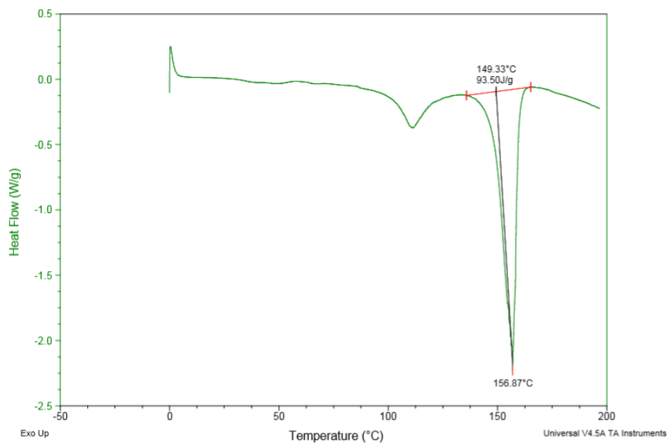
Figure S20: DSC spectra of 7.
