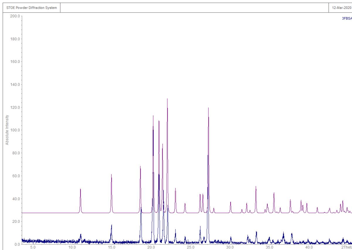
Figure S18: Experimental (blue) and theoretical (purple) PXRd data of 7 .
