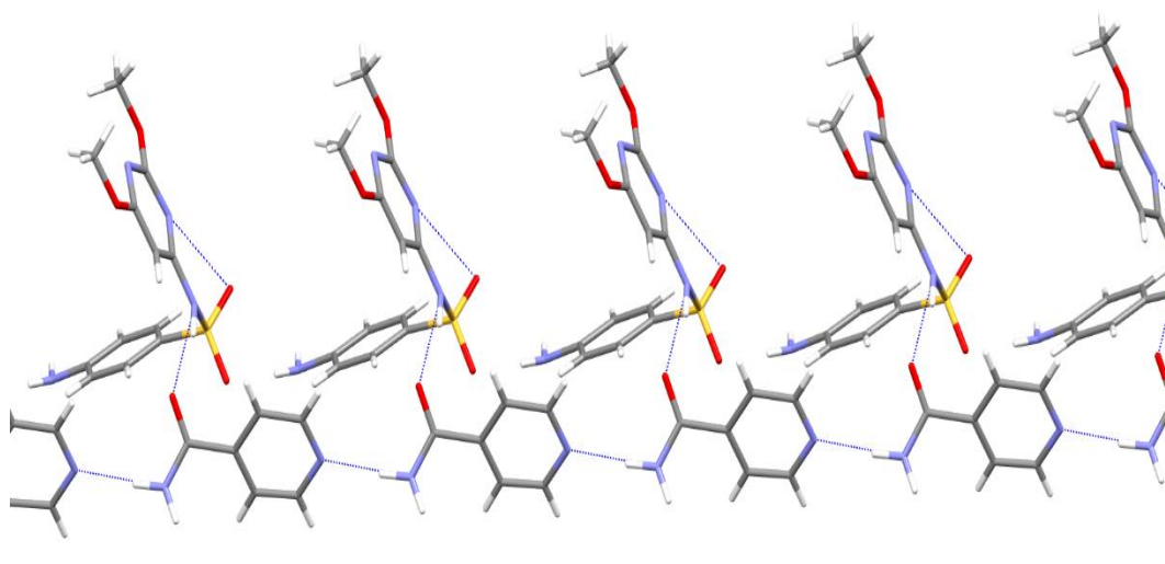
Figure 1.21: Sulfadimethoxine-Isonicotinamide cocrystal displaying N-H sulfonamide (SDM)···O(INA) (blue), and N-H amide (INA)···N terminal amine (SDM) interactions. 54
