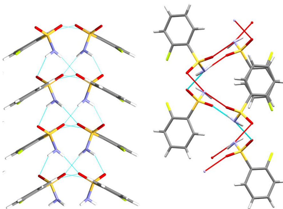
Figure S17: Packing diagrams of 6 showing the zig-zag arrangement formed by the tetramers. View along the b -axis, right.
