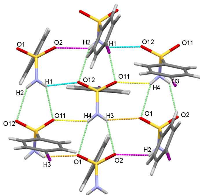
Figure S56: Hydrogen bonding in 13 . The blue, yellow, orange and pink hydrogen bonding indicates the individual C(4) hydrogen bonding at the unitary level and the green hydrogen bonding indicates the R_2^2(6) hydrogen bonding at the binary level. The C(4) chains are related by a glide plane perpendicular to the b-axis. 4
