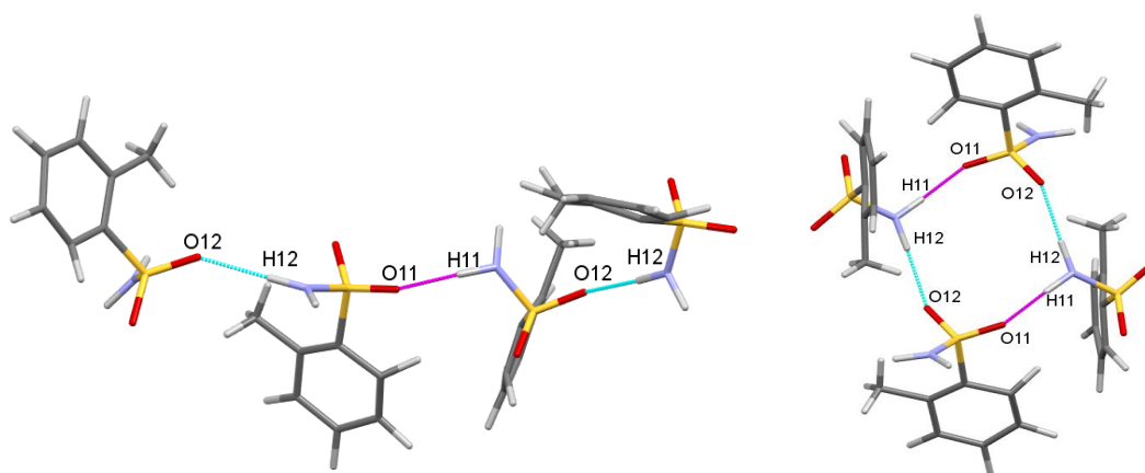
Figure S57: Hydrogen bonding in 14 . The blue and pink hydrogen bonding indicates the individual C(4) hydrogen bonding at the unitary level. The C(4) chains are related by the 4_1 -fold screw axis along the c-axis and a glide plane perpendicular to the c-axis. There is also a 2_{1\text{-rotation}} axis and a 2_1 rotoinversion axis along the c-axis. 6
