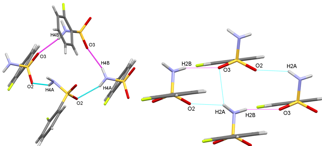
Figure 2.4: The R_4^4(14) motif observed for 6 , left, and 7 , right.
