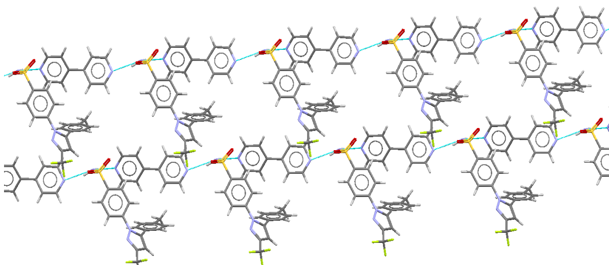
Figure 1.26: Binary cocrystal of celecoxib and bipyridine. 61
