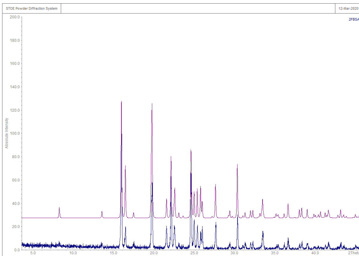
Figure S12: Experimental (blue) and theoretical (purple) PXRd data of 6 .
