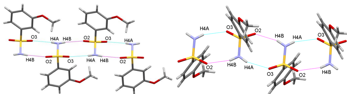
Figure 2.3. The binary level R_2^2(8) chain observed in 2 , left, and 3 , right. The blue and pink colors indicate the unitary level N-H \cdots O=S C(4) hydrogen bonded chains.
