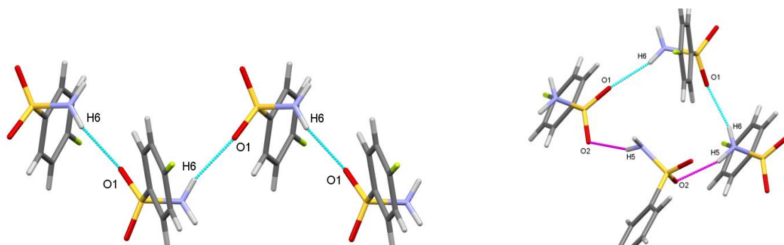
Figure S55: Hydrogen bonding in 12 . The blue and pink hydrogen bonding indicates the individual C(4) hydrogen bonding at the unitary level. The C(4) chains are related by the 2_1 -screw axis and the n glide plane. 4
