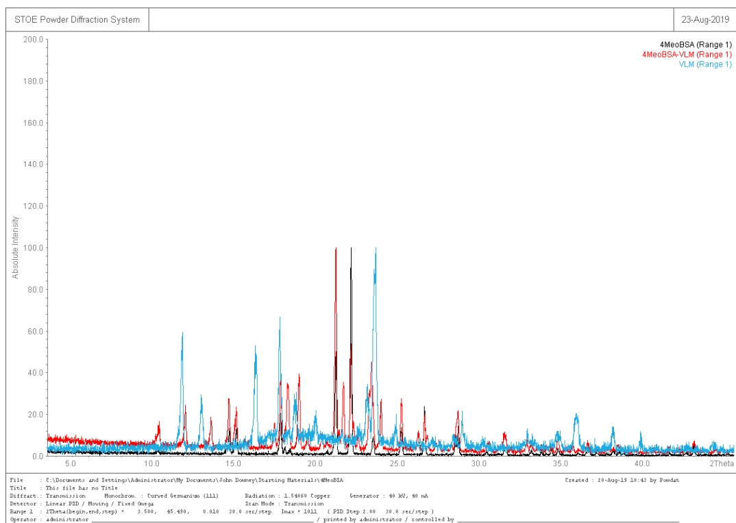
Figure S2: Overlay PXRD comparison of 4-OMeBSA—VLM cocrystal.
