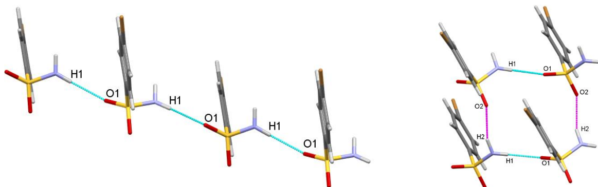
Figure S53: Hydrogen bonding in 10 . The blue and pink hydrogen bonding indicates the individual C(4) hydrogen bonding at the unitary level. The C(4) chains are related by the 2_1 -screw axis and the n glide plane. 4
