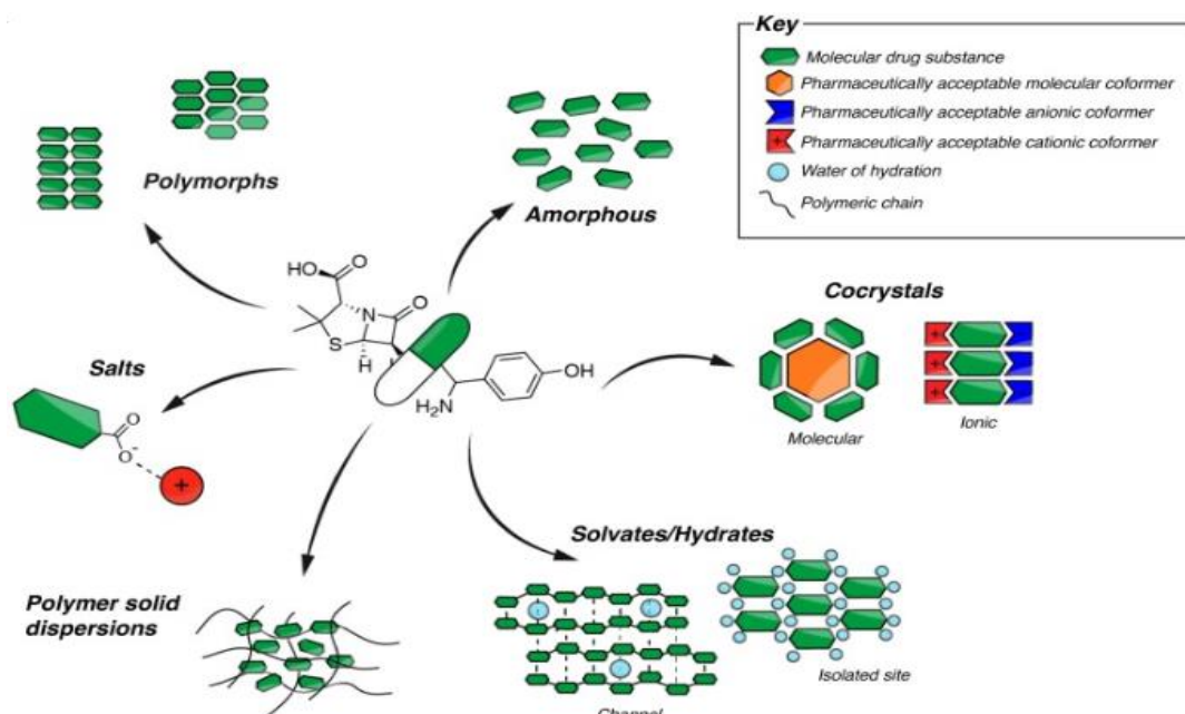
Figure 1.8: Profile of various pharmaceutical crystalline solid-state materials. 39
