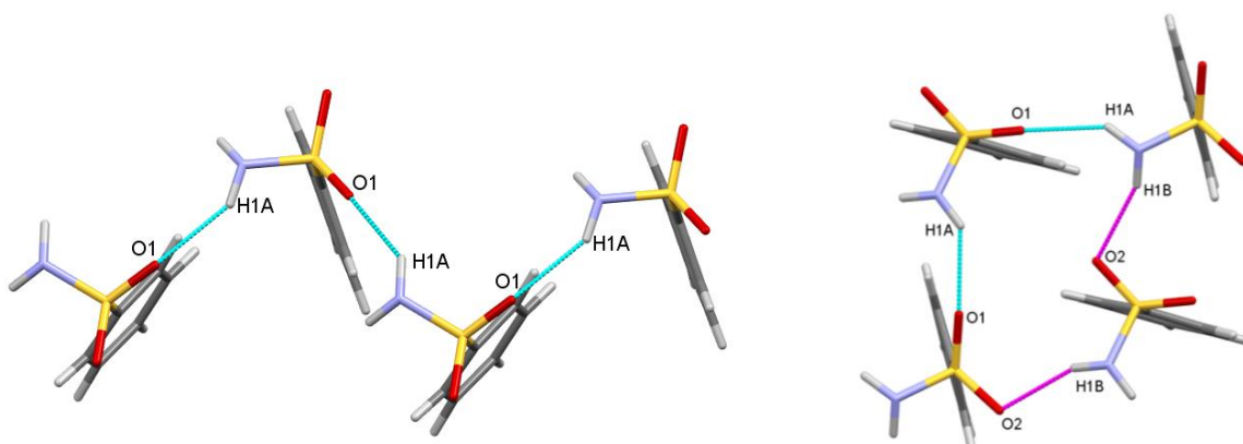
Figure S50: Hydrogen bonding in 5 . The blue and pink hydrogen bonding indicates the individual C(4) hydrogen bonding at the unitary level. The C(4) chains are related by the c -glide plane. 3
