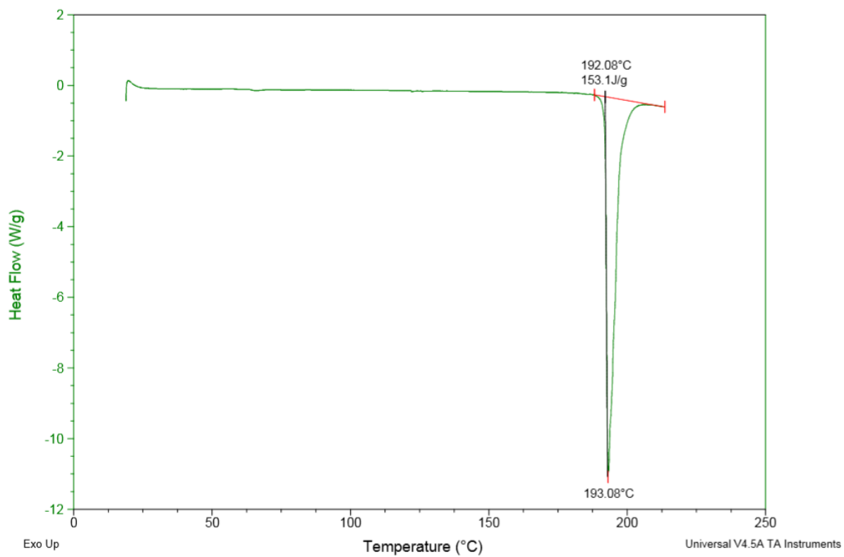
Figure S26: DSC spectra of 9 .
