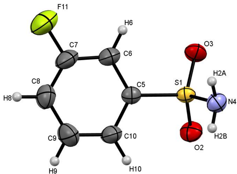
Figure S21: ORTEP diagram of 7, with numbering scheme. Thermal ellipsoids are drawn at the 50% level.
