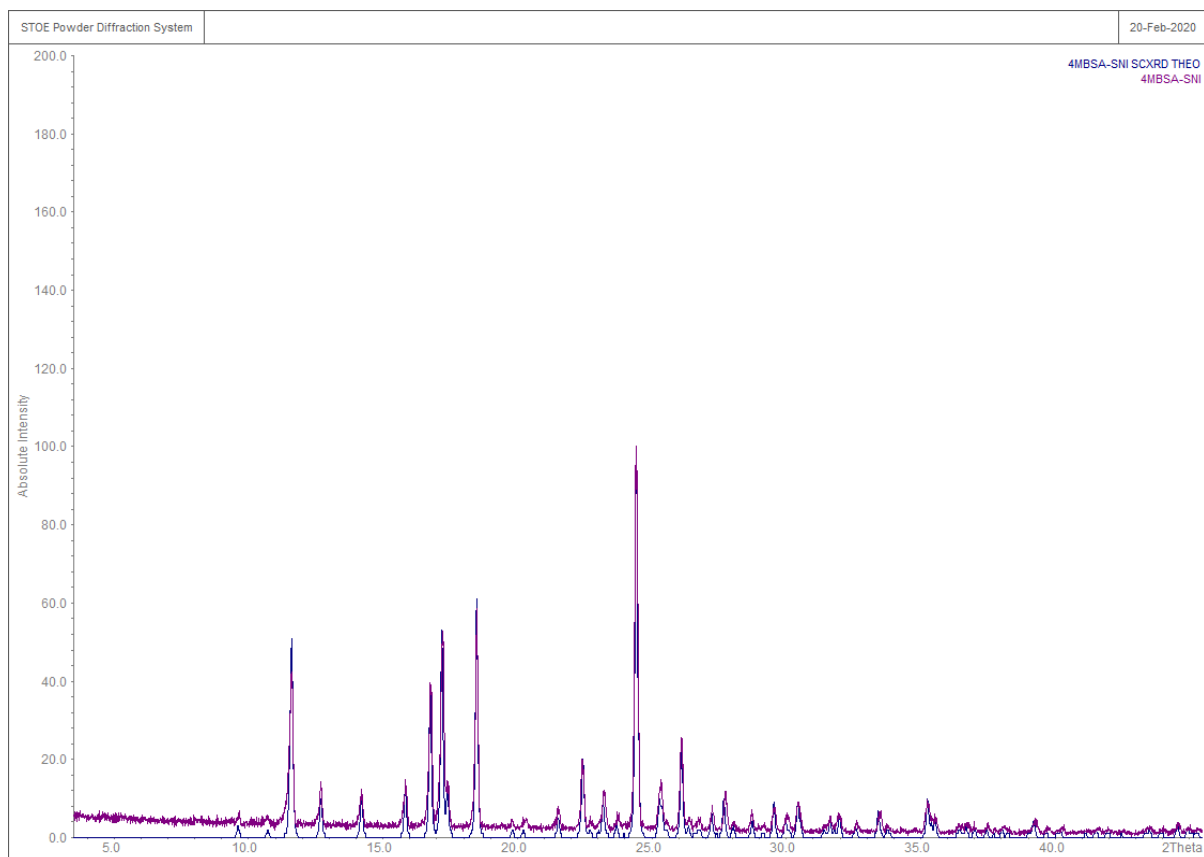
Figure S4: Overlay PXRD comparison of 4-MeBSA-SNI (1:1) cocrystal of powder pattern (purple) with the calculated pattern of the crystal structure (blue).
