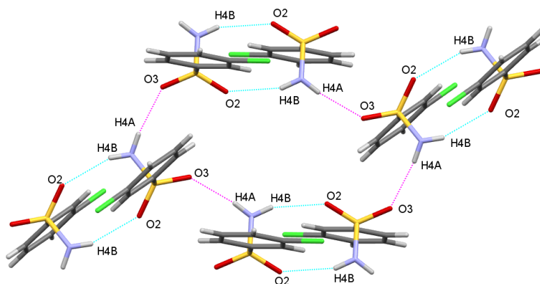
Figure 2.7: The R_2^2(8) dimer and R_6^6(20) hexamer rings present in the 2-D hydrogen bonded sheets in 20 and 21 .
