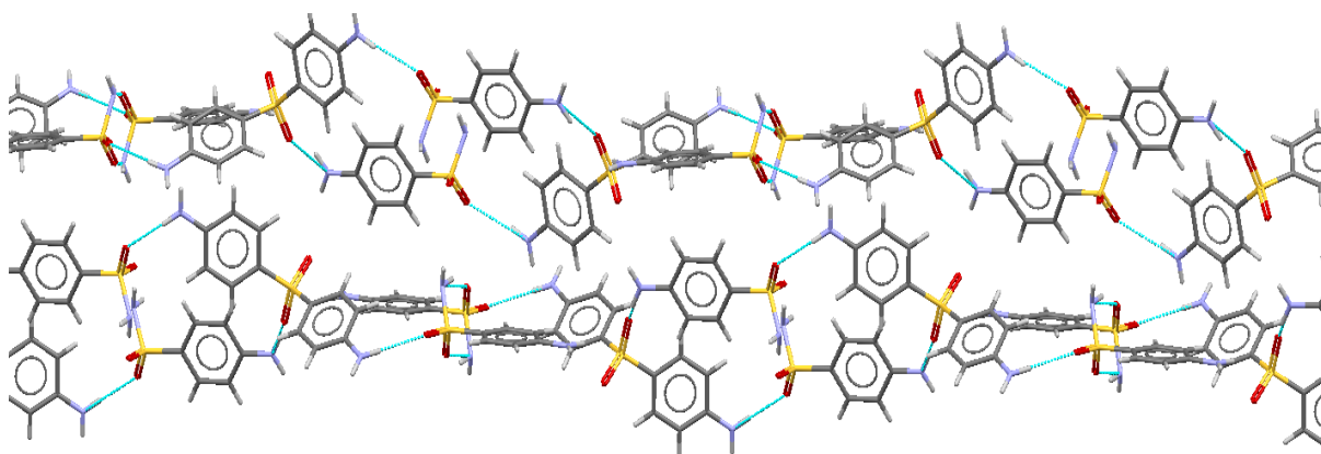
Figure 1.27: DAP and SUL were crystallized in 1:2 stoichiometry, and the single-crystal structure was solved and refined in the monoclinic system with the C2/c space group and one DAP and two SNA molecules in the asymmetric unit. 63
