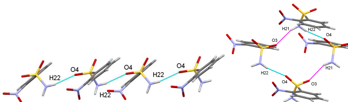
Figure S60: Hydrogen bonding in 17 (TIBPAW) . The blue and pink hydrogen bonding indicates the individual C(4) hydrogen bonding at the unitary level. The C(4) chains are related by the glide plane perpendicular to the b-axis. 9
