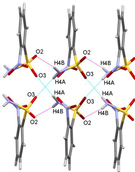
Figure 2.6: The six molecules forming two R_4^4(14) tetramers in 17 .
