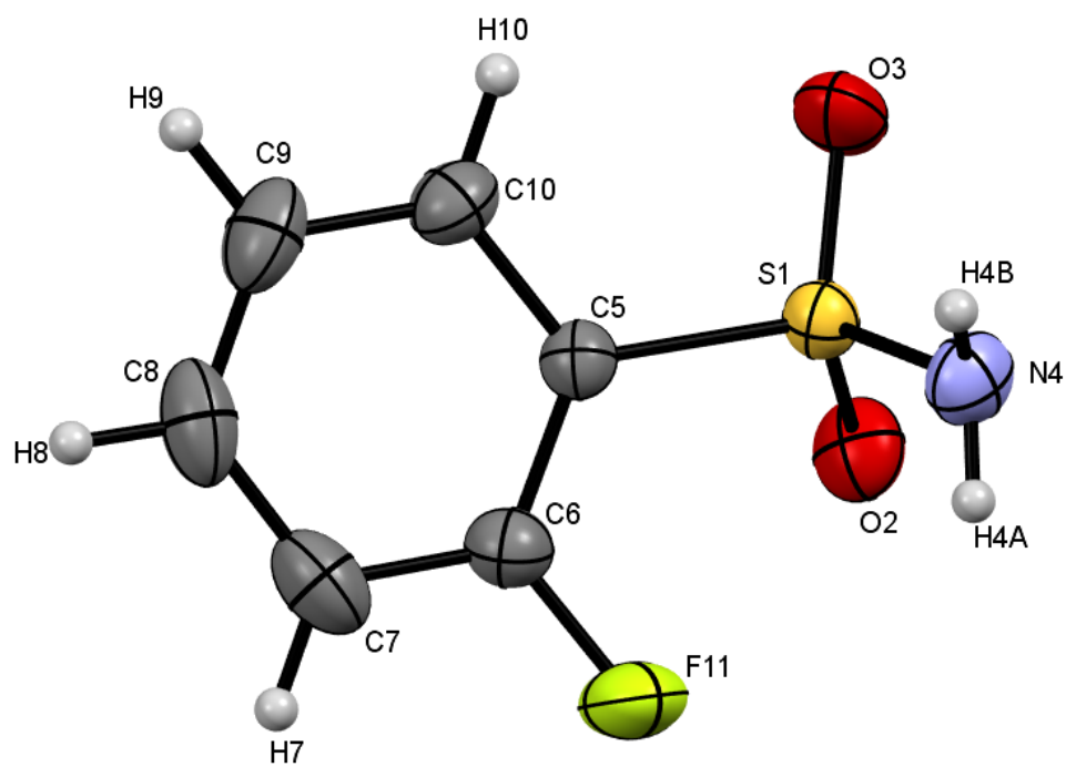
Figure S15: ORTEP diagram of 6 , with numbering scheme. Thermal ellipsoids are drawn at the 50% level.
