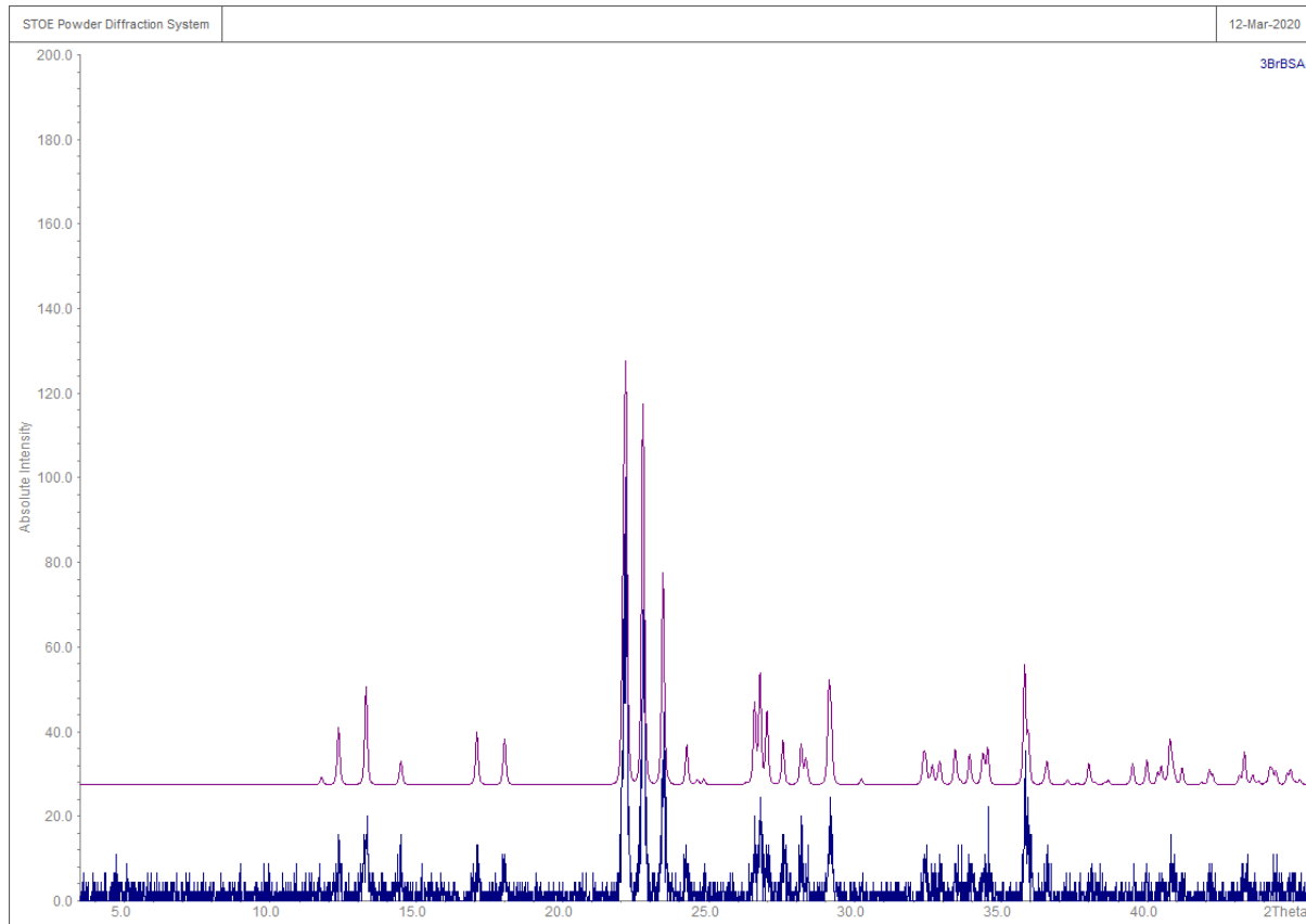
Figure S36: Experimental (blue) and theoretical (purple) PXRD data of 20 .
