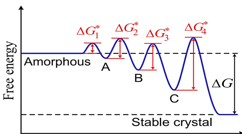
Figure 1.5: Diagrammatic representation of Ostwald's rule. 18
