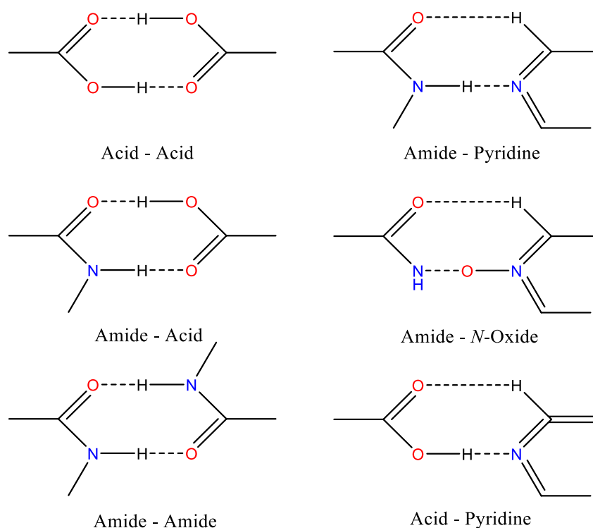
Figure 1.3: Some examples of homosynthons and heterosynthons where the dashed lines denote the hydrogen bond and the blue/red atoms are the hydrogen bonds donor/acceptor, adapted from reference 11.
