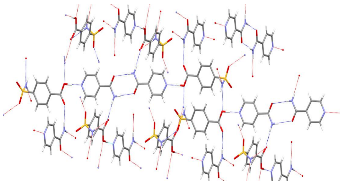
Figure 1.20: Crystal structure of 4-sulfamoylbenzenesulfonamide (3SMBA)-Isonicotinamide (INA) was solved in the monoclinic C2/c crystals system. 53
