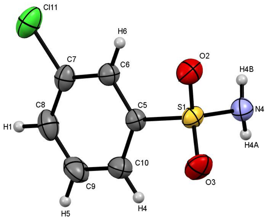
Figure S45: ORTEP diagram of 21 , with numbering scheme. Thermal ellipsoids are drawn at the 50% level.
