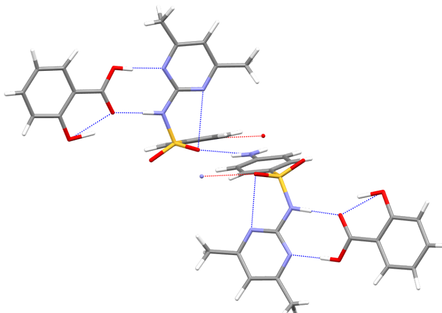
Figure 1.24: Sulfamethazine-Salicylic Acid cocrystal. 58
