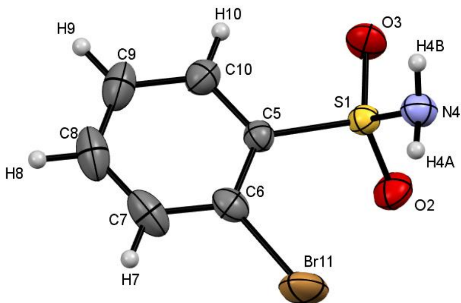
Figure S27: ORTEP diagram of 9 , with numbering scheme. Thermal ellipsoids are drawn at the 50% level.
