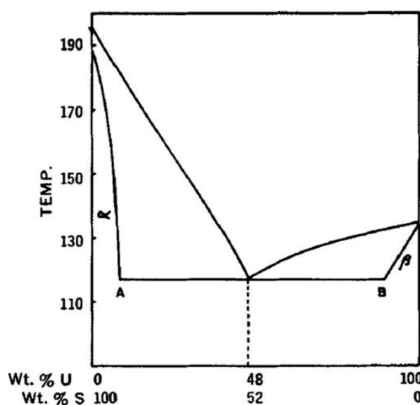
Figure 1.10: Phase diagram of sulfathiazole-urea eutectic composition. 45
