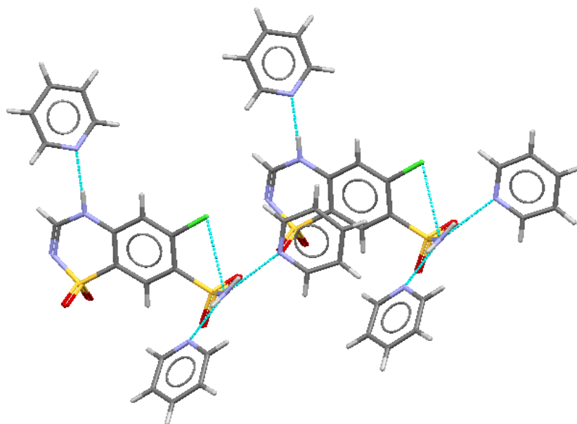
Figure 1.13: The crystal packing in chlorothiazide-pyridine (1/3) solvate. 47
