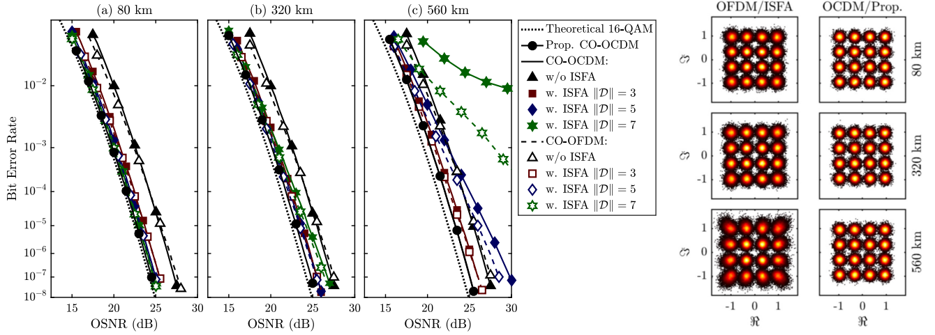
Fig. 7. Left: BER performance of the CO-OFDM systems with ISFA estimator and the CO-OCDDM systems with the proposed channel estimator with 16-QAM at (a) 80 km, (b) 320 km and (c) 560 km. Right: the received constellation diagrams with a received OSNR = 20 dB.
