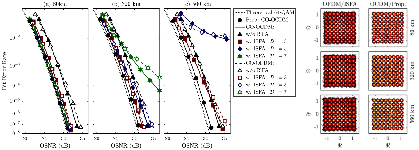
Fig. 8. Left: BER performance of the CO-OFDM systems with ISFA estimator and the CO-OCDDM systems with the proposed channel estimator with 64-QAM at (a) 80 km, (b) 320 km and (c) 560 km. Right: the received constellation diagrams with a received OSNR = 26 dB.
