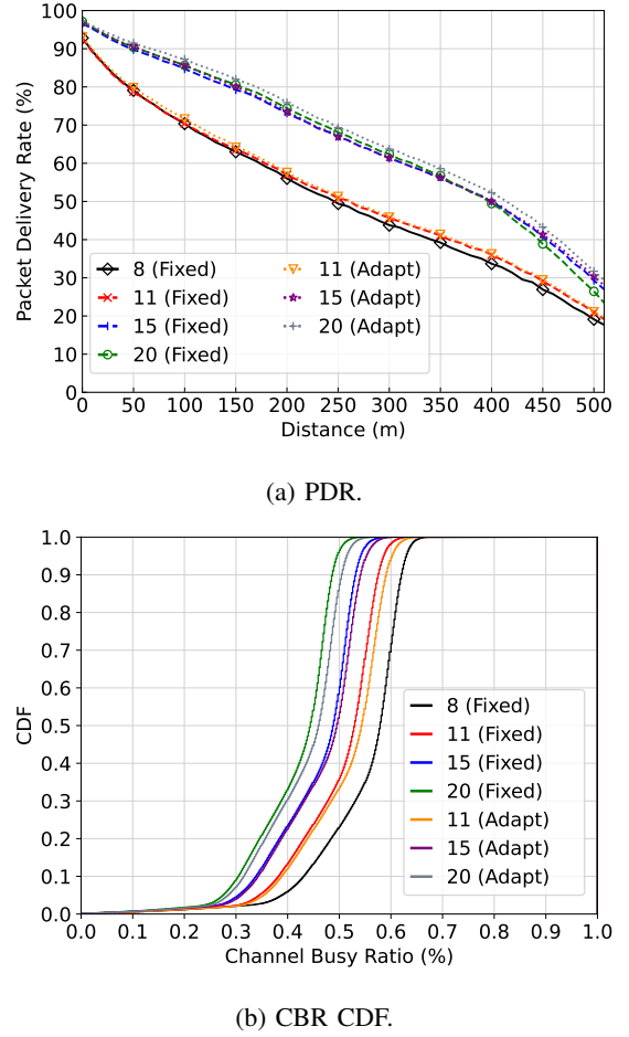
Fig. 5: Performance considering the Renault packet size distribution.
