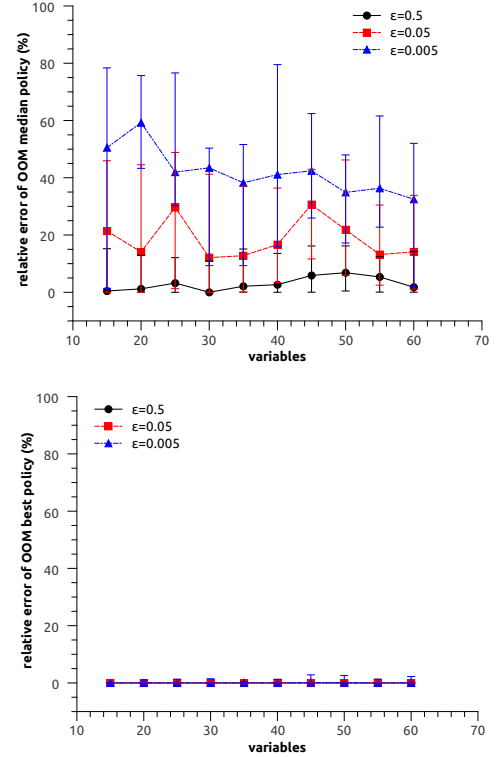
Figure 3: Results for class P influence diagrams. We show the distribution of the relative errors \eta_{med} (top) and \eta_{max} (bottom) for \epsilon \in \{0.5, 0.05, 0.005\} . # of samples s = 100 .
