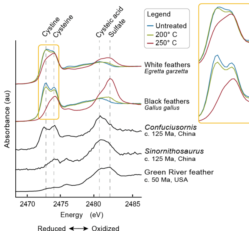
Fig. 5.1 Sulfur-XANES spectra for fossil feathers and untreated and experimentally degraded white ( Egretta garzetta ) and black ( Gallus gallus ) feathers.
