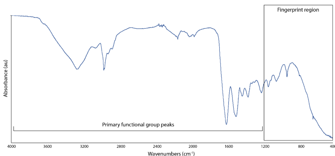
Fig. 2.5 Unprocessed FTIR spectrum of a feather sample showing the two primary spectral regions.
