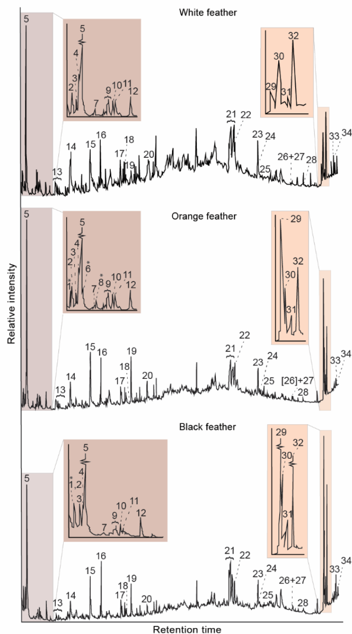
Fig. 6.3 Py-GC-MS pyrograms of black and orange ( Gallus gallus ) and white ( Egretta garzetta ) feathers degraded in sulfurization experiments.
