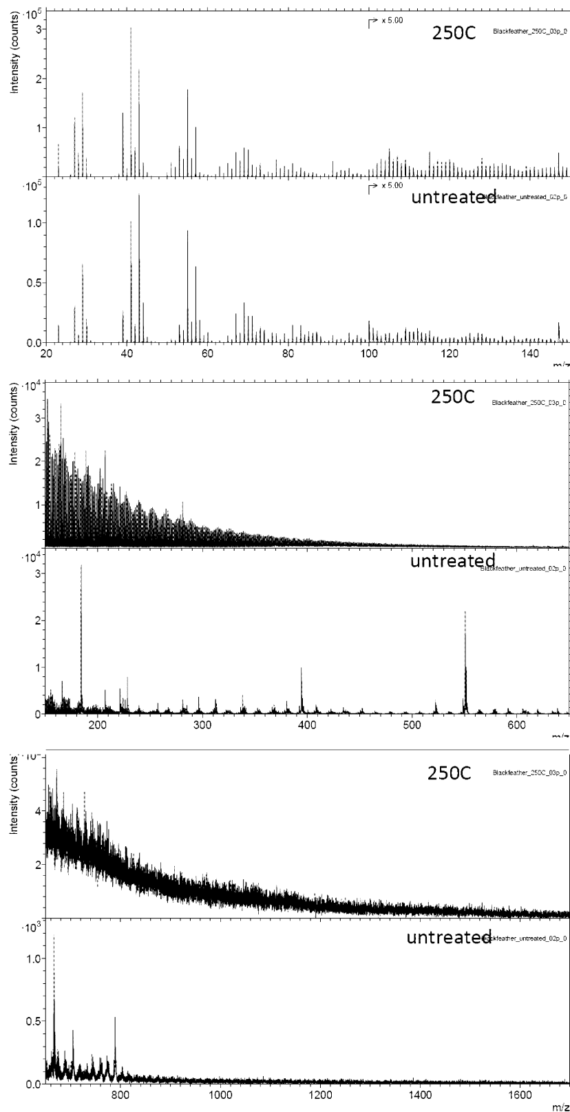
Fig. S4.4 (part 8) Positive ion ToF-SIMS spectra from melanin extracts of untreated and strongly matured black feathers from Gallus gallus . Matured feathers treated at 250°C for 1 h.
