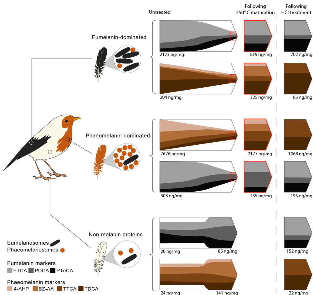
Fig. 4.5 Authentic chemical signals for fossil melanins. Schematic showing chemical degradation of eumelanin and phaeomelanin during fossilisation based on AHPO-HPLC analysis of experimentally matured black and orange ( Gallus gallus ) and white ( Egretta garzetta ) feathers. Dashed line separates data with and without HCl treatment. The long horizontal arrows illustrate the relative concentrations of melanin markers before treatment and after maturation at 250°C without HCl treatment. The short horizontal arrows (on the right) depict the relative concentrations of markers following maturation at 250°C with HCl treatment. Concentration values (in ng/mg) indicate absolute concentrations of melanin markers.
