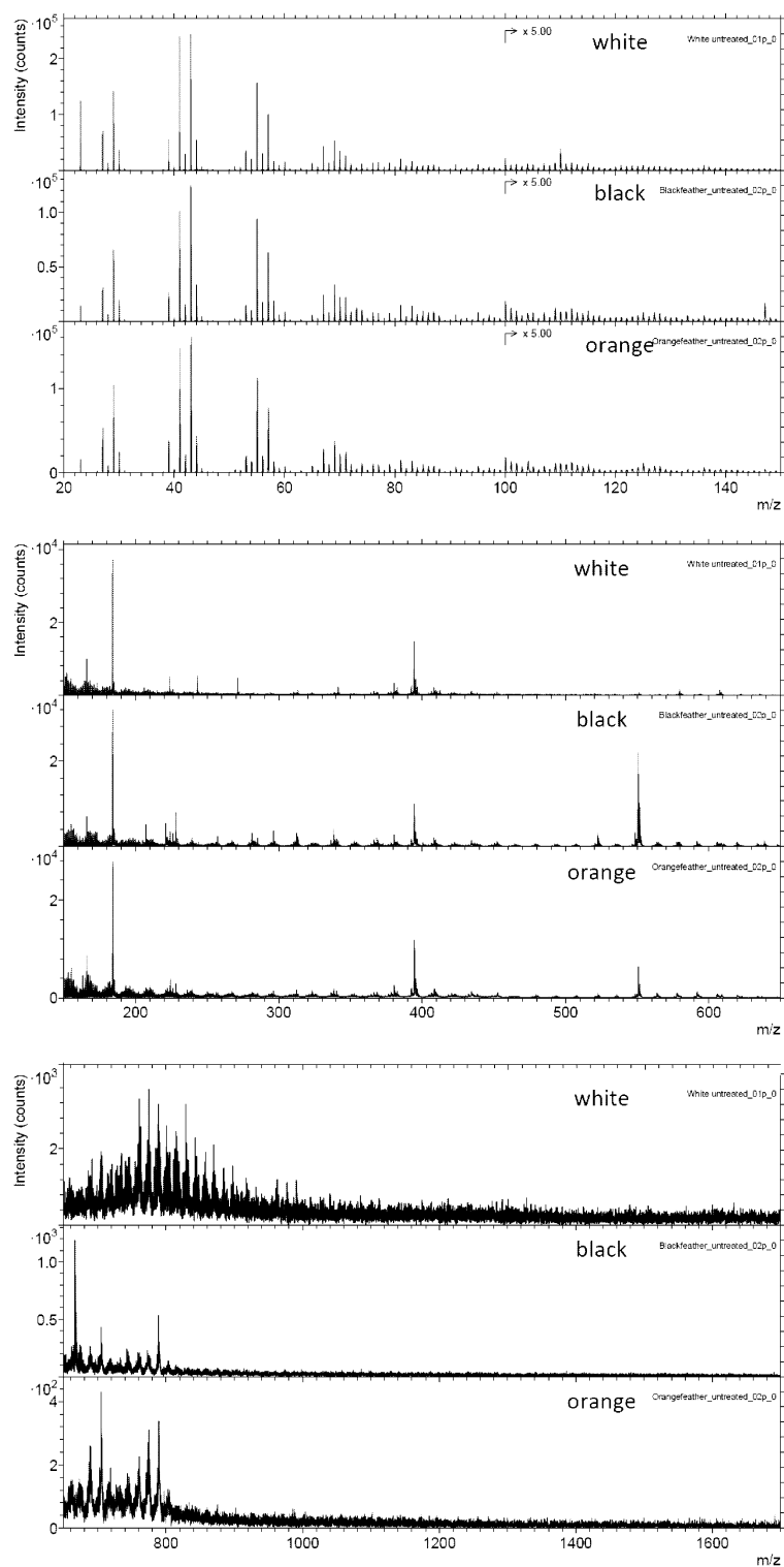
Fig. S4.4 (part 3) Positive ion ToF-SIMS spectra for untreated black, orange and white feathers from extant birds. Black and orange feathers are from the domestic chicken ( Gallus gallus ) and white feathers are from the little egret ( Egretta garzetta ).
