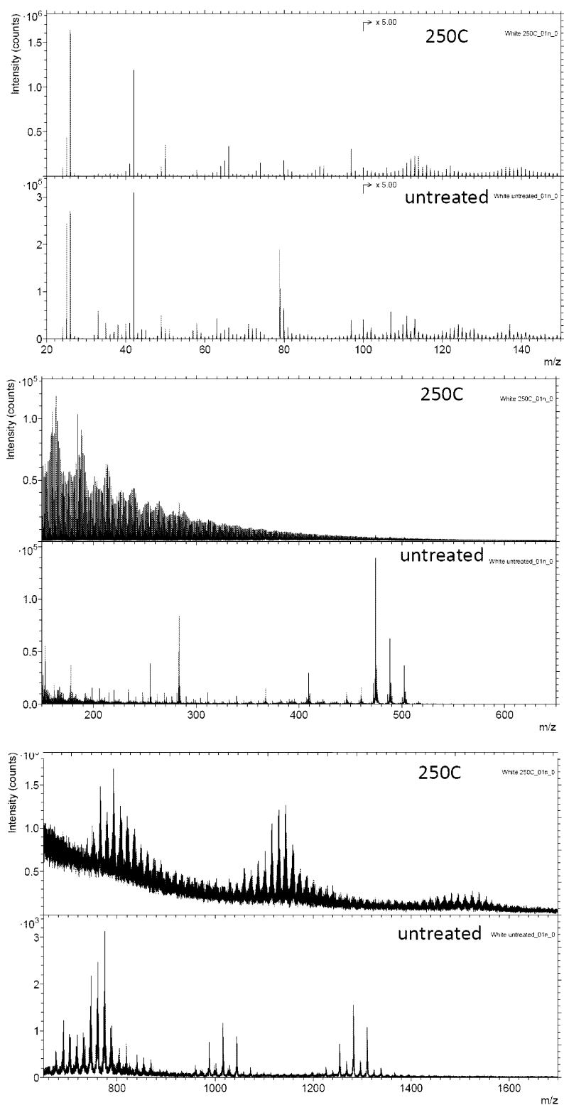
Fig. S4.4 (part 5) Negative ion ToF-SIMS spectra from melanin extracts of untreated and strongly matured white feathers from Egretta garzetta . Matured feathers treated at 250°C for 1 h.
