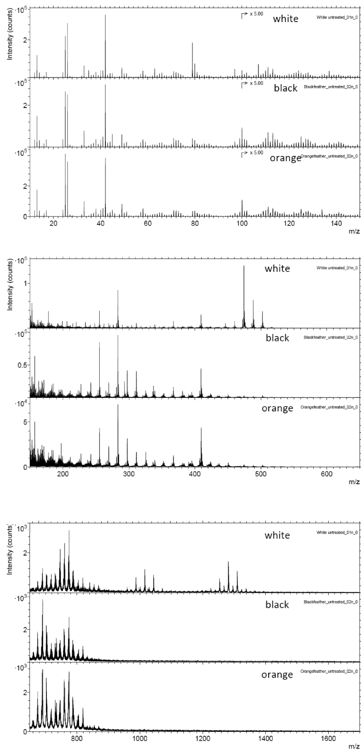
Fig. S4.4 (part 1) Negative ion ToF-SIMS spectra for untreated black, orange and white feathers from extant birds. Black and orange feathers are from the domestic chicken ( Gallus gallus ) and white feathers are from the little egret ( Egretta garzetta ).
