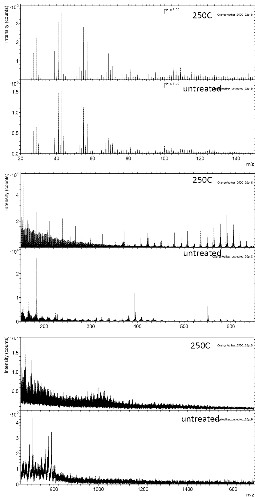
Fig. S4.4 (part 10) Positive ion ToF-SIMS spectra from melanin extracts of untreated and strongly matured orange feathers from Gallus gallus . Matured feathers treated at 250°C for 1 h.
