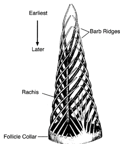
Fig. 1.3 A schematic illustration of a pennaceous feather in the early phase of its development. The distal end of the feather develops before the proximal end (from Prum and Brush, 2002).
