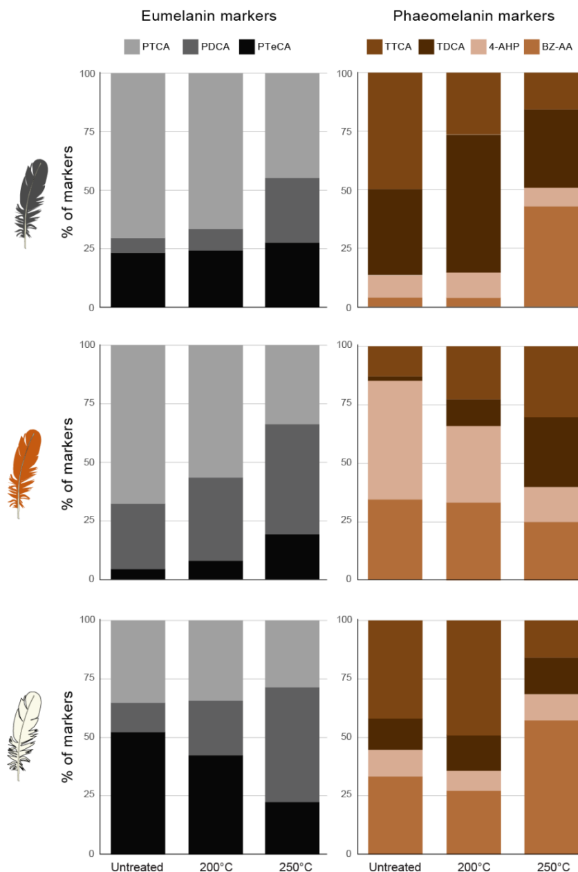
Fig. S4.3 AHPO- and HI-HPLC data for black, orange and white feathers from extant birds with and without thermal treatment. Eumelanin markers and the phaeomelanin markers TTCA and TDCA are derived during chemical degradation via AHPO. BZ-AA and 4-AHP are derived during HI hydrolysis. Black and orange feathers are from the domestic chicken ( Gallus gallus ) and white feathers are from the little egret ( Egretta garzetta ).
