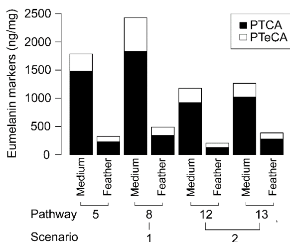
Fig. 3.6 AHPO analysis of Gallus gallus feathers and their experimental media. PTCA and PTeCA are eumelanin markers (PTeCA is a marker for diagenetically altered melanin).
