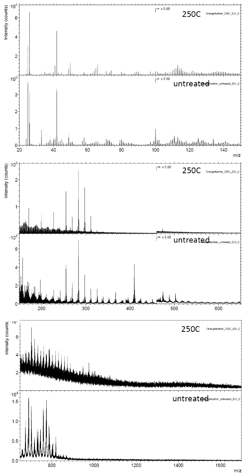
Fig. S4.4 (part 9) Negative ion ToF-SIMS spectra from melanin extracts of untreated and strongly matured orange feathers from Gallus gallus . Matured feathers treated at 250°C for 1 h.
