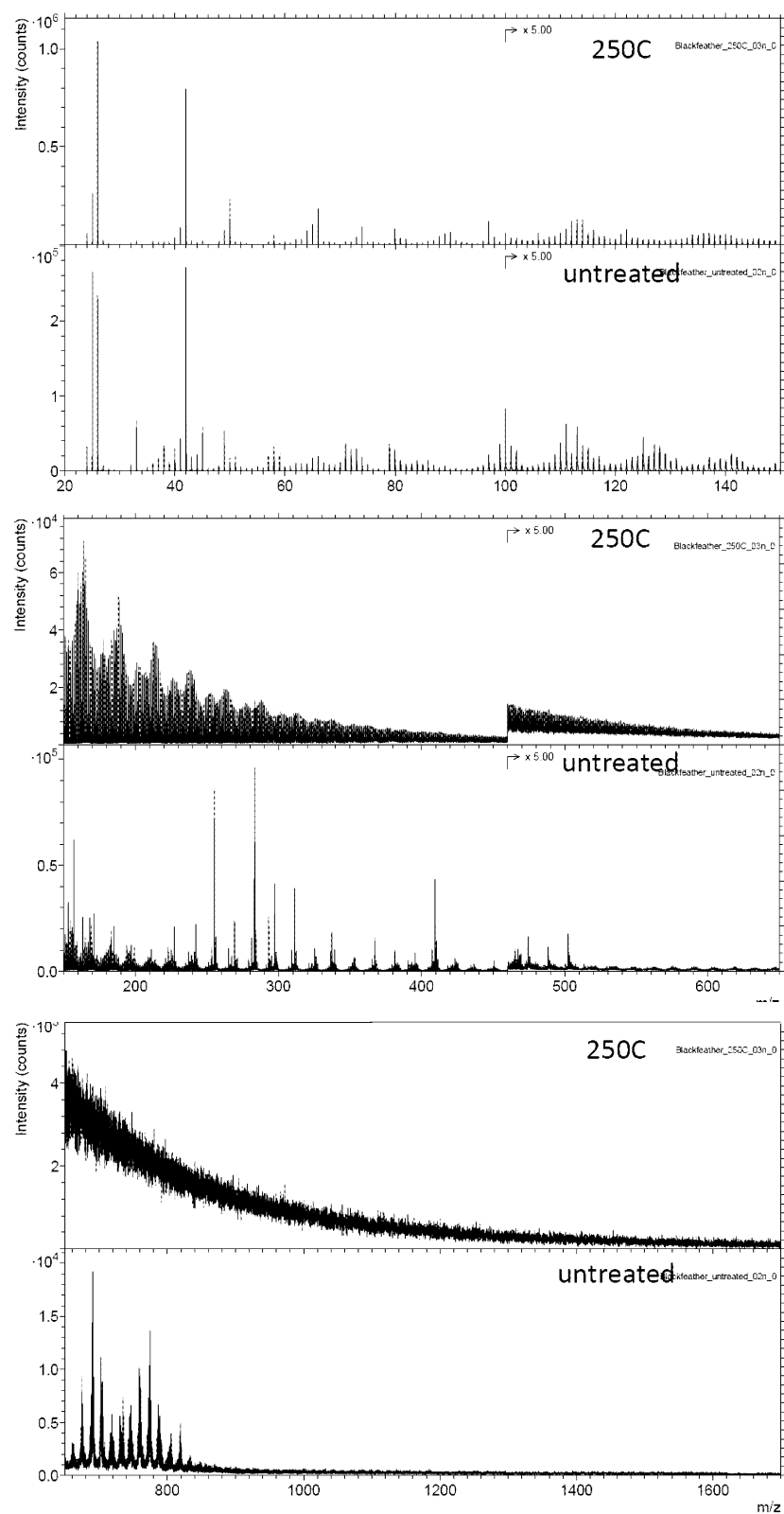
Fig. S4.4 (part 7) Negative ion ToF-SIMS spectra from melanin extracts of untreated and strongly matured black feathers from Gallus gallus . Matured feathers treated at 250°C for 1 h.
