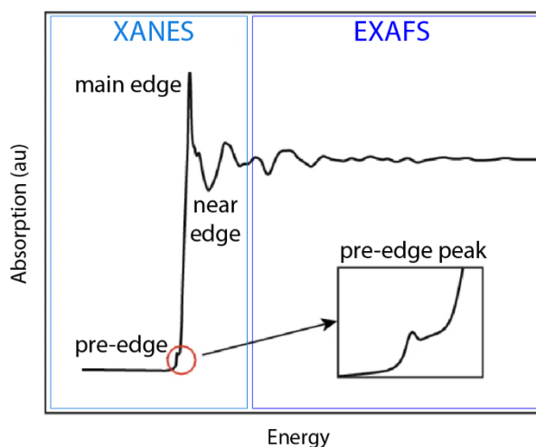
Fig. 2.4 X-ray absorption spectrum showing the primary features in a XANES spectrum and associated EXAFS region (modified from Wang et al. [2019]).
