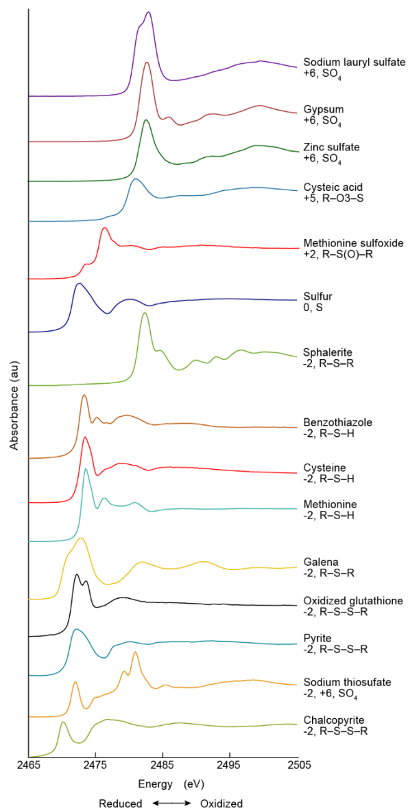
Fig. S5.4 Sulfur-XANES data for analytical standards for selected S-bearing compounds.
