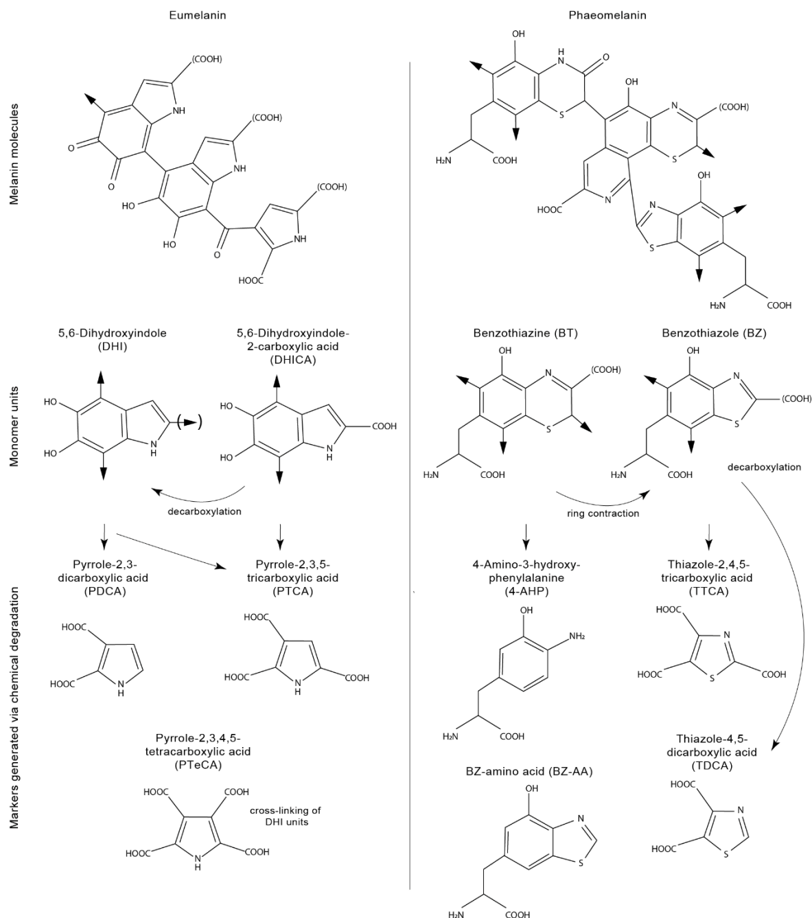
Fig. 4.1 Eumelanin and phaeomelanin molecules and their respective constituent monomers. Key eumelanin monomer units are DHI and DHICA; phaeomelanin monomer units are benzothiazine (BT) and benzothiazole (BZ). Chemical degradation of these units by alkaline hydrogen peroxide oxidation (AHPO) generates PDCA, PTCA, PTeCA, TTCA and TDCA markers. Hydroiodic acid (HI) hydrolysis generates 4-AHP (and 3-AHP, not shown here) and BZ-AA 33-35,39,40 .
