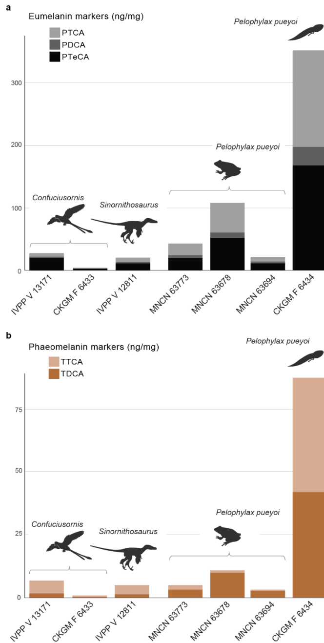
Fig. 4.4 HCl-AHPO-HPLC data for fossil melanins. Eumelanin (A) and phaeomelanin (B) marker concentrations in samples of melanosomes. Fossil feathers are from the early bird Confuciusornis and the feathered dinosaur Sinornithosaurus from the Jehol biota. Fossil frog samples are of internal melanosomes from Pelophylax pueyoi from the Libros biota.
