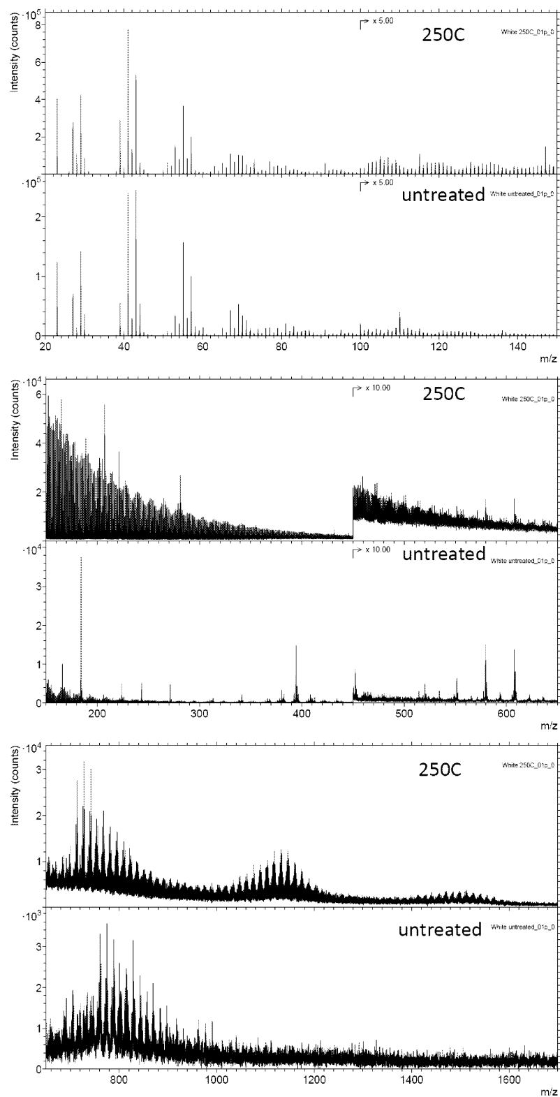
Fig. S4.4 (part 6) Positive ion ToF-SIMS spectra from melanin extracts of untreated and strongly matured white feathers from Egretta garzetta . Matured feathers treated at 250°C for 1 h.
