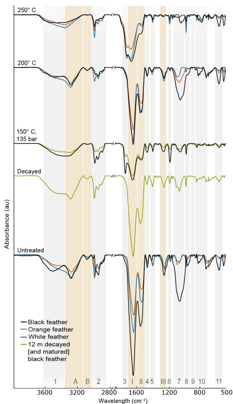
Fig. 6.4 FTIR spectra of experimentally degraded black and orange ( Gallus gallus ) and white ( Egretta garzetta ) feathers.
