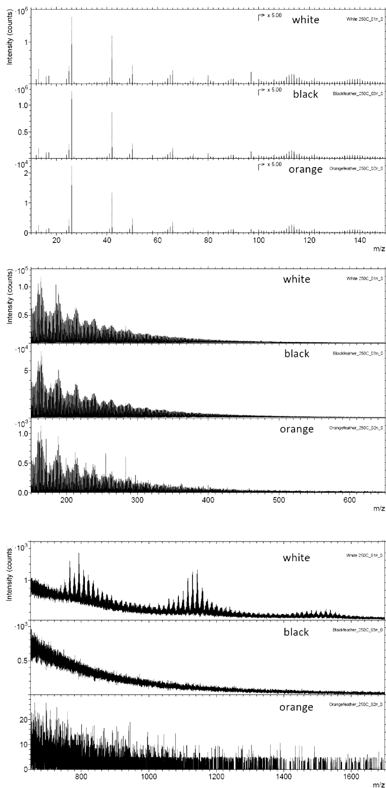
Fig. S4.4 (part 2) Negative ion ToF-SIMS spectra for black, orange and white feathers from extant birds matured at 250°C for 1 h. Black and orange feathers are from the domestic chicken ( Gallus gallus ) and white feathers are from the little egret ( Egretta garzetta ).
