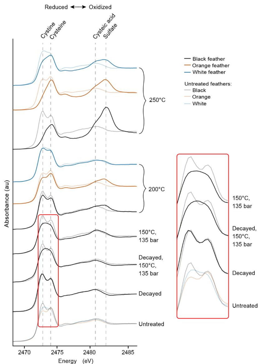
Fig. 6.1 S-XANES spectra of experimentally degraded black and orange ( Gallus gallus ) and white ( Egretta garzetta ) feathers.
