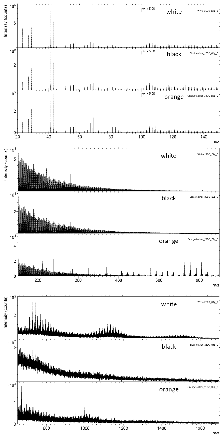
Fig. S4.4 (part 4) Positive ion ToF-SIMS spectra for black, orange and white feathers from extant birds matured at 250°C for 1 h. Black and orange feathers are from the domestic chicken ( Gallus gallus ) and white feathers are from the little egret ( Egretta garzetta ).
