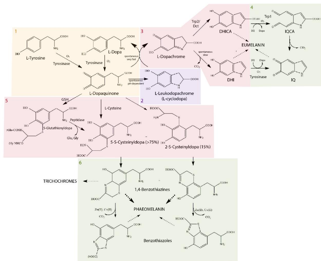
Fig. 1.7 Chemical pathways for the synthesis of eumelanin and phaeomelanin (modified from Galván and Solano [2016]).
