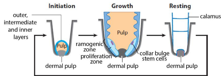
Fig. 1.5 Schematic illustration showing an adult feather follicle in the initiation, growth and rest phases of feather generation, collectively termed endysis (modified from Chen et al. [2015]).
