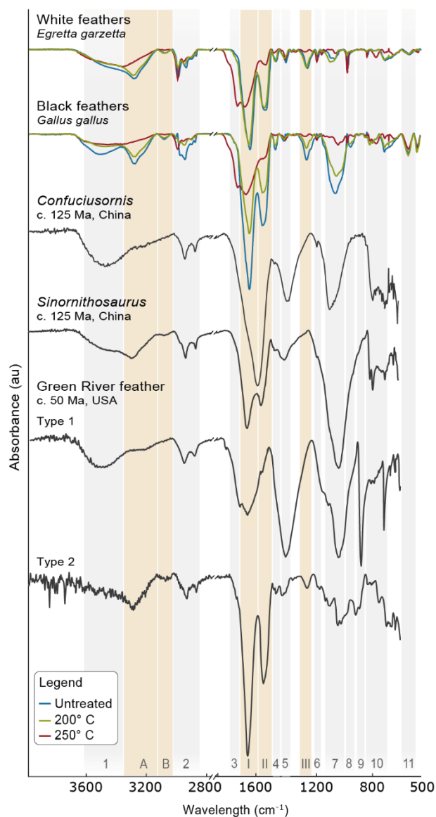
Fig. 5.2 FTIR spectra for fossil feathers and untreated and experimentally degraded white ( Egretta garzetta ) and black ( Gallus gallus ) feathers. Amide bands are indicated in brown boxes and all other bands in grey boxes.
