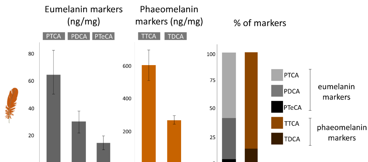
Fig. S4.8 HCl-AHPO-HPLC data for orange feathers from the common chicken ( Gallus gallus ) matured at 100°C. Melanin markers are derived during chemical degradation via HCl-AHPO. BZ and 4-AHP cannot be analysed following acid treatment.
