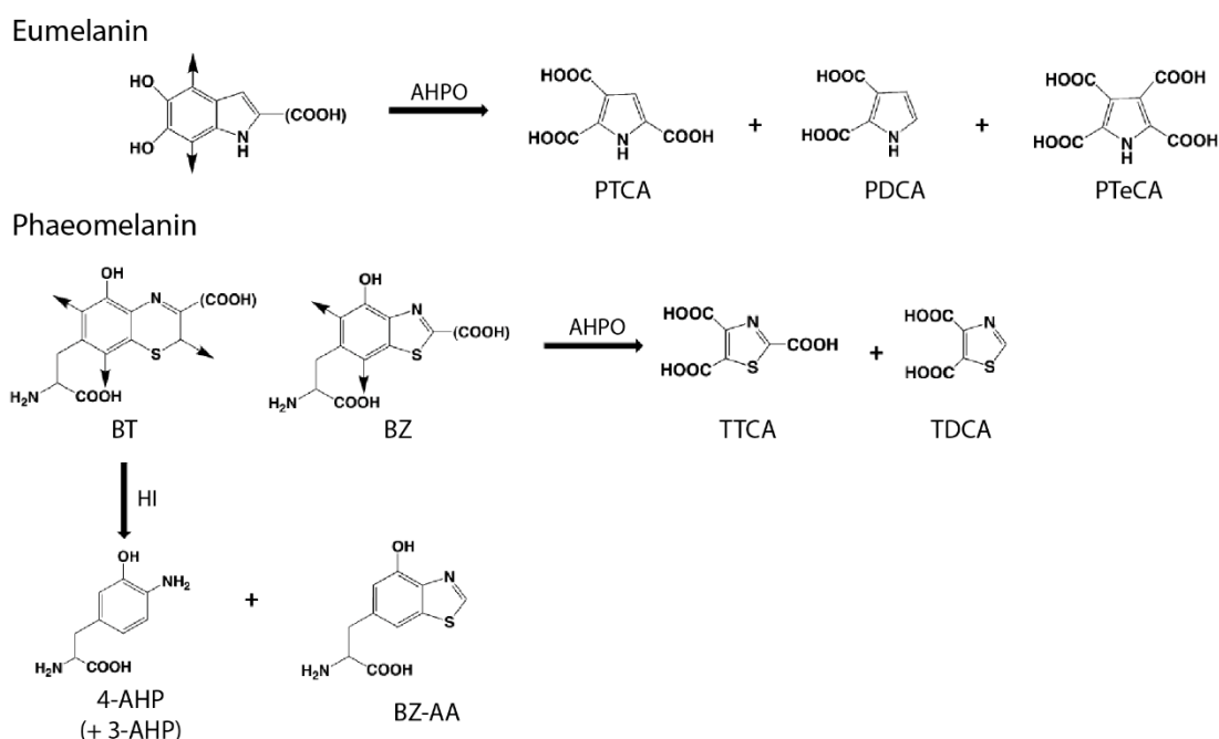
Fig. 2.2 Degradation products of eumelanin and phaeomelanin (modified from Ito et al. [2011]. Oxidation of eumelanin using alkaline hydrogen peroxide oxidation (AHPO) generates pyrrole-2,3,5-tricarboxylic acid (PTCA), pyrrole-2,3,4,5-tetracarboxylic acid (PTeCA) and pyrrole-2,3-dicarboxylic acid (PDCA) markers. AHPO treatment of phaeomelanin produces thiazole-2,4,5-tricarboxylic acid (TTCA) and thiazole-4,5-dicarboxylic acid (TDCA). Hydroiodic acid hydrolysis (HI) treatment of phaeomelanin produces 4-amino-3-hydroxyphenylalanine (4-AHP), 3-amino-4-hydroxyphenylalanine (3-AHP) and benzothiazole-amino acid (BZ-AA).
