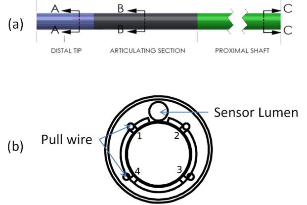
Fig. 5: (a) Catheter design with working channel. The distal tip (blue) houses the 5-DOF electromagnetic sensor used with the tracking system. (b) Cross section of distal tip showing four pull wires and sensor lumen.
