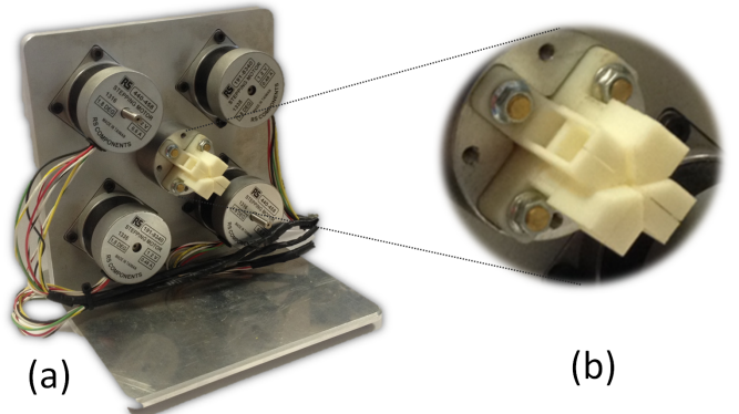
Fig. 7: (a) Electromechanical tensioning system. (b) Force sensing linear actuators for tensioning the catheter pull-wires.
