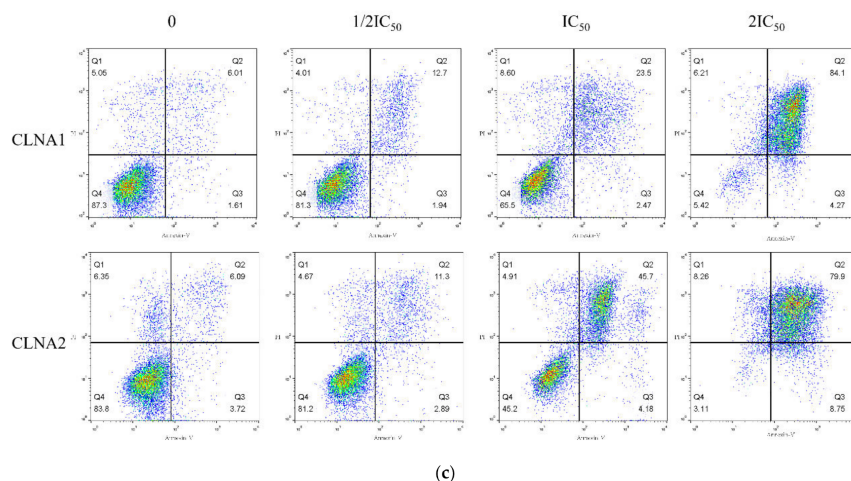
Figure 3. Anti-proliferative activity of CLNA1, CLNA2 against colon cancer cells. (a) Anti-proliferative effects of ALA, CLNA1, CLNA2 on three kinds of colon cancer cell lines and the corresponding IC 50 . (b) Morphology and quantity of Caco-2 cells treated by CLNA1 and CLNA2 at different time points. And the scale bar of every picture is 50 µm. (c) Flow cytometry of propidium iodide and annexin V-fluorescein isothiocyanate (FITC)-stained Caco-2 cells stimulated by different concentrations of CLNA1 or CLNA2 for 48 h. Data are presented as mean ± SEM and at least three separate experiments were performed in all studies. *, p < 0.05 , **, p < 0.01 and ***, p < 0.001 compared with control.
