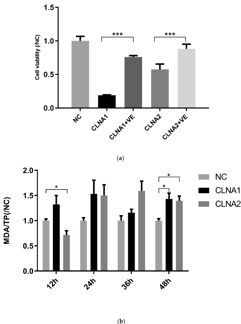
Figure 4. Induction of lipid peroxidation by CLNA1 and CLNA2 in Caco-2 cells. (a) The effects of inhibitor VE on the Caco-2 cells treated with CLNA1 and CLNA2, respectively ( n = 6 ). (b) The changes of MDA protein expression in Caco-2 cells during the treatment with CLNA isomers ( n = 3 ). NC indicated control group without CLNA treatment. Data are presented as mean \pm SEM and at least three separate experiments in all studies. * p < 0.05 , ** p < 0.01 and *** p < 0.001 compared with control.
