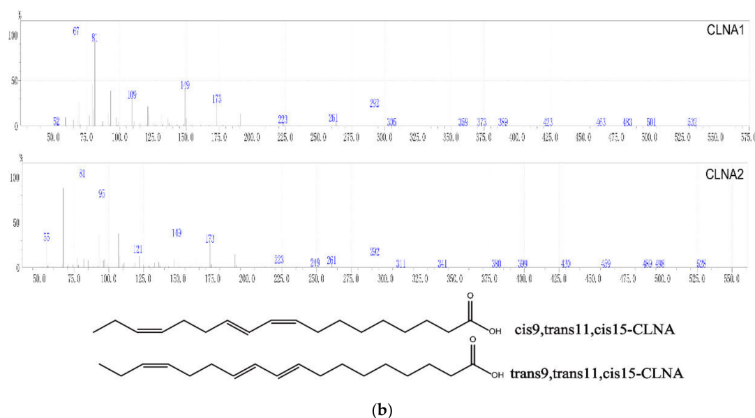
Figure 2. Preparation and purity detection of CLNA1 and CLNA2. (a) Separation of CLNA1 and CLNA2 by liquid chromatograph. The purity of CLNA1 and CLNA2 detected by GC-MS (C17:0 was added as a standard). (b) Mass spectrum and chemical structures of conjugated linolenic acid (CLNA) isomers used in this study (CLNA1: c9, t11, c15-CLNA, CLNA2: t9, t11, c15-CLNA).
