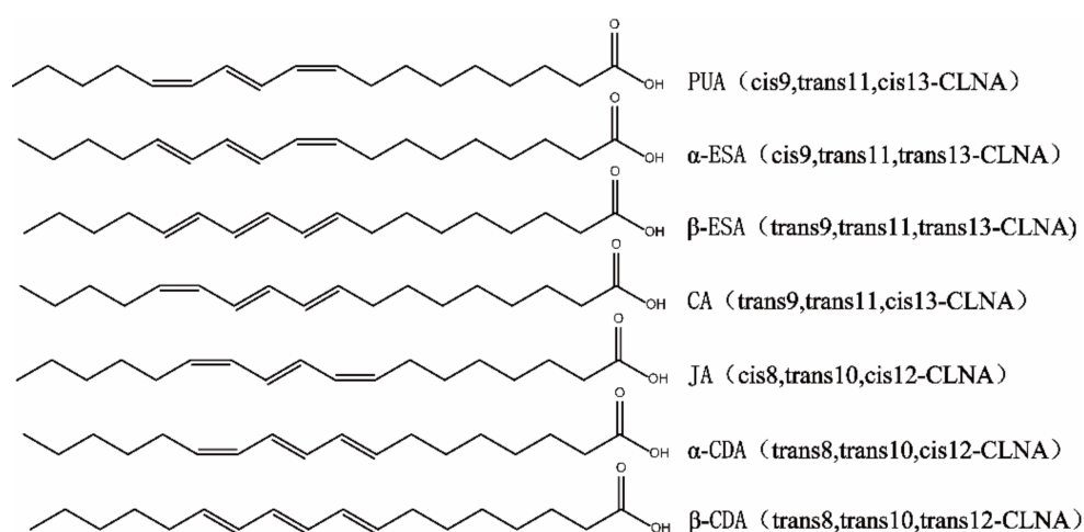
Figure 1. Chemical structure of plant-derived CLNAs.
