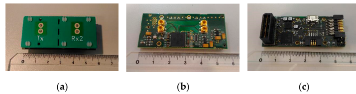
Figure 12. Ultra-wideband radar module. (a) Antenna board; (b) RF board; (c) digital board.
