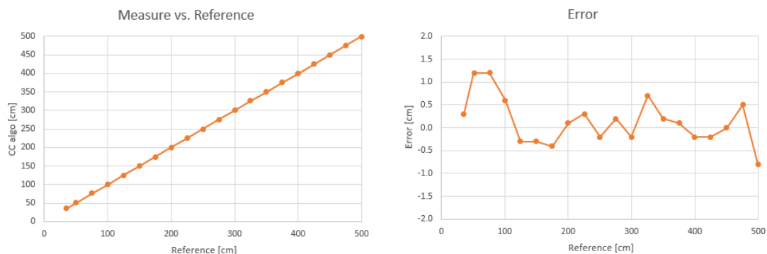
Figure 6. Measured distance vs. reference and its error.
