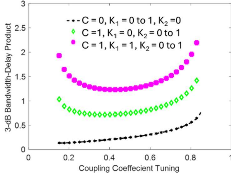
Figure 3: Bandwidth-delay product v/s coupling coefficients around f_0 .
