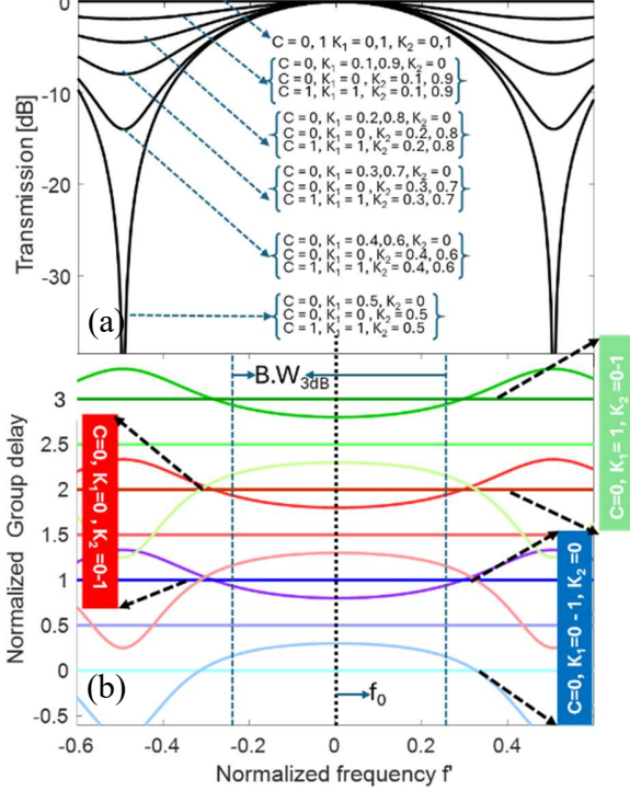
Figure 2: (a) Transmission spectra and (b) normalized group delay spectra for different combinations of coupling coefficient K .
