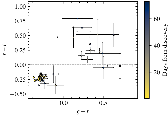
Fig. 4. Colour locus plot of GOTO0650 from LCO and TTT gri photometry, showing the distinct two clusters corresponding to the high and low state. The points are shaded to show the phase relative to discovery.
