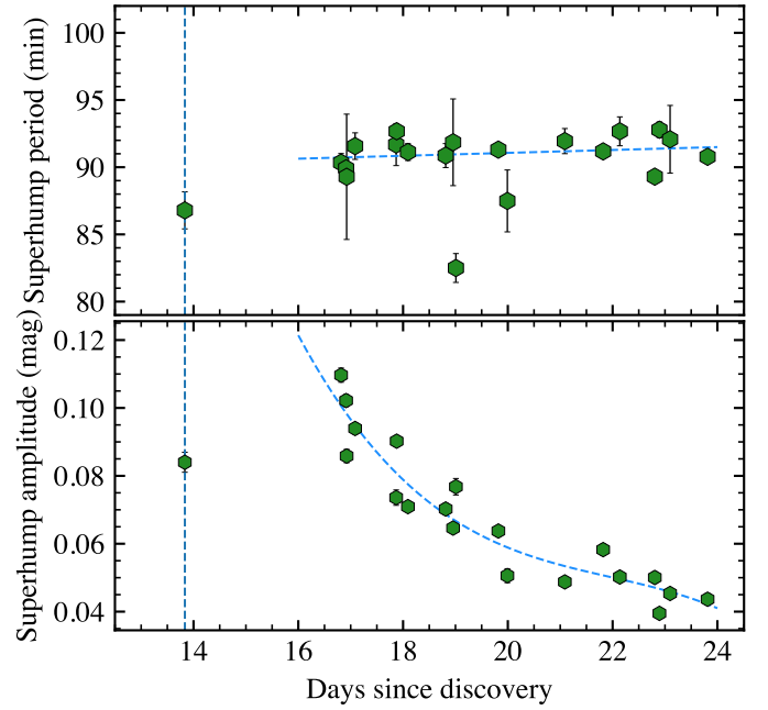
Fig. 8. Superhump period and amplitude evolution in GOTO0650. The time is given relative to the GOTO discovery date. The dashed blue line indicates the first epoch at which superhumps were detected. The error bars in both plots are the 1\sigma statistical uncertainties. An illustrative fit to the superhump period and amplitude is overplotted to show the overall evolution.
