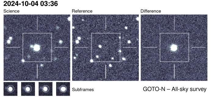
Fig. 1. GOTO discovery triplet of GOTO0650 as seen by citizen scientists on the Kilonova Seekers project, with the science frame, the historical reference image, and the difference image. The inner box corresponds to a scale of \approx 80 arcsec across. The labelling indicates the time of observation of this source and the GOTO site and survey mode that the observation was taken from. Below the science image, we show a series of subframes of the four individual exposures that were stacked to create the science image.
