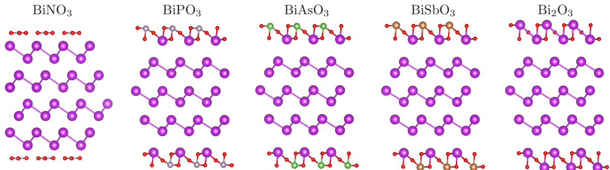
FIG. 6. Relaxed films with oxide termination including different group V elements. All oxide layers except for \text{BiNO}_3 have a very similar structure compared to \text{Bi}_2\text{O}_3 . The bond lengths within the oxide layer increase the heavier the group V element is. The light nitrogen atoms detach with the bonded oxygen atoms so that the Bi-O distance becomes larger than 2.5 \text{ \AA} , which is an increase by more than 10% compared to the other structures. Presumably, the N-O bonds are too short to allow for the formation of a comparable oxide.
