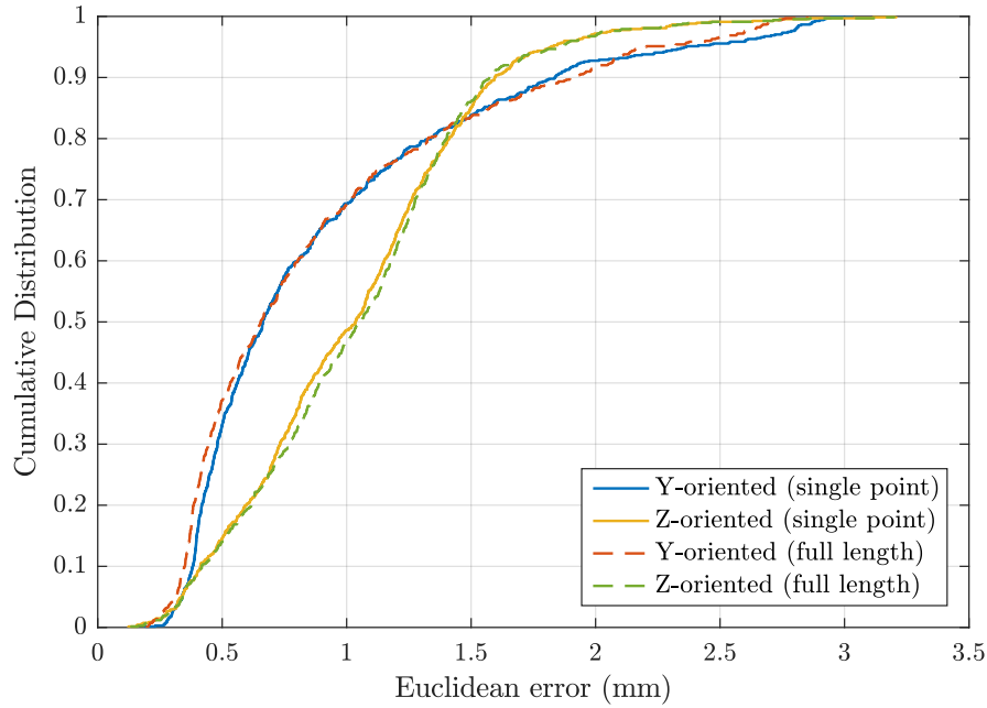
Figure 6.6: Cumulative distribution function of the position error obtained using the full-length and the single-point magnetic models. The associated error metrics are reported in Table 6.2.
