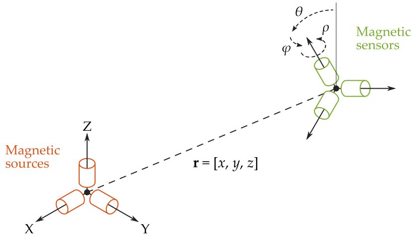
Figure 2.1: The magnetic sources generate a magnetic reference frame where unique magnetic field vectors characterise each position. The signal measured by the magnetic sensors is used to determine the relative pose, [x, y, z, \rho, \theta, \varphi] , between the sources and the sensors.
