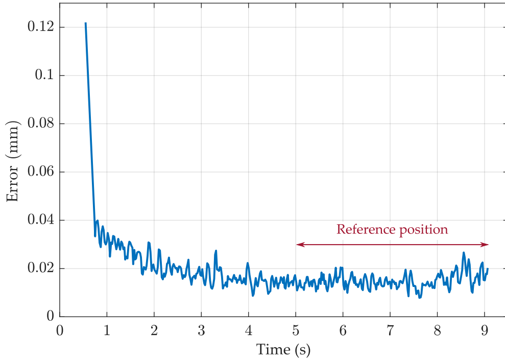
Figure 3.15: Position error due to mechanical oscillations. The error is calculated in relation to the value at convergence.
