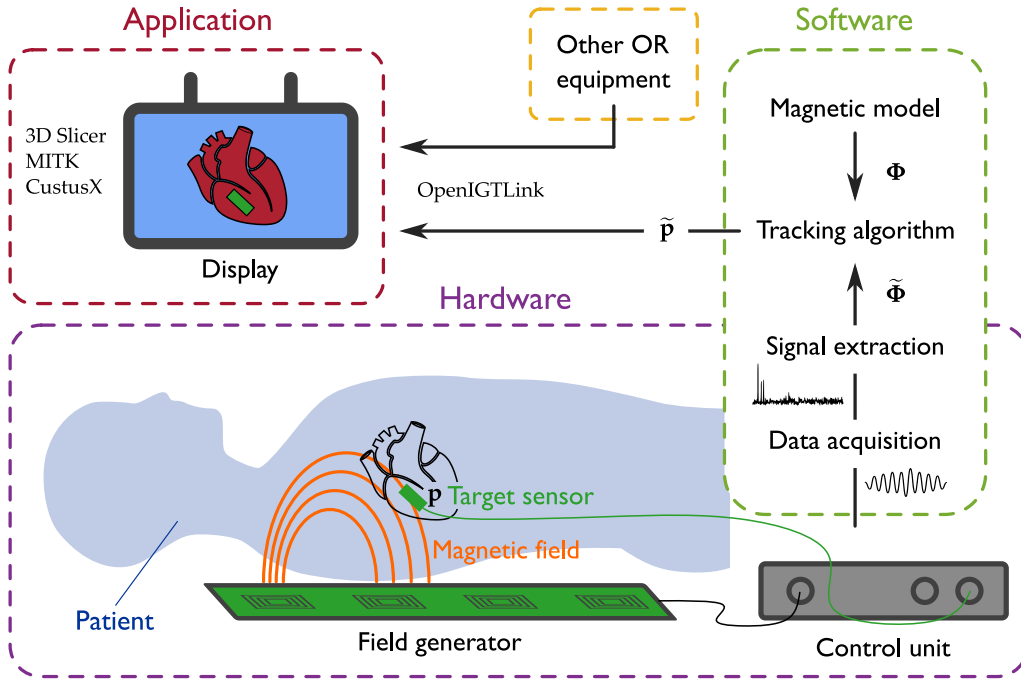
Figure 3.1: A schematic representation of the overall data flow in the ANSER EMT system. The target sensor, typically attached to the instrument tip, measures the magnetic field generated by a set of transmitter coils inside the field generator. The signal is acquired in the control unit and transmitted to a personal computer, where it is processed to determine sensor position and orientation using a known magnetic field model. The instrument can be visualised inside a pre-recorded anatomical image to assist the medical procedure.
