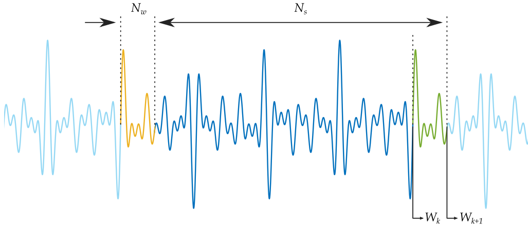
Figure 5.1: A sliding window of size N_s is updated every N_w samples, for an increased update-rate. The latency does not change, as the average delay remains of N_s/2 samples.
