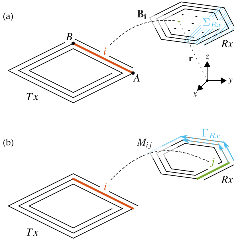
Figure 7.1: The mutual inductance between coil Tx and coil Rx can be calculated in two ways: (a) from Equation 7.1 and numerically approximated by evaluation of the magnetic field generated by Tx across the area of Rx ; (b) from Equation 7.2 as the sum of the partial mutual inductances between the straight filaments of the two coils.
