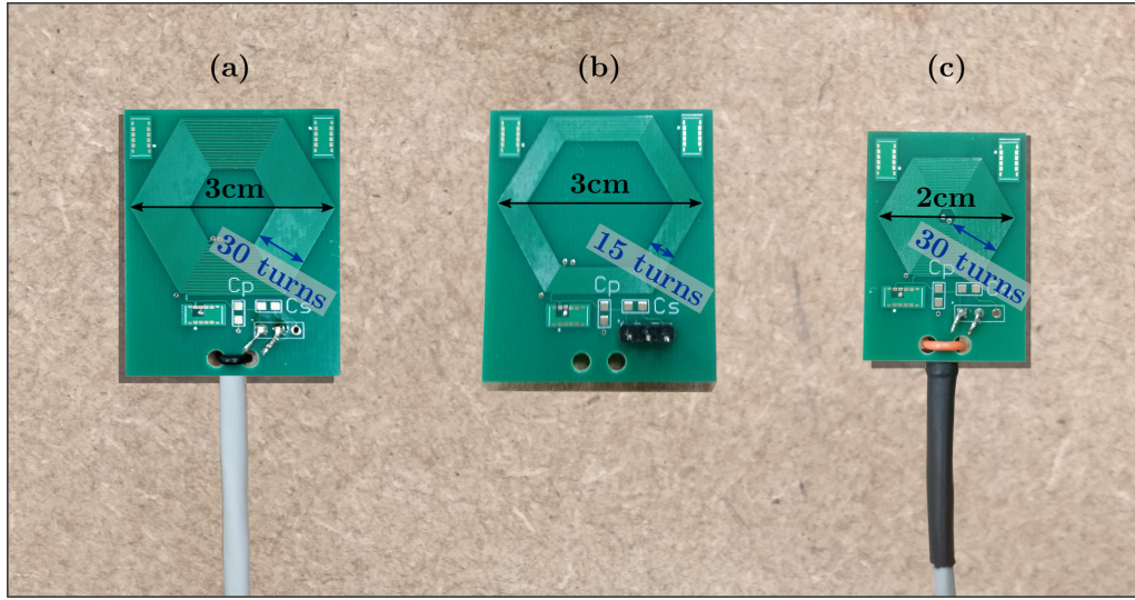
Figure 7.6: Three hexagonal sensors were manufactured on a four-layer PCB. (a) The reference coil has a diagonal, D_{out} , of 3 cm and 30 turns per layer. (b) Another version with 15 turns, and (c) a smaller coil with D_{out} = 2 cm, were realised to validate the formulas used in the coil design procedure.
