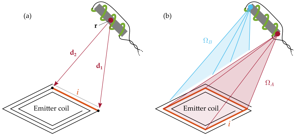
Figure 6.1: Calculation of the magnetic flux crossing an elongated inductive sensor (a) from the sum of the contributions due to the individual filaments forming the emitter coil, where the sensor is approximated as a single point. (b) The full sensor length is considered by calculating the flux as the finite difference of the magnetic scalar potential, which depends on the solid angles, \Omega_A and \Omega_B , subtended by the emitter coil current path at the sensor end-points.
