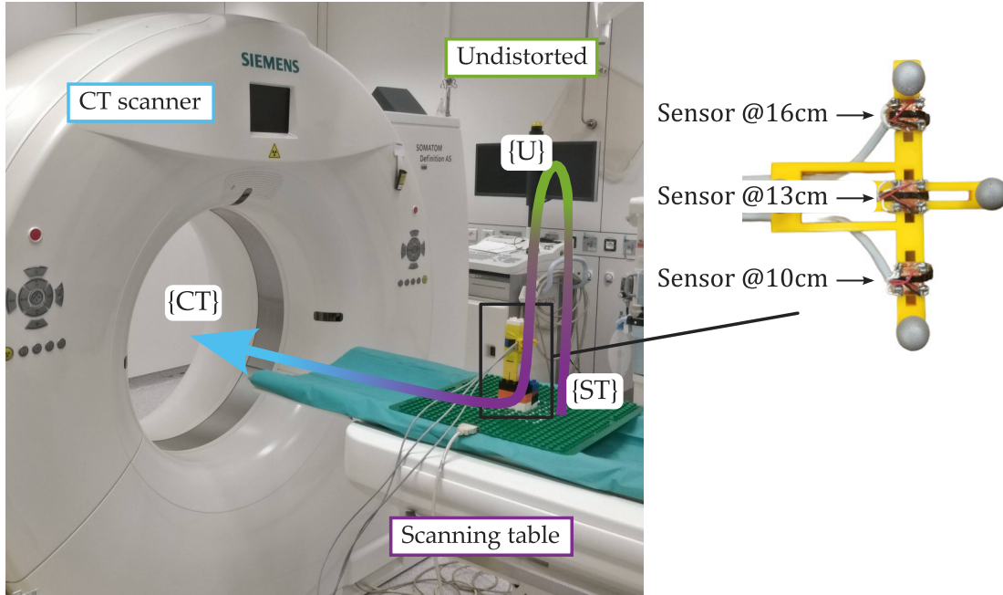
Figure 4.13: Tool C was mounted on Duplo blocks at a fixed position on the field generator, which was positioned on the scanner table, position {ST}. The assembly was then lifted to obtain undistorted measurements, position {U}. Finally, the field generator was placed back on the bed and slid into the CT scanner, position {CT}. Throughout the entire process, the EMT algorithm and distortion detection techniques were continuously in operation.
