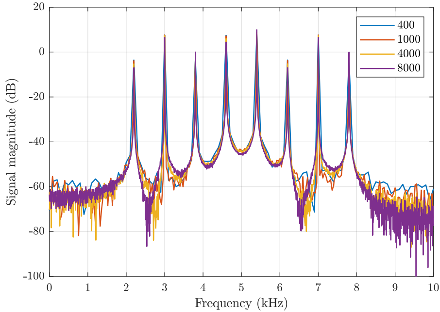
Figure 3.7: Effect of sensor linear motion in the X direction starting from \mathbf{p} = [0, 0, 150, 0, 0] , for different numbers of samples at 40 kHz. The sensor was moved at the unrealistic speed of 25 cm/s, for visualisation purposes, corresponding to a displacement of 2.5 mm in the shortest window case (400 samples) and 50 mm for the longest window (8000 samples).
