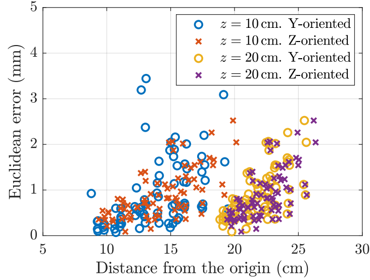
Figure 3.23: Scatter plot of the Euclidean position error as a function of the distance of the test point from the field generator centre.
