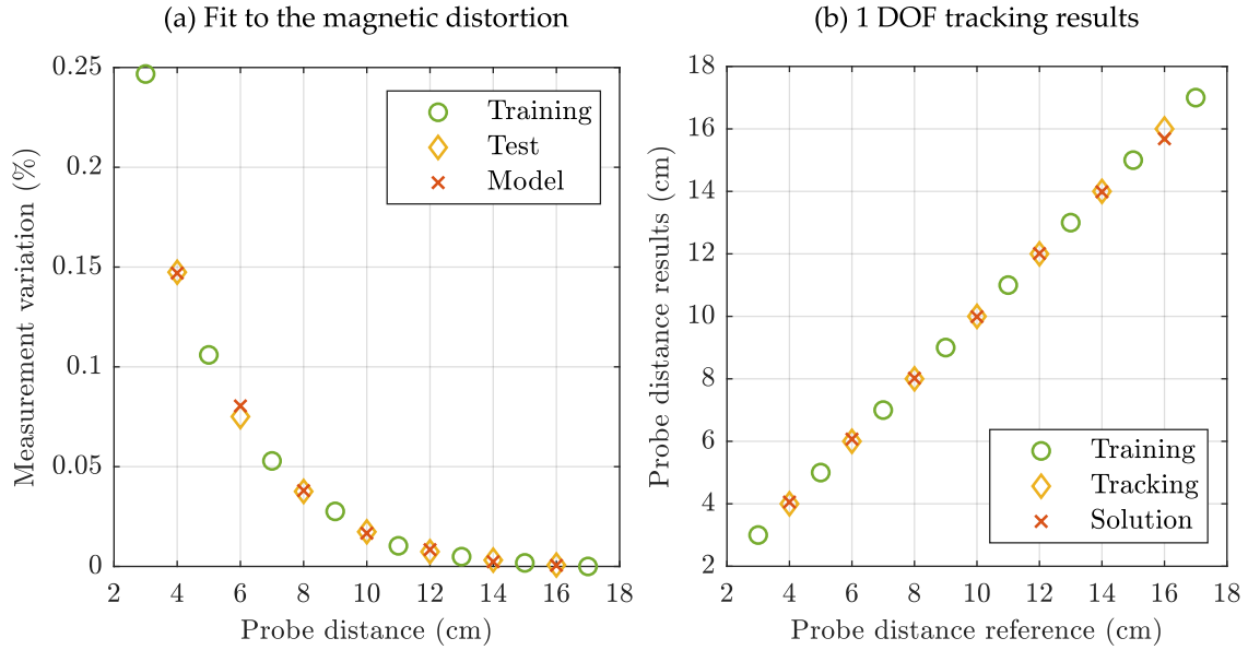
Figure 4.20: (a) Fitting effectiveness of the distortion model outlined in Equation 4.11. (b) Distortion-based tracking with one degree of freedom.
