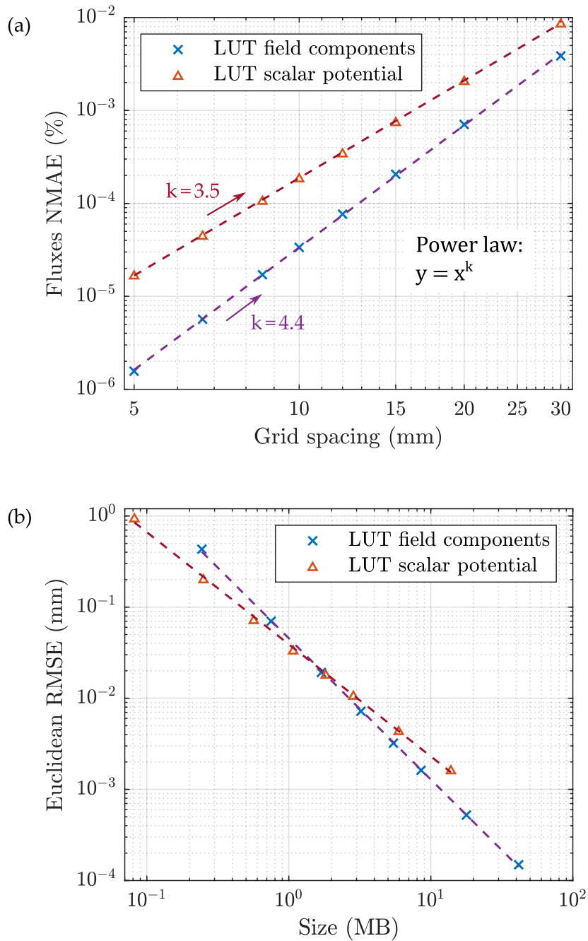
Figure 6.5: (a) Interpolation error and (b) correspondent position tracking error as a function of the table size for the two tabulated models compared. Blue crosses: the three magnetic field components are stored independently, and the fluxes are obtained from Equation 6.1. Red triangles: the magnetic scalar potential is saved at grid points, and the fluxes are calculated from Equation 6.6. The interpolation error follows a power law with exponents of k = 3.5 and k = 4.4 , respectively.
