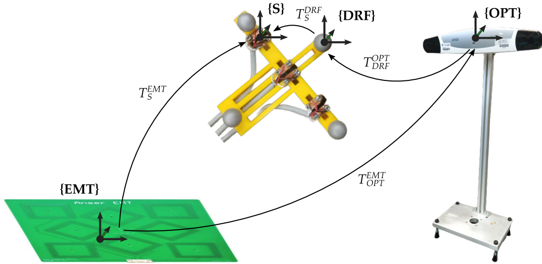
Figure 3.12: Linear transformations between the reference frames of ANSER EMT \{\text{EMT}\} , the optical system \{\text{OPT}\} , the optical marker \{\text{DRF}\} , and the sensor pose within the dynamic reference frame \{\text{S}\} .
