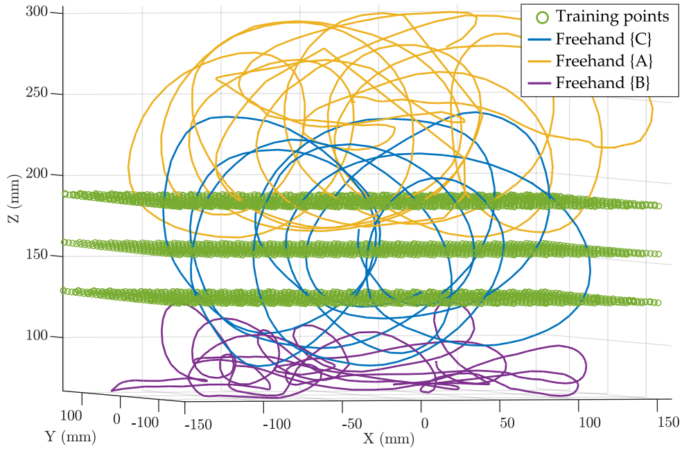
Figure 4.3: Trajectories of the three freehand tests performed in the central region, {C}, above {A}, and below {B} the training points used to build the data-driven magnetic model.
