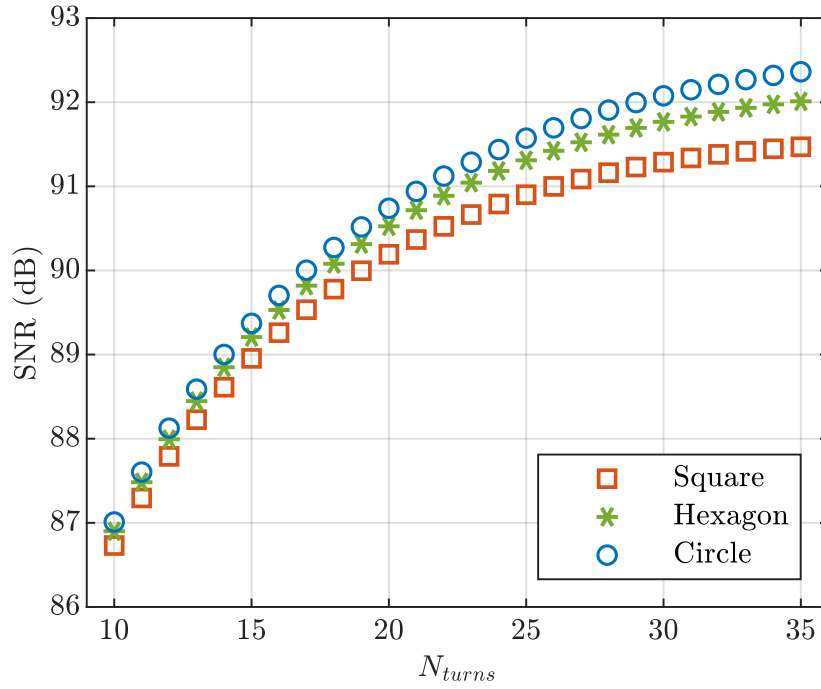
Figure 7.4: SNR predicted from Equation 7.26 with variation in turn count. Circular, hexagonal, and square planar coil shapes are compared. The three planar coils have the same footprint area of a hexagon with a diagonal of 3 cm ( A_c = 5.85 \text{ cm}^2 ).
