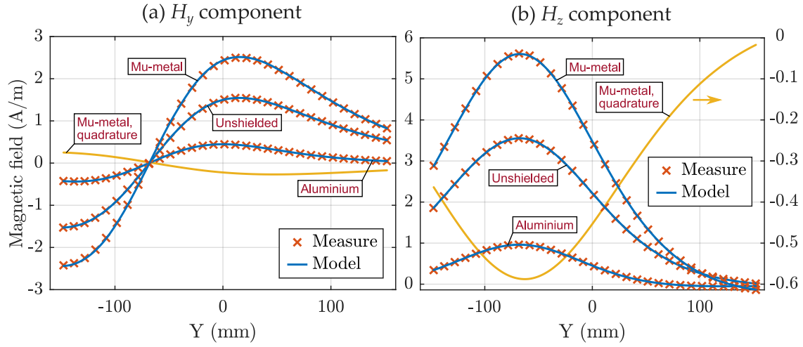
Figure 4.8: Effect of shielding on the magnetic field of the emitter coil number 4, which is defined in Figure 3.2, at X = 0 mm and Z = 150 mm. (a) Y component and (b) Z component of the field. The quadrature field component, which appeared in the presence of the mu-metal shield, is plotted in yellow.
