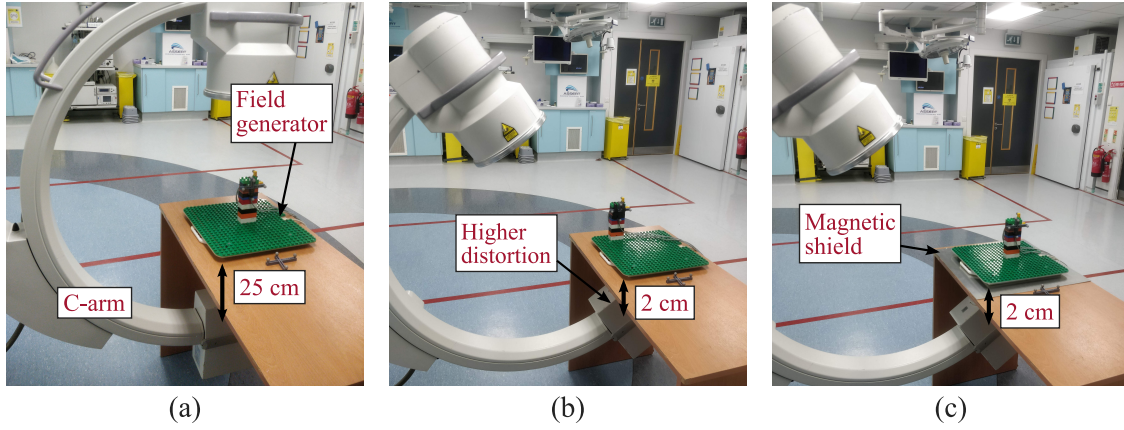
Figure 4.9: The C-arm effect was evaluated at different distances from the field generator, (a) from 25 cm, which caused the smallest distortion, (b) to the minimum distance of 2 cm, which caused the largest distortion. (c) Aluminium and mu-metal magnetic shields placed below the field generator were tested as a possible solution against static and dynamic distorters below the field generator.
