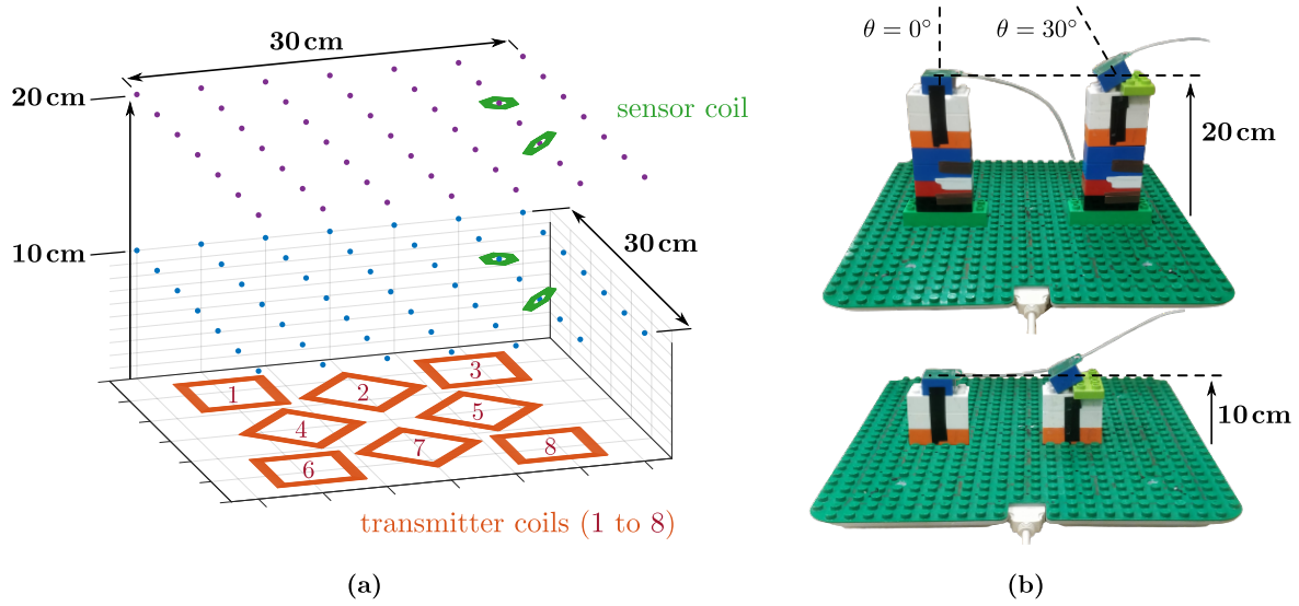
Figure 7.10: (a,b) The mutual inductance was measured on a grid of 7 \times 7 points at 10 cm and 20 cm from the planar field generator, for two sensor orientations: pitch angles \theta = 0^\circ and \theta = 30^\circ . At every test point, the eight mutual inductances between the sensor coil and the eight transmitter coils are considered, leading to a total of 49 \times 4 \times 8 = 1568 mutual inductances experimentally evaluated.
