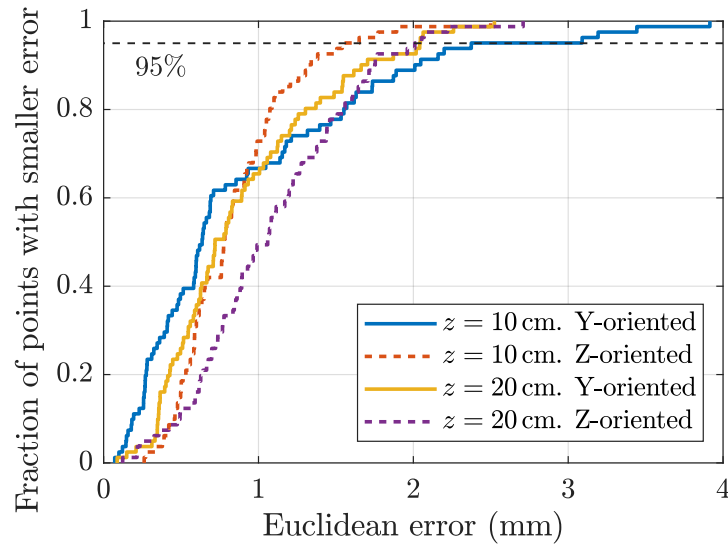
Figure 3.22: Cumulative distribution function of the Euclidean position error calculated at test points as per Equation 3.28.
