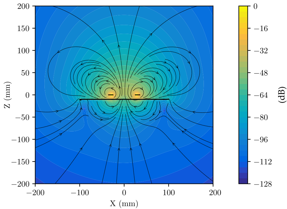
Figure 8.1: (a) Current distribution for an active shield located at 1 cm below the transmitting coil. (b) Magnetic field magnitude map of the self-shielded coil configuration.
