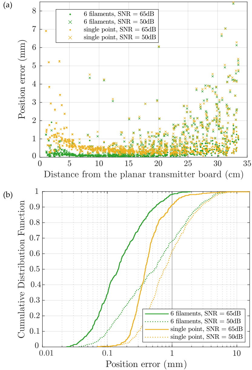
Figure 7.9: (a) Static accuracy test simulation for two noise levels compared. Position errors depend on model approximations and noise magnitude. (b) Cumulative distribution function of the position error for the two magnetic models considered and average noise levels of -50 and -65 dB.
