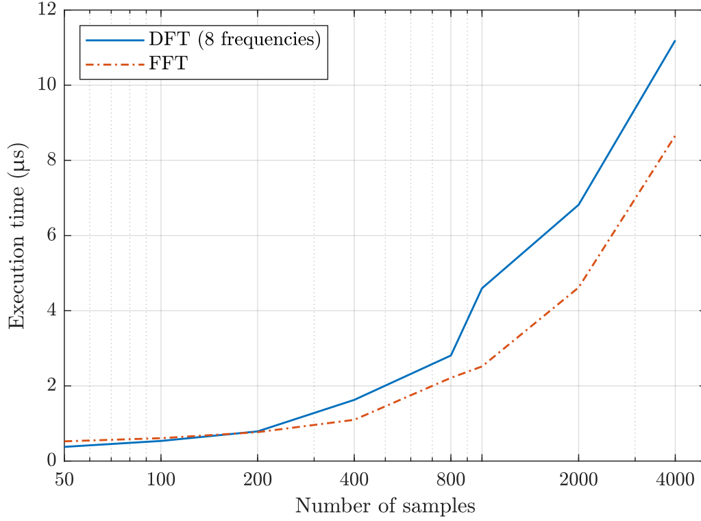
Figure 3.8: Average computation time of the DFT sum for the eight frequencies of interest and the fft MATLAB function for an increasing number of samples.
