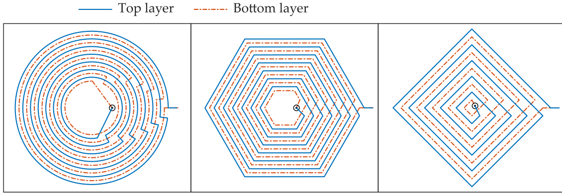
Figure 7.5: The footprints of subsequent layers are shifted so that the traces do not overlap. In this way, the parasitic capacitance of the winding is minimised, and the self-resonance frequency is maximised.
