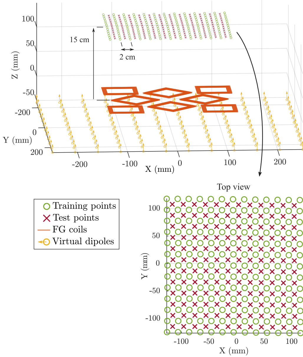
Figure 4.7: Modelling of the highly distorted magnetic field in the presence of metallic shields under the field generator. The model was represented by an array of 12 \times 12 virtual magnetic dipole sources, the magnitude of which was optimised to match the training points magnetic measurements. Interpolation results were evaluated on the test points.
