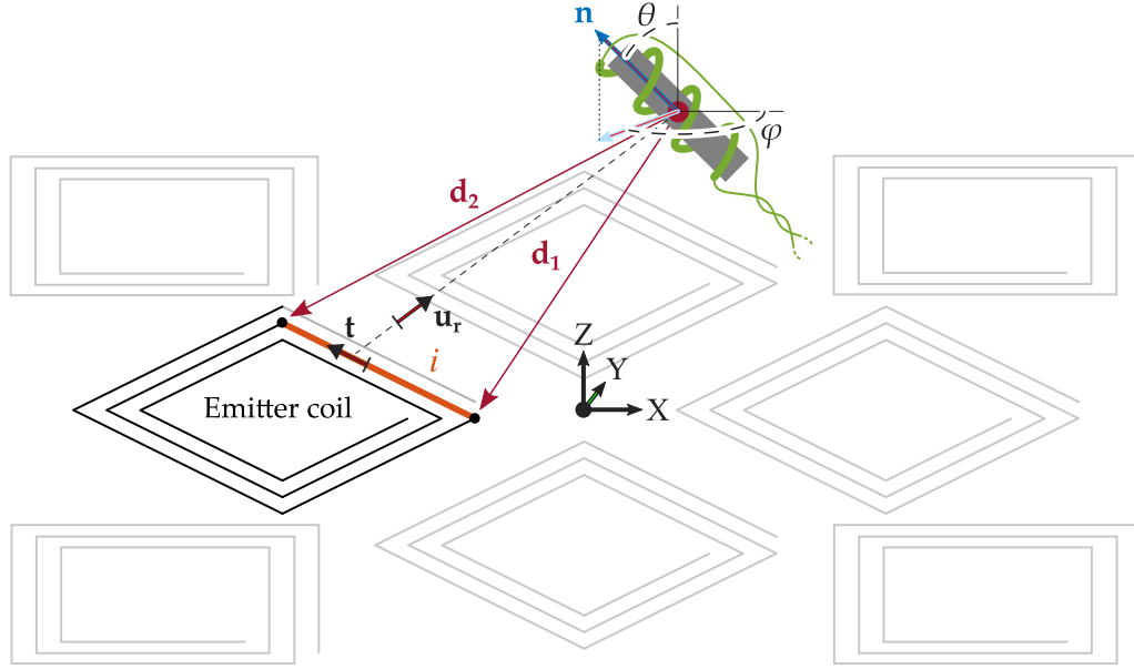
Figure 3.9: Analytical model for the magnetic flux crossing an inductive sensor located at \mathbf{r} with orientation \mathbf{n} . For every emitter coil, the field is split into the sum of the contributions due to the individual filaments forming the coil, each calculated as per Equation 3.7.
