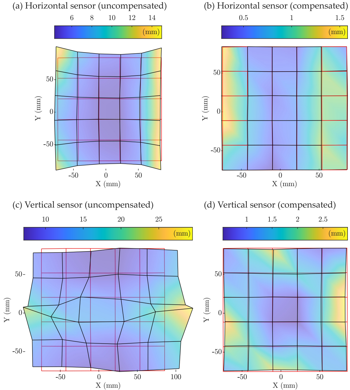
Figure 4.17: EMT accuracy with the field generator placed on top of the fluoroscopy system, evaluated on the plane at 6 cm from the reference plane shown in Figure 4.16. The results are shown for (a,b) horizontally and (c,d) vertically oriented sensors, (a,c) before and (b,d) after applying the compensation technique proposed in this section. The red grids are formed by joining the undistorted optical positions, while the black grids represent the EMT points. The colour maps show the error in millimetres. The distortion in the Z-direction is not appreciable from these 2D plots.
