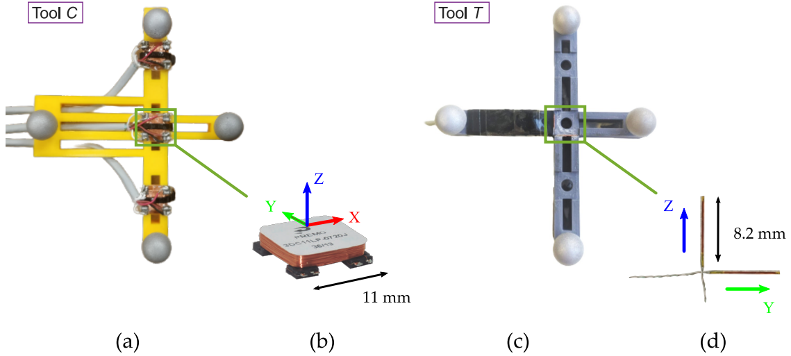
Figure 3.11: (a) Tool C includes (b) three triaxial sensor coils. (c) Tool T is equipped with (d) two uniaxial clinical-size sensors.
