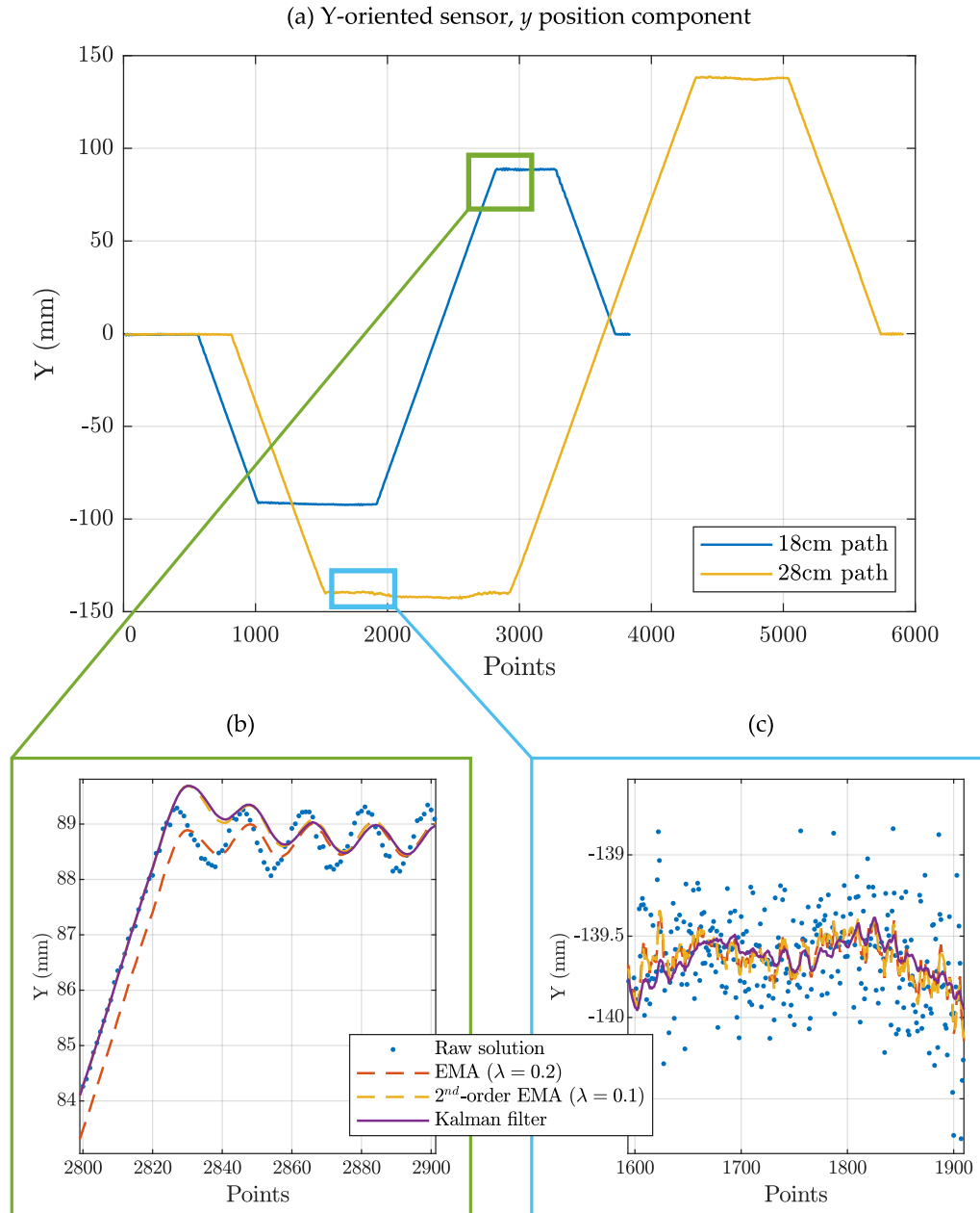
Figure 5.3: (a) Profile of the tracked y coordinate of the Y-oriented sensor. Two sections were selected to better visualise the performance of the filters (b) at constant velocity and with a sudden change in the motion direction, and (c) when the y coordinate is constant and the jitter noise is more evident.
