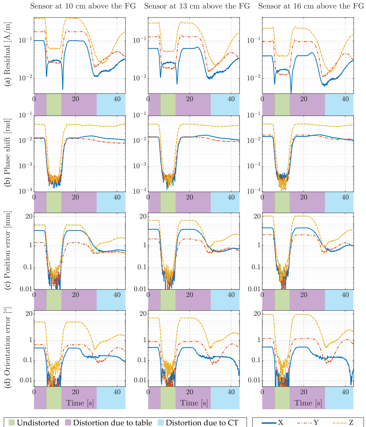
Figure 4.15: Distortion detection compared to the corresponding EMT errors, for three triaxial sensors, at 10, 13, and 16 cm from the field generator (FG), with axes oriented along X, Y, and Z. (a) EMT algorithm residual, as given by Equation 4.9. (b) Signal phase shift, calculated according to Equation 4.10. (c) Position error in millimetres, relative to the position measured without distortion {U}. (d) Orientation error in degrees, in relation to the same EMT point used for the position error.
