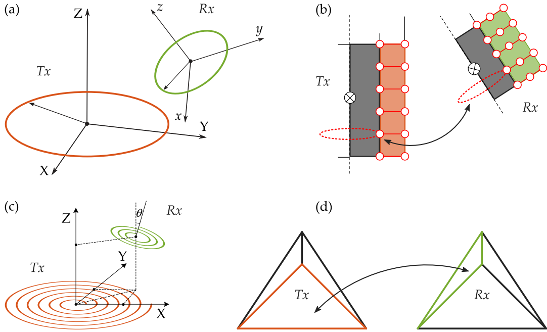
Figure 2.2: Magnetic models for spatially extended transmitting, T_x , and receiving, R_x , antennas. The mutual inductance is calculated using approximations such as (a) circular loops [18], (b) distributed loops [19], (c) spiral coils [20], and (d) straight-line conductors [21].
