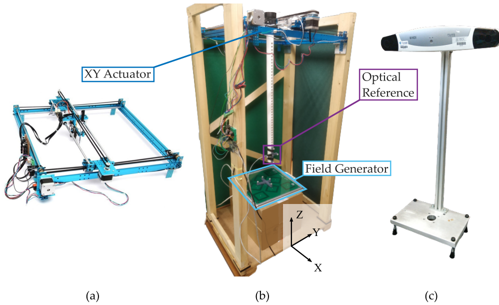
Figure 3.14: (a) XY Plotter Robot Kit available in the market [87]. (b) A wooden frame is used to keep the robot far from the ROI and avoid magnetic distortion. The sensor is mounted on a plastic rod. (c) Accurate pose reference is provided by an external optical system [82].
