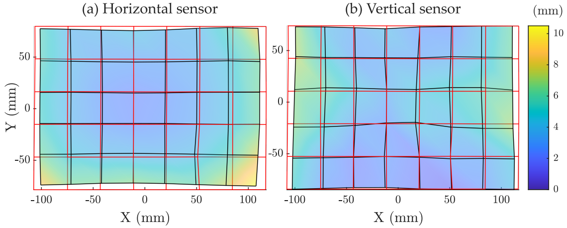
Figure 4.11: Effect of the C-arm on the position tracking error when it was placed directly below (2 cm) the planar field generator, without magnetic shielding or distortion compensation, when the magnetic sensor was (a) Y oriented (horizontal) or (b) Z-oriented (vertical). The red grid is formed by joining the test points, and the black grid represents the EMT sensor position. The colour map, in mm, also accounts for the error in the Z direction, which is not appreciable from the 2D grids.
