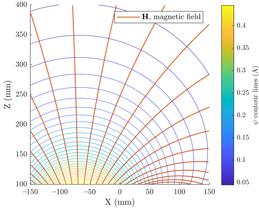
Figure 6.2: Magnetic field and associated scalar potential of the 4 th emitter coil of the field generator, evaluated on an XZ plane at Y = 0 .
