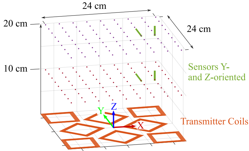
Figure 3.21: The magnetic field generated by the eight transmitter coils was measured at two grids of 81 points for two different sensor orientations, i.e. \theta = 90^\circ (Y-oriented) and \theta = 0^\circ (Z-oriented).
