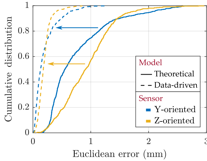
Figure 4.4: Cumulative distribution of EMT position errors obtained in a distortion-free environment with the existing theoretical model and the new data-driven model for the static tracking measurements indicated in Figure 4.1. Two commercial miniature sensors, Y and Z-oriented (horizontal and vertical), were placed on a 25 \times 25 \text{ cm}^2 grid approximately 15 cm above the field generator.
