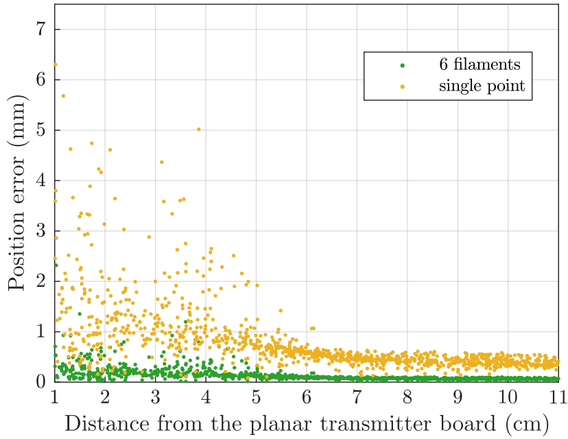
Figure 7.8: Static accuracy test simulation with no added noise. The position errors are due to model approximations. The two simplified models presented in Section 7.4.1 are compared.
