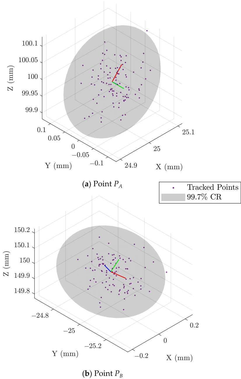
Figure 6.7: Simulated position error where the signal was perturbed with white Gaussian noise at -63 dB. The tracked positions are visualised in (a) and (b) for end-points P_A and P_B of the 128 mm flexible sensor depicted in Figure 6.4 . The position noise of P_A is highly correlated to P_B and is modelled by a 6 \times 6 covariance matrix. The two corresponding uncorrelated trivariate Gaussian distributions are visualised through the 99.7% confidence regions (CR), which are ellipsoids with the main axes indicated by the RGB triplets.
