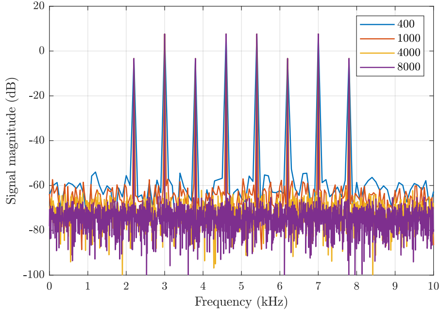
Figure 3.6: Noise level for different numbers of samples at 40 kHz. The shortest window (400 samples) has a bin resolution of 100 Hz, while the longest window (8000 samples) has a bin resolution of 5 Hz.
