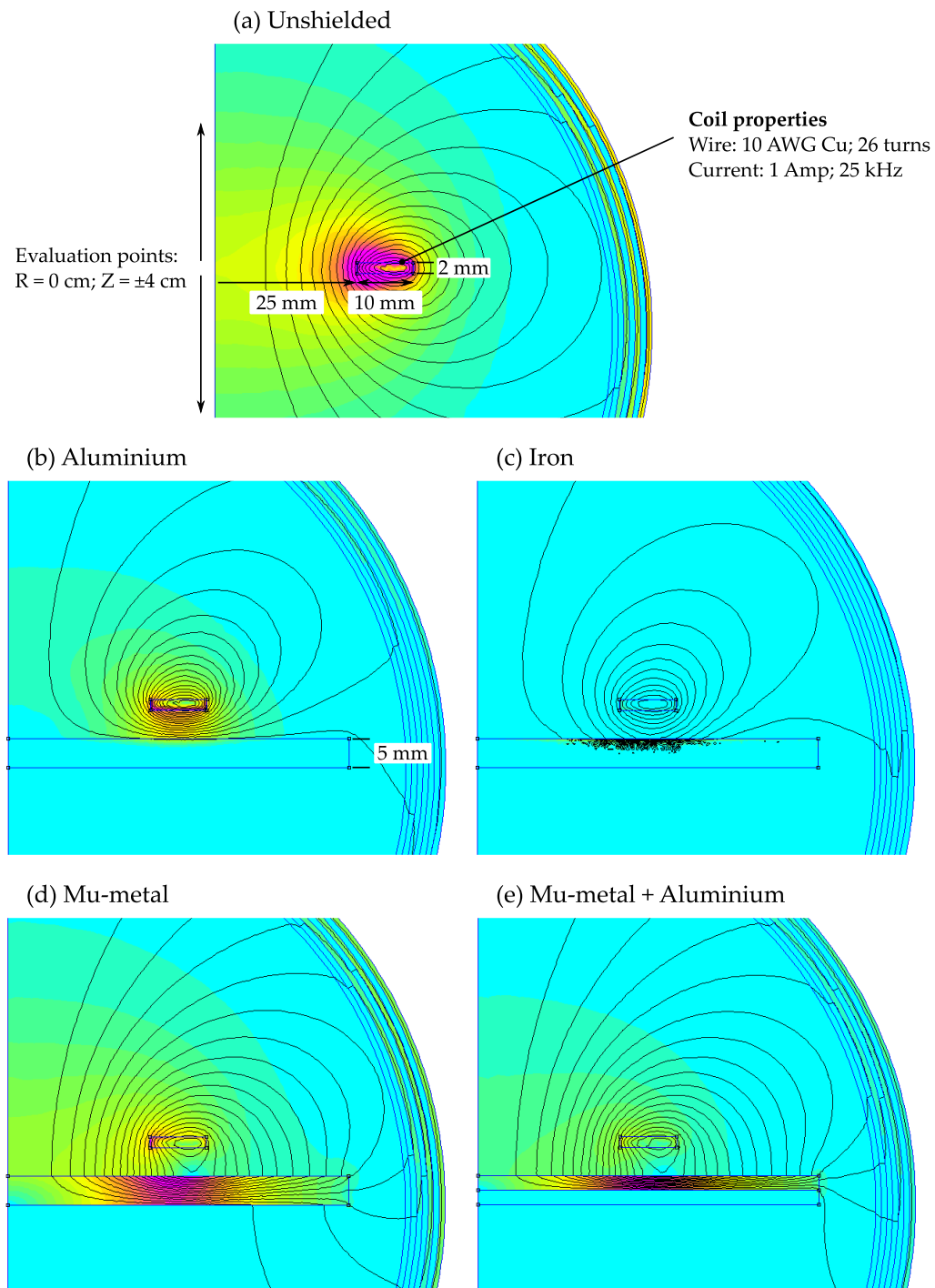
Figure 4.6: FEA simulation results showing the magnetic flux magnitude for different shielding materials placed under an emitter coil. Shielding effectiveness is reported in Table 4.2 .
