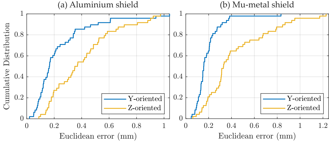
Figure 4.12: Tracking errors when the fluoroscopy system was at minimum distance, 2 cm below the field generator, using (a) an aluminium plate and (b) a mu-metal plate to shield the distortion. The field model used to find the sensor position was trained on data collected in an undistorted environment where the fluoroscopy C-arm was removed.
