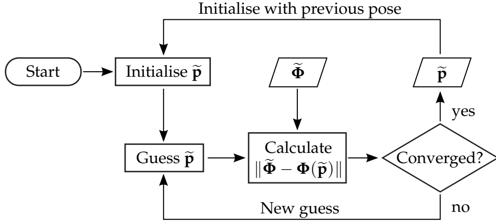
Figure 3.10: A schematic representation of the iterative algorithm used to estimate the EMT pose.
