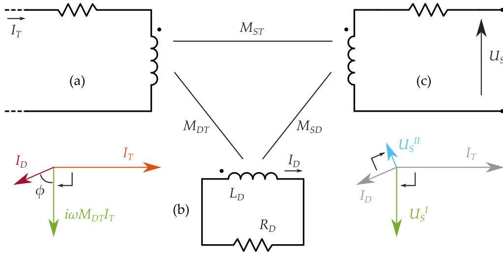
Figure 2.5: Equivalent RL circuit model for (a) one transmitting coil, (b) one conductive distorter, and (c) the inductive sensor coil.
