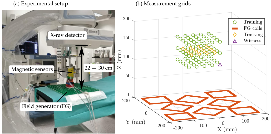
Figure 4.21: (a) The X-ray detector was moved to different vertical distances from the field generator ( Z = 22, 24, 26 , and 30 cm), and the magnetic field vector was captured on the training grid. Then, the X-ray detector was placed at Z = 28 cm, and the distance was estimated from the witness sensor measurement. A new calibrated field model was calculated based on the values pre-characterised and used to evaluate the EMT error on the tracking grid. (b) Position of the training grid, the tracking grid, and the witness sensor relative to the field generator coils.
