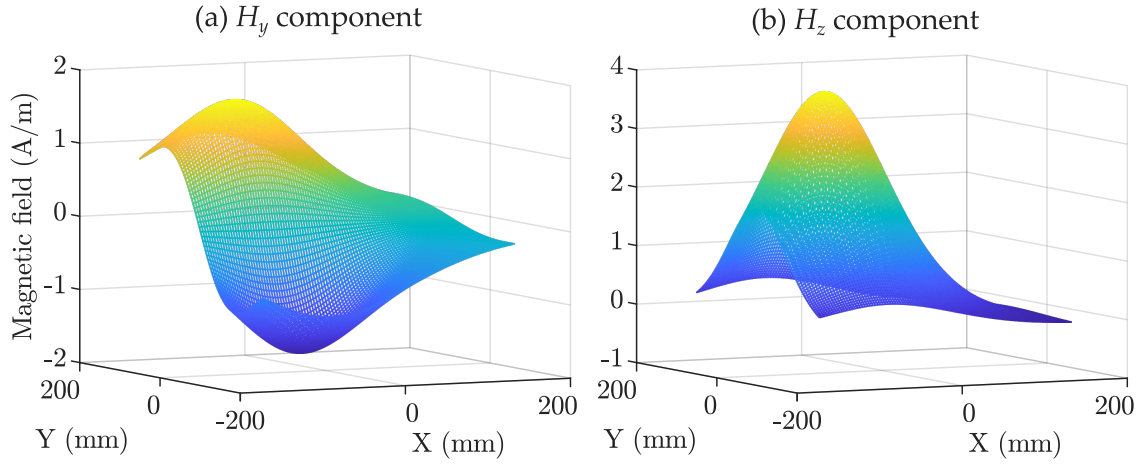
Figure 4.2: Data-driven magnetic field model, fit results. (a) Y component and (b) Z component of the magnetic field modelled for emitter coil 4, which is defined in Figure 4.1. The values are captured on a horizontal plane located 150 mm above the field generator.
