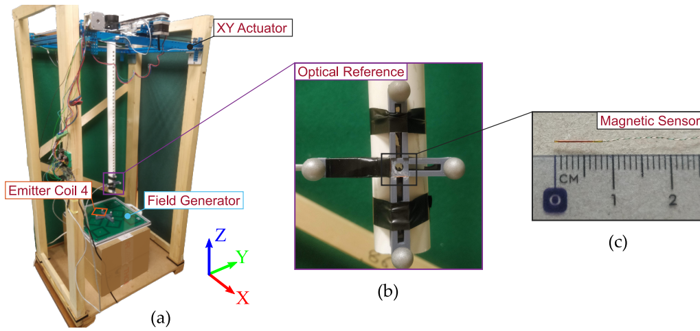
Figure 6.3: (a) The motorised actuator introduced in Section 3.4 was used to move the EMT sensors on an XY plane. Optical tracking provided accurate pose reference. One of the eight emitter coils of the field generator is highlighted in orange. (b) Two sensors were embedded in the dynamic reference frame to collect data in different directions. (c) A miniature sensor coil was used in the experiments [16].
