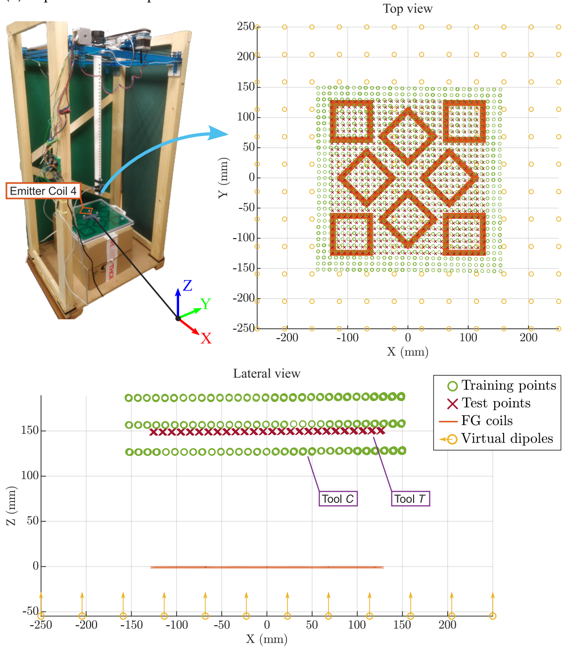
Figure 4.1: (a) Sensors used for characterisation (tool C) and tracking (tool T). (b) Experimental setup to characterise a volume within the ROI.
