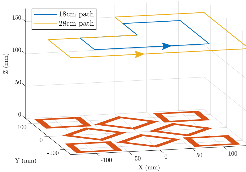
Figure 5.2: Dynamic tracking test. Two sensors, horizontally (Y) and vertically (Z) oriented, were tracked using a high update rate of 100 Hz. The experiment was repeated for two path lengths.
