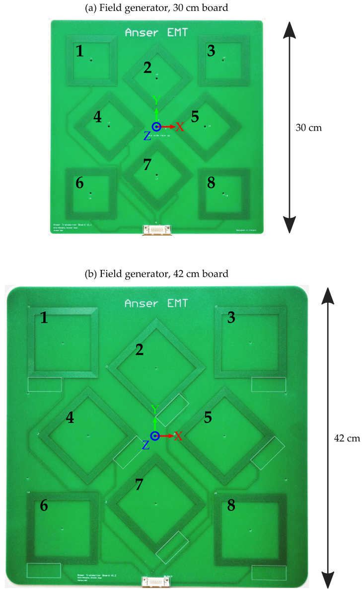
Figure 3.2: Two of the field generators available for the ANSER EMT system, with board dimensions of (a) 30 cm and (b) 42 cm, respectively. The eight emitter coils embedded in the field generators are visible and are numbered from 1 to 8.
