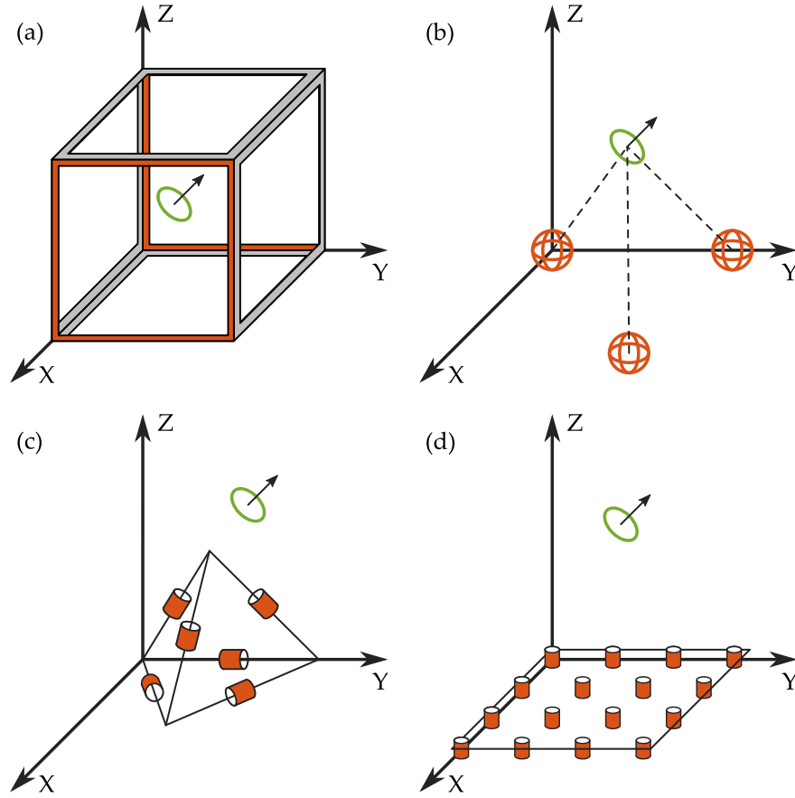
Figure 2.3: Alternative topologies for uniaxial tracking. (a) Rectangular cube transmitter [37]. (b) Triaxial sources or sensors [68]. (c) Tetrahedron configuration [69]. (d) Coplanar array of emitter coils [70].
