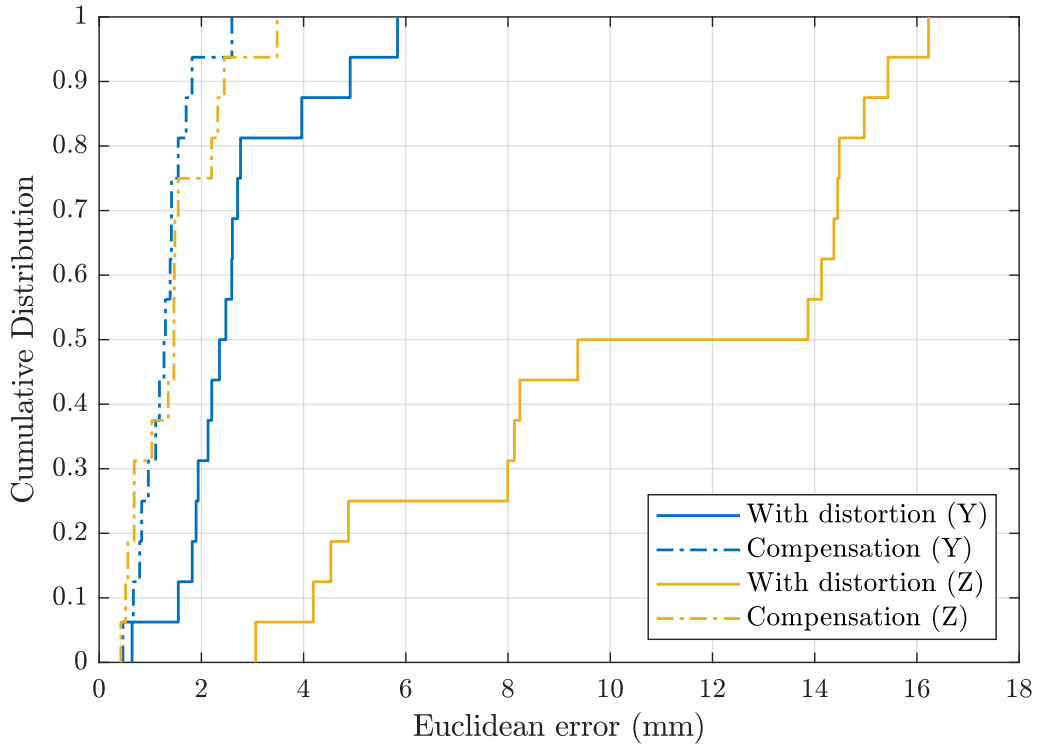
Figure 4.22: Position error with the X-ray detector placed Z = 28 cm above the field generator, for Y and Z-orientations. Errors are shown before and after applying the compensated magnetic field model to track the sensor.
