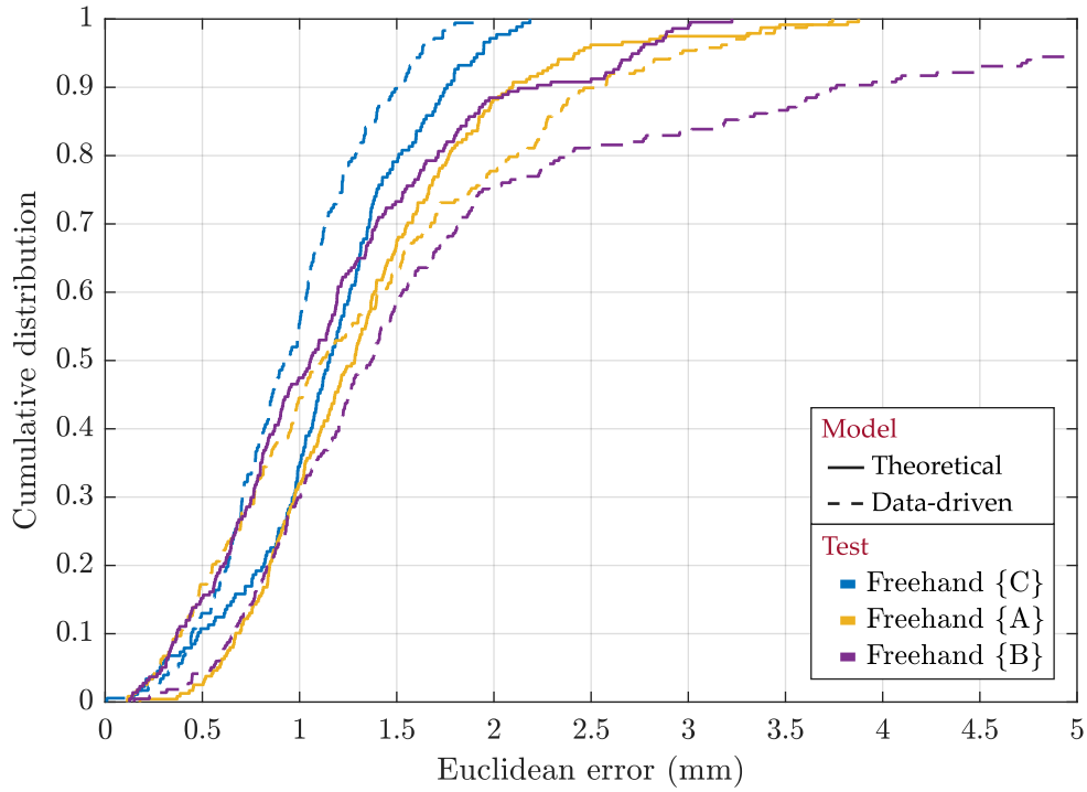
Figure 4.5: Cumulative distribution of EMT position errors obtained in a distortion-free environment with the theoretical model and the compensated data-driven model for freehand trajectory tracking as represented in Figure 4.3. One sensor was moved freehand within three regions, respectively centred {C}, above {A}, and below {B} the training grid.
