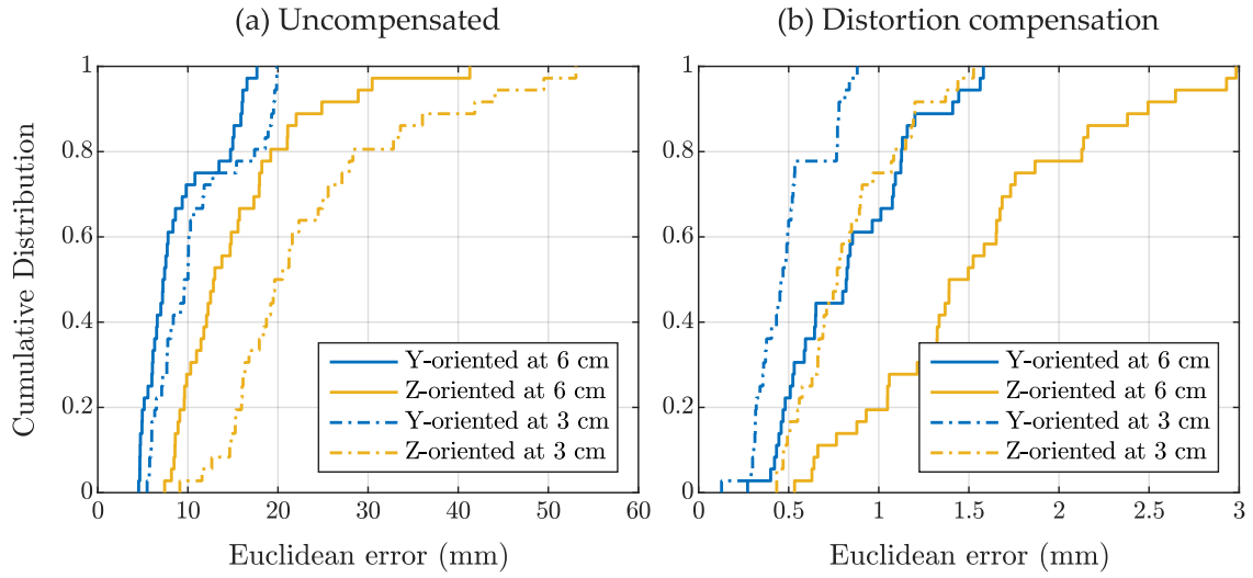
Figure 4.18: EMT errors with the field generator placed on top of the X-ray collimator. (a) Errors caused by metallic distortion before compensation. (b) Errors obtained using the calibrated magnetic field model. The results are reported for the two evaluation planes shown in Figure 4.16 .
