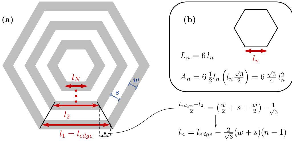
Figure 7.3: The spiral of a hexagonal planar coil is approximated as a set of concentric hexagons to calculate the coil's cross-sectional area and total length. (a) The edge length, l_n , of the n^{th} inner turn depends on the external edge, l_{edge} , and the trace width, w , and spacing, s .
