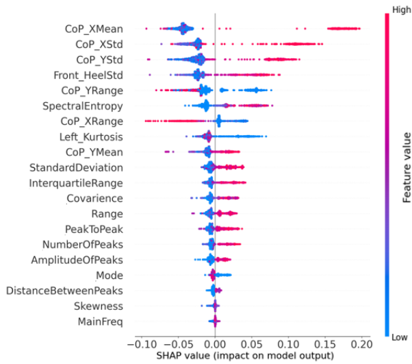
FIGURE 7. SHAP analysis of feature importance for walking in the 5 second observation window.
