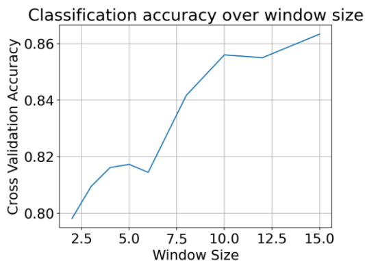
FIGURE 3. Accuracies of the random forest classifiers across all nine observation window sizes (2, 3, 4, 5, 6, 8, 10, 12, and 15 seconds).
