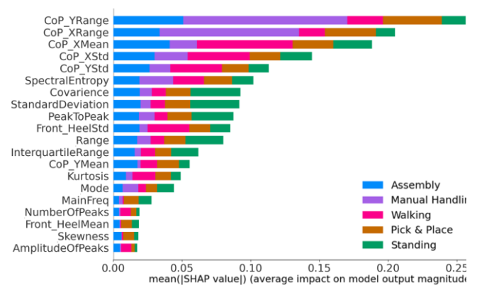
FIGURE 5. Analysis of feature importance for the 5 second observation window.
