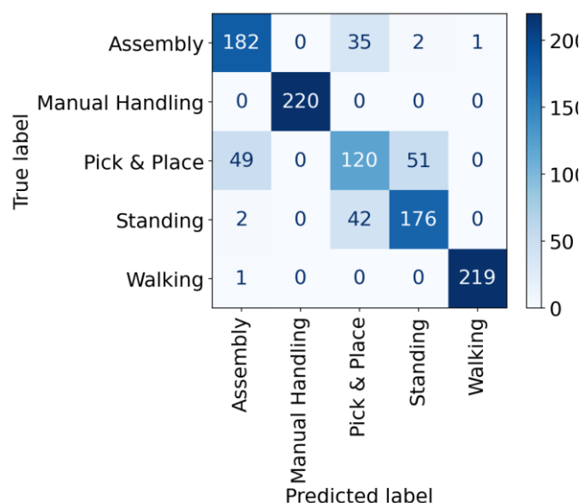
FIGURE 12. Confusion matrix showing the prediction accuracy for the top 5 features in the 5 second observation window.
