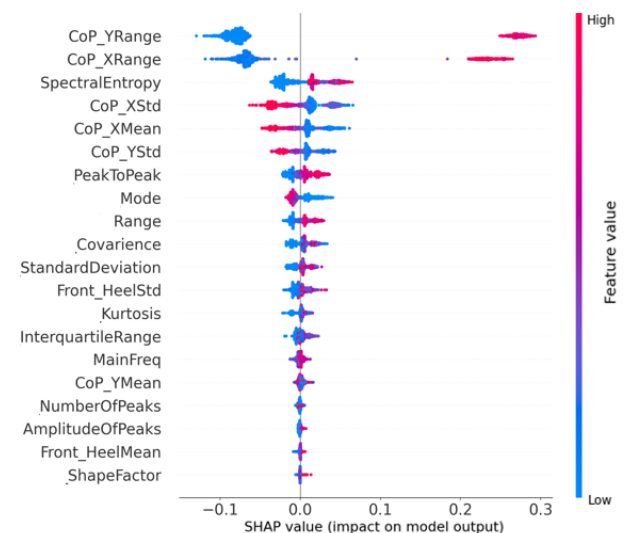
FIGURE 6. SHAP analysis of feature importance for manual handling in the 5 second observation window.
