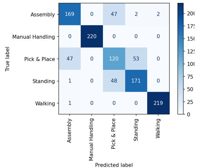
FIGURE 4. Confusion matrix showing the prediction accuracy for the 5 second observation window.
