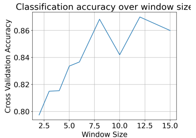
FIGURE 10. Accuracy values across all windows after re-analysis with the five most impactful classification features.
