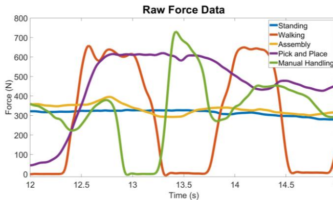
FIGURE 1. A subject's left foot raw data while carrying out all five tasks.
