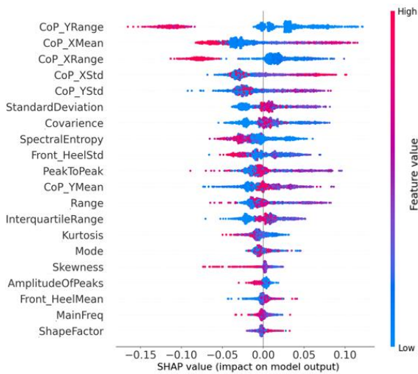
FIGURE 8. SHAP analysis of feature importance for assembly in the 5 second observation window.
