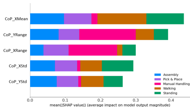
FIGURE 11. Analysis of feature importance for the 5 second observation window and the highest performing features.
