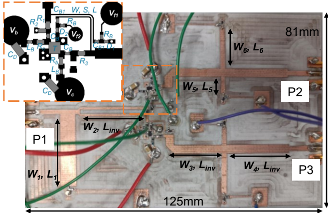
Fig. 4. Photograph of the manufactured QCFS prototype. The UFS components are listed as follows. T: BFU760F, D_1 & D_2 : SMV1405, R_b = 511 \Omega , R_c = 0 \Omega , L_B = 30 \text{ nH} , C_D = 220 \mu\text{F} , C_B = 100 \text{ pF} , C_{B1} = 3 \text{ pF} , R_B = 10 \text{ M}\Omega , R_1 = 57.6 \Omega , R_2 = 14 \Omega , R_3 = 46.4 \Omega , coupled line: W = 0.2 \text{ mm} , S = 0.2 \text{ mm} , L = 11 \text{ mm} . Other dimensions are listed as follows. W_1 = 6.5 \text{ mm} , L_1 = 30 \text{ mm} , W_2 = 1 \text{ mm} , L_{inv} = 26.5 \text{ mm} , W_3 = 3.1 \text{ mm} , W_4 = 3.3 \text{ mm} , W_5 = 1.5 \text{ mm} , L_5 = 7 \text{ mm} , W_6 = 1.9 \text{ mm} , L_6 = 17 \text{ mm} . Varactors in reciprocal resonators: MA46H072 (left side) and four SMV1405s (right side).
