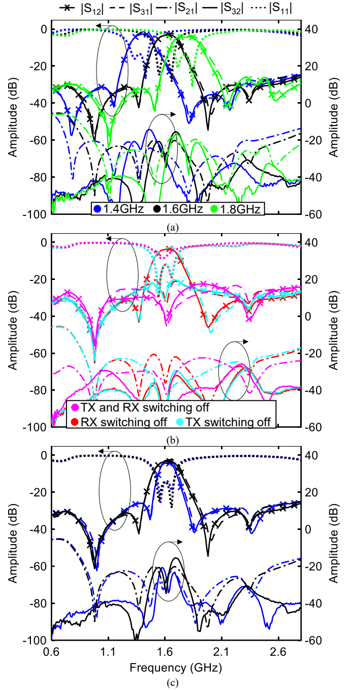
Fig. 5. (a) Measured center frequency tuning, (b) RX/TX switching-off and (c) BW tuning response.
