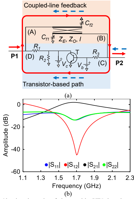
Fig. 2. (a) Circuit schematic of the tunable UFS based on coupled-line feedback. T: BFU760F, V_b = 0.78 V, V_c = 0.8 V, C_{f1} = 1.14 pF, C_{f2} = 1.1 pF, R_1 = 63.5 \Omega , R_2 = 18 \Omega , R_3 = 58 \Omega , Z_E = 163 \Omega , Z_O = 64 \Omega , l = 36^\circ at 1.7 GHz. (b) Circuit-simulated S-parameters of the UFS at 1.7 GHz.
