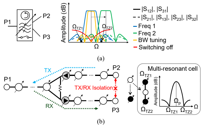
Fig. 1. (a) Symbol of QCFS and its conceptual power transmission and isolation responses demonstrating center frequency, BW tunability, and switch-off capability, and (b) block diagram of tunable RF co-designed QCFS based on a Wilkinson power divider, transistor-based unilateral frequency-selective stages (grey circle with triangle) and passive resonators (white circle), which can be simple resonators or multi-resonant cells.
