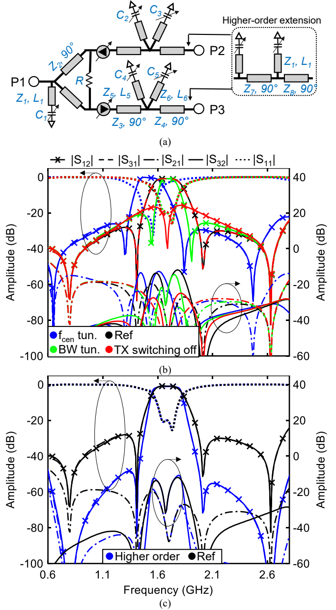
Fig. 3. (a) Block diagram of reference QCFS that comprises two UFS, one half-wavelength and two multi-resonant microstrip resonators, with option of high-order extension. (b) Circuit-simulated center-frequency, BW tuning, TX switching off responses of (a). (c) Comparison with higher-order design. Z_1 = 13.5 \Omega , L_1 = 137^\circ , Z_2 = 61 \Omega , Z_3 = 28 \Omega , Z_4 = 25 \Omega , Z_5 = 55 \Omega , L_5 = 27^\circ , Z_6 = 48 \Omega , L_6 = 55^\circ , Z_7 = 58 \Omega , Z_8 = 52 \Omega , R = 123 \Omega . For Ref case: C_1 = 7.2 pF, C_2 = C_3 = C_4 = C_5 = 2.3 pF; for f_{\text{cen}} tuning case: V_b = 0.785 V, V_c = 0.56 V, C_{f1} = 1.49 pF, C_{f2} = 1.44 pF, C_1 = 14 pF, C_2 = C_3 = C_4 = C_5 = 2.8 pF; for BW tuning case: C_2 = C_4 = 2.6 pF, C_3 = C_5 = 1.8 pF; for TX switching off case: C_2 = 3.4 pF, C_3 = 1.4 pF.
