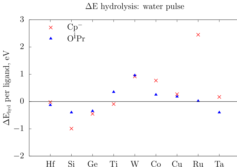
Figure 7.4: \Delta E of hydrolysis reaction during the water pulse. Surface with \text{Cp}^- or \text{O}^i\text{Pr} groups after the successful ligand-exchange process during the precursor pulse are represented by molecules m_1\text{Cp}(\text{dma})_{x-1} and m_1(\text{O}^i\text{Pr})_x , respectively. m_2 = \text{Hf, Si, Ge, Ti, W, Co, Cu, Ru, Ta} . x=4 for Hf, Si, Ge, Ti, W, x=2 for Co, Cu, Ru and x=1 for Ta. \Delta E_{\text{hyd}} values are shown in Table 7.2.
