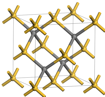
Figure 3.2: Silicon carbide bulk unit cell. Colour schemes: yellow=silicon, grey=carbon.
