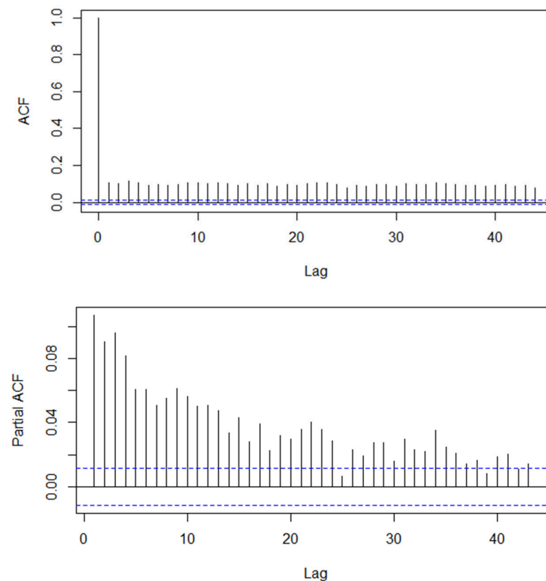
Figure A3. Auto-correlation (dashed lines indicate the approximate 95% confidence limits for zero autocorrelation; spikes outside these limits suggest statistically notable residual autocorrelation at the corresponding lag) and partial auto-correlation plots (dashed lines indicate the approximate 95% confidence limits for zero partial autocorrelation; spikes outside these limits suggest statistically notable residual dependence at the corresponding lag) for residuals.
