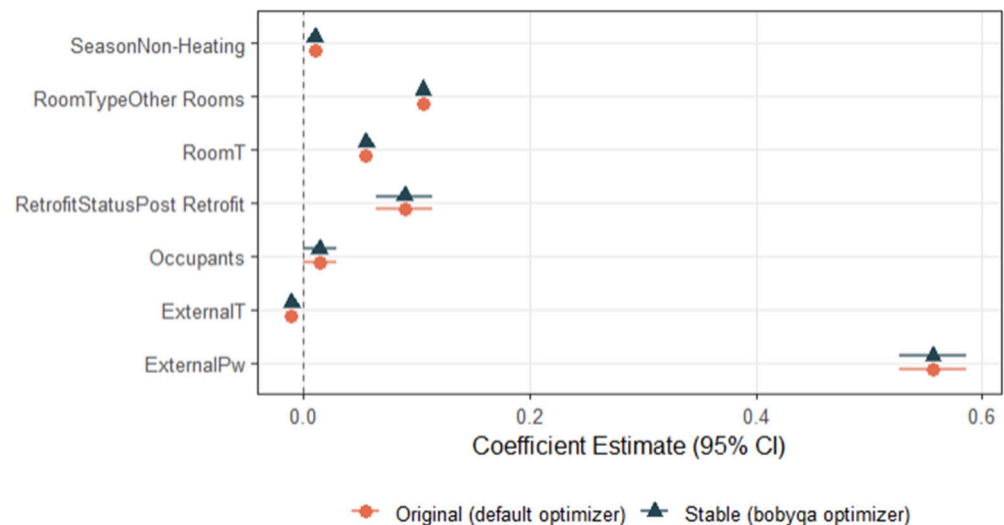
Figure 1. Convergence stability checks for model coefficients—default optimizer compared with Bobyqa optimizer results.
