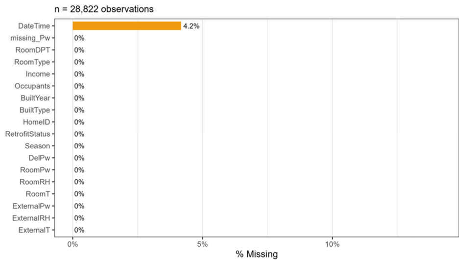
Figure A1. Variable specific missing proportions (Section 2.1.3).
