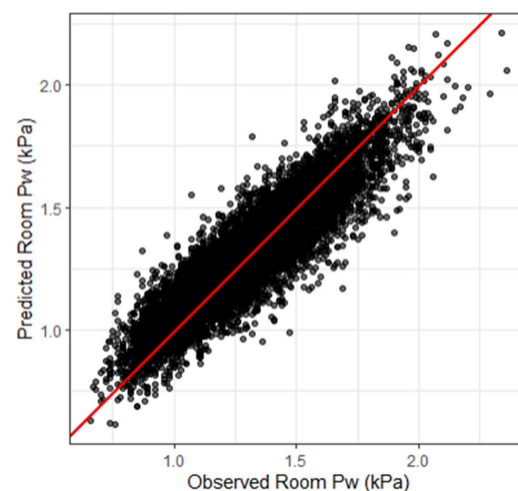
Figure 4. Predicted versus observed indoor vapor pressure (kPa) on the held-out test set (30% of observations, n \approx 8647 ). The model was fitted on the training set (70%) and applied to unseen observations using fixed effect predictions with home-level random effects estimated from training data. The red line denotes perfect agreement (slope = 1, intercept = 0). Test R^2 = 0.817 ; RMSE = 0.110 kPa.
