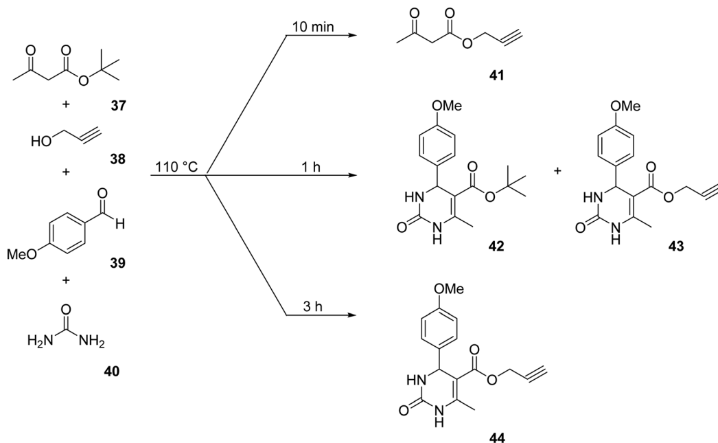
Scheme 10 Pathways to dihydropyrimidin-2(1 H )-one C5 ester derivatives. 129
